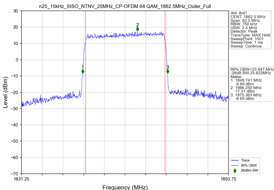
n25_15kHz_SISO_NTNV_25MHz_CP-OFDM 64 QAM_1862.5MHz_Outer_Full
