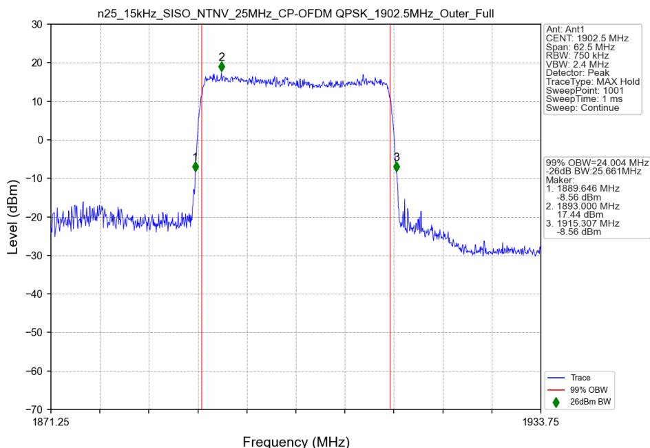
n25_15kHz_SISO_NTNV_25MHz_CP-OFDM QPSK_1902.5MHz_Outer_Full
