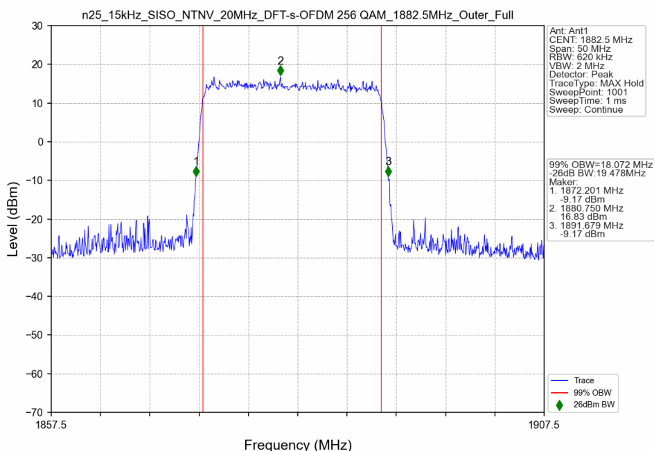
n25_15kHz_SISO_NTNV_20MHz_DFT-s-OFDM 256 QAM_1882.5MHz_Outer_Full
