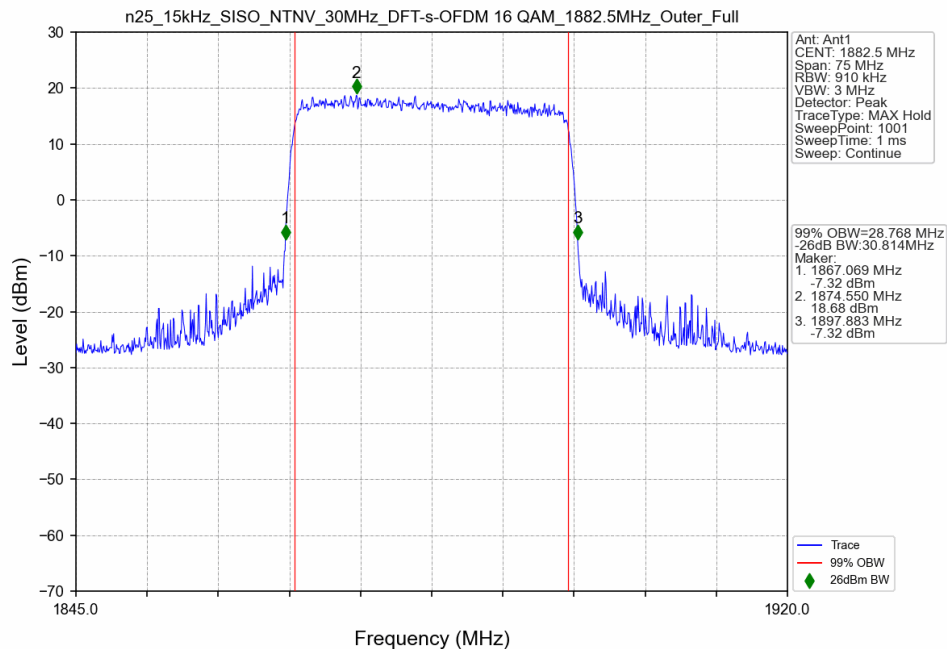
n25_15kHz_SISO_NTNV_30MHz_DFT-s-OFDM 16 QAM_1882.5MHz_Outer_Full
