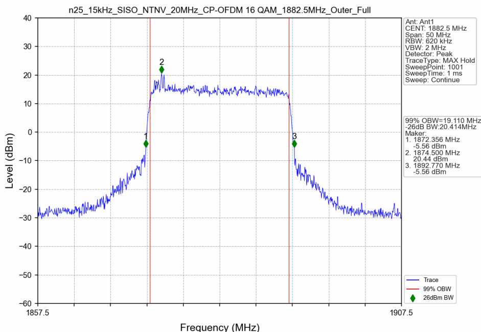
n25_15kHz_SISO_NTNV_20MHz_CP-OFDM 16 QAM_1882.5MHz_Outer_Full
