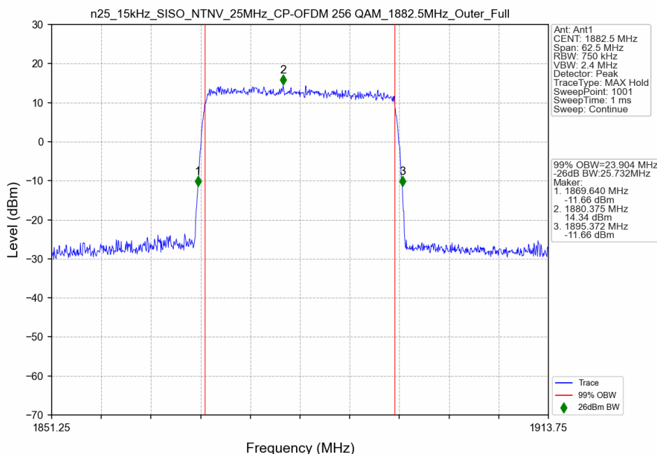
n25_15kHz_SISO_NTNV_25MHz_CP-OFDM 256 QAM_1882.5MHz_Outer_Full
