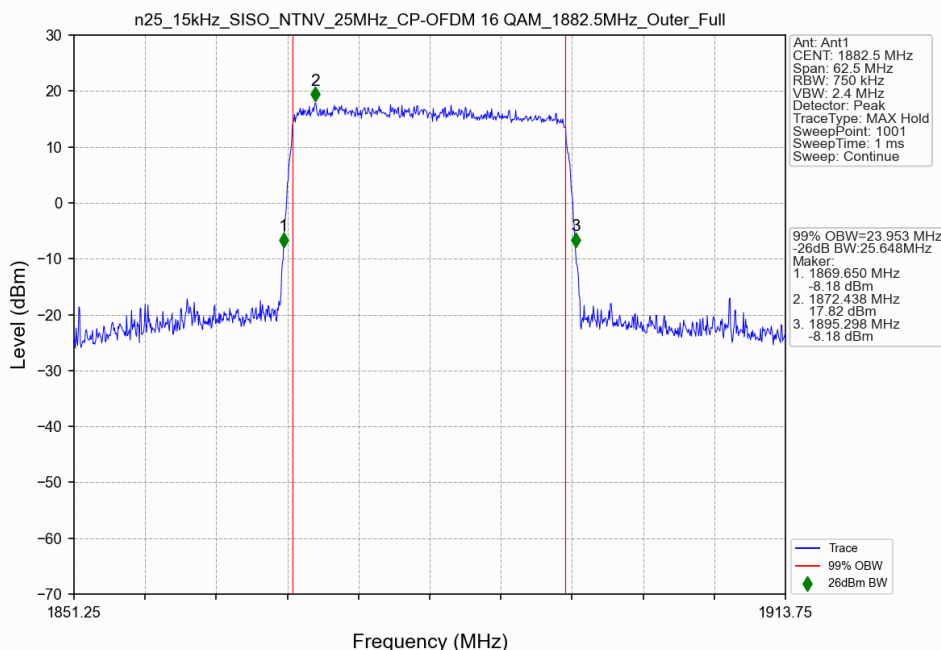
n25_15kHz_SISO_NTNV_25MHz_CP-OFDM 16 QAM_1882.5MHz_Outer_Full
