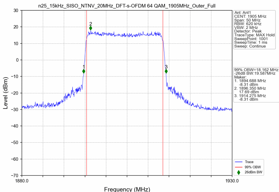
n25_15kHz_SISO_NTNV_20MHz_DFT-s-OFDM 64 QAM_1905MHz_Outer_Full
