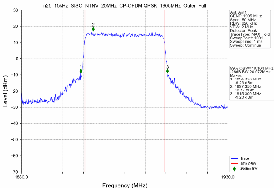
n25_15kHz_SISO_NTNV_20MHz_CP-OFDM QPSK_1905MHz_Outer_Full
