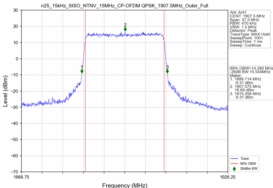
n25_15kHz_SISO_NTNV_15MHz_CP-OFDM QPSK_1907.5MHz_Outer_Full
