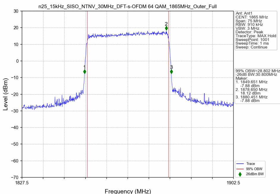
n25_15kHz_SISO_NTNV_30MHz_DFT-s-OFDM 64 QAM_1865MHz_Outer_Full
