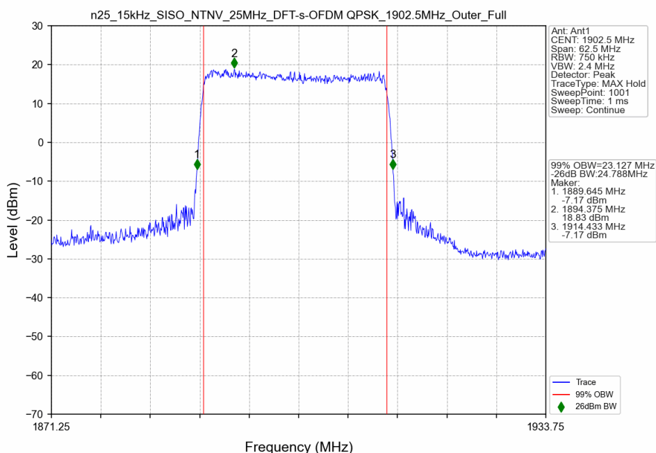
n25_15kHz_SISO_NTNV_25MHz_DFT-s-OFDM QPSK_1902.5MHz_Outer_Full
