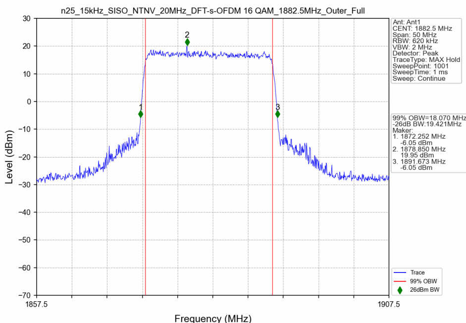
n25_15kHz_SISO_NTNV_20MHz_DFT-s-OFDM 16 QAM_1882.5MHz_Outer_Full
