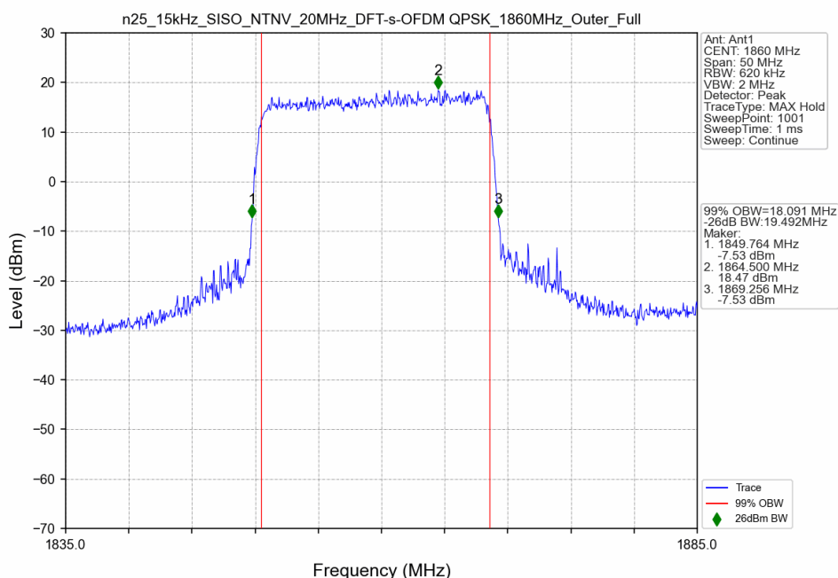
n25_15kHz_SISO_NTNV_20MHz_DFT-s-OFDM QPSK_1860MHz_Outer_Full
