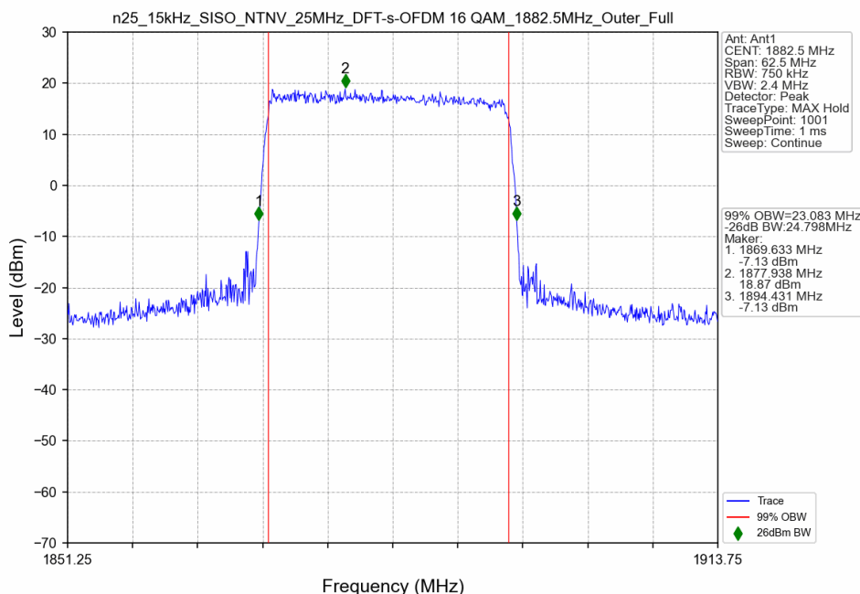
n25_15kHz_SISO_NTNV_25MHz_DFT-s-OFDM 16 QAM_1882.5MHz_Outer_Full
