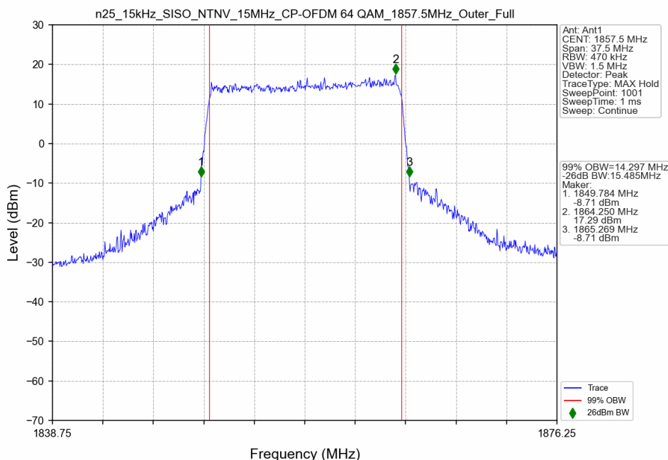
n25_15kHz_SISO_NTNV_15MHz_CP-OFDM 64 QAM_1857.5MHz_Outer_Full
