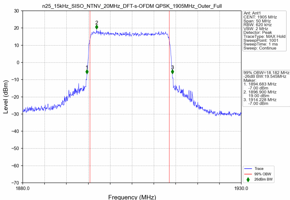
n25_15kHz_SISO_NTNV_20MHz_DFT-s-OFDM QPSK_1905MHz_Outer_Full
