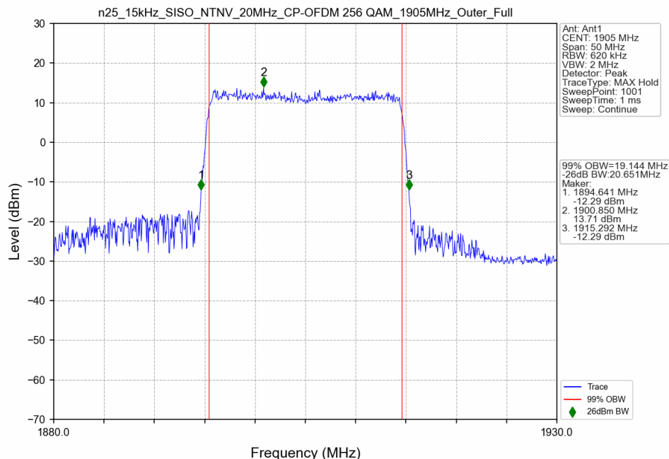
n25_15kHz_SISO_NTNV_20MHz_CP-OFDM 256 QAM_1905MHz_Outer_Full
