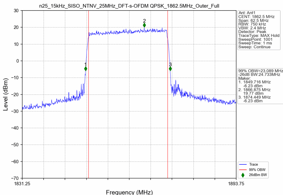
n25_15kHz_SISO_NTNV_25MHz_DFT-s-OFDM QPSK_1862.5MHz_Outer_Full
