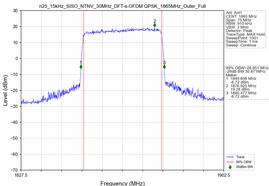
n25_15kHz_SISO_NTNV_30MHz_DFT-s-OFDM QPSK_1865MHz_Outer_Full
