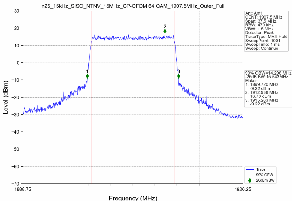
n25_15kHz_SISO_NTNV_15MHz_CP-OFDM 64 QAM_1907.5MHz_Outer_Full
