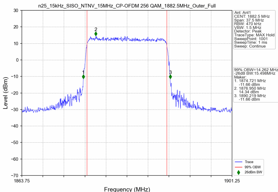
n25_15kHz_SISO_NTNV_15MHz_CP-OFDM 256 QAM_1882.5MHz_Outer_Full
