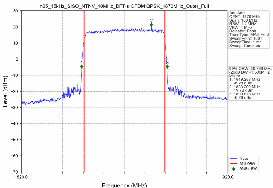
n25_15kHz_SISO_NTNV_40MHz_DFT-s-OFDM QPSK_1870MHz_Outer_Full
