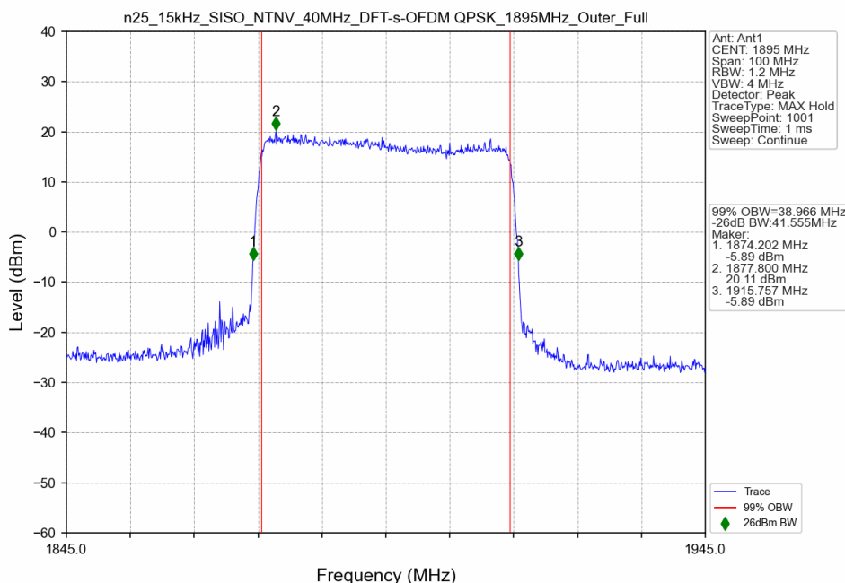
n25_15kHz_SISO_NTNV_40MHz_DFT-s-OFDM QPSK_1895MHz_Outer_Full
