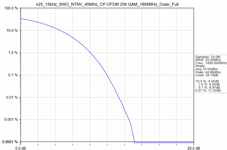
n25_15kHz_SISO_NTNV_40MHz_CP-OFDM 256 QAM_1895MHz_Outer_Full
