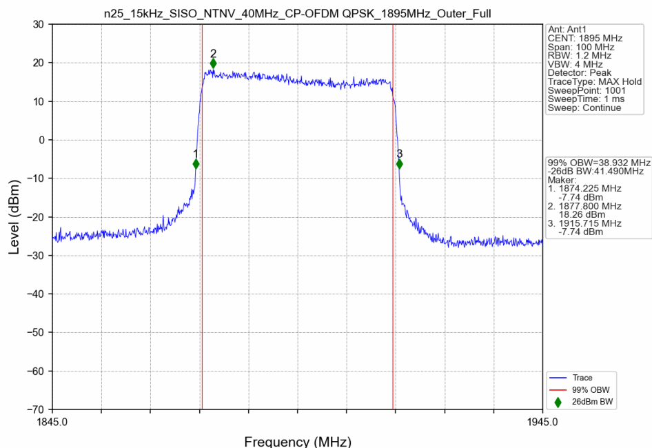
n25_15kHz_SISO_NTNV_40MHz_CP-OFDM QPSK_1895MHz_Outer_Full
