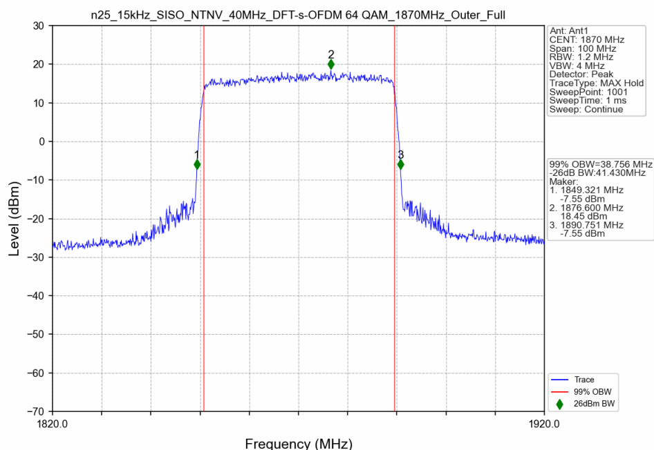
n25_15kHz_SISO_NTNV_40MHz_DFT-s-OFDM 64 QAM_1870MHz_Outer_Full
