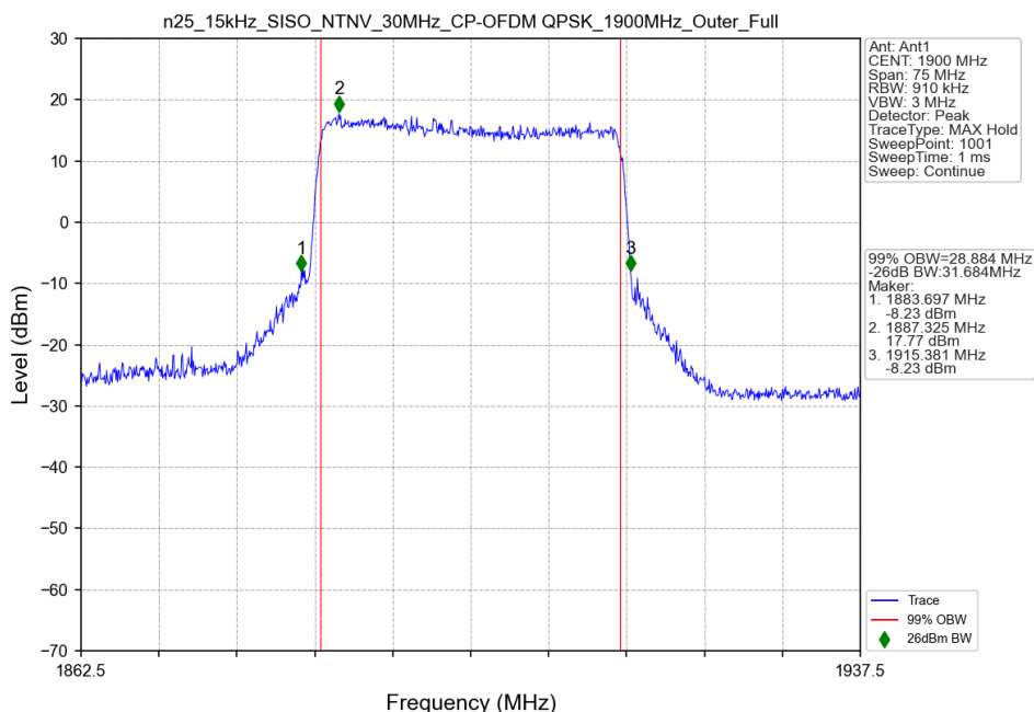
n25_15kHz_SISO_NTNV_30MHz_CP-OFDM QPSK_1900MHz_Outer_Full
