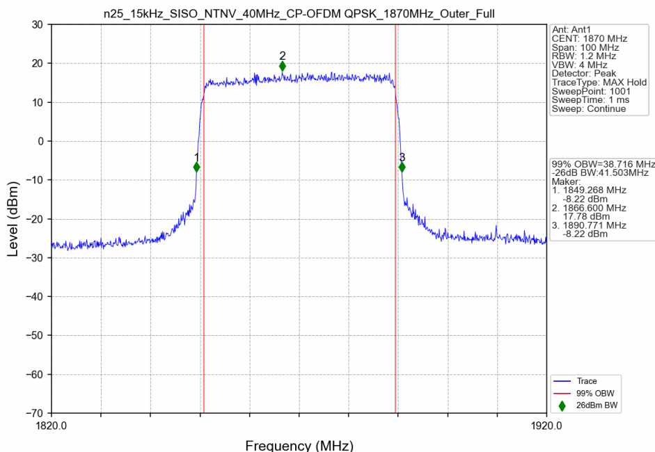
n25_15kHz_SISO_NTNV_40MHz_CP-OFDM QPSK_1870MHz_Outer_Full
