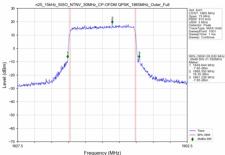
n25_15kHz_SISO_NTNV_30MHz_CP-OFDM QPSK_1865MHz_Outer_Full
