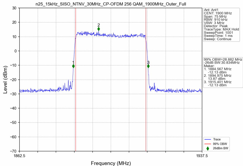
n25_15kHz_SISO_NTNV_30MHz_CP-OFDM 256 QAM_1900MHz_Outer_Full
