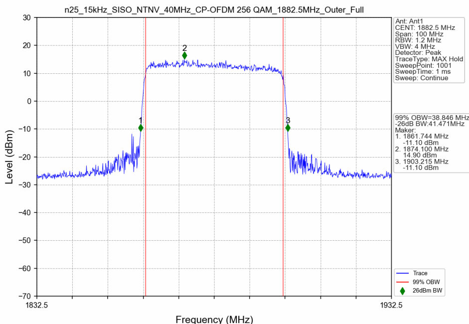
n25_15kHz_SISO_NTNV_40MHz_CP-OFDM 256 QAM_1882.5MHz_Outer_Full
