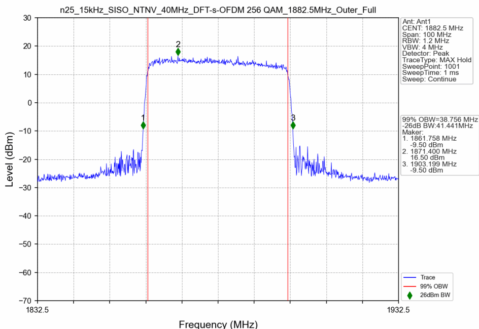
n25_15kHz_SISO_NTNV_40MHz_DFT-s-OFDM 256 QAM_1882.5MHz_Outer_Full
