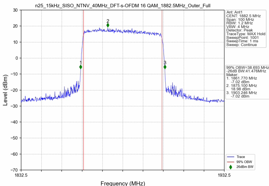
n25_15kHz_SISO_NTNV_40MHz_DFT-s-OFDM 16 QAM_1882.5MHz_Outer_Full
