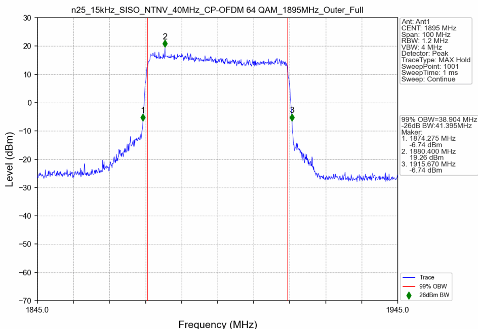
n25_15kHz_SISO_NTNV_40MHz_CP-OFDM 64 QAM_1895MHz_Outer_Full
