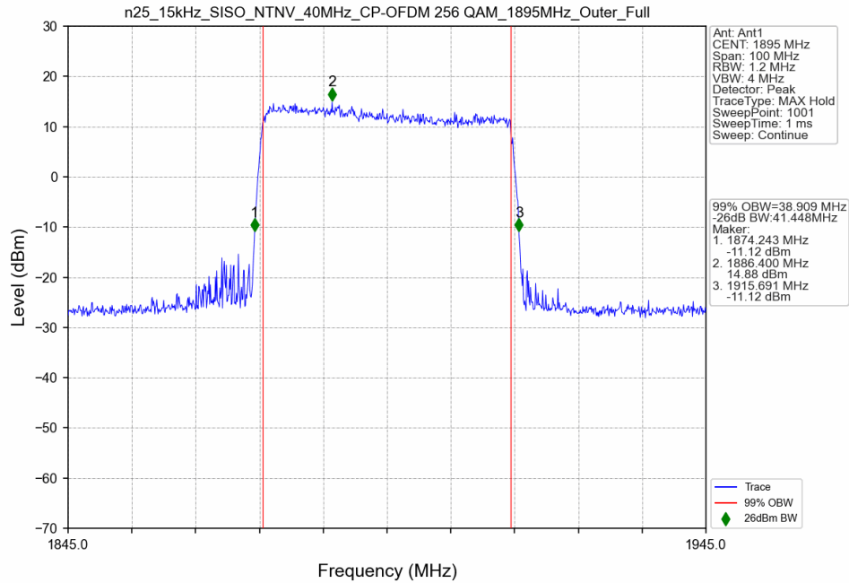
n25_15kHz_SISO_NTNV_40MHz_CP-OFDM 256 QAM_1895MHz_Outer_Full
