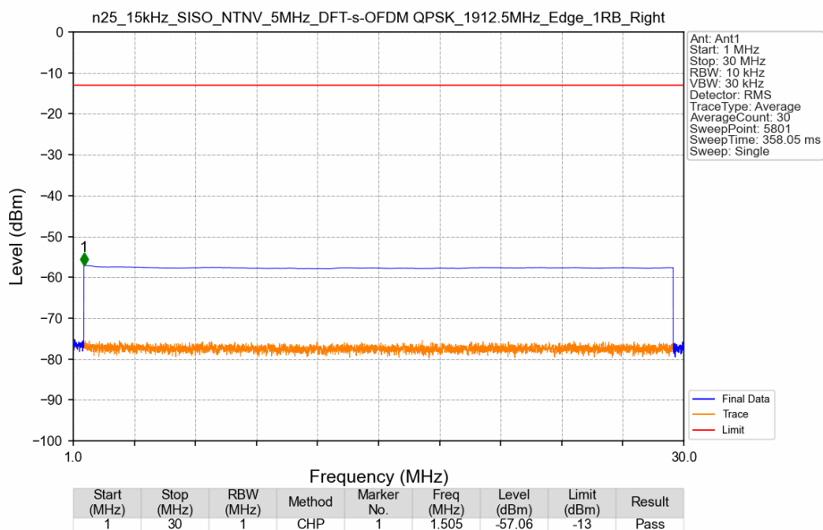
n25_15kHz_SISO_NTNV_5MHz_DFT-s-OFDM QPSK_1912.5MHz_Edge_1RB_Right
