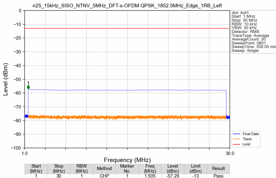
n25_15kHz_SISO_NTNV_5MHz_DFT-s-OFDM QPSK_1852.5MHz_Edge_1RB_Left
