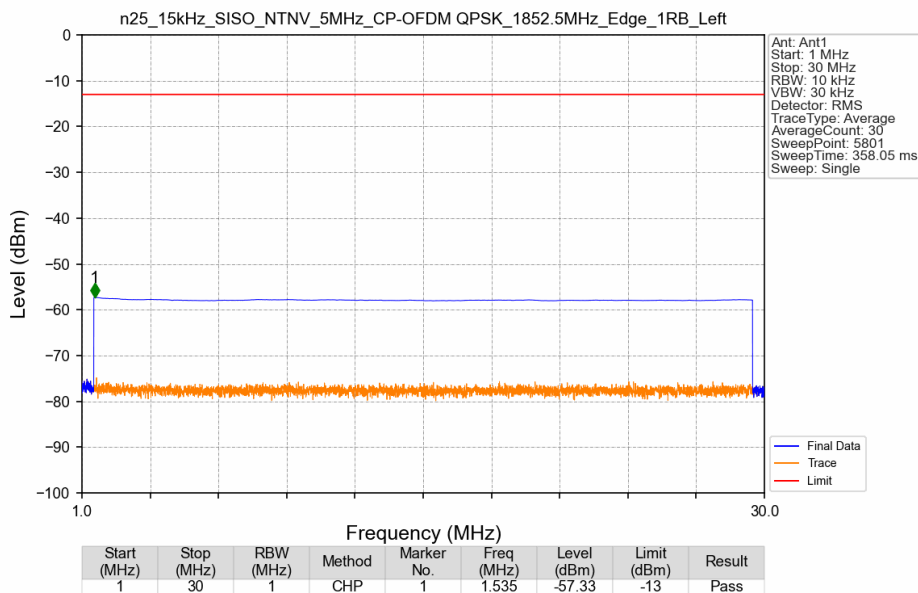
n25_15kHz_SISO_NTNV_5MHz_CP-OFDM QPSK_1852.5MHz_Edge_1RB_Left
