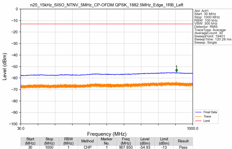
n25_15kHz_SISO_NTNV_5MHz_CP-OFDM QPSK_1882.5MHz_Edge_1RB_Left
