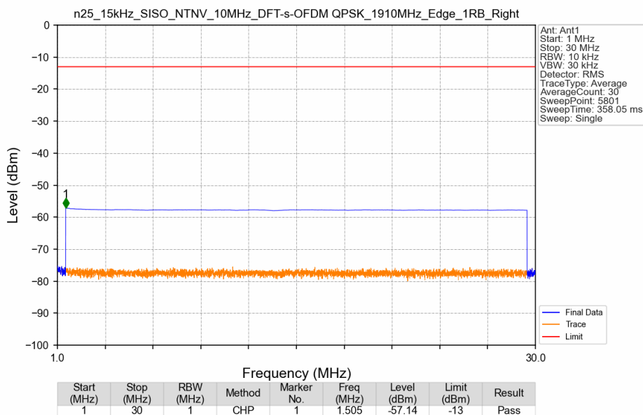
n25_15kHz_SISO_NTNV_10MHz_DFT-s-OFDM QPSK_1910MHz_Edge_1RB_Right
