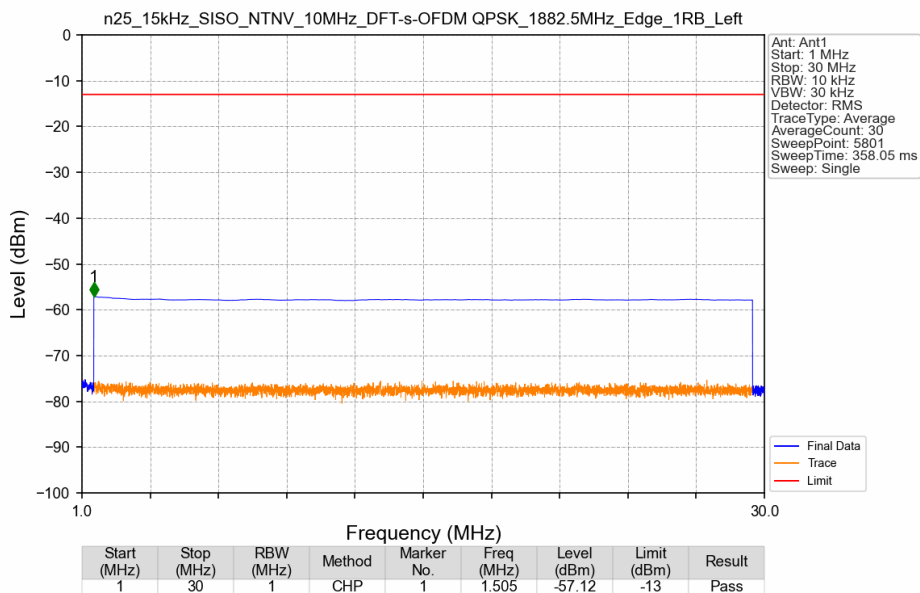
n25_15kHz_SISO_NTNV_10MHz_DFT-s-OFDM QPSK_1882.5MHz_Edge_1RB_Left
