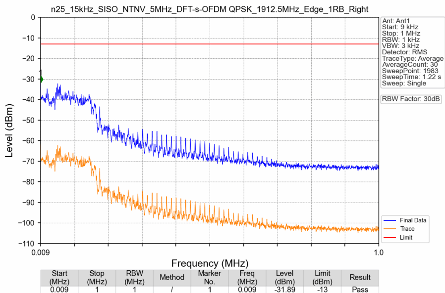
n25_15kHz_SISO_NTNV_5MHz_DFT-s-OFDM QPSK_1912.5MHz_Edge_1RB_Right
