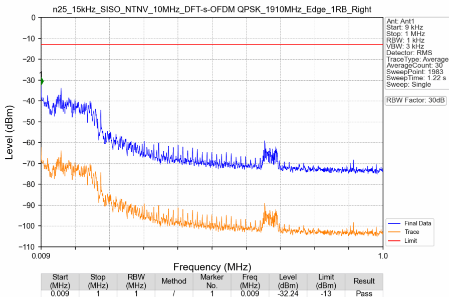
n25_15kHz_SISO_NTNV_10MHz_DFT-s-OFDM QPSK_1910MHz_Edge_1RB_Right
