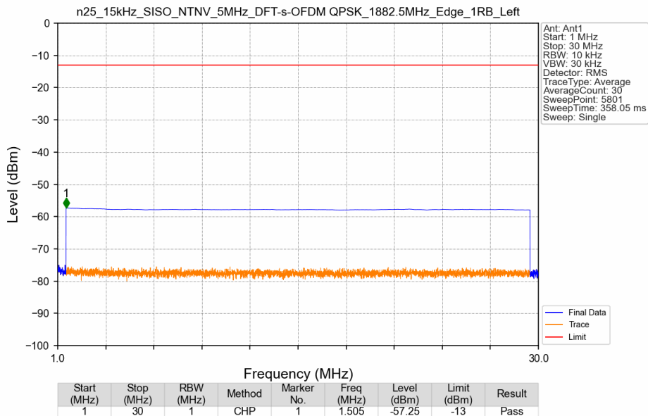
n25_15kHz_SISO_NTNV_5MHz_DFT-s-OFDM QPSK_1882.5MHz_Edge_1RB_Left
