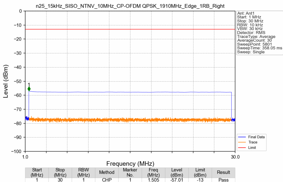
n25_15kHz_SISO_NTNV_10MHz_CP-OFDM QPSK_1910MHz_Edge_1RB_Right
