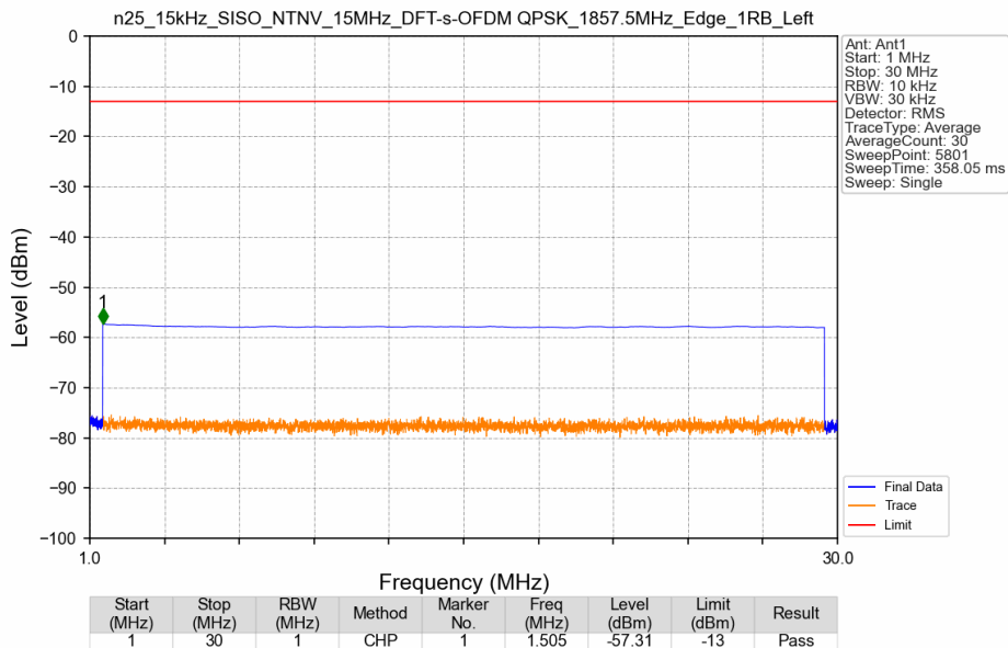
n25_15kHz_SISO_NTNV_15MHz_DFT-s-OFDM QPSK_1857.5MHz_Edge_1RB_Left
