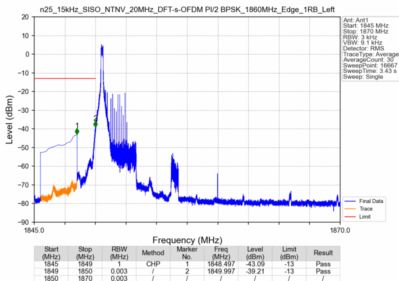
n25_15kHz_SISO_NTNV_20MHz_DFT-s-OFDM PI/2 BPSK_1860MHz_Edge_1RB_Left
