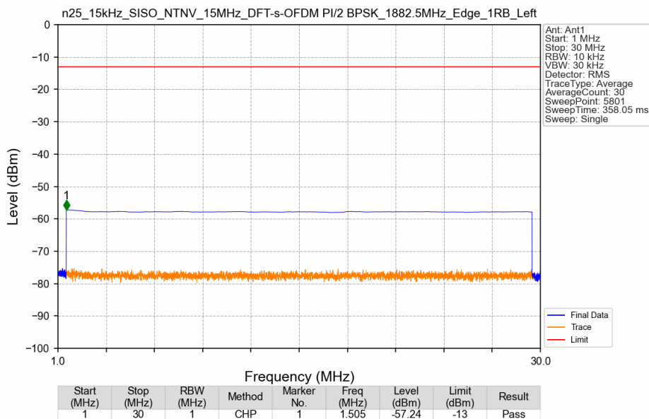
n25_15kHz_SISO_NTNV_15MHz_DFT-s-OFDM PI/2 BPSK_1882.5MHz_Edge_1RB_Left
