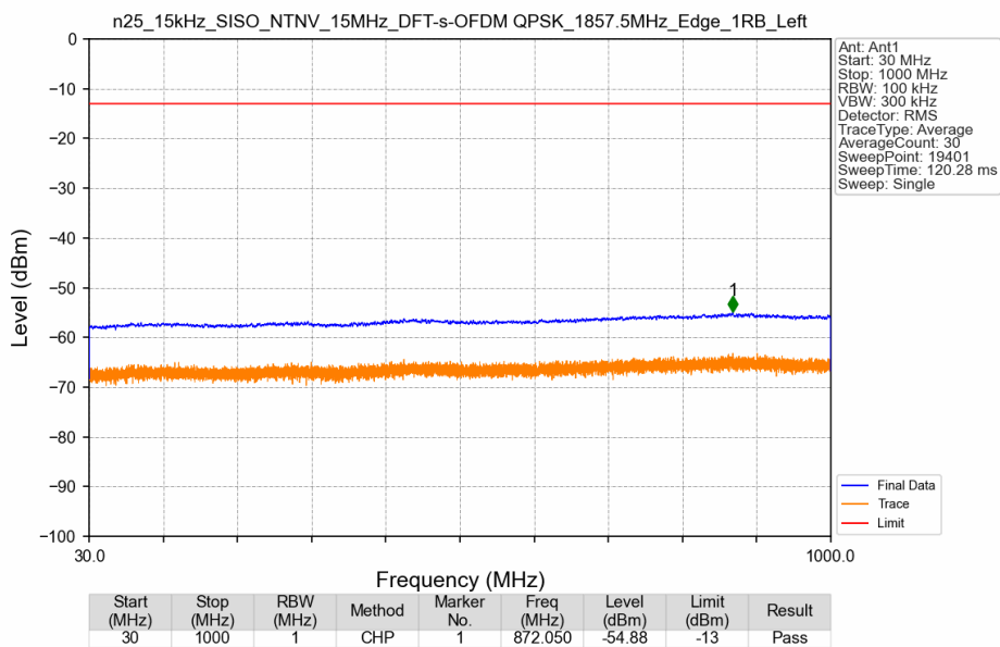
n25_15kHz_SISO_NTNV_15MHz_DFT-s-OFDM QPSK_1857.5MHz_Edge_1RB_Left
