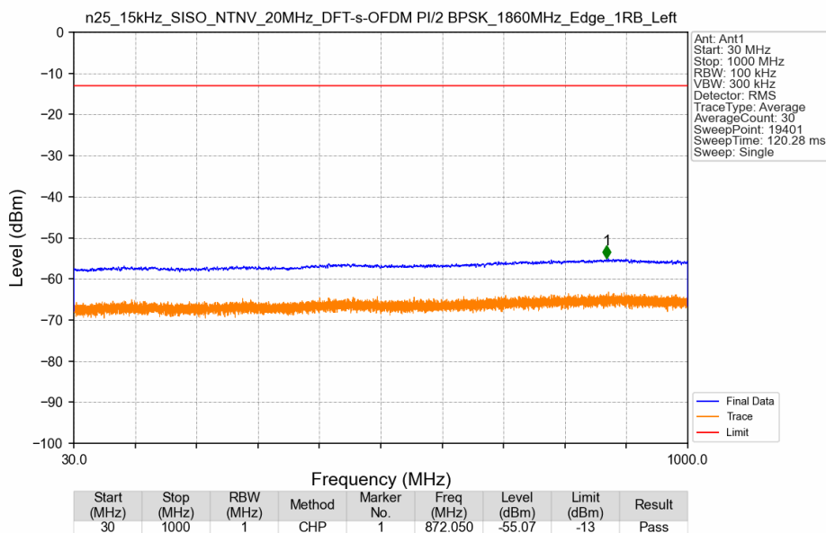
n25_15kHz_SISO_NTNV_20MHz_DFT-s-OFDM PI/2 BPSK_1860MHz_Edge_1RB_Left
