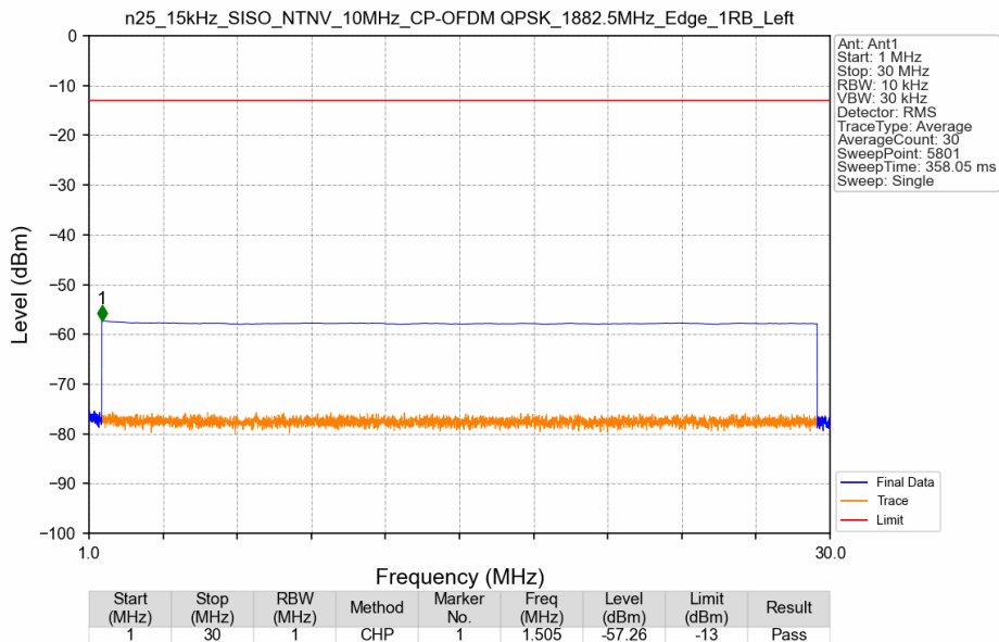
n25_15kHz_SISO_NTNV_10MHz_CP-OFDM QPSK_1882.5MHz_Edge_1RB_Left
