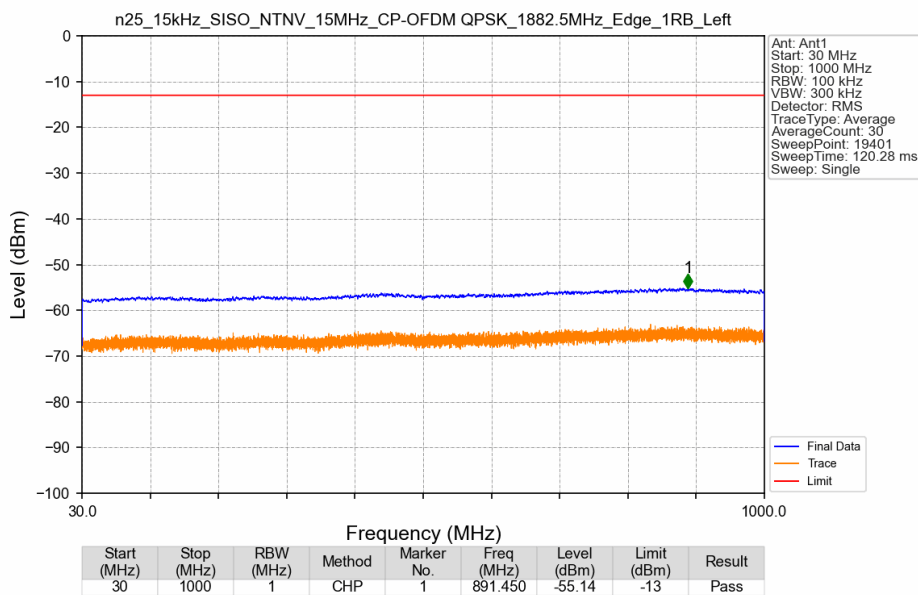
n25_15kHz_SISO_NTNV_15MHz_CP-OFDM QPSK_1882.5MHz_Edge_1RB_Left
