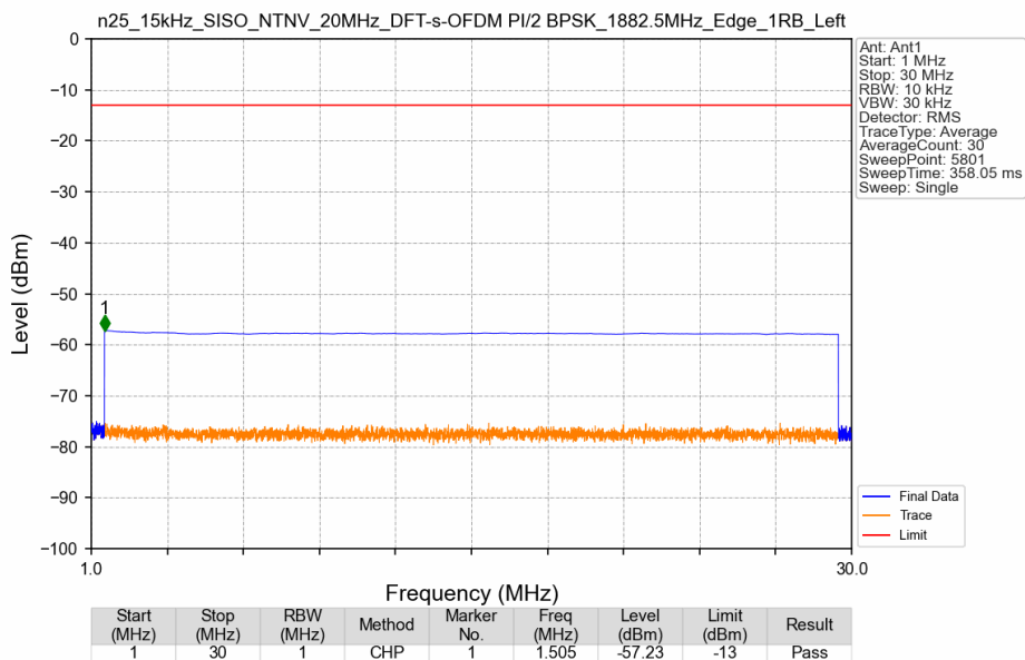
n25_15kHz_SISO_NTNV_20MHz_DFT-s-OFDM PI/2 BPSK_1882.5MHz_Edge_1RB_Left
