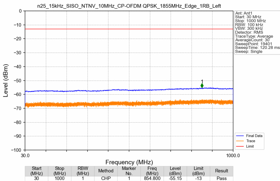
n25_15kHz_SISO_NTNV_10MHz_CP-OFDM QPSK_1855MHz_Edge_1RB_Left
