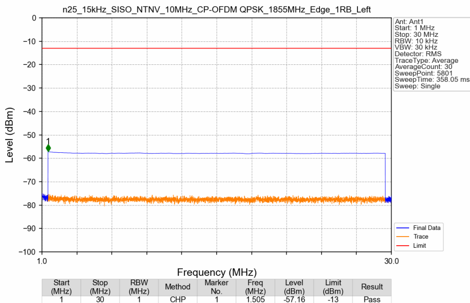
n25_15kHz_SISO_NTNV_10MHz_CP-OFDM QPSK_1855MHz_Edge_1RB_Left
