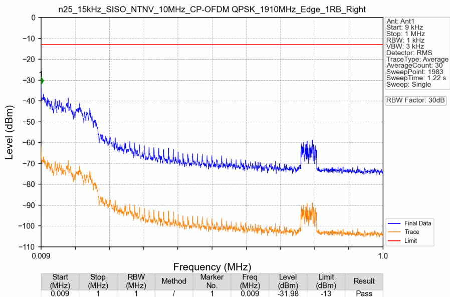
n25_15kHz_SISO_NTNV_10MHz_CP-OFDM QPSK_1910MHz_Edge_1RB_Right
