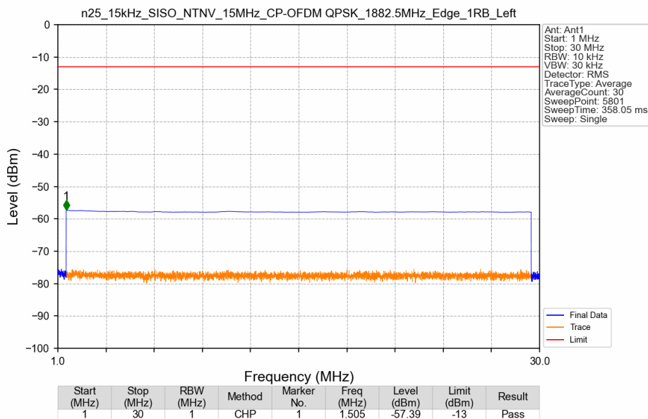
n25_15kHz_SISO_NTNV_15MHz_CP-OFDM QPSK_1882.5MHz_Edge_1RB_Left
