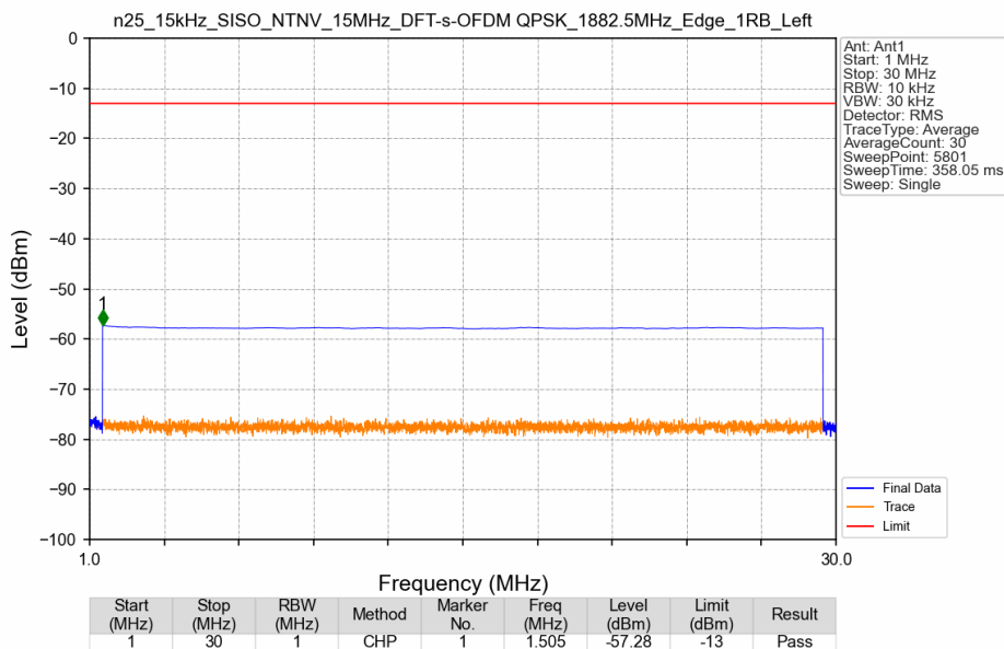
n25_15kHz_SISO_NTNV_15MHz_DFT-s-OFDM QPSK_1882.5MHz_Edge_1RB_Left
