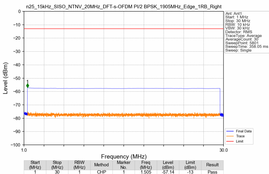
n25_15kHz_SISO_NTNV_20MHz_DFT-s-OFDM PI/2 BPSK_1905MHz_Edge_1RB_Right
