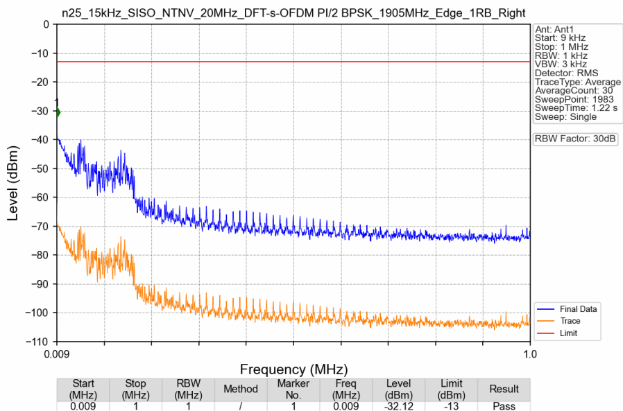
n25_15kHz_SISO_NTNV_20MHz_DFT-s-OFDM PI/2 BPSK_1905MHz_Edge_1RB_Right
