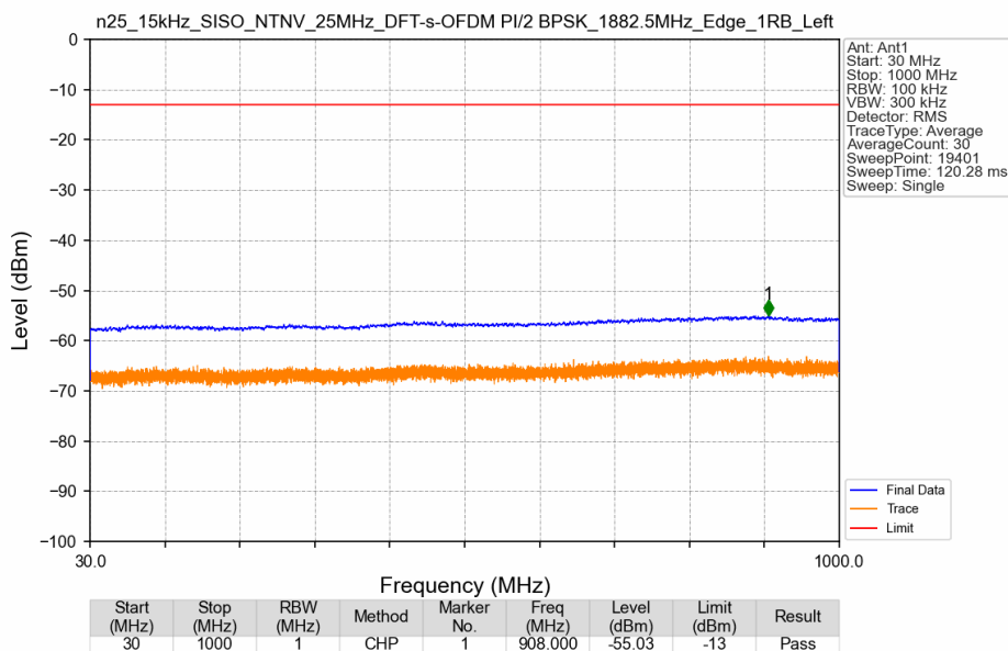
n25_15kHz_SISO_NTNV_25MHz_DFT-s-OFDM PI/2 BPSK_1882.5MHz_Edge_1RB_Left
