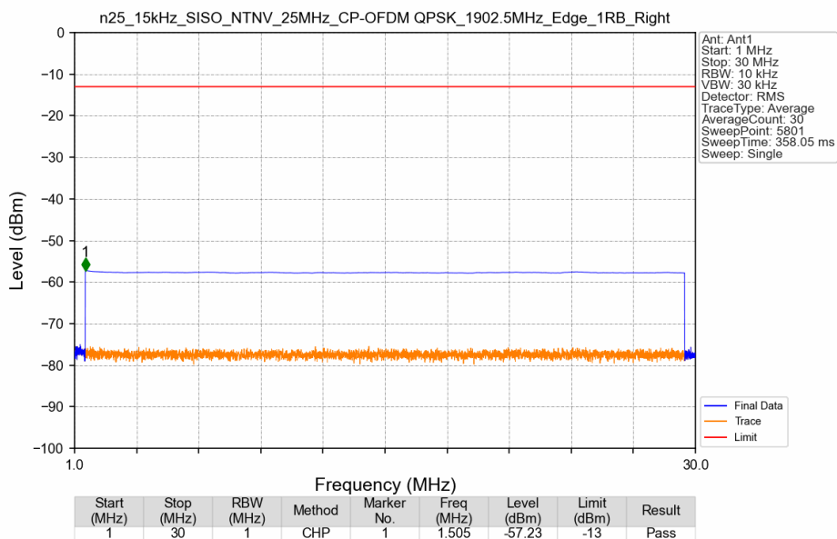
n25_15kHz_SISO_NTNV_25MHz_CP-OFDM QPSK_1902.5MHz_Edge_1RB_Right
