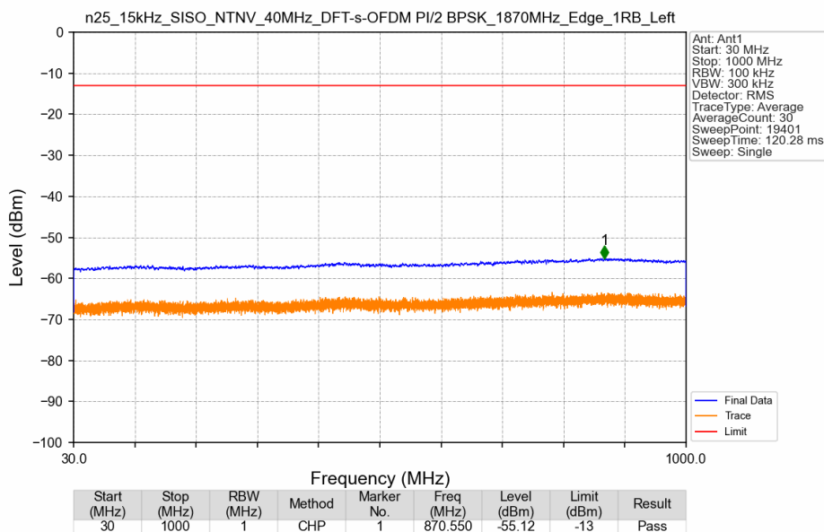
n25_15kHz_SISO_NTNV_40MHz_DFT-s-OFDM PI/2 BPSK_1870MHz_Edge_1RB_Left
