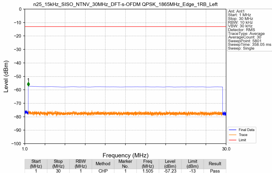
n25_15kHz_SISO_NTNV_30MHz_DFT-s-OFDM QPSK_1865MHz_Edge_1RB_Left
