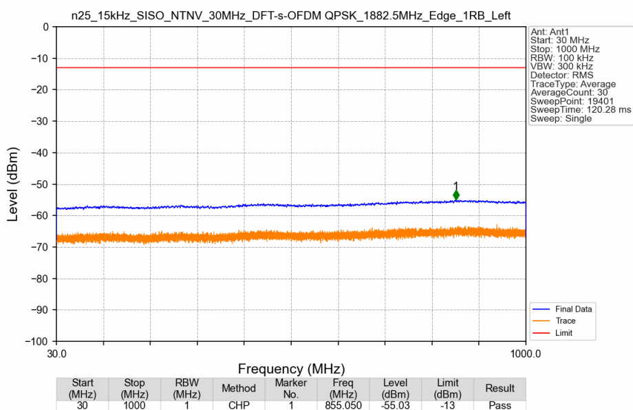
n25_15kHz_SISO_NTNV_30MHz_DFT-s-OFDM QPSK_1882.5MHz_Edge_1RB_Left
