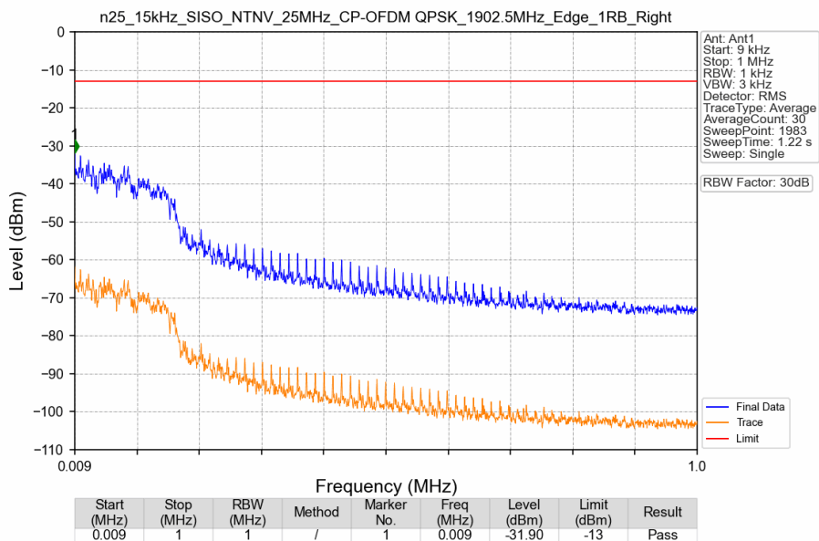
n25_15kHz_SISO_NTNV_25MHz_CP-OFDM QPSK_1902.5MHz_Edge_1RB_Right
