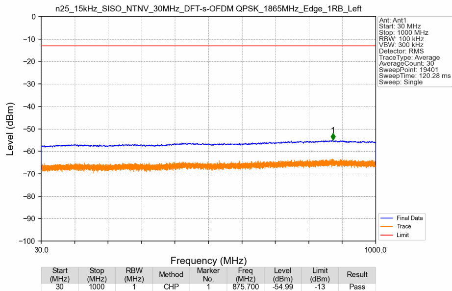
n25_15kHz_SISO_NTNV_30MHz_DFT-s-OFDM QPSK_1865MHz_Edge_1RB_Left
