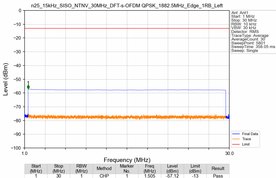
n25_15kHz_SISO_NTNV_30MHz_DFT-s-OFDM QPSK_1882.5MHz_Edge_1RB_Left
