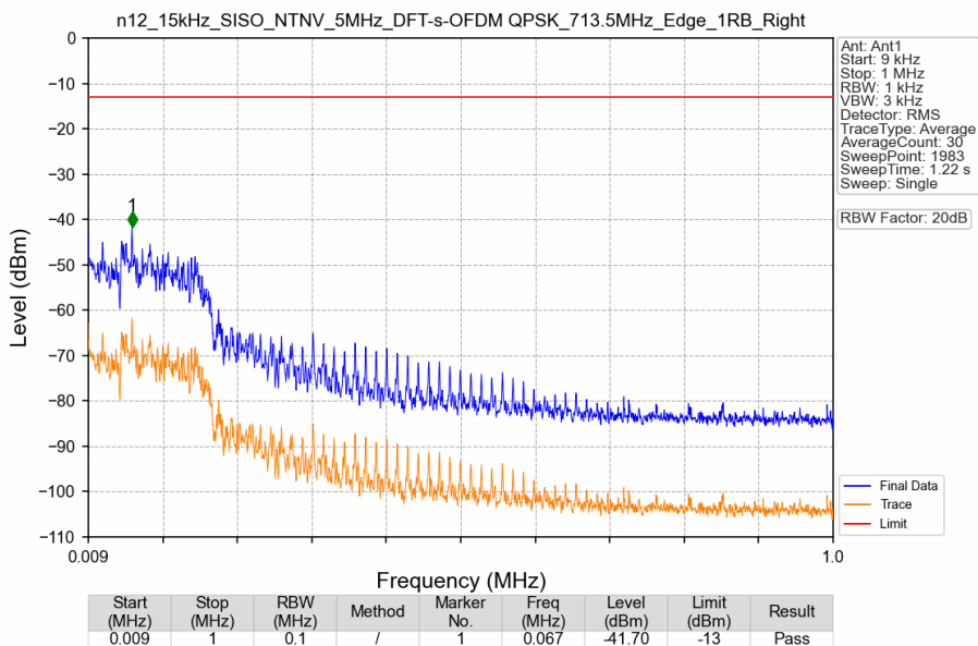
n12_15kHz_SISO_NTNV_5MHz_DFT-s-OFDM QPSK_713.5MHz_Edge_1RB_Right
