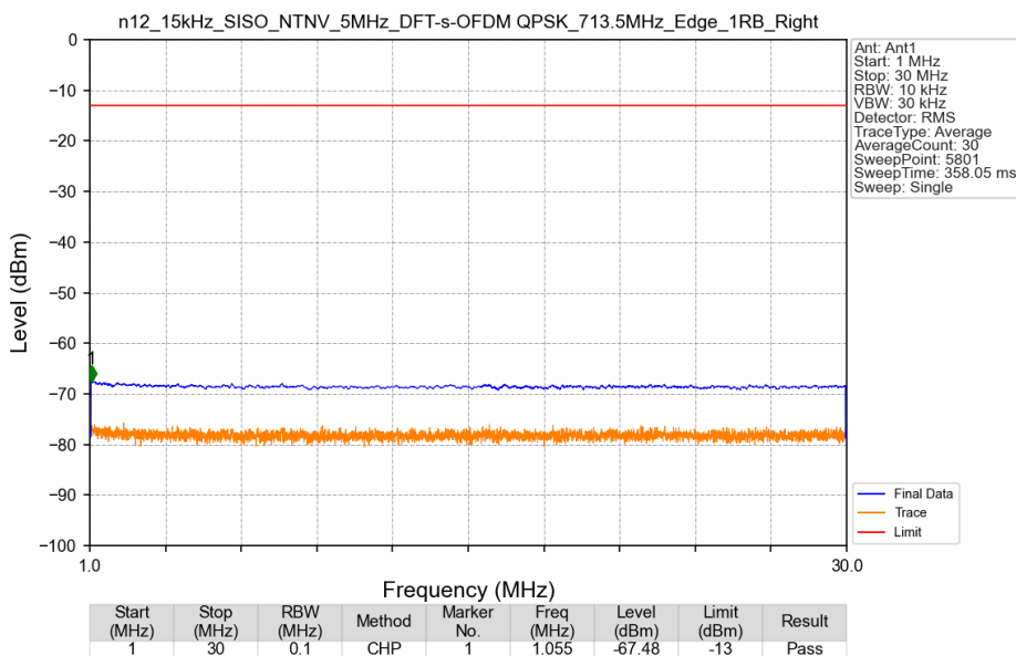
n12_15kHz_SISO_NTNV_5MHz_DFT-s-OFDM QPSK_713.5MHz_Edge_1RB_Right
