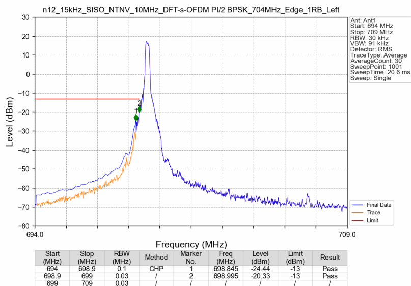
n12_15kHz_SISO_NTNV_10MHz_DFT-s-OFDM PI/2 BPSK_704MHz_Edge_1RB_Left
