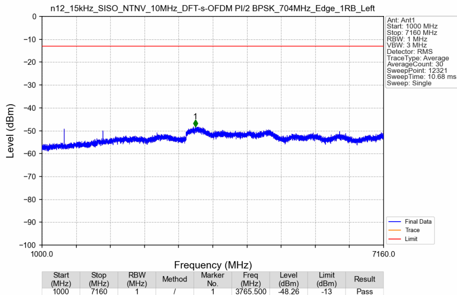
n12_15kHz_SISO_NTNV_10MHz_DFT-s-OFDM PI/2 BPSK_704MHz_Edge_1RB_Left
