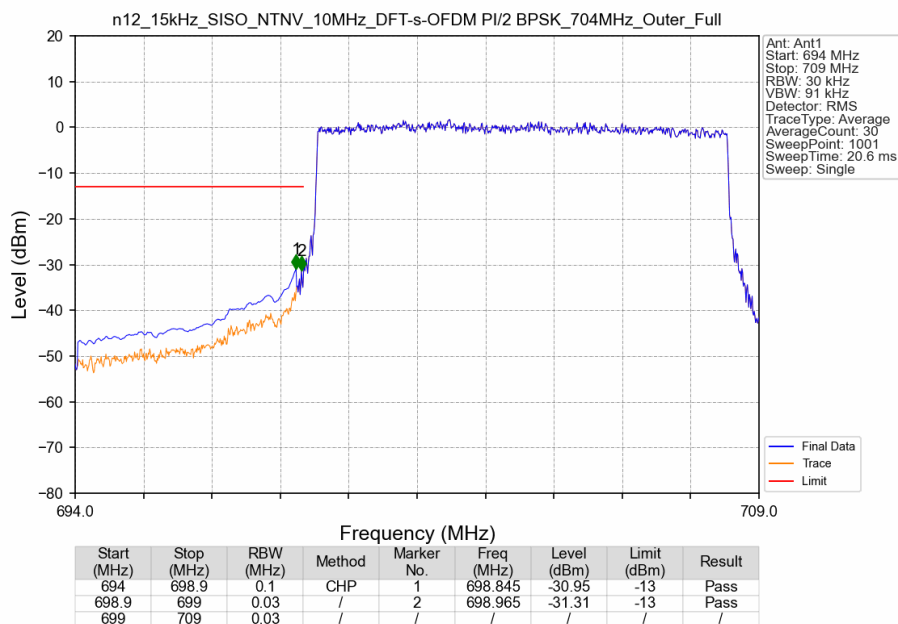
n12_15kHz_SISO_NTNV_10MHz_DFT-s-OFDM PI/2 BPSK_704MHz_Outer_Full
