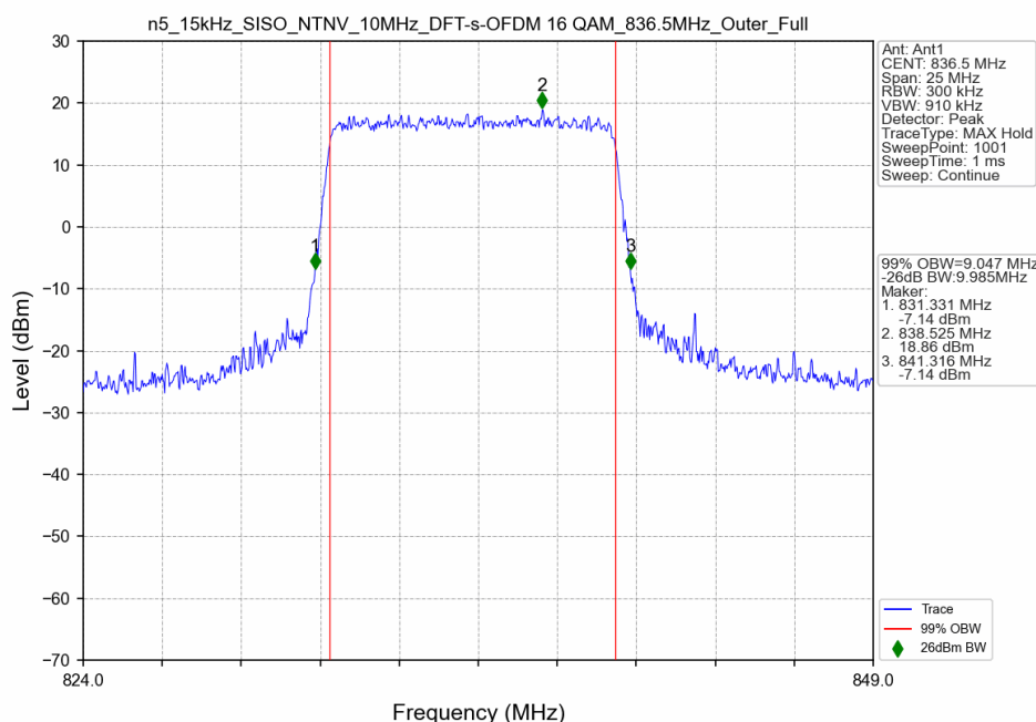
n5_15kHz_SISO_NTNV_10MHz_DFT-s-OFDM 16 QAM_836.5MHz_Outer_Full
