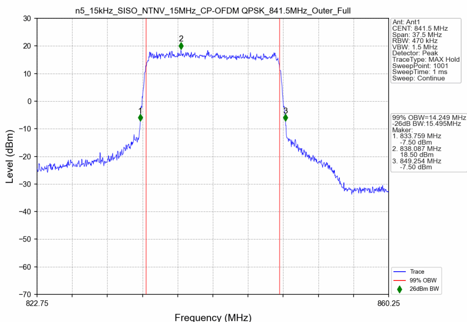
n5_15kHz_SISO_NTNV_15MHz_CP-OFDM QPSK_841.5MHz_Outer_Full
