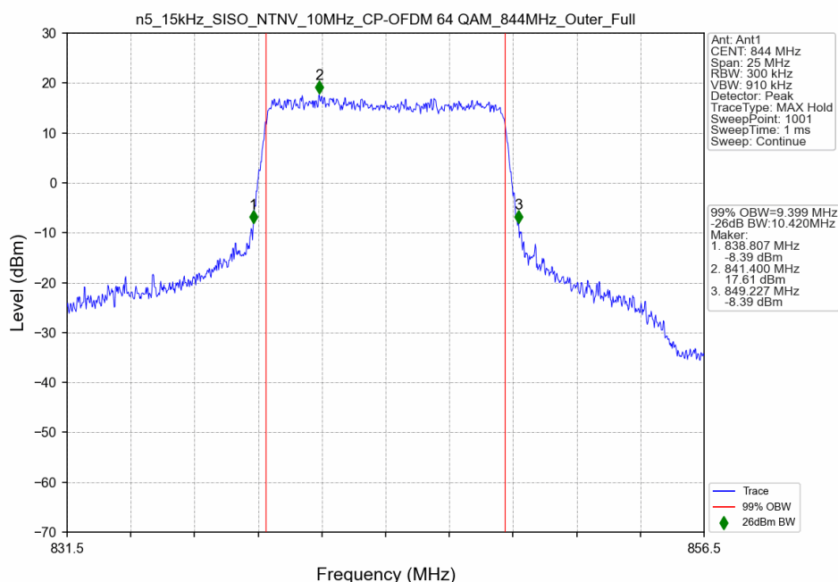
n5_15kHz_SISO_NTNV_10MHz_CP-OFDM 64 QAM_844MHz_Outer_Full
