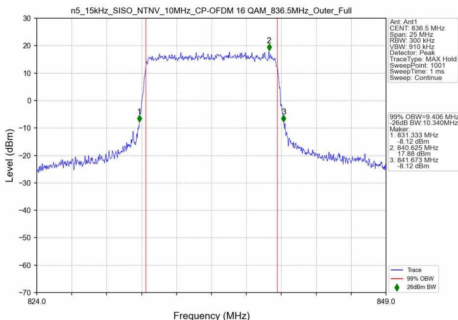
n5_15kHz_SISO_NTNV_10MHz_CP-OFDM 16 QAM_836.5MHz_Outer_Full
