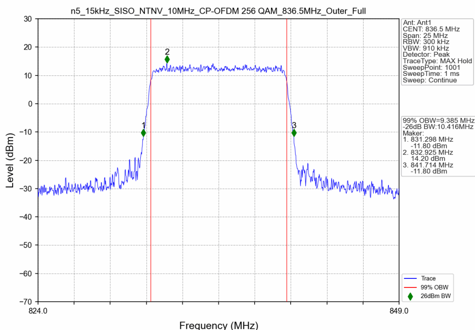
n5_15kHz_SISO_NTNV_10MHz_CP-OFDM 256 QAM_836.5MHz_Outer_Full
