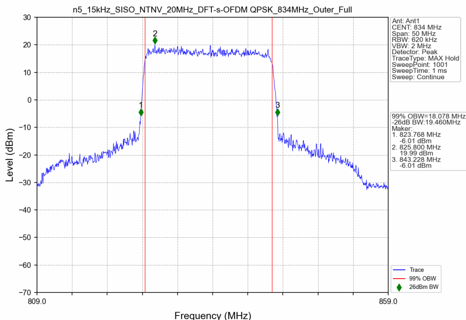
n5_15kHz_SISO_NTNV_20MHz_DFT-s-OFDM QPSK_834MHz_Outer_Full
