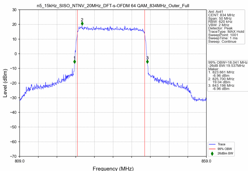
n5_15kHz_SISO_NTNV_20MHz_DFT-s-OFDM 64 QAM_834MHz_Outer_Full
