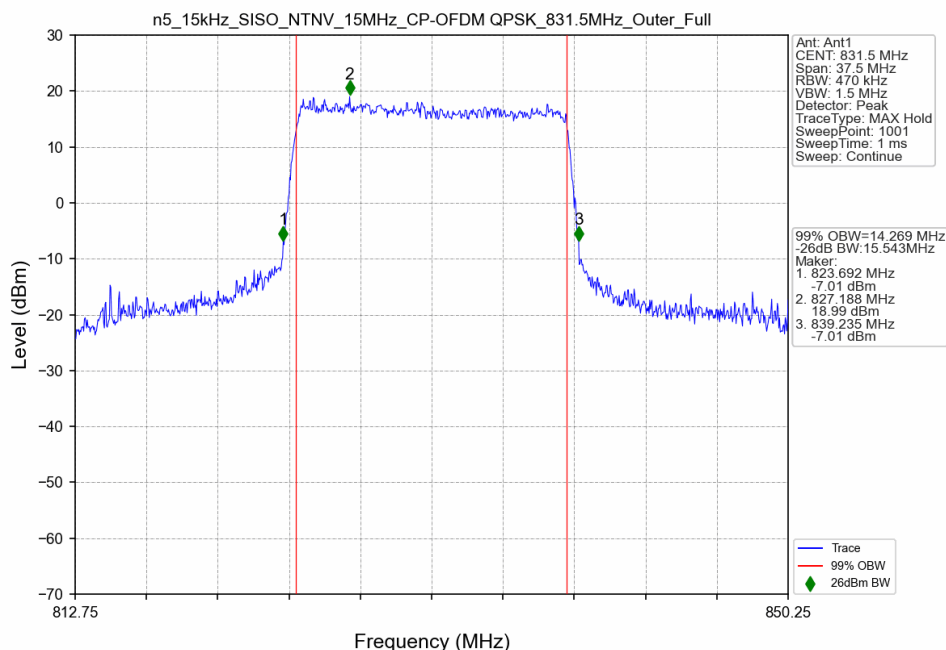
n5_15kHz_SISO_NTNV_15MHz_CP-OFDM QPSK_831.5MHz_Outer_Full
