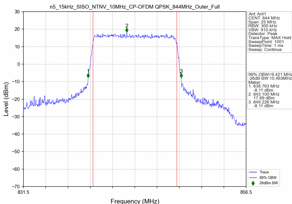
n5_15kHz_SISO_NTNV_10MHz_CP-OFDM QPSK_844MHz_Outer_Full
