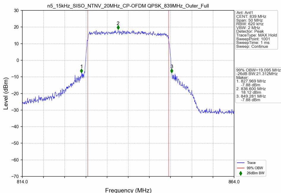
n5_15kHz_SISO_NTNV_20MHz_CP-OFDM QPSK_839MHz_Outer_Full
