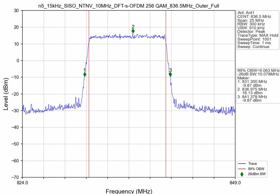
n5_15kHz_SISO_NTNV_10MHz_DFT-s-OFDM 256 QAM_836.5MHz_Outer_Full
