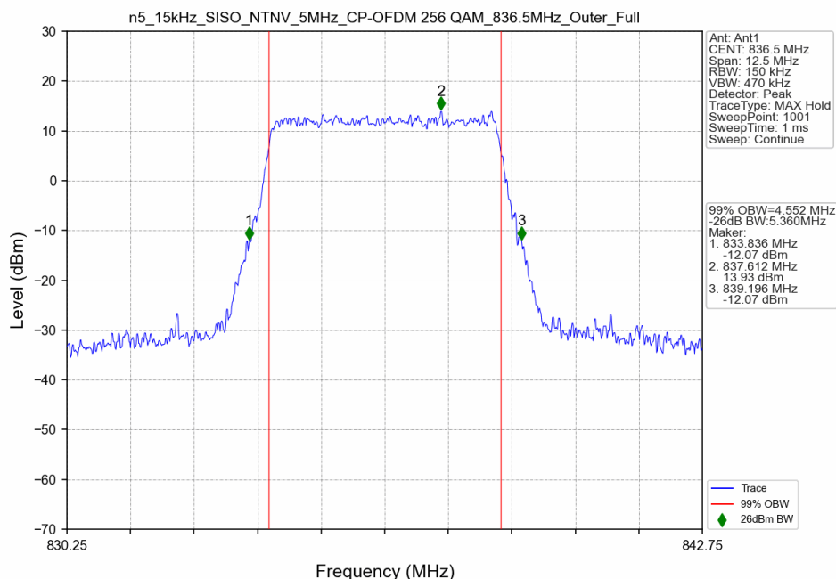
n5_15kHz_SISO_NTNV_5MHz_CP-OFDM 256 QAM_836.5MHz_Outer_Full
