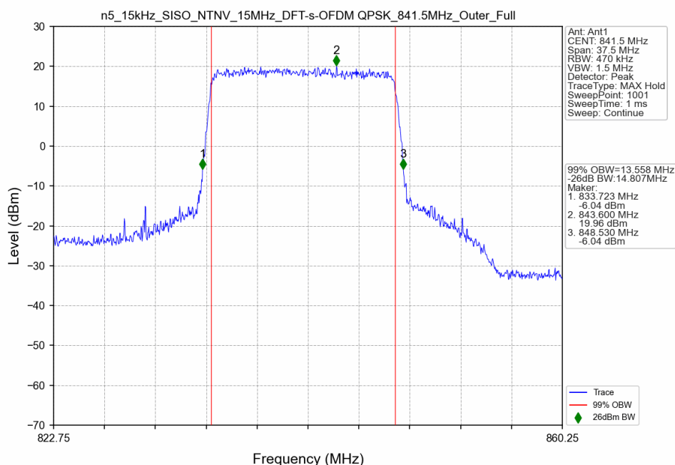
n5_15kHz_SISO_NTNV_15MHz_DFT-s-OFDM QPSK_841.5MHz_Outer_Full
