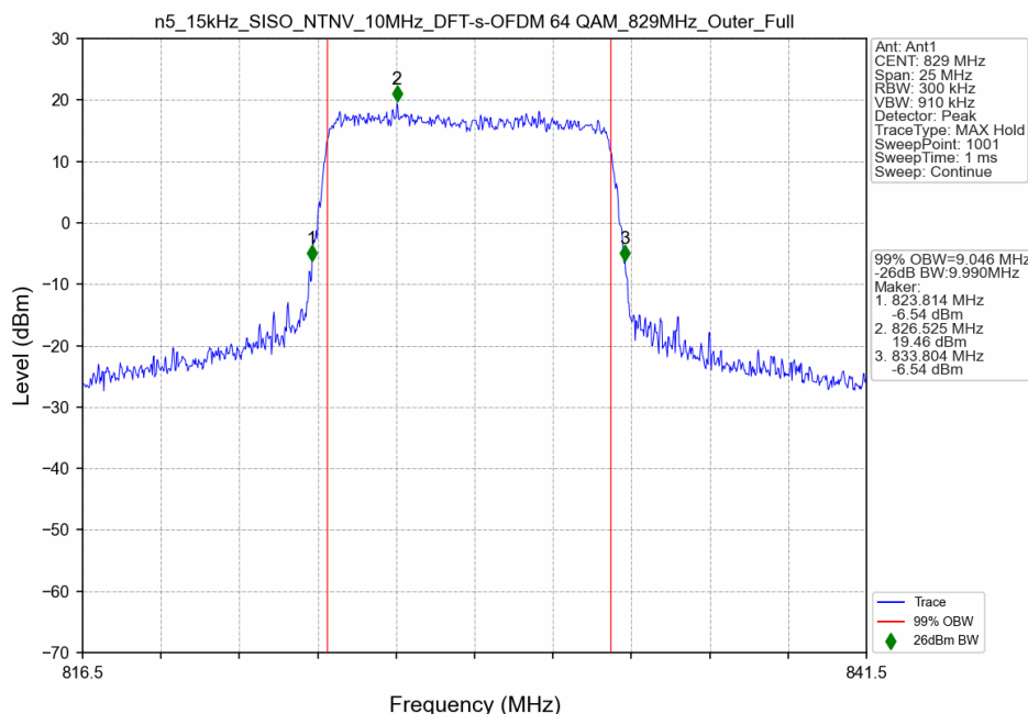
n5_15kHz_SISO_NTNV_10MHz_DFT-s-OFDM 64 QAM_829MHz_Outer_Full
