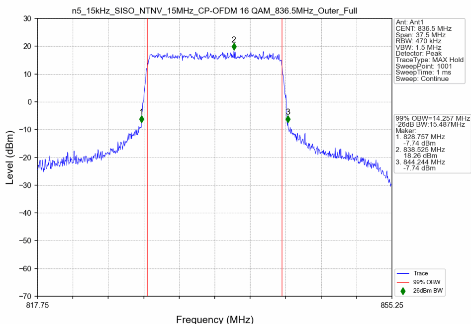
n5_15kHz_SISO_NTNV_15MHz_CP-OFDM 16 QAM_836.5MHz_Outer_Full
