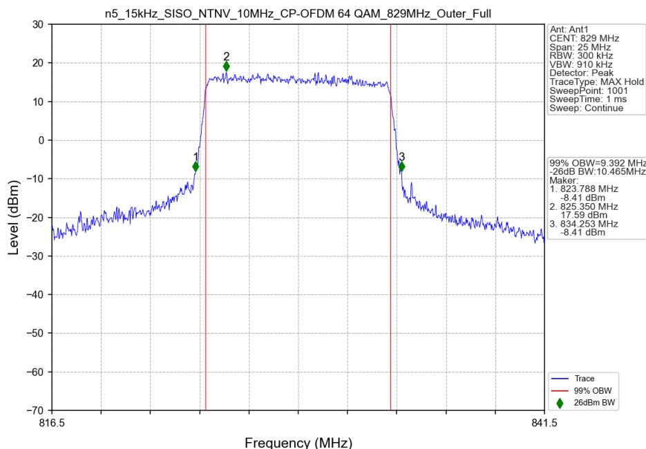
n5_15kHz_SISO_NTNV_10MHz_CP-OFDM 64 QAM_829MHz_Outer_Full
