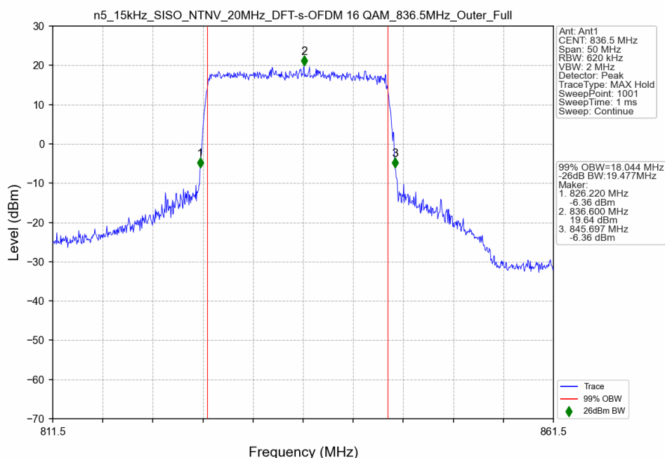
n5_15kHz_SISO_NTNV_20MHz_DFT-s-OFDM 16 QAM_836.5MHz_Outer_Full
