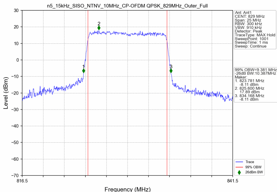
n5_15kHz_SISO_NTNV_10MHz_CP-OFDM QPSK_829MHz_Outer_Full
