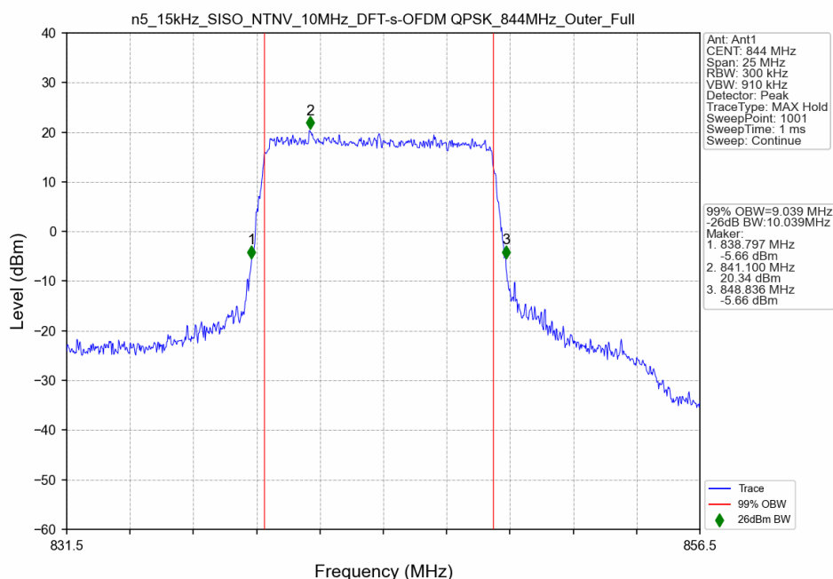
n5_15kHz_SISO_NTNV_10MHz_DFT-s-OFDM QPSK_844MHz_Outer_Full
