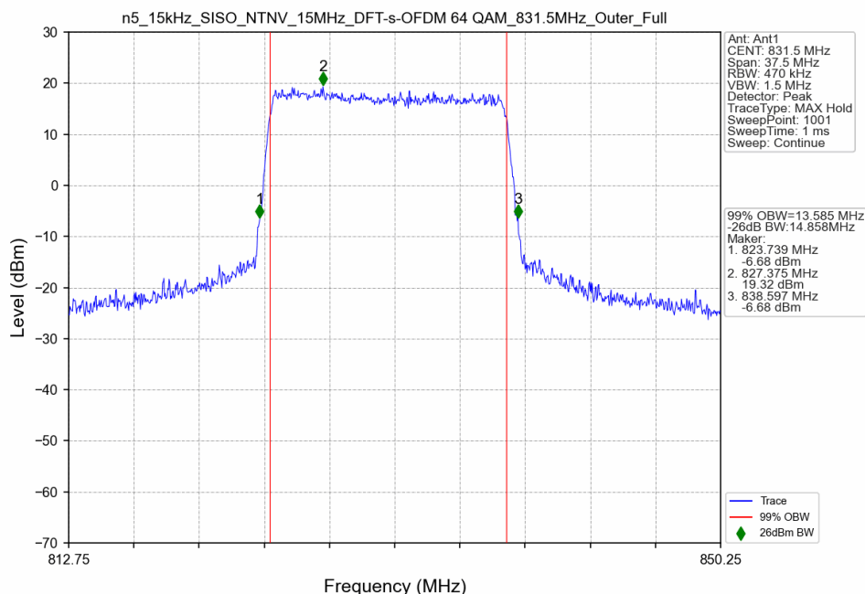
n5_15kHz_SISO_NTNV_15MHz_DFT-s-OFDM 64 QAM_831.5MHz_Outer_Full
