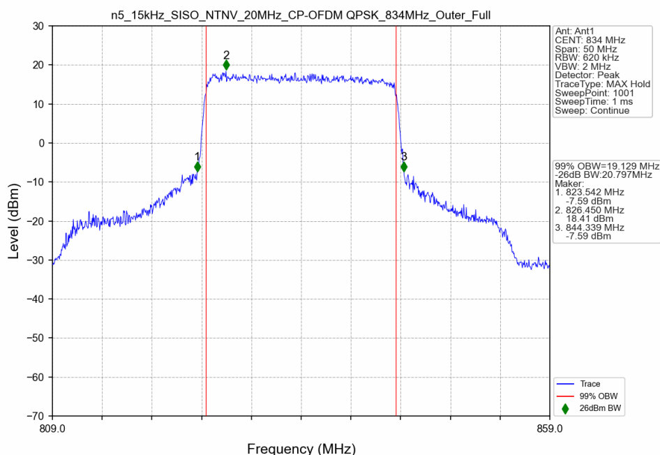
n5_15kHz_SISO_NTNV_20MHz_CP-OFDM QPSK_834MHz_Outer_Full
