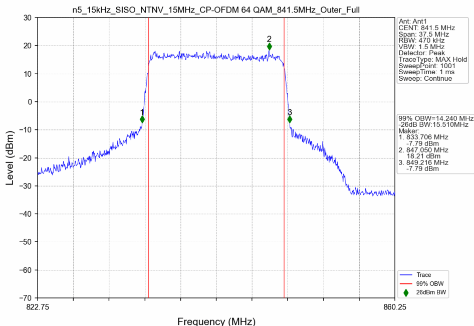
n5_15kHz_SISO_NTNV_15MHz_CP-OFDM 64 QAM_841.5MHz_Outer_Full
