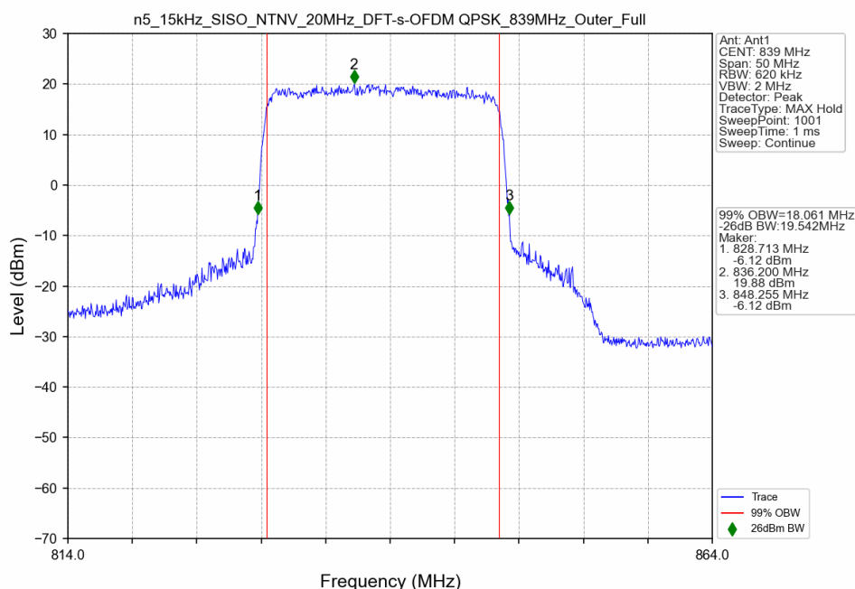
n5_15kHz_SISO_NTNV_20MHz_DFT-s-OFDM QPSK_839MHz_Outer_Full
