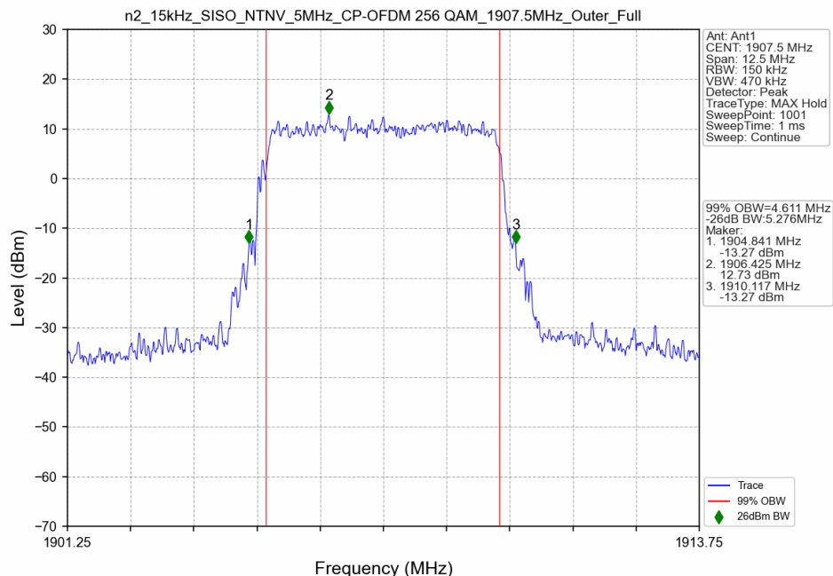
n2_15kHz_SISO_NTNV_5MHz_CP-OFDM 256 QAM_1907.5MHz_Outer_Full
