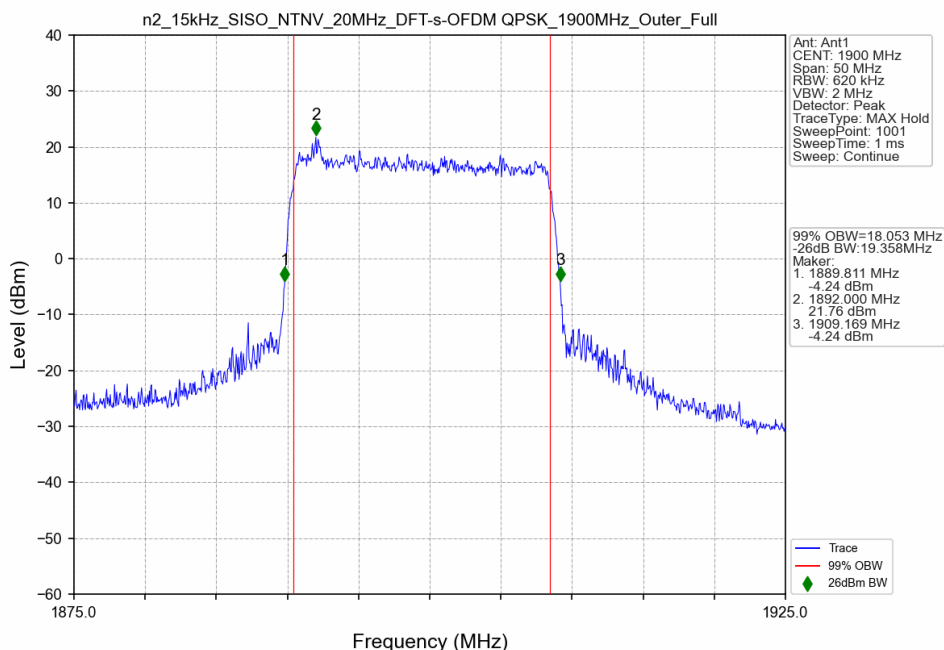
n2_15kHz_SISO_NTNV_20MHz_DFT-s-OFDM QPSK_1900MHz_Outer_Full
