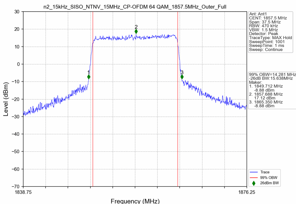
n2_15kHz_SISO_NTNV_15MHz_CP-OFDM 64 QAM_1857.5MHz_Outer_Full
