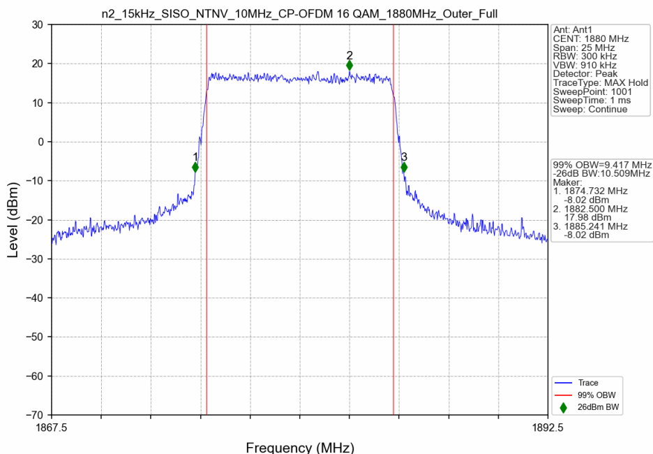
n2_15kHz_SISO_NTNV_10MHz_CP-OFDM 16 QAM_1880MHz_Outer_Full
