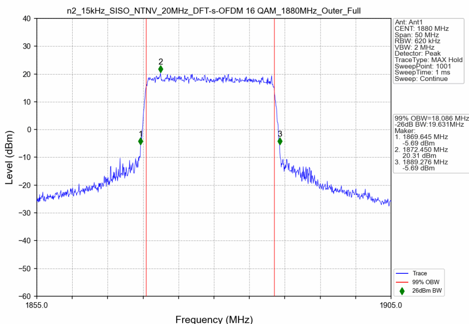
n2_15kHz_SISO_NTNV_20MHz_DFT-s-OFDM 16 QAM_1880MHz_Outer_Full
