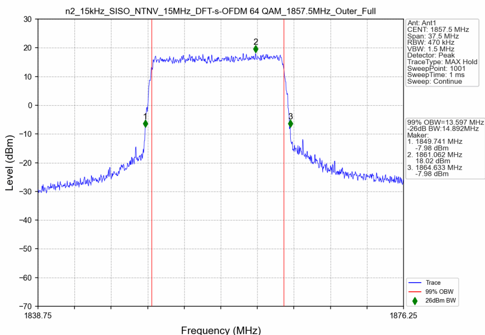
n2_15kHz_SISO_NTNV_15MHz_DFT-s-OFDM 64 QAM_1857.5MHz_Outer_Full
