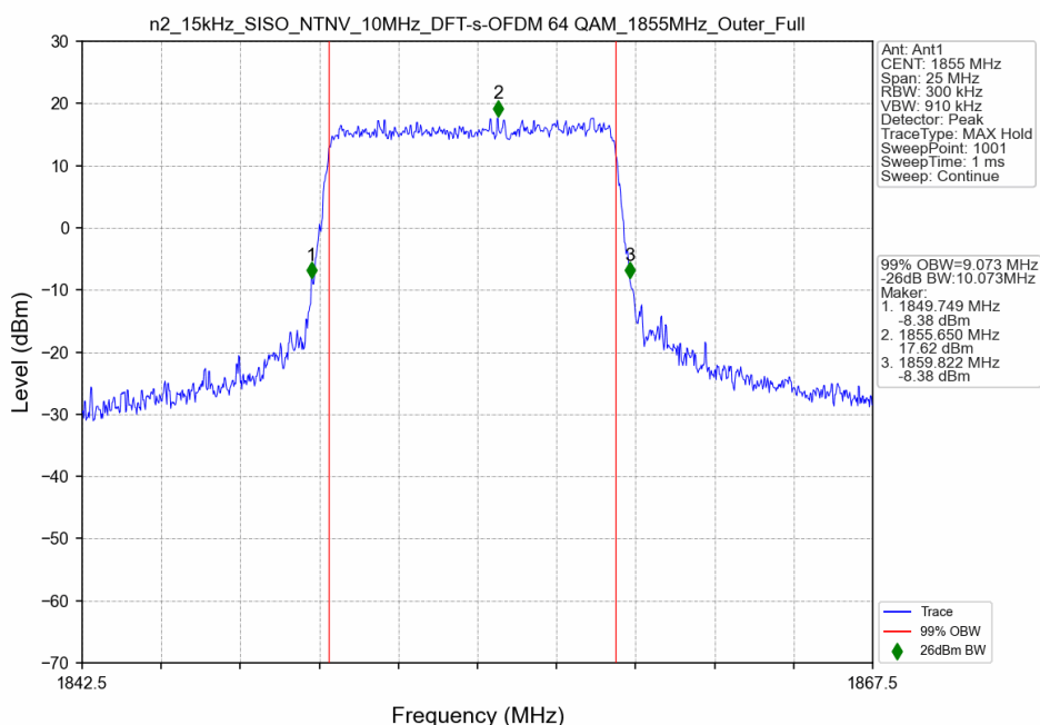
n2_15kHz_SISO_NTNV_10MHz_DFT-s-OFDM 64 QAM_1855MHz_Outer_Full
