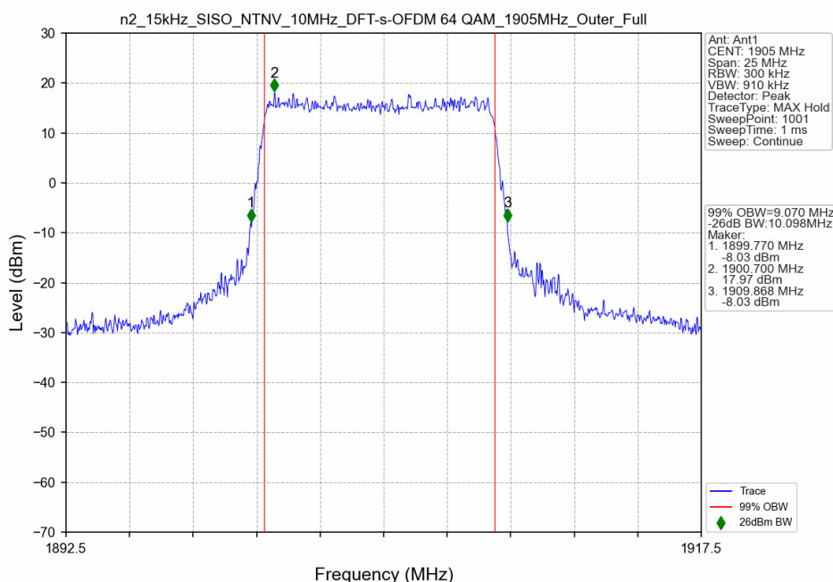
n2_15kHz_SISO_NTNV_10MHz_DFT-s-OFDM 64 QAM_1905MHz_Outer_Full
