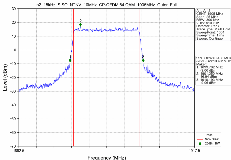
n2_15kHz_SISO_NTNV_10MHz_CP-OFDM 64 QAM_1905MHz_Outer_Full
