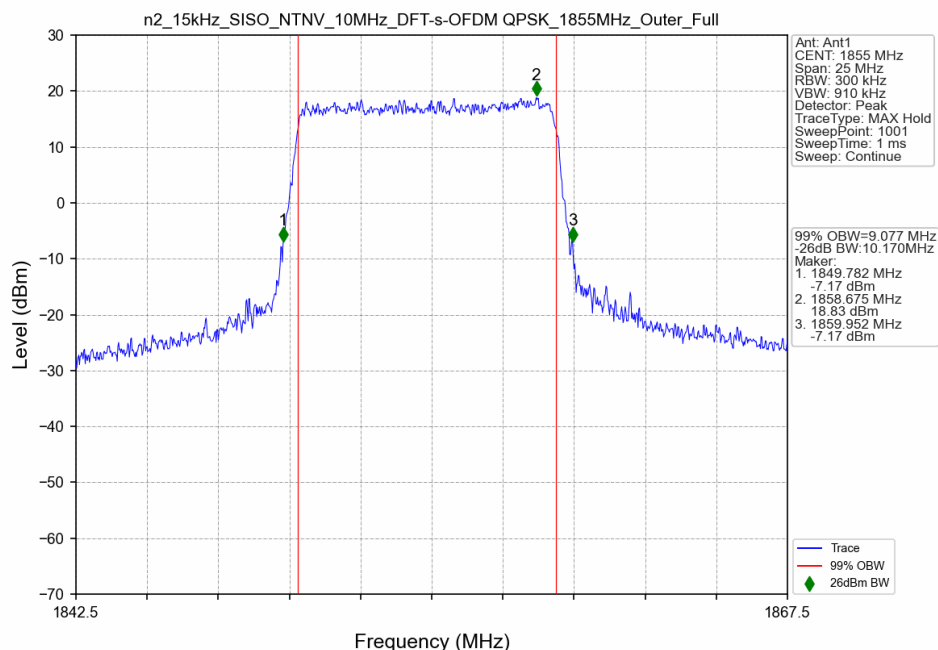
n2_15kHz_SISO_NTNV_10MHz_DFT-s-OFDM QPSK_1855MHz_Outer_Full
