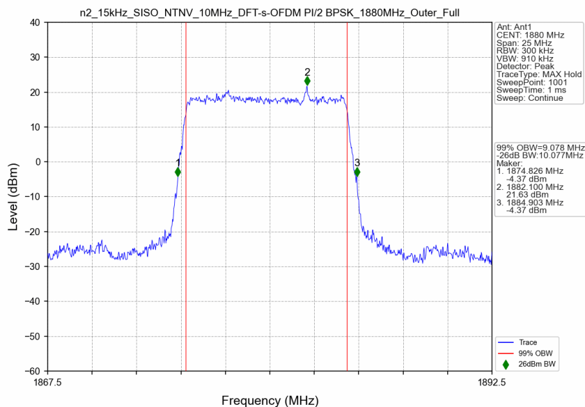
n2_15kHz_SISO_NTNV_10MHz_DFT-s-OFDM PI/2 BPSK_1880MHz_Outer_Full
