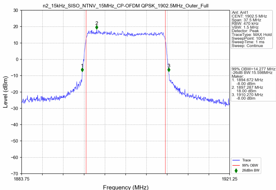
n2_15kHz_SISO_NTNV_15MHz_CP-OFDM QPSK_1902.5MHz_Outer_Full
