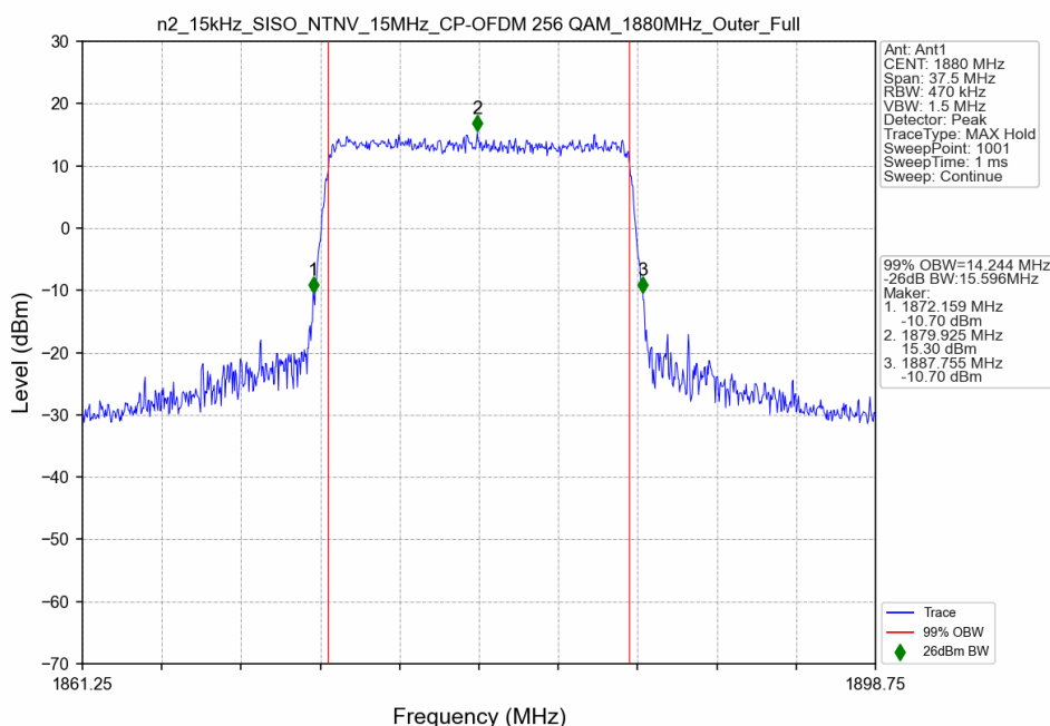
n2_15kHz_SISO_NTNV_15MHz_CP-OFDM 256 QAM_1880MHz_Outer_Full
