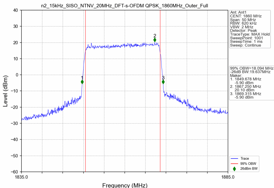
n2_15kHz_SISO_NTNV_20MHz_DFT-s-OFDM QPSK_1860MHz_Outer_Full
