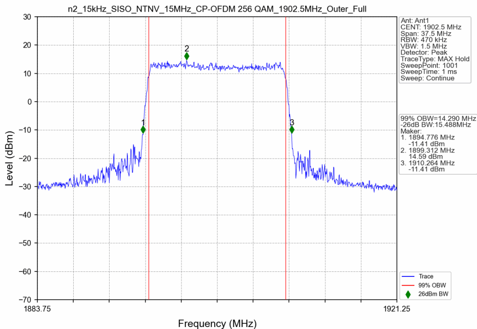
n2_15kHz_SISO_NTNV_15MHz_CP-OFDM 256 QAM_1902.5MHz_Outer_Full
