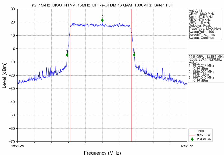
n2_15kHz_SISO_NTNV_15MHz_DFT-s-OFDM 16 QAM_1880MHz_Outer_Full
