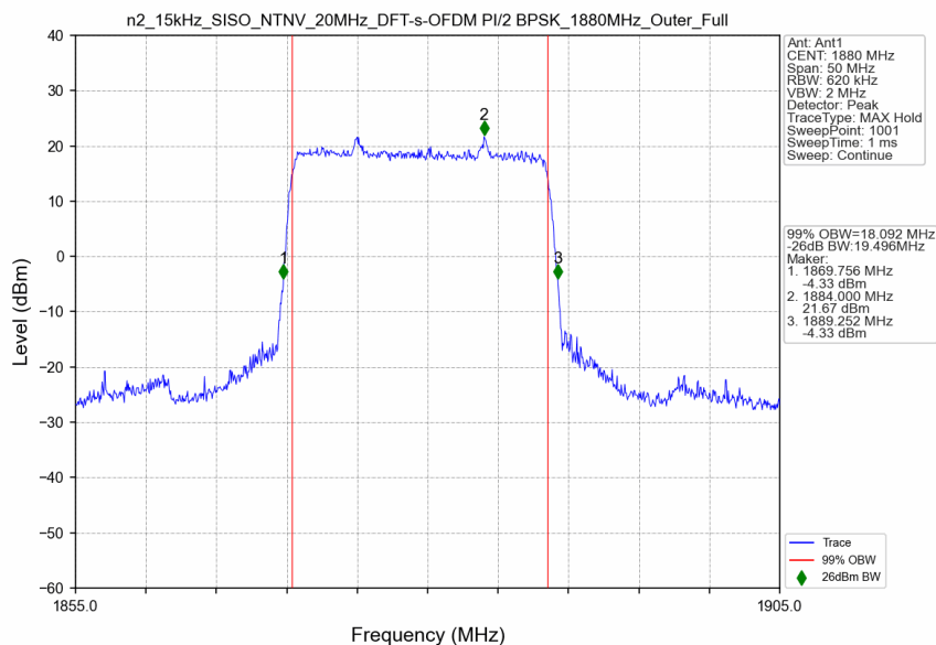
n2_15kHz_SISO_NTNV_20MHz_DFT-s-OFDM PI/2 BPSK_1880MHz_Outer_Full
