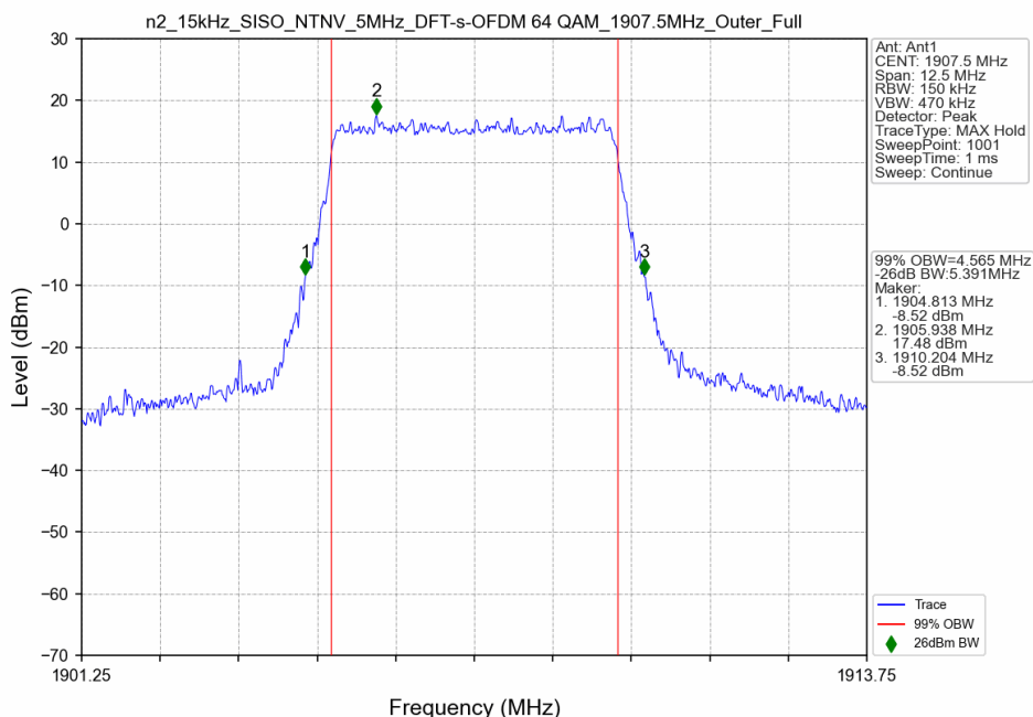
n2_15kHz_SISO_NTNV_5MHz_DFT-s-OFDM 64 QAM_1907.5MHz_Outer_Full
