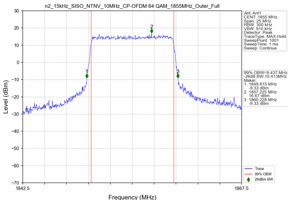
n2_15kHz_SISO_NTNV_10MHz_CP-OFDM 64 QAM_1855MHz_Outer_Full
