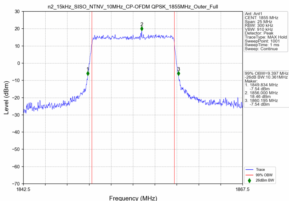
n2_15kHz_SISO_NTNV_10MHz_CP-OFDM QPSK_1855MHz_Outer_Full
