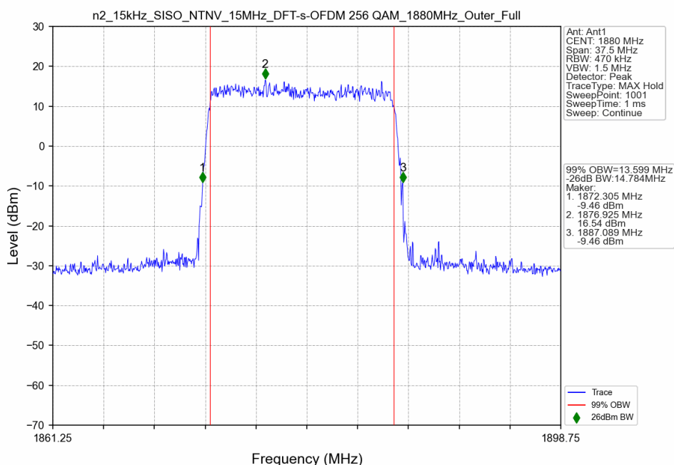
n2_15kHz_SISO_NTNV_15MHz_DFT-s-OFDM 256 QAM_1880MHz_Outer_Full
