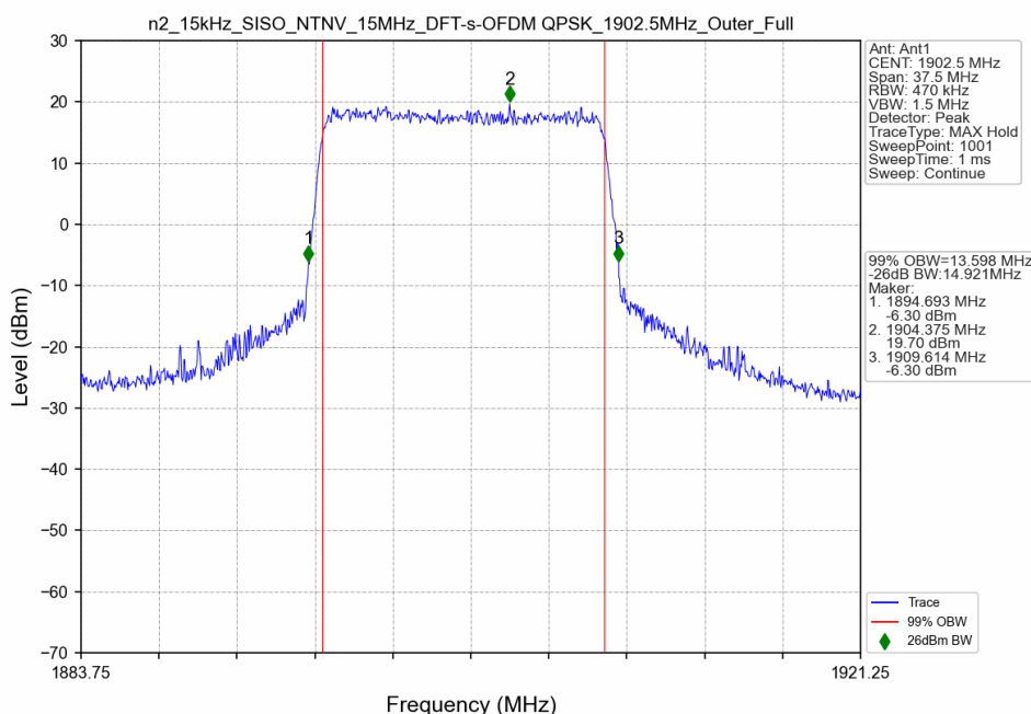
n2_15kHz_SISO_NTNV_15MHz_DFT-s-OFDM QPSK_1902.5MHz_Outer_Full
