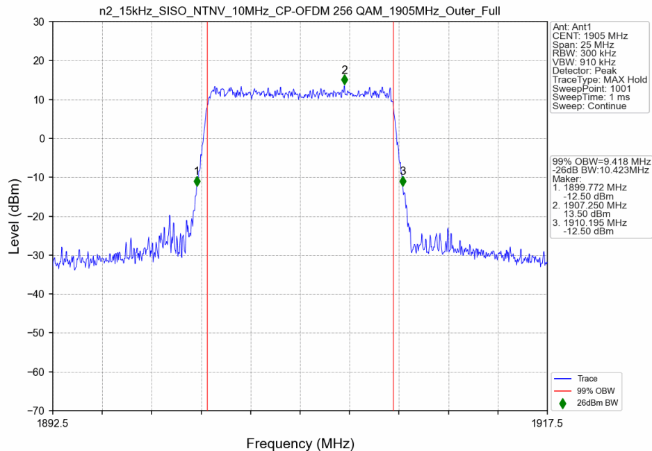
n2_15kHz_SISO_NTNV_10MHz_CP-OFDM 256 QAM_1905MHz_Outer_Full
