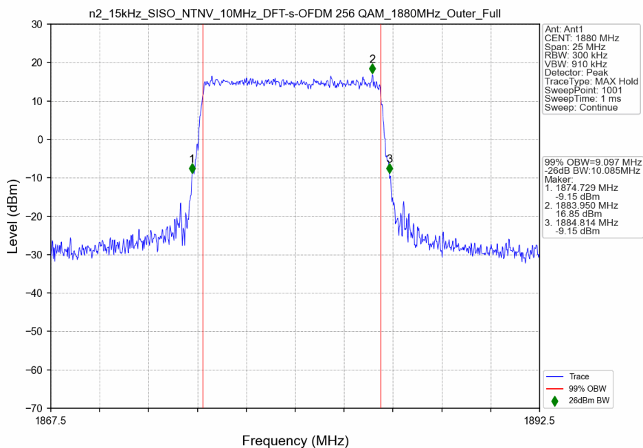
n2_15kHz_SISO_NTNV_10MHz_DFT-s-OFDM 256 QAM_1880MHz_Outer_Full
