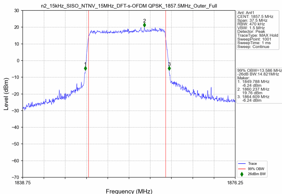
n2_15kHz_SISO_NTNV_15MHz_DFT-s-OFDM QPSK_1857.5MHz_Outer_Full
