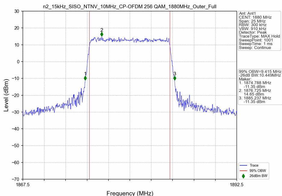
n2_15kHz_SISO_NTNV_10MHz_CP-OFDM 256 QAM_1880MHz_Outer_Full
