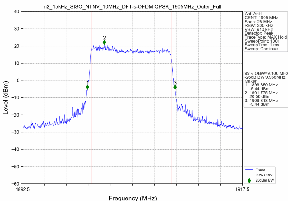
n2_15kHz_SISO_NTNV_10MHz_DFT-s-OFDM QPSK_1905MHz_Outer_Full
