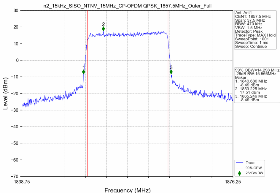
n2_15kHz_SISO_NTNV_15MHz_CP-OFDM QPSK_1857.5MHz_Outer_Full
