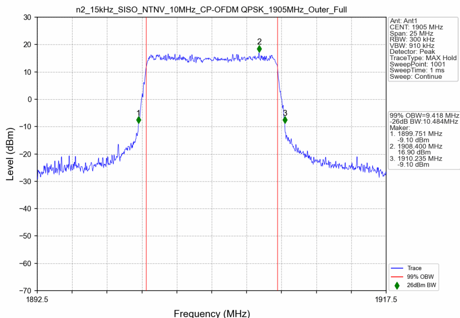
n2_15kHz_SISO_NTNV_10MHz_CP-OFDM QPSK_1905MHz_Outer_Full
