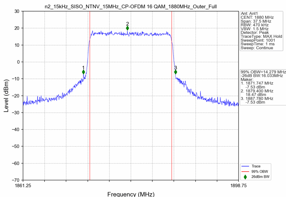
n2_15kHz_SISO_NTNV_15MHz_CP-OFDM 16 QAM_1880MHz_Outer_Full
