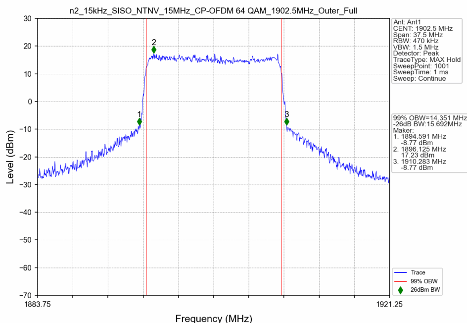
n2_15kHz_SISO_NTNV_15MHz_CP-OFDM 64 QAM_1902.5MHz_Outer_Full
