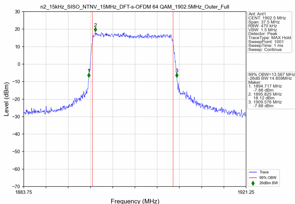
n2_15kHz_SISO_NTNV_15MHz_DFT-s-OFDM 64 QAM_1902.5MHz_Outer_Full
