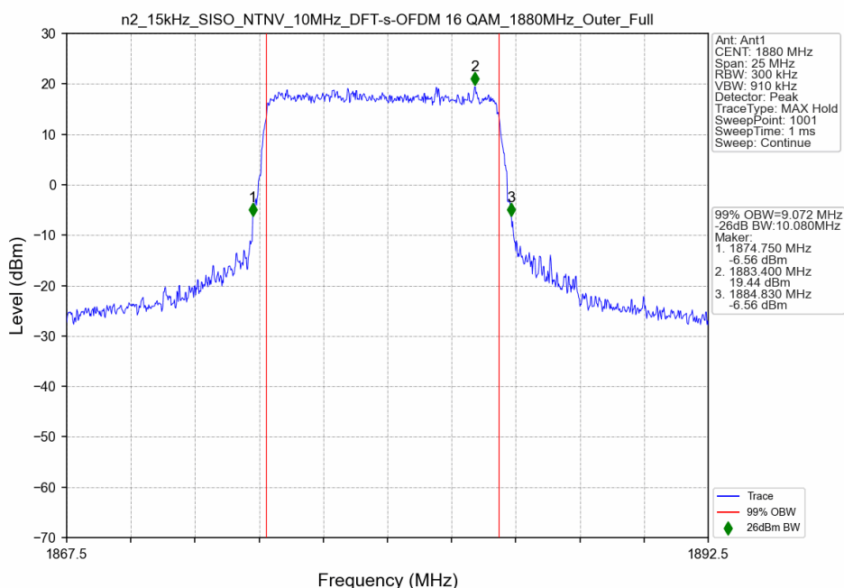
n2_15kHz_SISO_NTNV_10MHz_DFT-s-OFDM 16 QAM_1880MHz_Outer_Full
