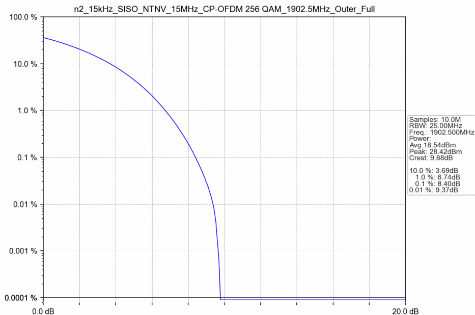
n2_15kHz_SISO_NTNV_15MHz_CP-OFDM 256 QAM_1902.5MHz_Outer_Full
