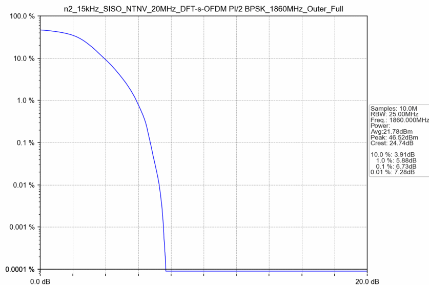
n2_15kHz_SISO_NTNV_20MHz_DFT-s-OFDM PI/2 BPSK_1860MHz_Outer_Full
