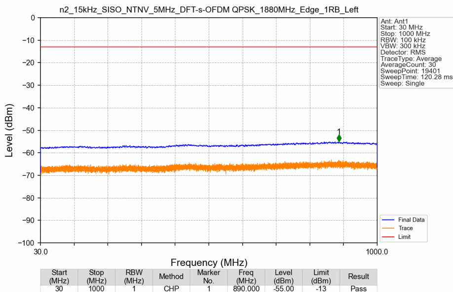
n2_15kHz_SISO_NTNV_5MHz_DFT-s-OFDM QPSK_1880MHz_Edge_1RB_Left
