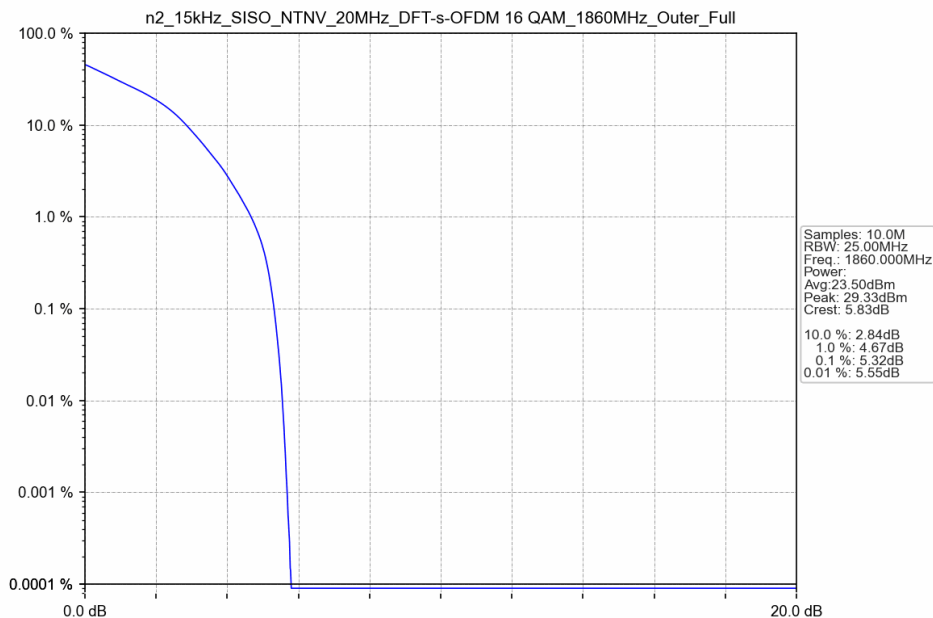
n2_15kHz_SISO_NTNV_20MHz_DFT-s-OFDM 16 QAM_1860MHz_Outer_Full
