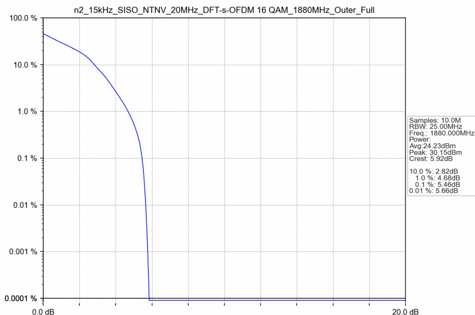
n2_15kHz_SISO_NTNV_20MHz_DFT-s-OFDM 16 QAM_1880MHz_Outer_Full
