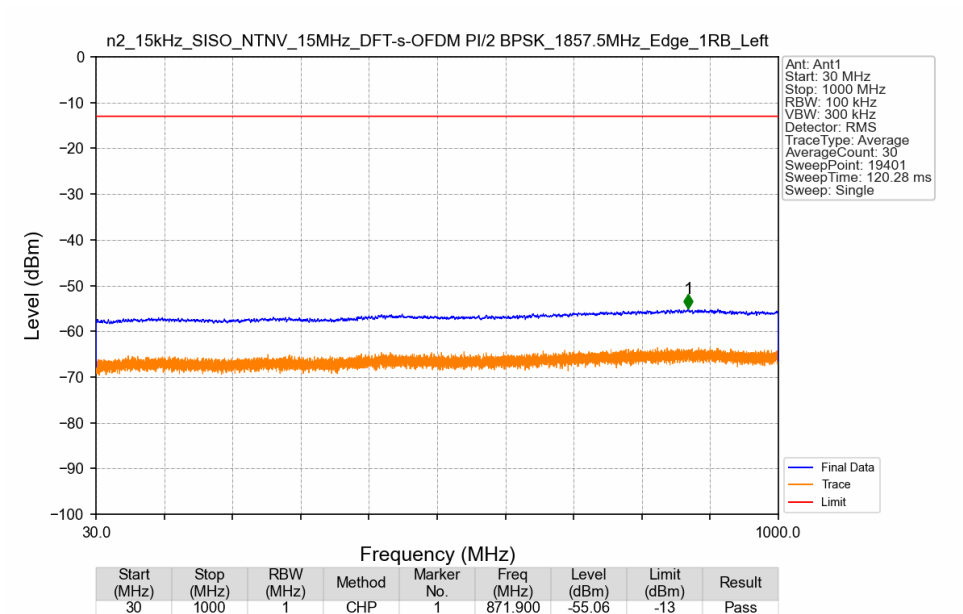
n2_15kHz_SISO_NTNV_15MHz_DFT-s-OFDM PI/2 BPSK_1857.5MHz_Edge_1RB_Left
