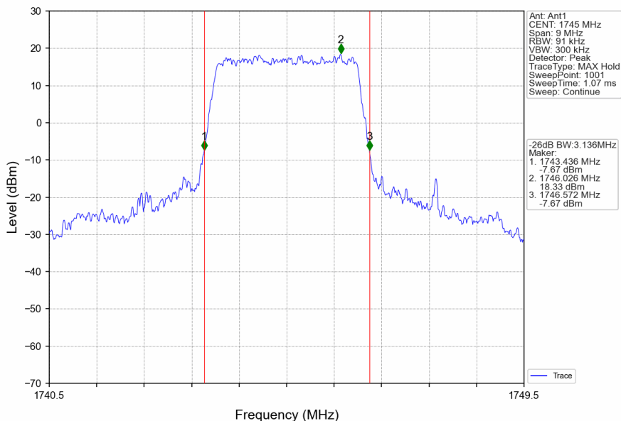
Band66_3MHz_QPSK_MCH_1745MHz_RB_15_0_NTNV
