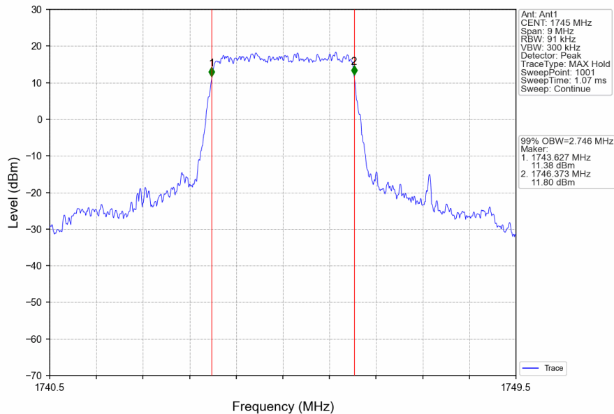
Band66_3MHz_QPSK_MCH_1745MHz_RB_15_0_NTNV
