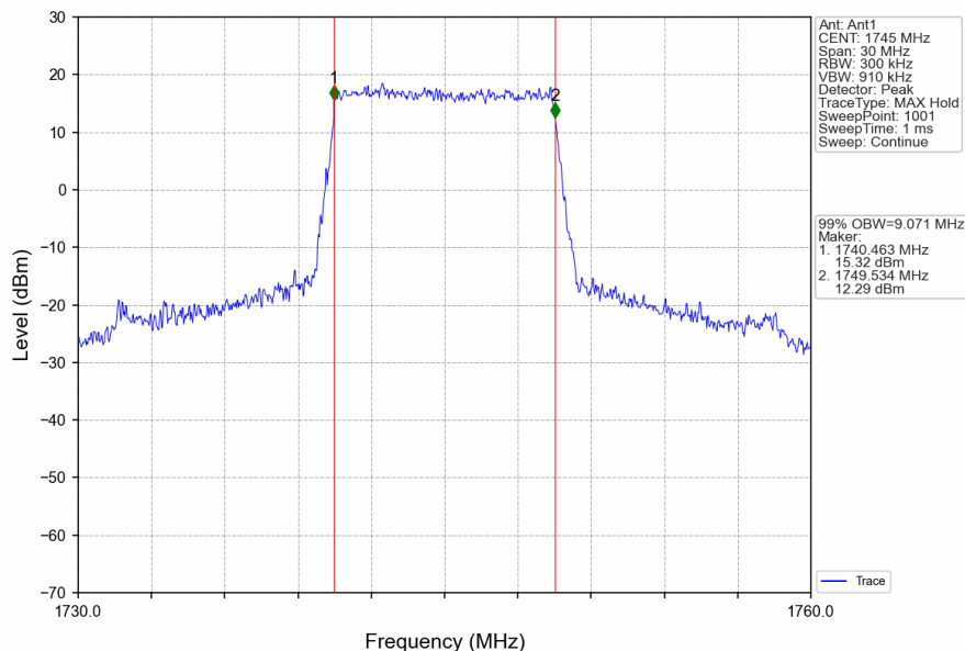
Band66_10MHz_QPSK_MCH_1745MHz_RB_50_0_NTNV
