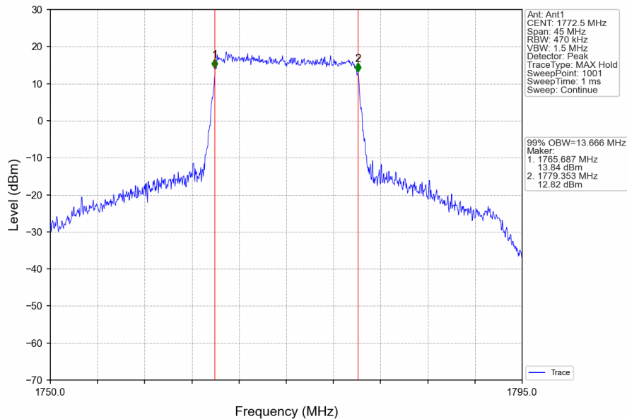
Band66_15MHz_16QAM_HCH_1772.5MHz_RB_75_0_NTNV
