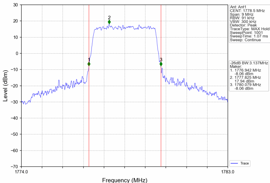
Band66_3MHz_16QAM_HCH_1778.5MHz_RB_15_0_NTNV
