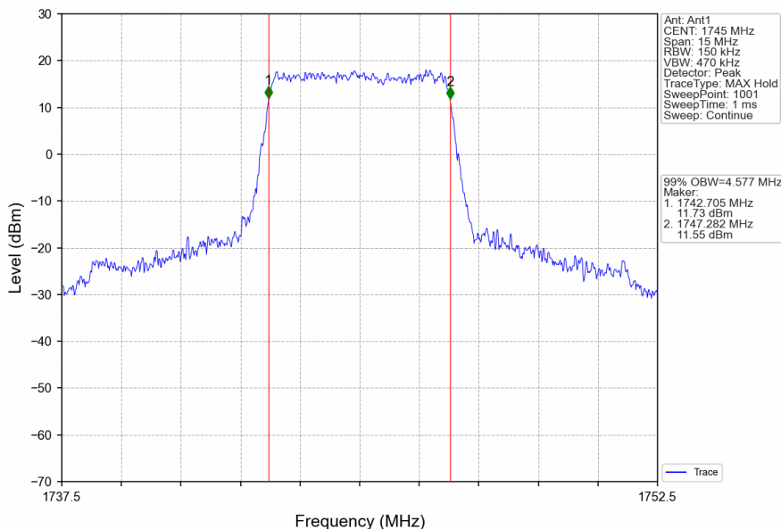
Band66_5MHz_QPSK_MCH_1745MHz_RB_25_0_NTNV
