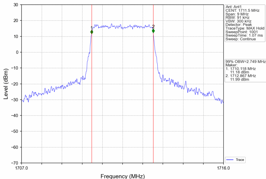
Band66_3MHz_16QAM_LCH_1711.5MHz_RB_15_0_NTNV
