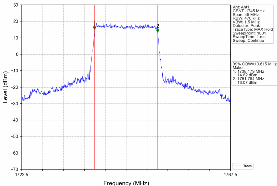
Band66_15MHz_QPSK_MCH_1745MHz_RB_75_0_NTNV
