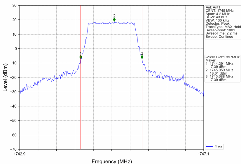
Band66_1.4MHz_QPSK_MCH_1745MHz_RB_6_0_NTNV
