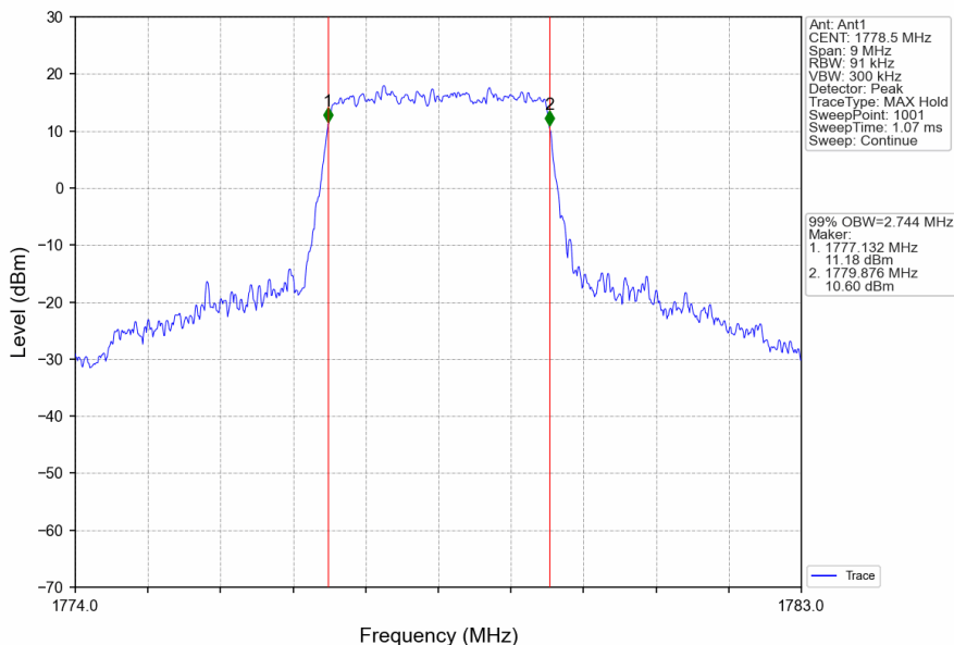
Band66_3MHz_16QAM_HCH_1778.5MHz_RB_15_0_NTNV
