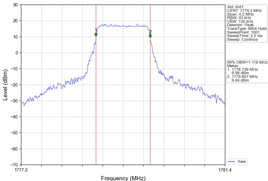
Band66_1.4MHz_16QAM_HCH_1779.3MHz_RB_6_0_NTNV
