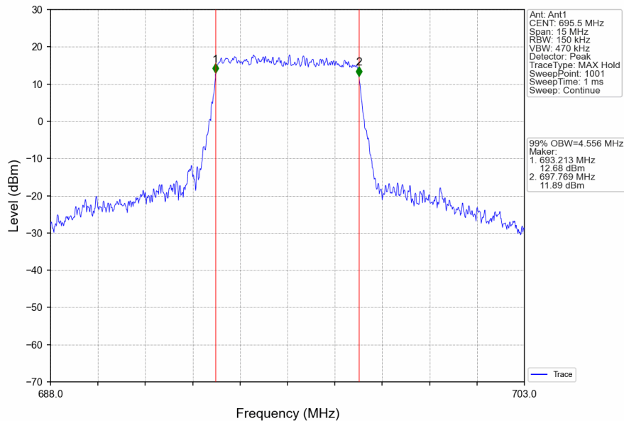
Band71_5MHz_16QAM_HCH_695.5MHz_RB_25_0_NTNV
