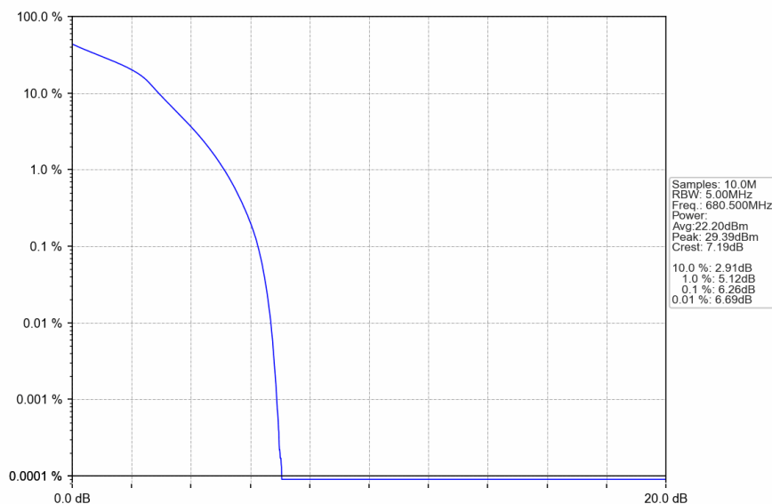
Band71_5MHz_16QAM_MCH_680.5MHz_RB_25_0_NTNV
