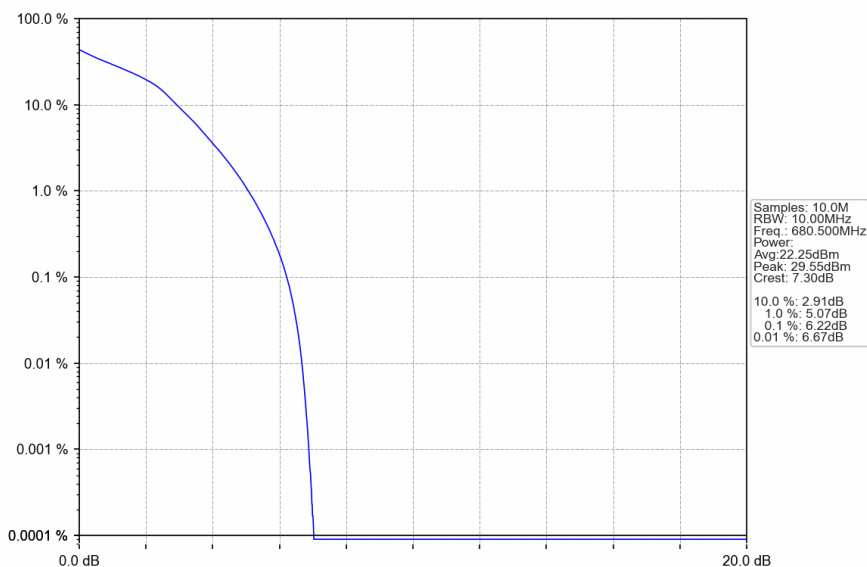
Band71_10MHz_16QAM_MCH_680.5MHz_RB_50_0_NTNV
