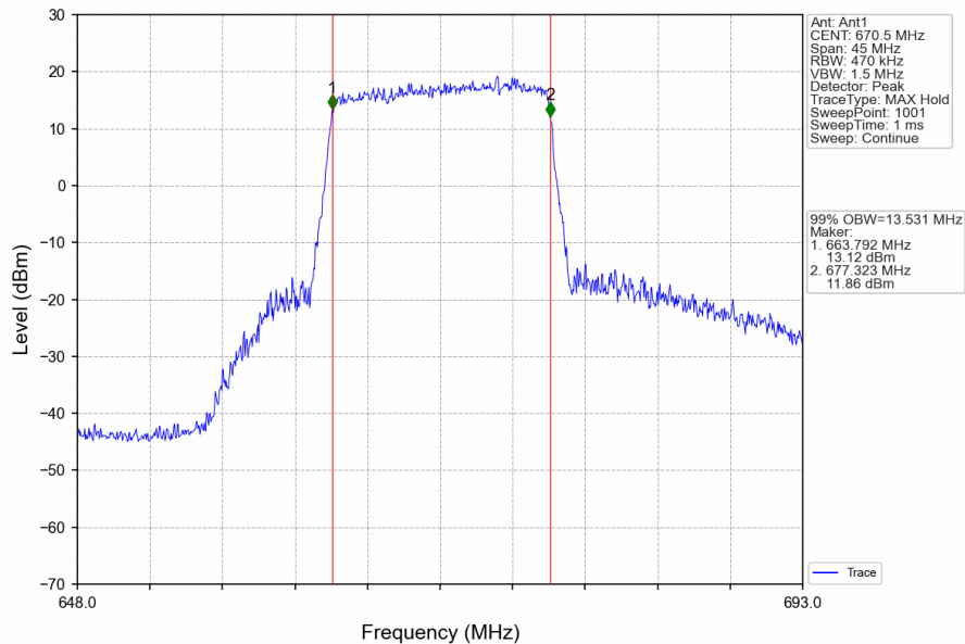
Band71_15MHz_16QAM_LCH_670.5MHz_RB_75_0_NTNV
