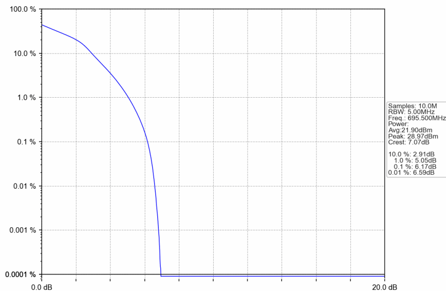
Band71_5MHz_16QAM_HCH_695.5MHz_RB_25_0_NTNV
