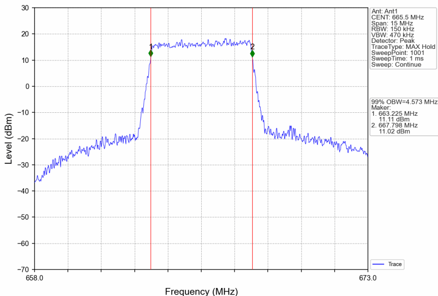
Band71_5MHz_16QAM_LCH_665.5MHz_RB_25_0_NTNV
