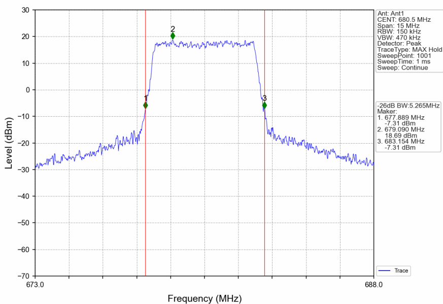
Band71_5MHz_QPSK_MCH_680.5MHz_RB_25_0_NTNV
