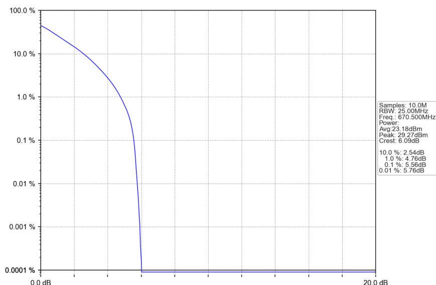
Band71_15MHz_QPSK_LCH_670.5MHz_RB_75_0_NTNV
