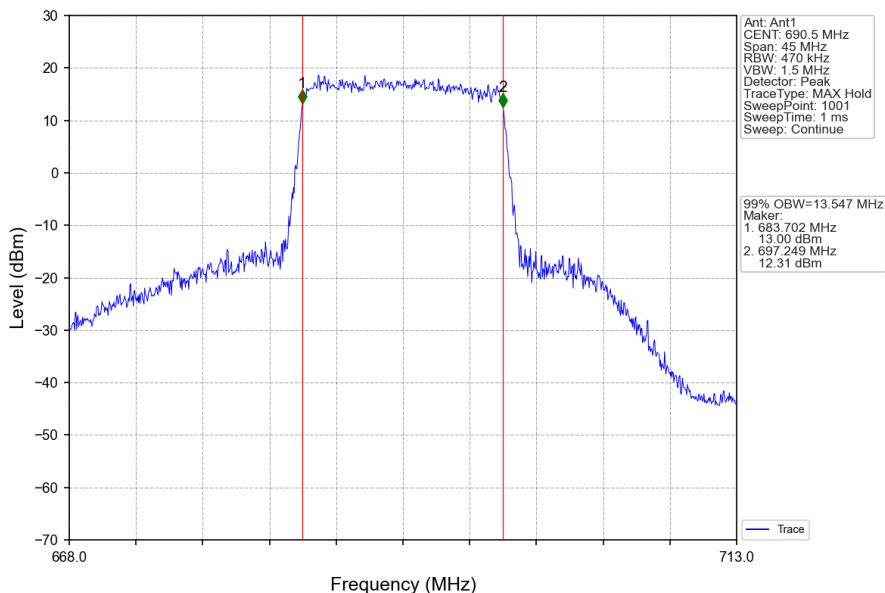
Band71_15MHz_16QAM_HCH_690.5MHz_RB_75_0_NTNV
