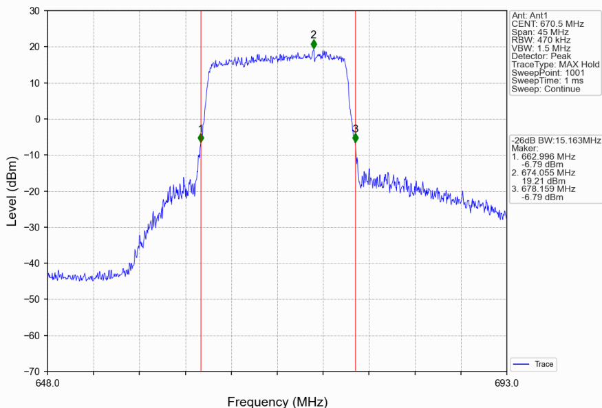
Band71_15MHz_16QAM_LCH_670.5MHz_RB_75_0_NTNV
