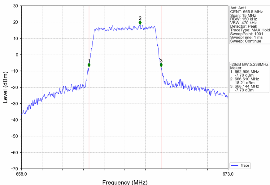
Band71_5MHz_16QAM_LCH_665.5MHz_RB_25_0_NTNV
