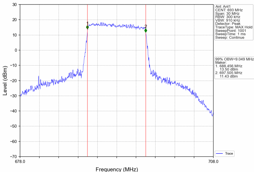
Band71_10MHz_16QAM_HCH_693MHz_RB_50_0_NTNV
