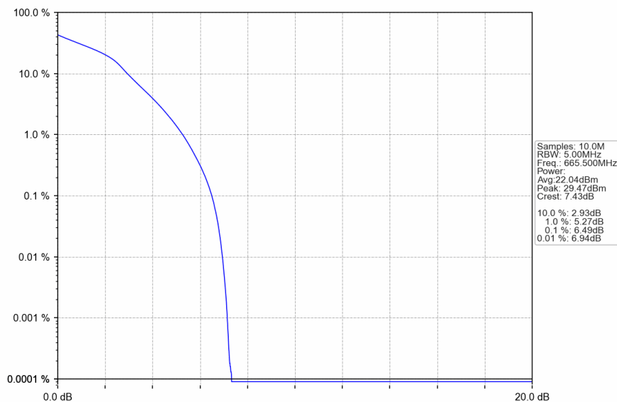
Band71_5MHz_16QAM_LCH_665.5MHz_RB_25_0_NTNV
