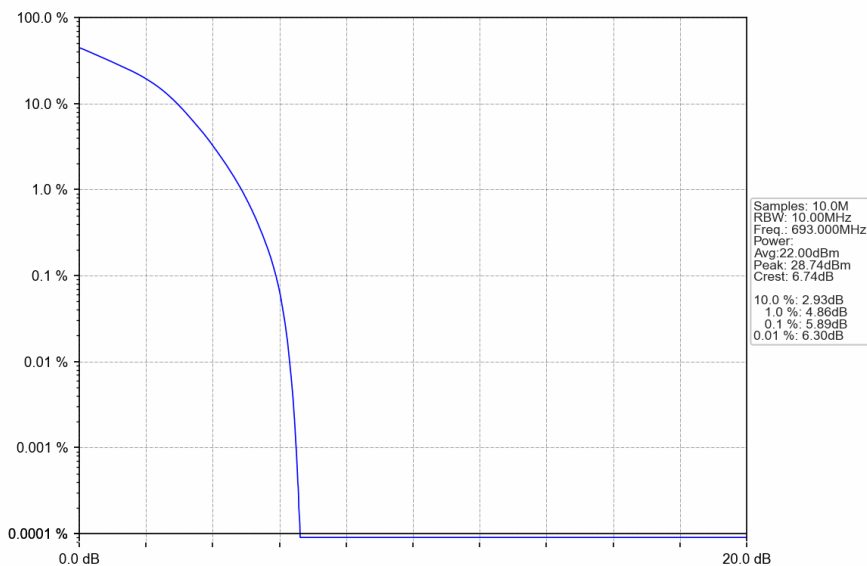
Band71_10MHz_16QAM_HCH_693MHz_RB_50_0_NTNV
