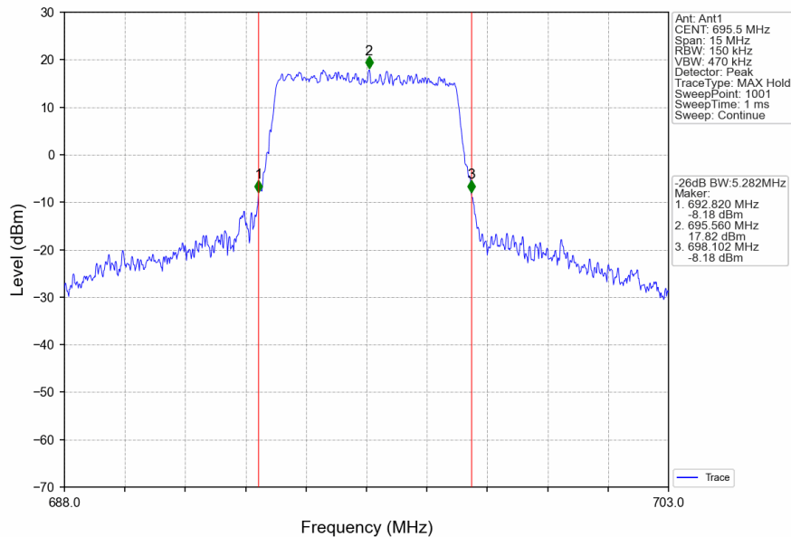
Band71_5MHz_16QAM_HCH_695.5MHz_RB_25_0_NTNV
