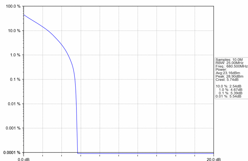
Band71_15MHz_QPSK_MCH_680.5MHz_RB_75_0_NTNV
