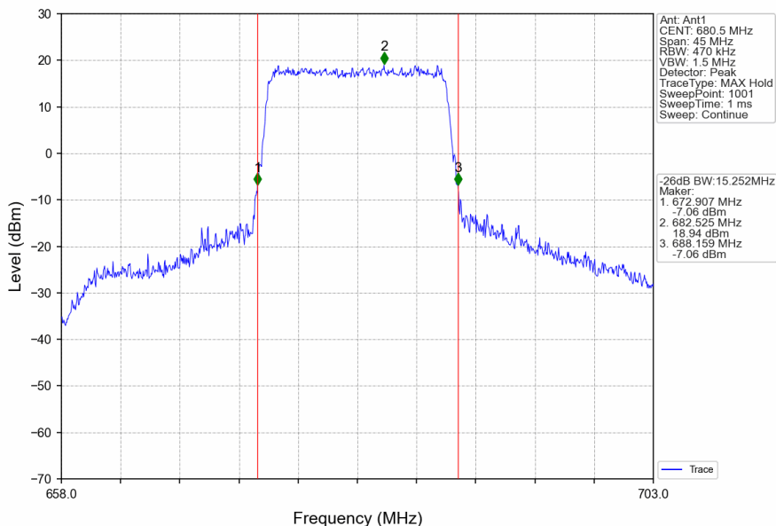
Band71_15MHz_QPSK_MCH_680.5MHz_RB_75_0_NTNV
