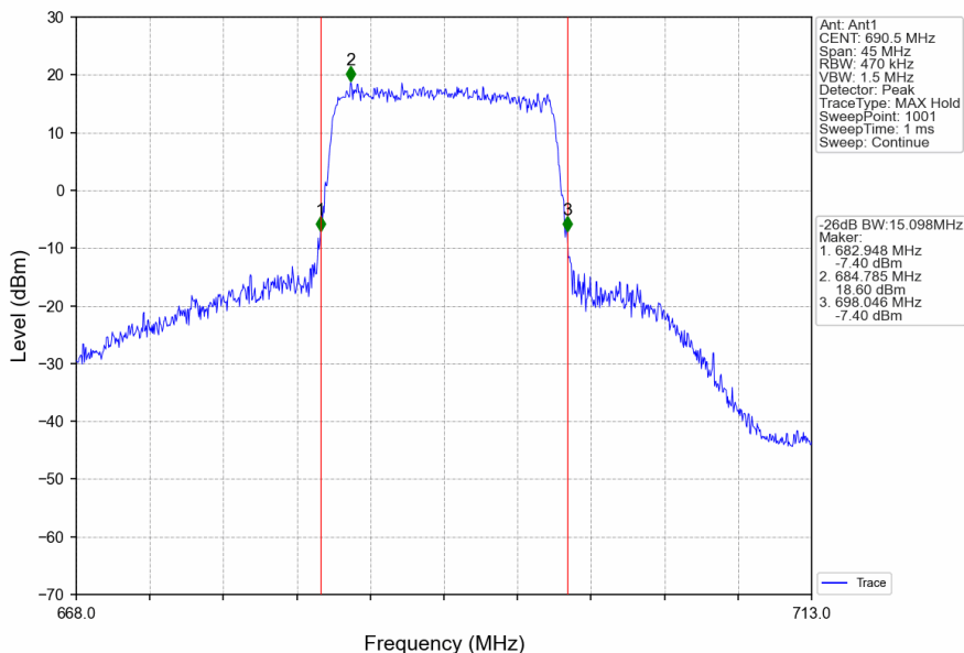
Band71_15MHz_16QAM_HCH_690.5MHz_RB_75_0_NTNV
