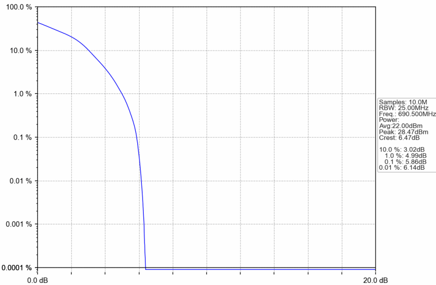
Band71_15MHz_16QAM_HCH_690.5MHz_RB_75_0_NTNV
