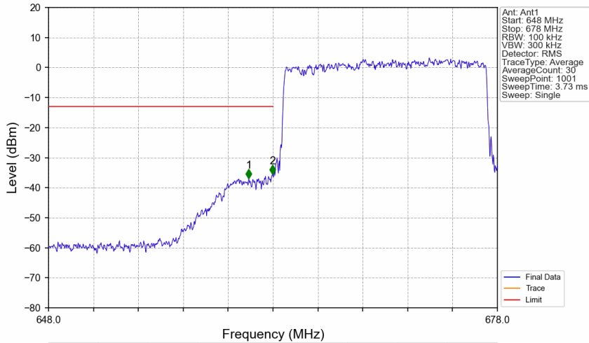
Band71_15MHz_16QAM_LCH_670.5MHz_RB_75_0_NTNV
