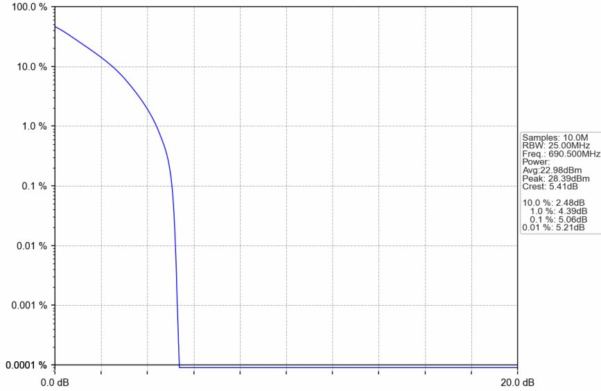
Band71_15MHz_QPSK_HCH_690.5MHz_RB_75_0_NTNV
