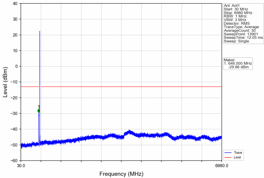
Band71_15MHz_16QAM_HCH_690.5MHz_RB_1_0_NTNV
