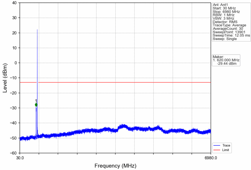
Band71_15MHz_16QAM_LCH_670.5MHz_RB_75_0_NTNV
