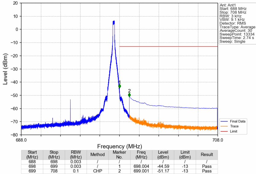
Band71_10MHz_16QAM_HCH_693MHz_RB_1_49_NTNV
