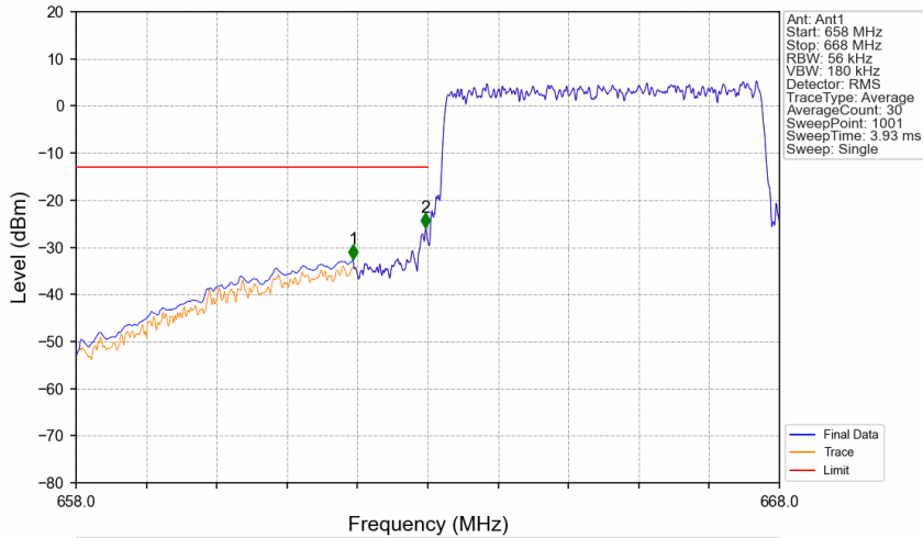
Band71_5MHz_16QAM_LCH_665.5MHz_RB_25_0_NTNV
