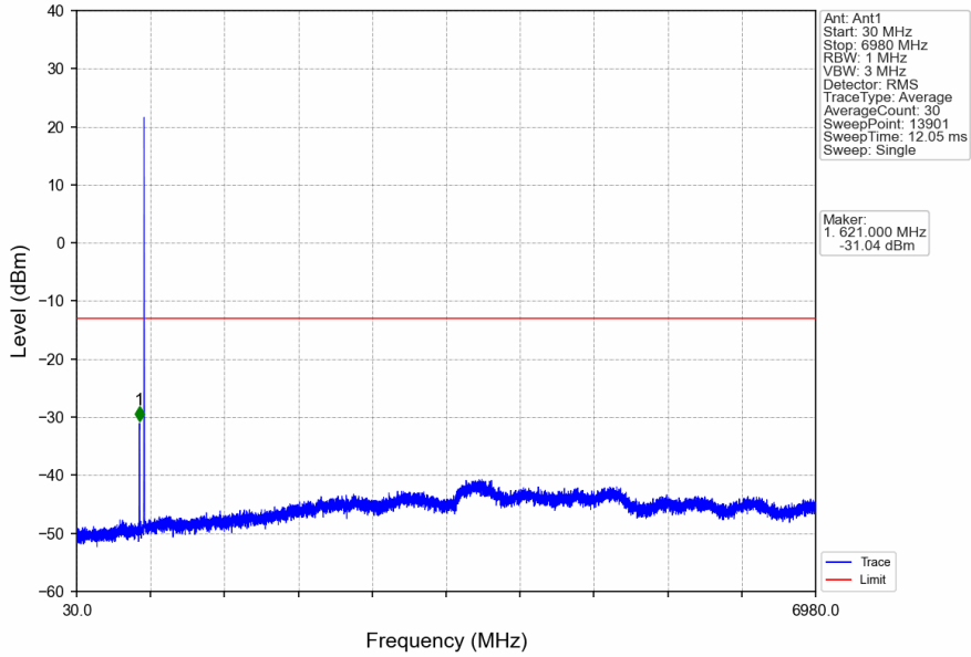
Band71_5MHz_16QAM_LCH_665.5MHz_RB_25_0_NTNV
