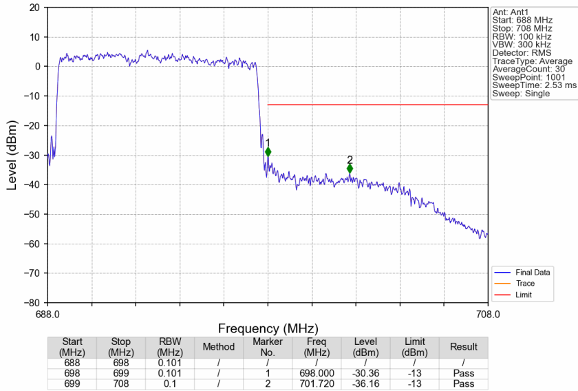
Band71_10MHz_16QAM_HCH_693MHz_RB_50_0_NTNV
