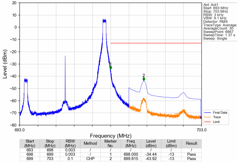
Band71_5MHz_16QAM_HCH_695.5MHz_RB_1_24_NTNV
