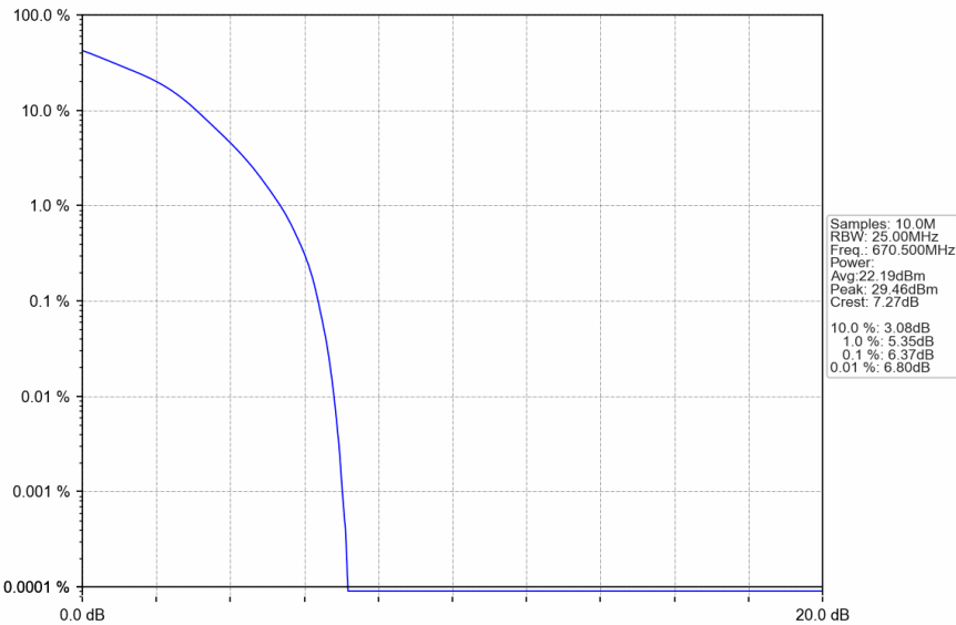
Band71_15MHz_16QAM_LCH_670.5MHz_RB_75_0_NTNV
