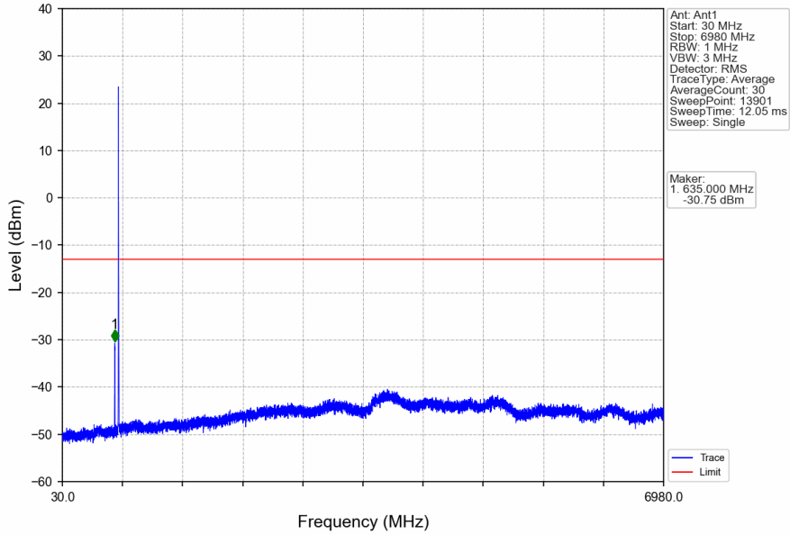
Band71_5MHz_16QAM_HCH_695.5MHz_RB_1_0_NTNV
