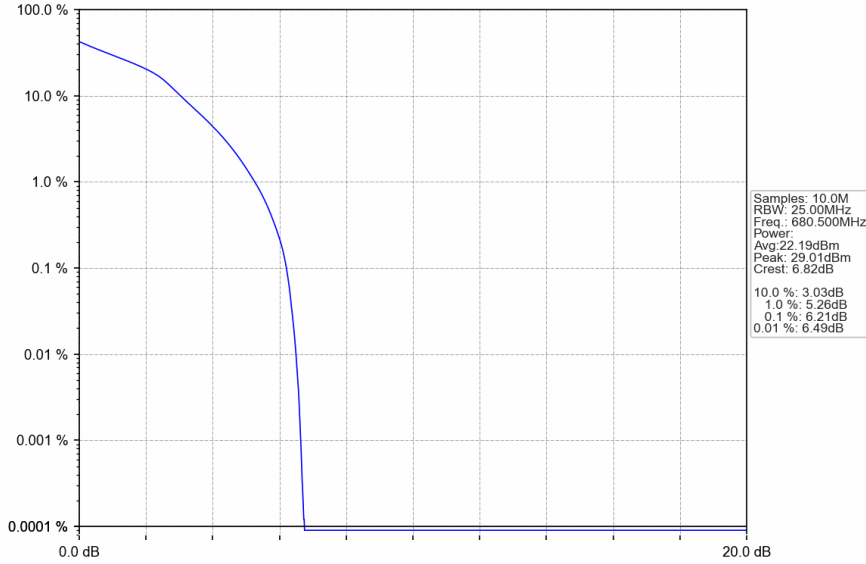
Band71_15MHz_16QAM_MCH_680.5MHz_RB_75_0_NTNV
