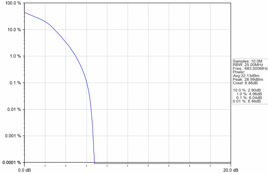
Band71_20MHz_16QAM_MCH_683MHz_RB_100_0_NTNV
