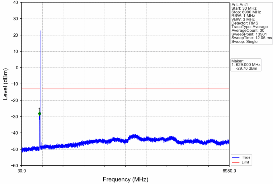
Band71_15MHz_16QAM_HCH_690.5MHz_RB_1_0_NTNV
