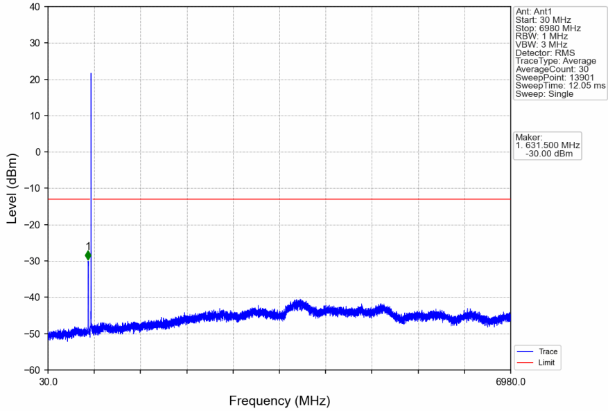
Band71_10MHz_16QAM_HCH_693MHz_RB_1_0_NTNV
