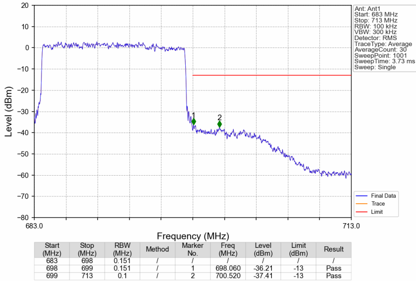
Band71_15MHz_16QAM_HCH_690.5MHz_RB_75_0_NTNV
