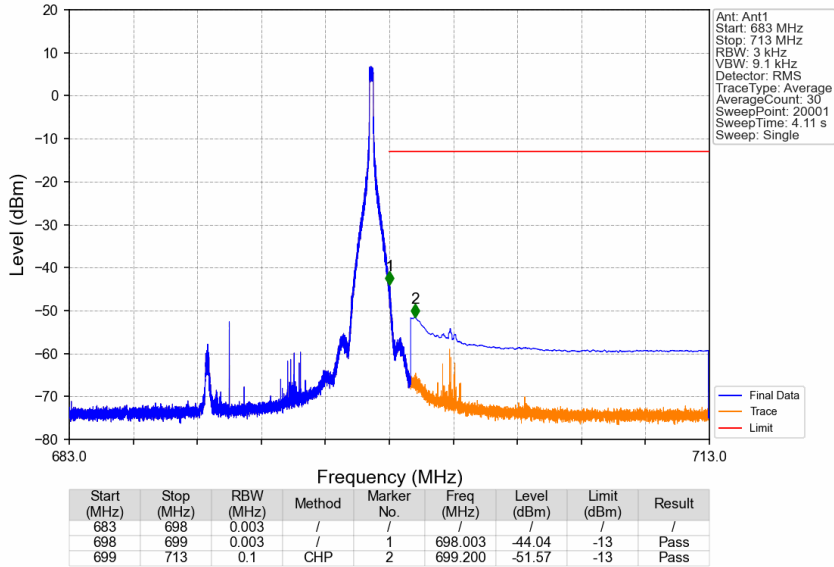
Band71_15MHz_16QAM_HCH_690.5MHz_RB_1_74_NTNV
