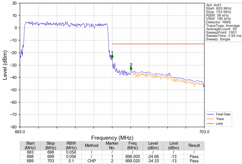
Band71_5MHz_16QAM_HCH_695.5MHz_RB_25_0_NTNV
