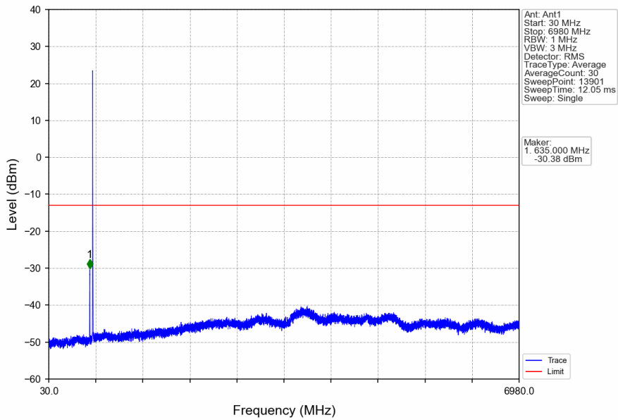
Band71_5MHz_QPSK_MCH_680.5MHz_RB_1_0_NTNV
