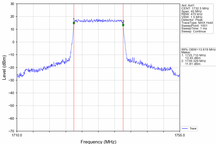
Band4_15MHz_QPSK_MCH_1732.5MHz_RB_75_0_NTNV
