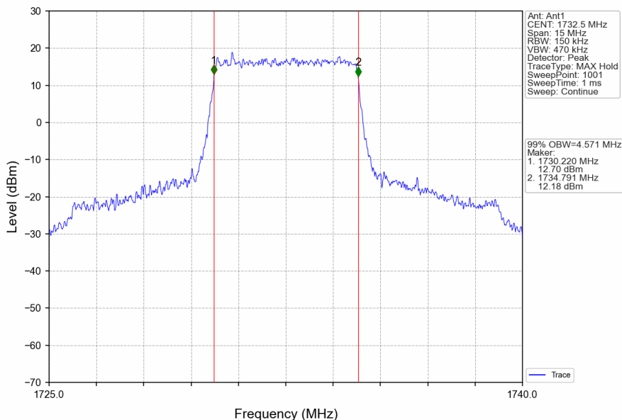
Band4_5MHz_QPSK_MCH_1732.5MHz_RB_25_0_NTNV
