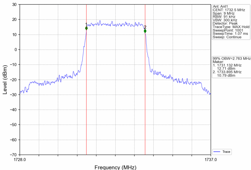
Band4_3MHz_QPSK_MCH_1732.5MHz_RB_15_0_NTNV
