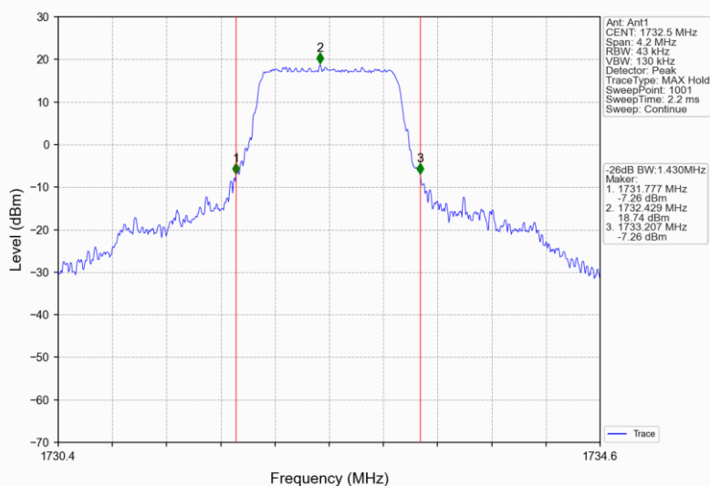
Band4_1.4MHz_QPSK_MCH_1732.5MHz_RB_6_0_NTNV
