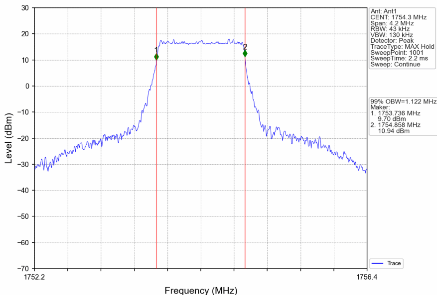
Band4_1.4MHz_16QAM_HCH_1754.3MHz_RB_6_0_NTNV
