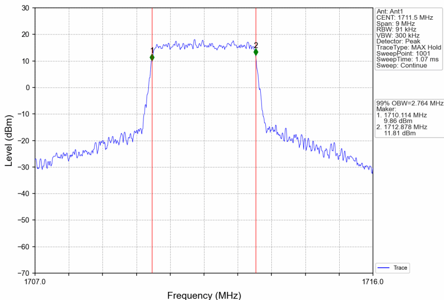
Band4_3MHz_16QAM_LCH_1711.5MHz_RB_15_0_NTNV
