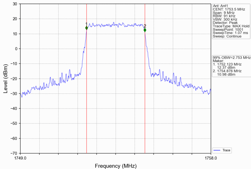
Band4_3MHz_16QAM_HCH_1753.5MHz_RB_15_0_NTNV
