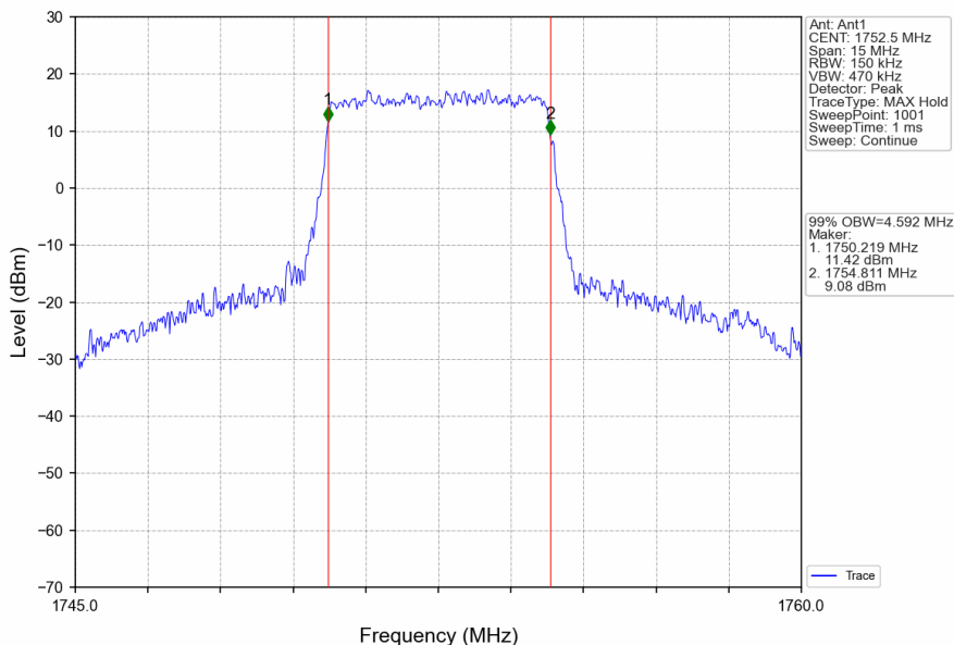
Band4_5MHz_16QAM_HCH_1752.5MHz_RB_25_0_NTNV
