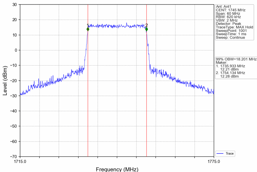
Band4_20MHz_16QAM_HCH_1745MHz_RB_100_0_NTNV
