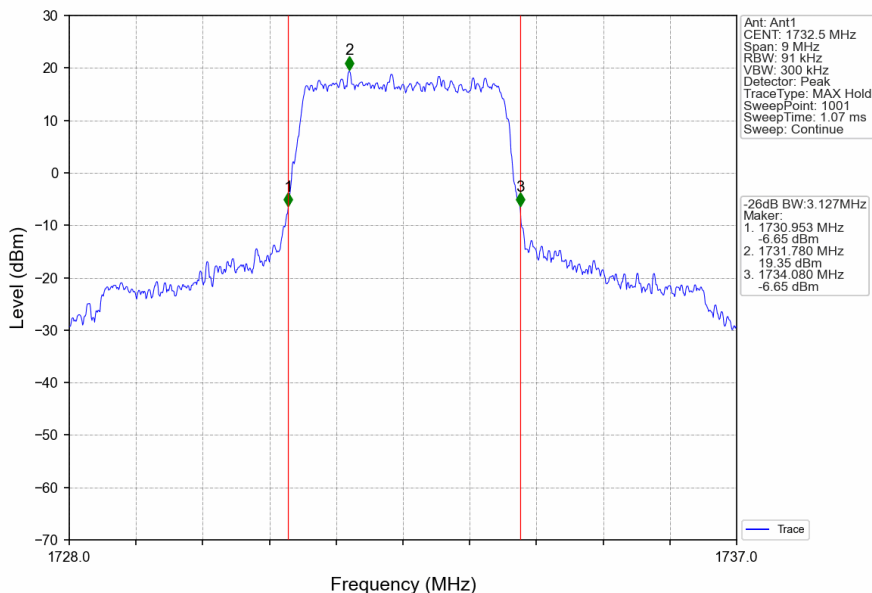
Band4_3MHz_QPSK_MCH_1732.5MHz_RB_15_0_NTNV
