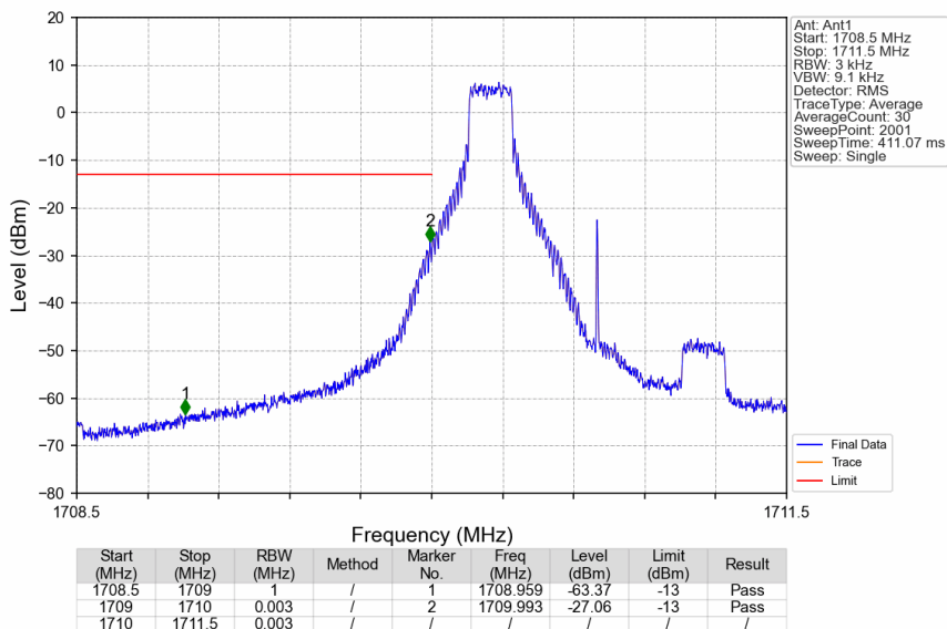
Band4_1.4MHz_16QAM_LCH_1710.7MHz_RB_1_0_NTNV
