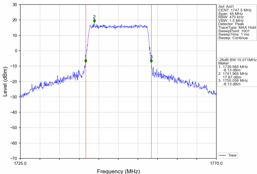
Band4_15MHz_16QAM_HCH_1747.5MHz_RB_75_0_NTNV
