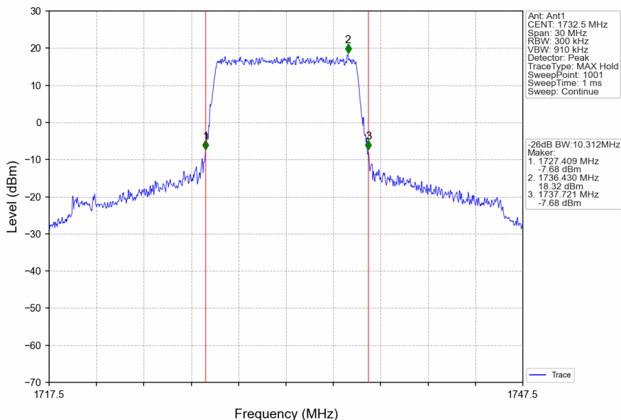
Band4_10MHz_QPSK_MCH_1732.5MHz_RB_50_0_NTNV
