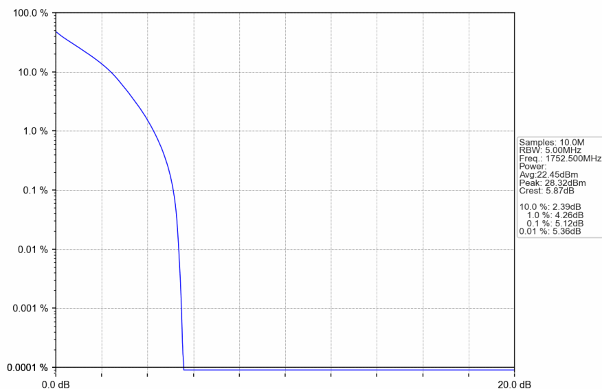
Band4_5MHz_QPSK_HCH_1752.5MHz_RB_25_0_NTNV
