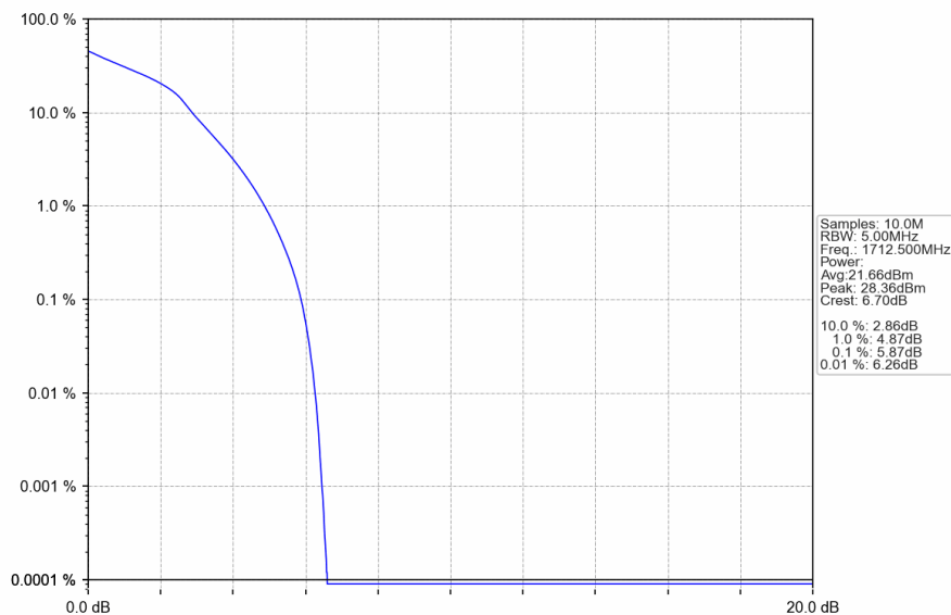
Band4_5MHz_16QAM_LCH_1712.5MHz_RB_25_0_NTNV
