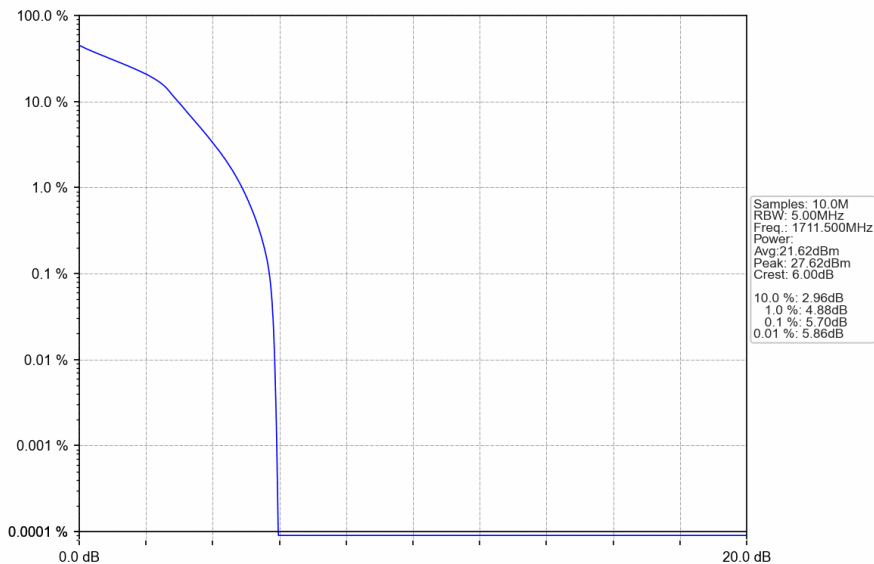
Band4_3MHz_16QAM_LCH_1711.5MHz_RB_15_0_NTNV
