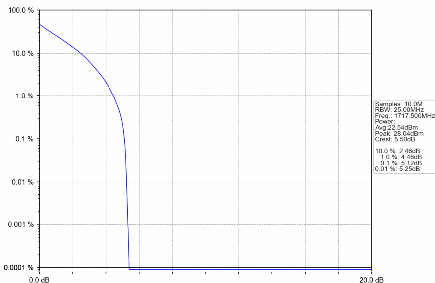
Band4_15MHz_QPSK_LCH_1717.5MHz_RB_75_0_NTNV
