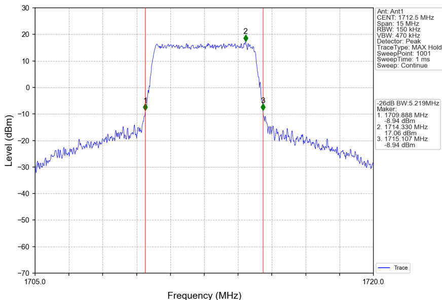
Band4_5MHz_16QAM_LCH_1712.5MHz_RB_25_0_NTNV
