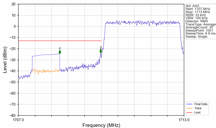
Band4_3MHz_QPSK_LCH_1711.5MHz_RB_15_0_NTNV
