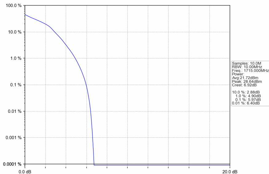
Band4_10MHz_16QAM_LCH_1715MHz_RB_50_0_NTNV
