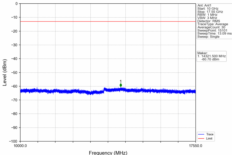
Band4_1.4MHz_16QAM_LCH_1710.7MHz_RB_6_0_NTNV
