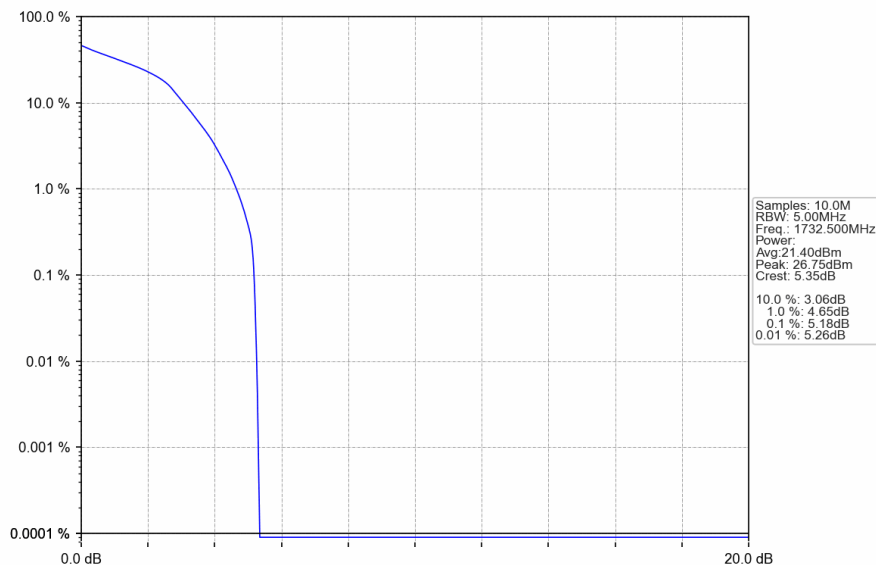
Band4_1.4MHz_16QAM_MCH_1732.5MHz_RB_6_0_NTNV
