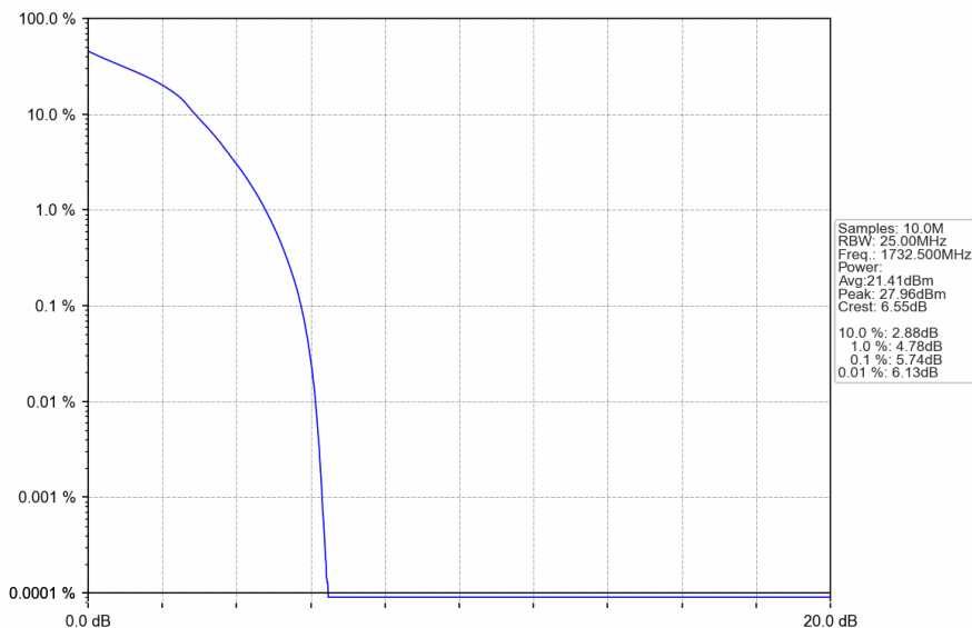
Band4_20MHz_16QAM_MCH_1732.5MHz_RB_100_0_NTNV
