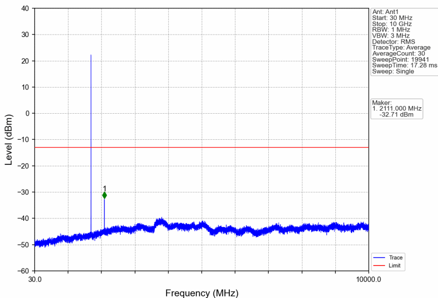
Band4_1.4MHz_QPSK_LCH_1710.7MHz_RB_1_0_NTNV
