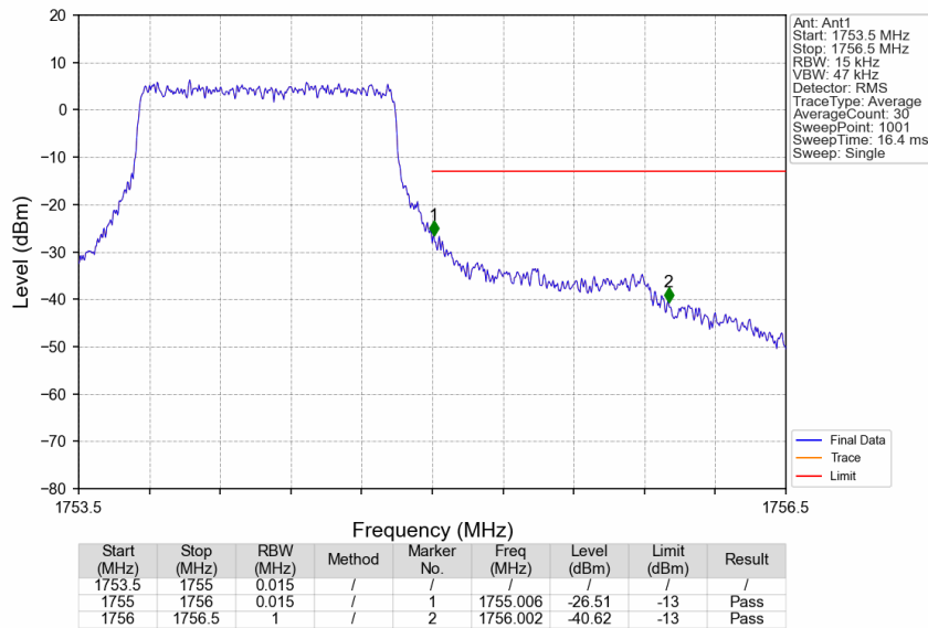
Band4_1.4MHz_QPSK_HCH_1754.3MHz_RB_6_0_NTNV
