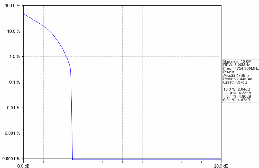
Band4_1.4MHz_QPSK_HCH_1754.3MHz_RB_6_0_NTNV
