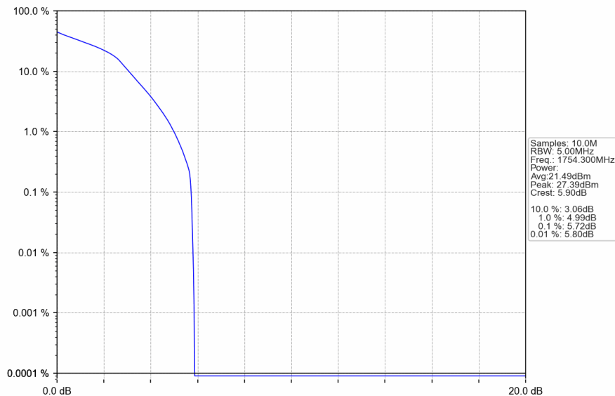
Band4_1.4MHz_16QAM_HCH_1754.3MHz_RB_6_0_NTNV
