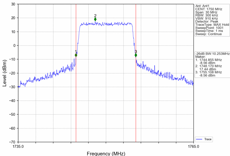
Band4_10MHz_16QAM_HCH_1750MHz_RB_50_0_NTNV
