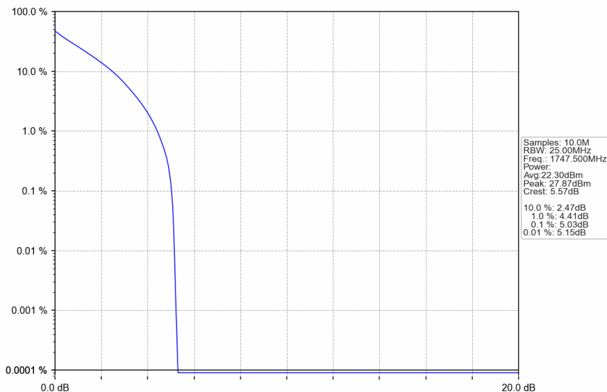
Band4_15MHz_QPSK_HCH_1747.5MHz_RB_75_0_NTNV
