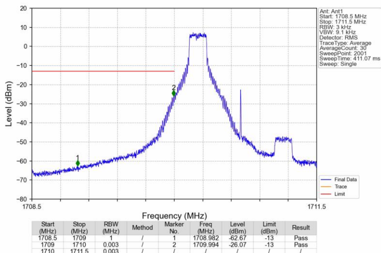
Band4_1.4MHz_QPSK_LCH_1710.7MHz_RB_1_0_NTNV
