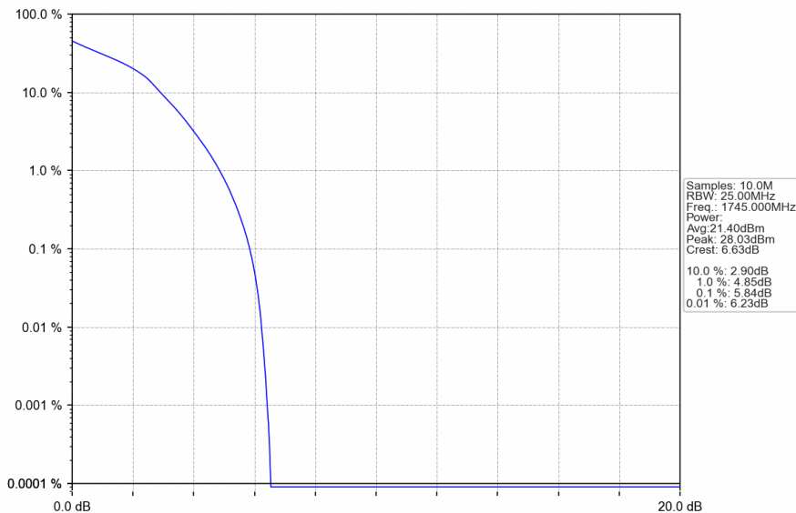
Band4_20MHz_16QAM_HCH_1745MHz_RB_100_0_NTNV
