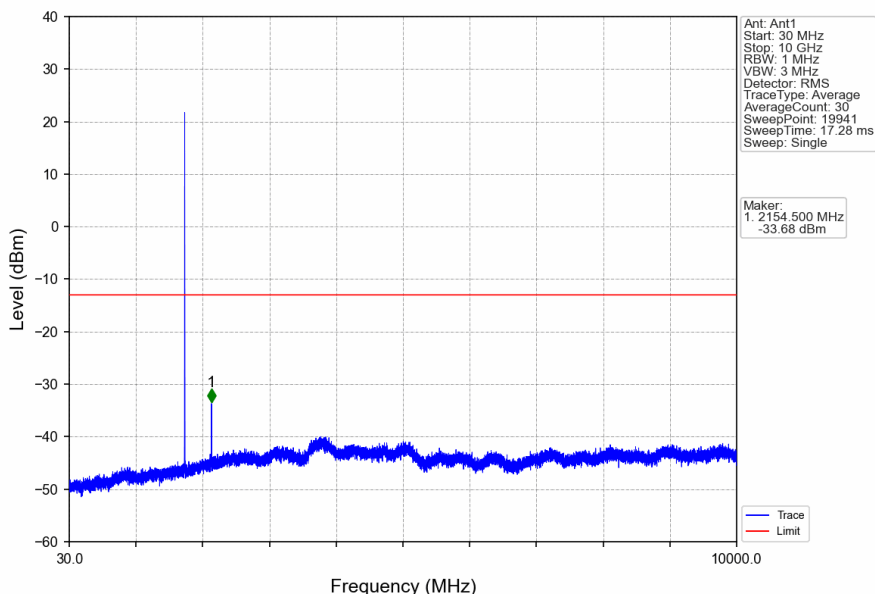
Band4_1.4MHz_16QAM_HCH_1754.3MHz_RB_1_0_NTNV
