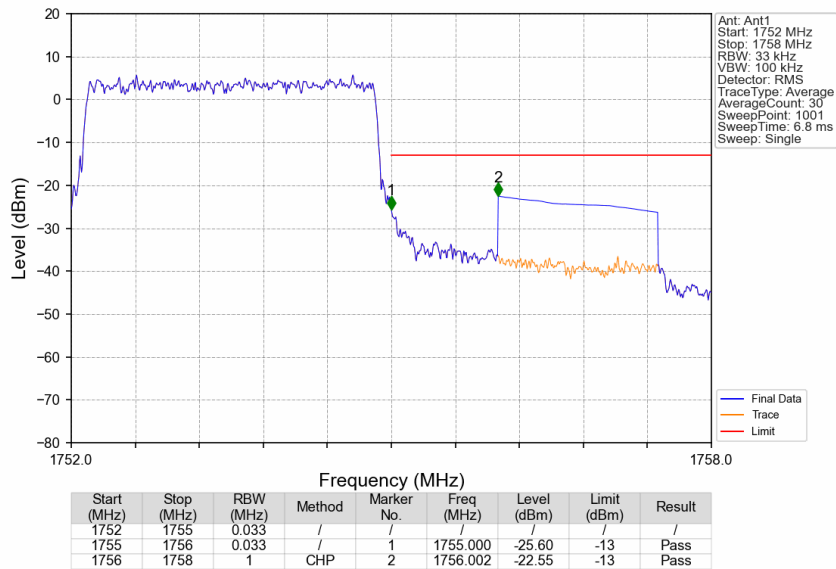
Band4_3MHz_QPSK_HCH_1753.5MHz_RB_15_0_NTNV
