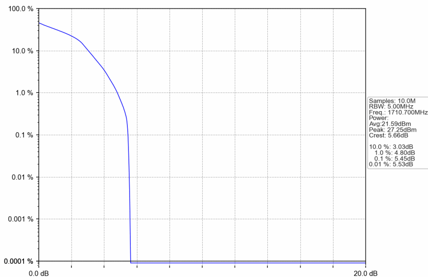
Band4_1.4MHz_16QAM_LCH_1710.7MHz_RB_6_0_NTNV
