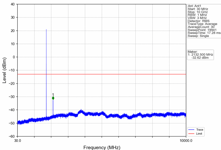
Band4_1.4MHz_16QAM_MCH_1732.5MHz_RB_1_0_NTNV
