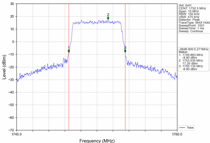
Band4_5MHz_16QAM_HCH_1752.5MHz_RB_25_0_NTNV
