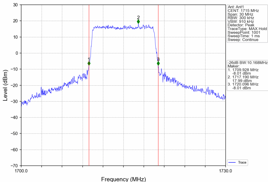
Band4_10MHz_16QAM_LCH_1715MHz_RB_50_0_NTNV
