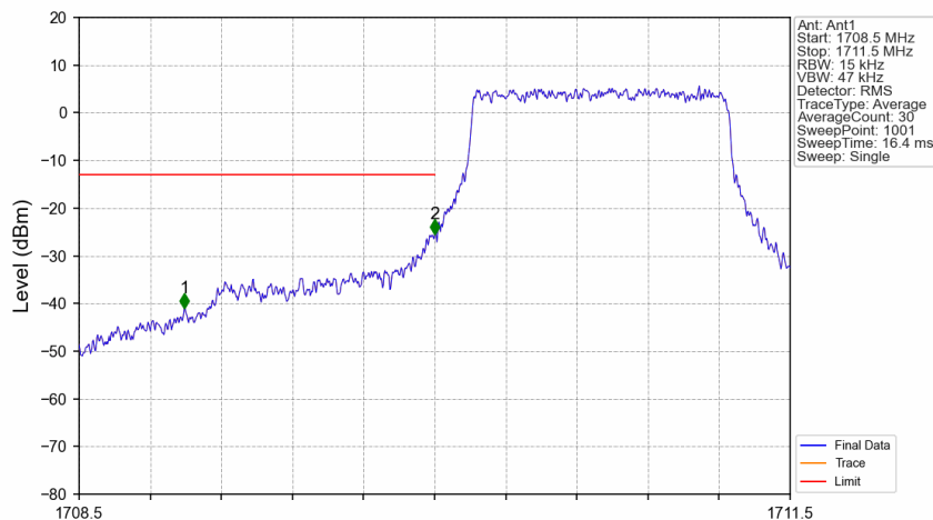
Band4_1.4MHz_QPSK_LCH_1710.7MHz_RB_6_0_NTNV
