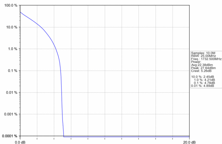
Band4_15MHz_QPSK_MCH_1732.5MHz_RB_75_0_NTNV
