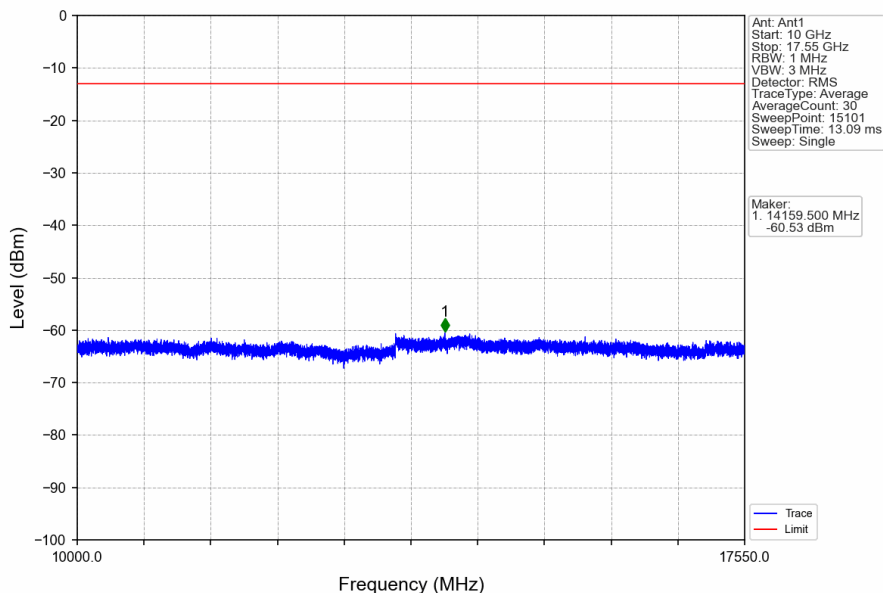
Band4_1.4MHz_16QAM_HCH_1754.3MHz_RB_1_0_NTNV
