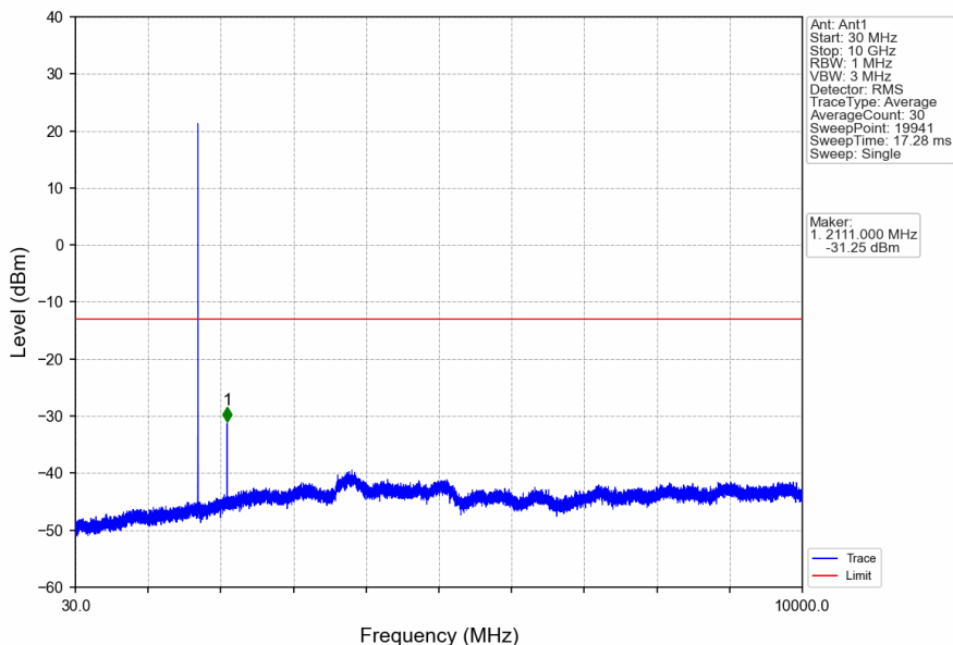
Band4_1.4MHz_16QAM_LCH_1710.7MHz_RB_1_0_NTNV
