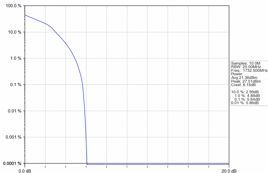
Band4_15MHz_16QAM_MCH_1732.5MHz_RB_75_0_NTNV
