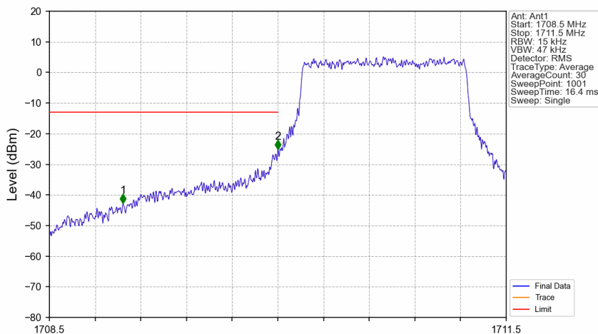
Band4_1.4MHz_16QAM_LCH_1710.7MHz_RB_6_0_NTNV
