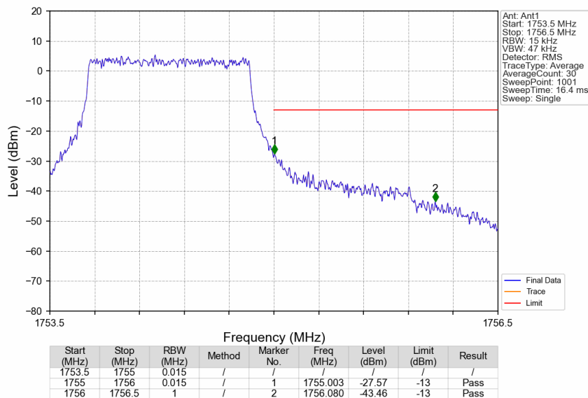
Band4_1.4MHz_16QAM_HCH_1754.3MHz_RB_6_0_NTNV
