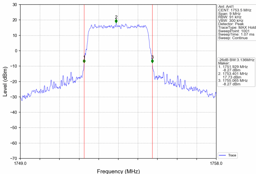
Band4_3MHz_16QAM_HCH_1753.5MHz_RB_15_0_NTNV
