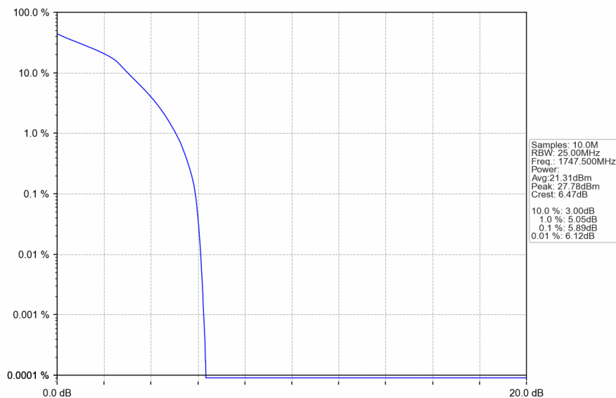
Band4_15MHz_16QAM_HCH_1747.5MHz_RB_75_0_NTNV
