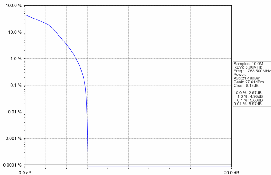
Band4_3MHz_16QAM_HCH_1753.5MHz_RB_15_0_NTNV
