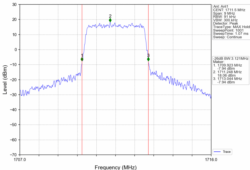
Band4_3MHz_16QAM_LCH_1711.5MHz_RB_15_0_NTNV
