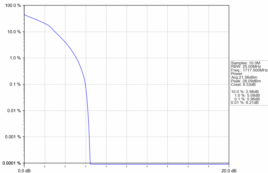
Band4_15MHz_16QAM_LCH_1717.5MHz_RB_75_0_NTNV
