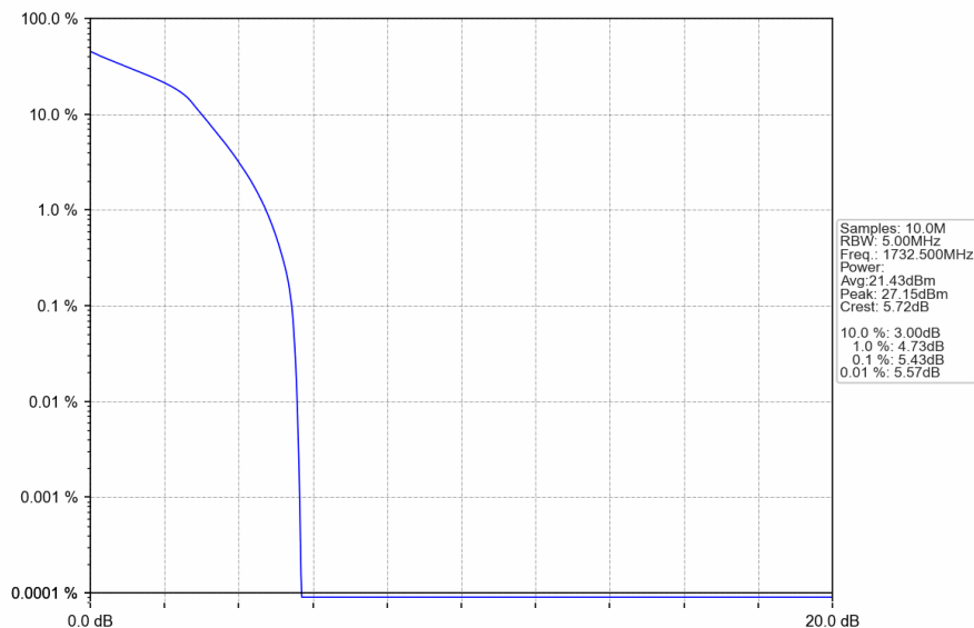
Band4_3MHz_16QAM_MCH_1732.5MHz_RB_15_0_NTNV
