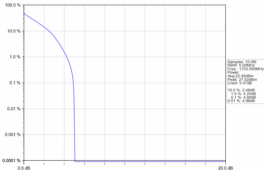
Band4_3MHz_QPSK_HCH_1753.5MHz_RB_15_0_NTNV
