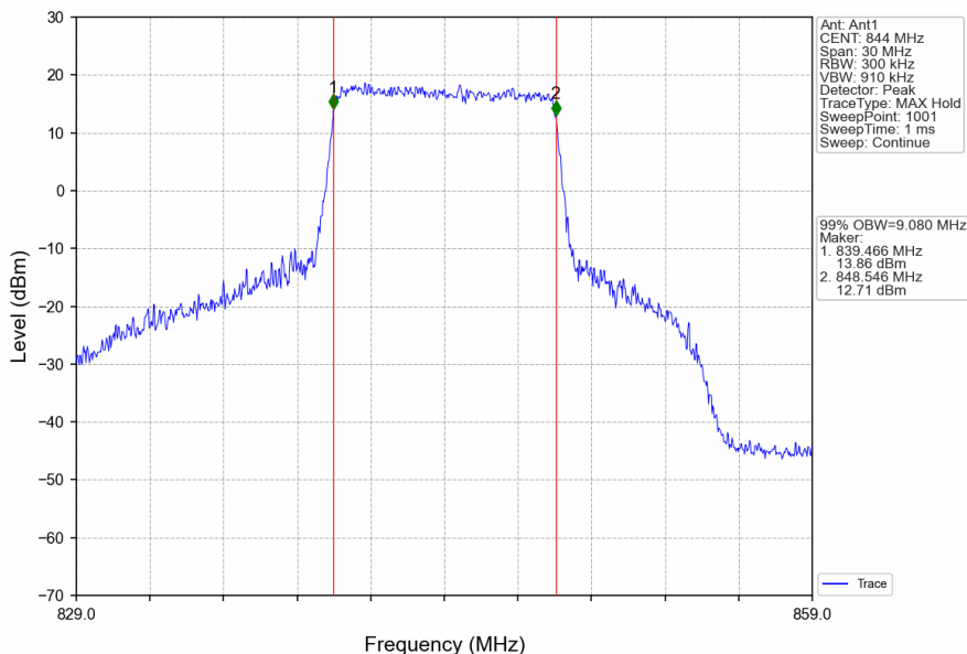
Band5_10MHz_16QAM_HCH_844MHz_RB_50_0_NTNV
