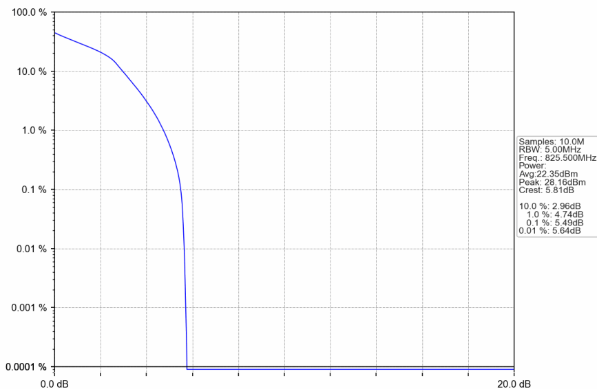
Band5_3MHz_16QAM_LCH_825.5MHz_RB_15_0_NTNV
