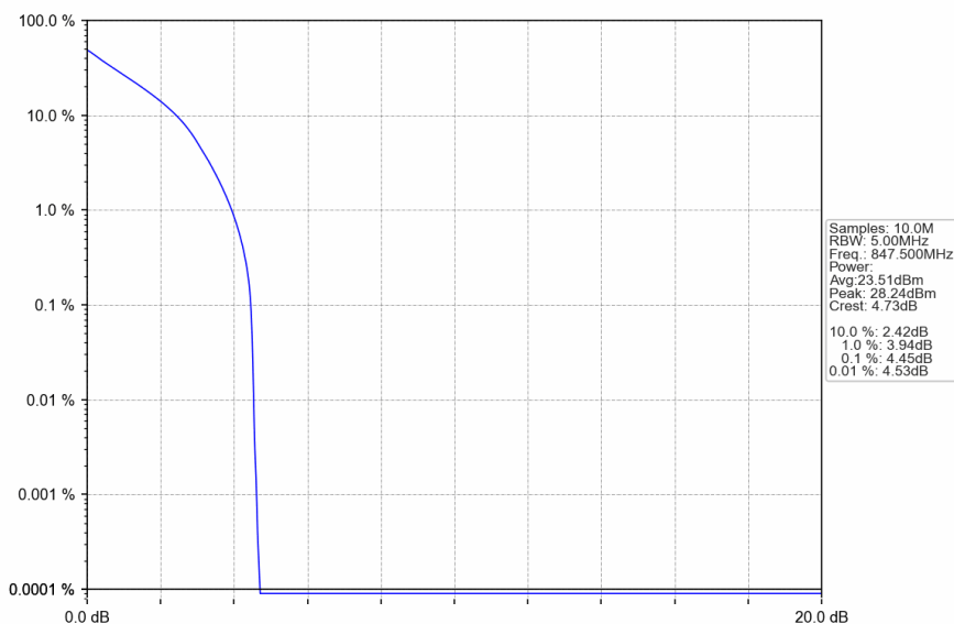
Band5_3MHz_QPSK_HCH_847.5MHz_RB_15_0_NTNV
