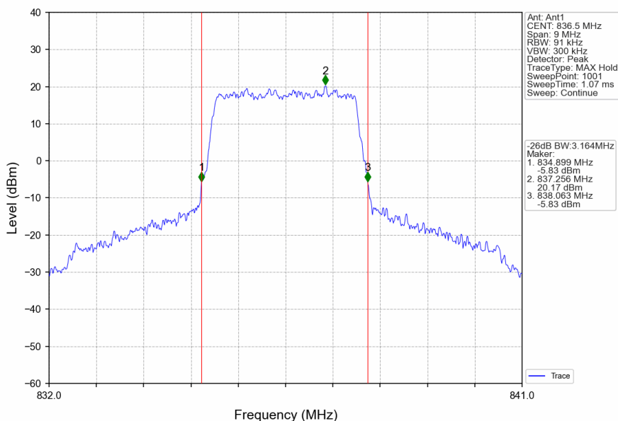
Band5_3MHz_QPSK_MCH_836.5MHz_RB_15_0_NTNV
