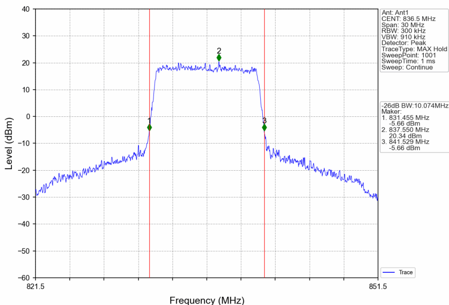
Band5_10MHz_QPSK_MCH_836.5MHz_RB_50_0_NTNV
