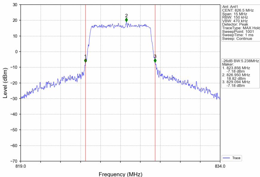
Band5_5MHz_16QAM_LCH_826.5MHz_RB_25_0_NTNV
