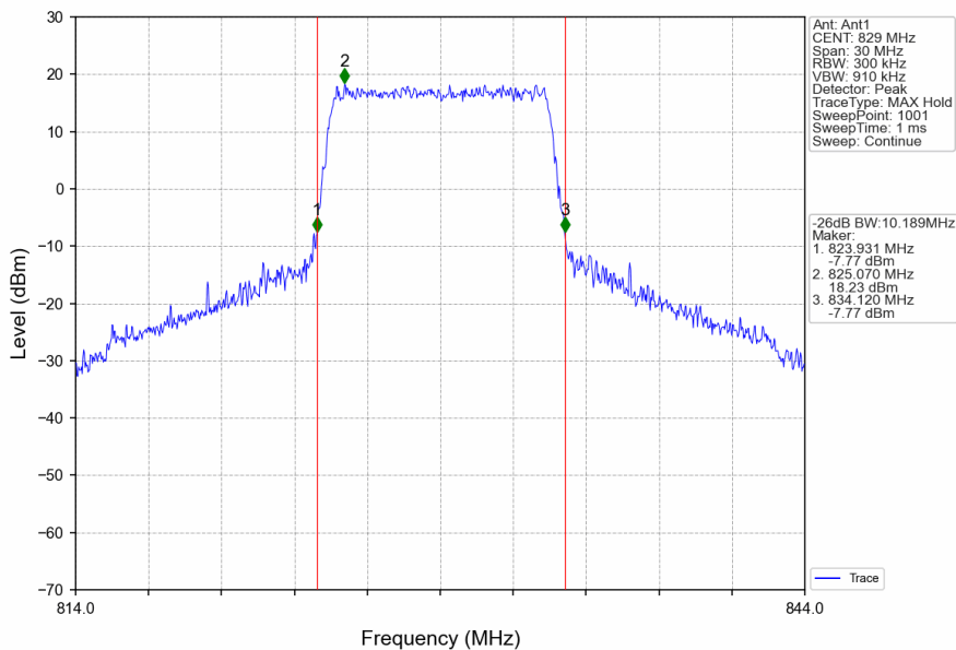
Band5_10MHz_16QAM_LCH_829MHz_RB_50_0_NTNV
