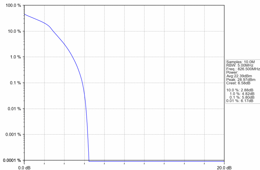
Band5_5MHz_16QAM_LCH_826.5MHz_RB_25_0_NTNV
