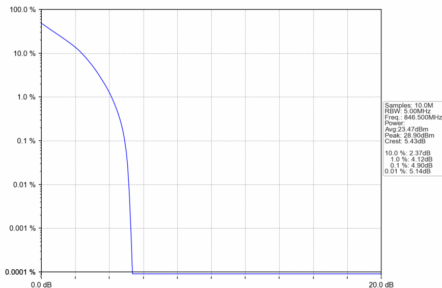
Band5_5MHz_QPSK_HCH_846.5MHz_RB_25_0_NTNV
