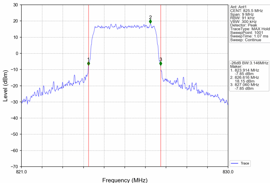
Band5_3MHz_16QAM_LCH_825.5MHz_RB_15_0_NTNV
