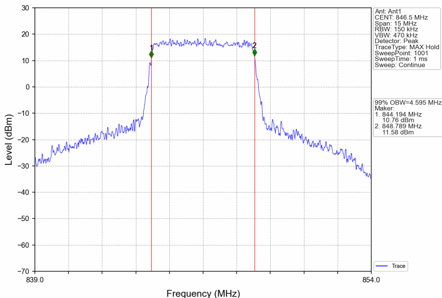
Band5_5MHz_16QAM_HCH_846.5MHz_RB_25_0_NTNV
