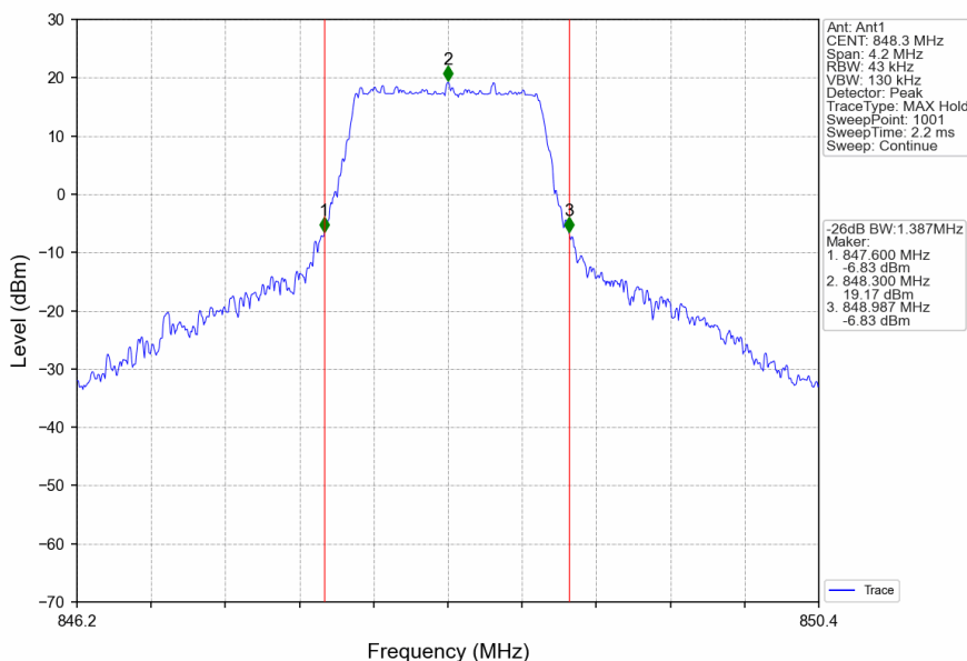
Band5_1.4MHz_16QAM_HCH_848.3MHz_RB_6_0_NTNV
