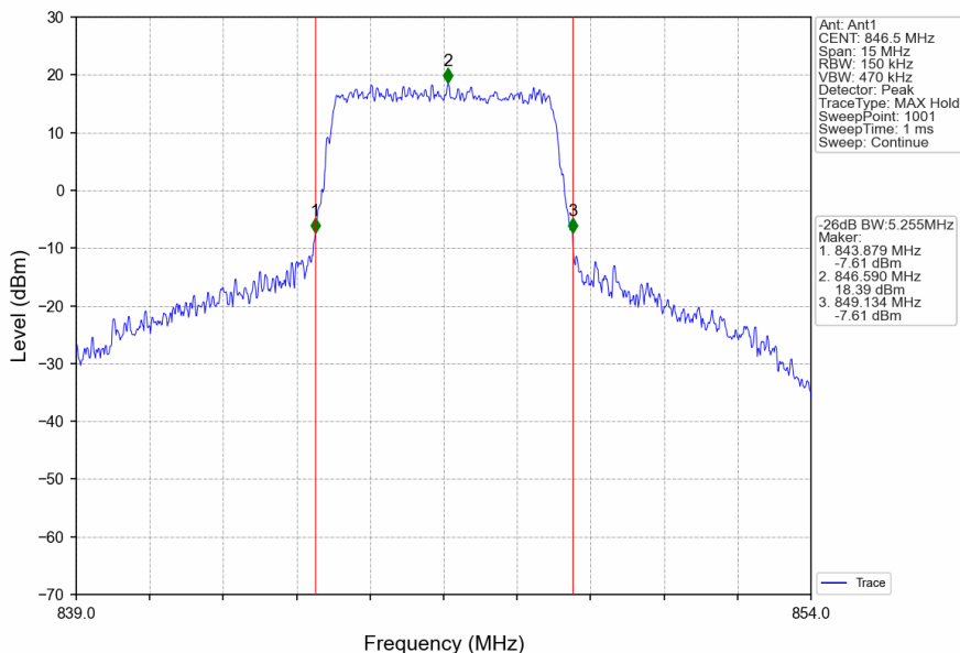
Band5_5MHz_16QAM_HCH_846.5MHz_RB_25_0_NTNV
