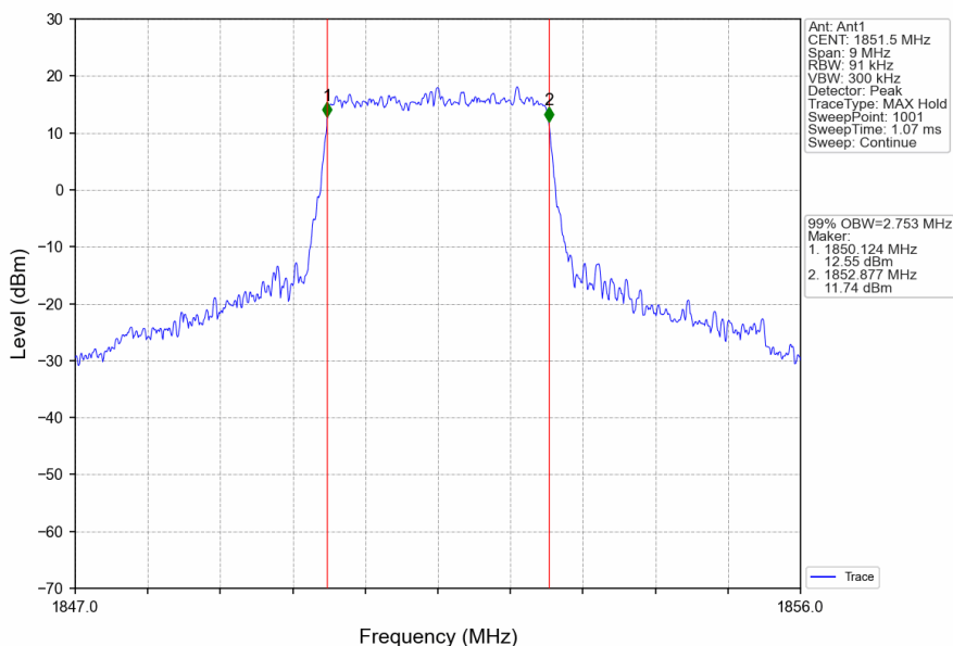
Band25_3MHz_16QAM_LCH_1851.5MHz_RB_15_0_NTNV
