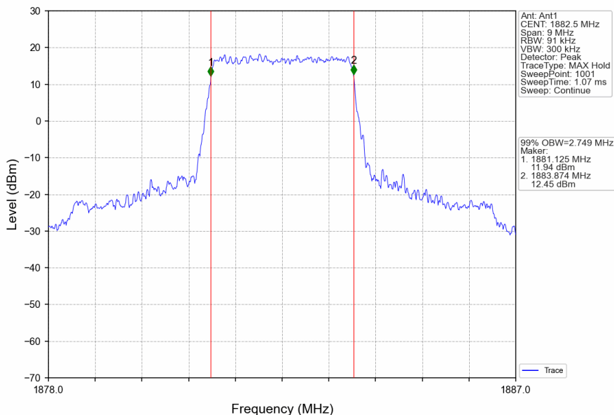
Band25_3MHz_QPSK_MCH_1882.5MHz_RB_15_0_NTNV
