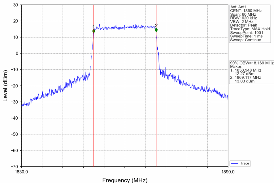
Band25_20MHz_16QAM_LCH_1860MHz_RB_100_0_NTNV
