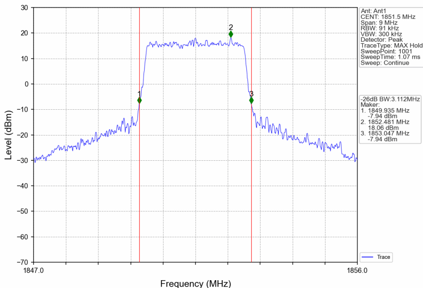
Band25_3MHz_16QAM_LCH_1851.5MHz_RB_15_0_NTNV
