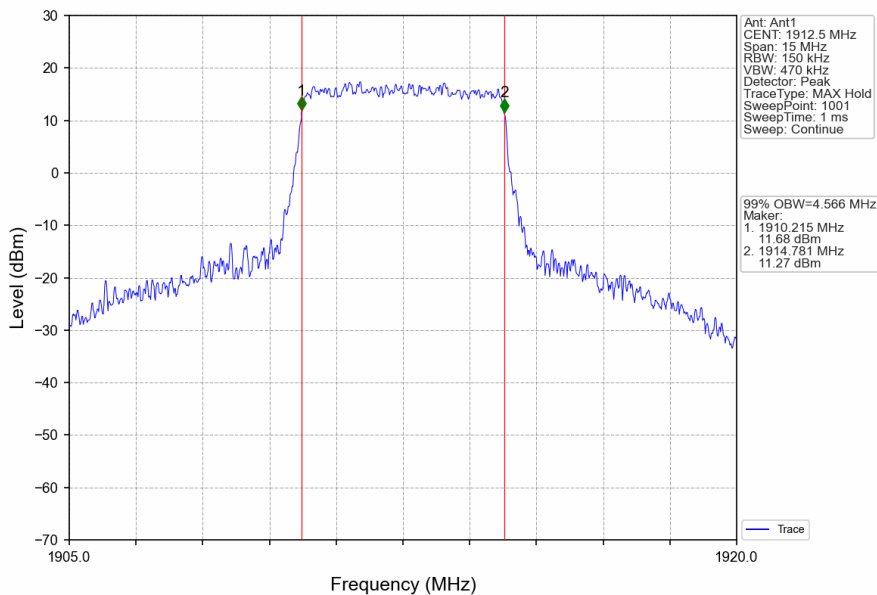
Band25_5MHz_16QAM_HCH_1912.5MHz_RB_25_0_NTNV
