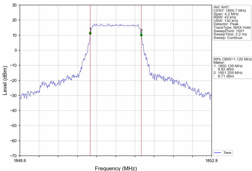
Band25_1.4MHz_16QAM_LCH_1850.7MHz_RB_6_0_NTNV
