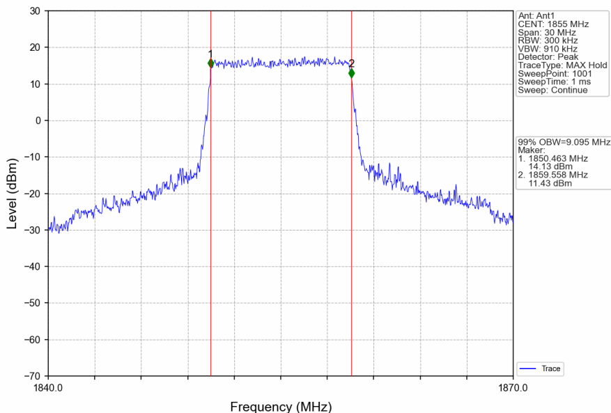
Band25_10MHz_16QAM_LCH_1855MHz_RB_50_0_NTNV
