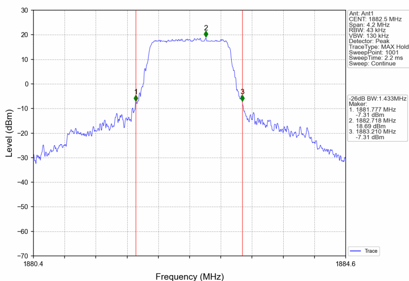
Band25_1.4MHz_QPSK_MCH_1882.5MHz_RB_6_0_NTNV
