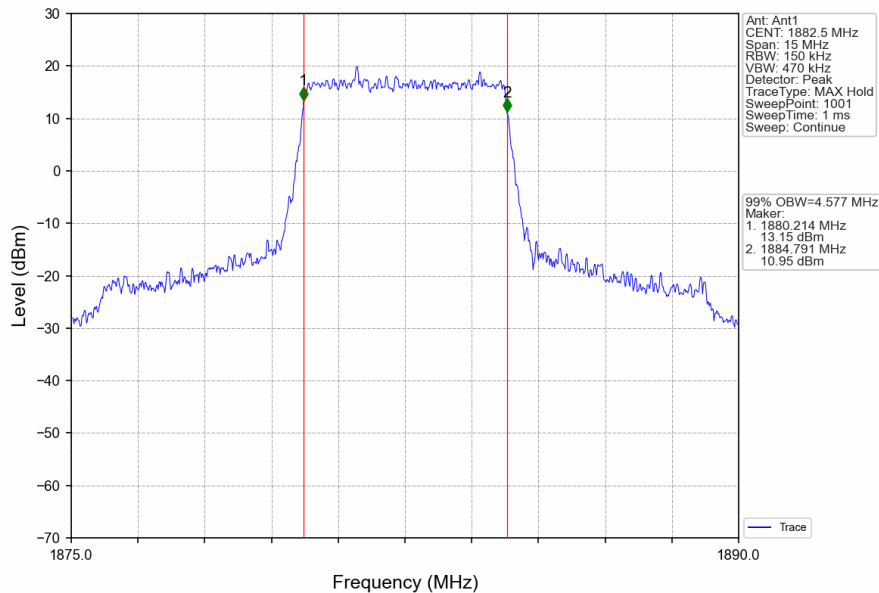
Band25_5MHz_QPSK_MCH_1882.5MHz_RB_25_0_NTNV
