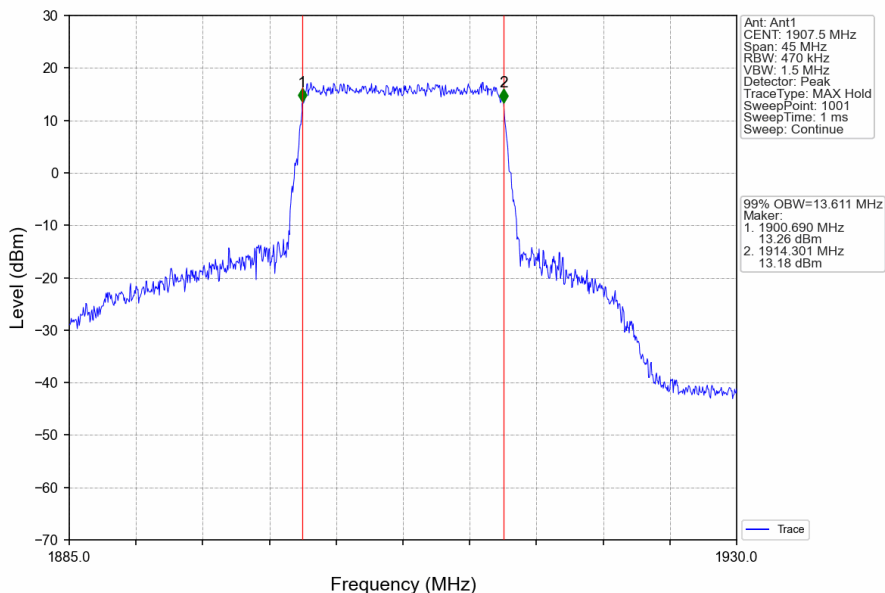
Band25_15MHz_16QAM_HCH_1907.5MHz_RB_75_0_NTNV
