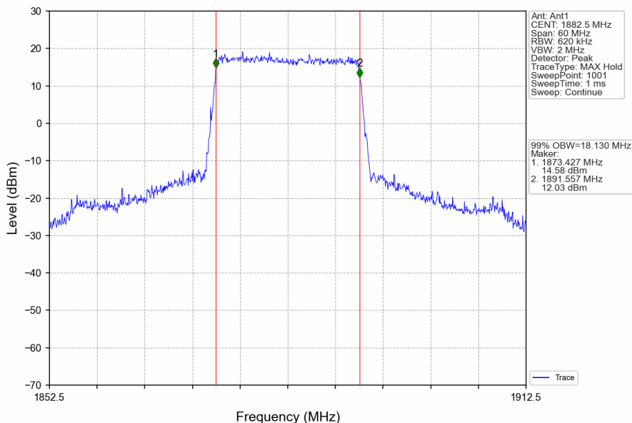
Band25_20MHz_QPSK_MCH_1882.5MHz_RB_100_0_NTNV
