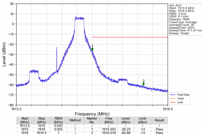
Band25_1.4MHz_QPSK_HCH_1914.3MHz_RB_1_5_NTNV
