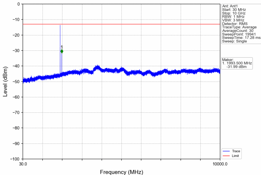
Band25_3MHz_16QAM_HCH_1913.5MHz_RB_1_0_NTNV
