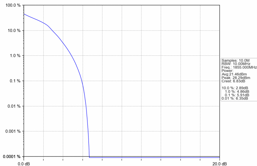
Band25_10MHz_16QAM_LCH_1855MHz_RB_50_0_NTNV
