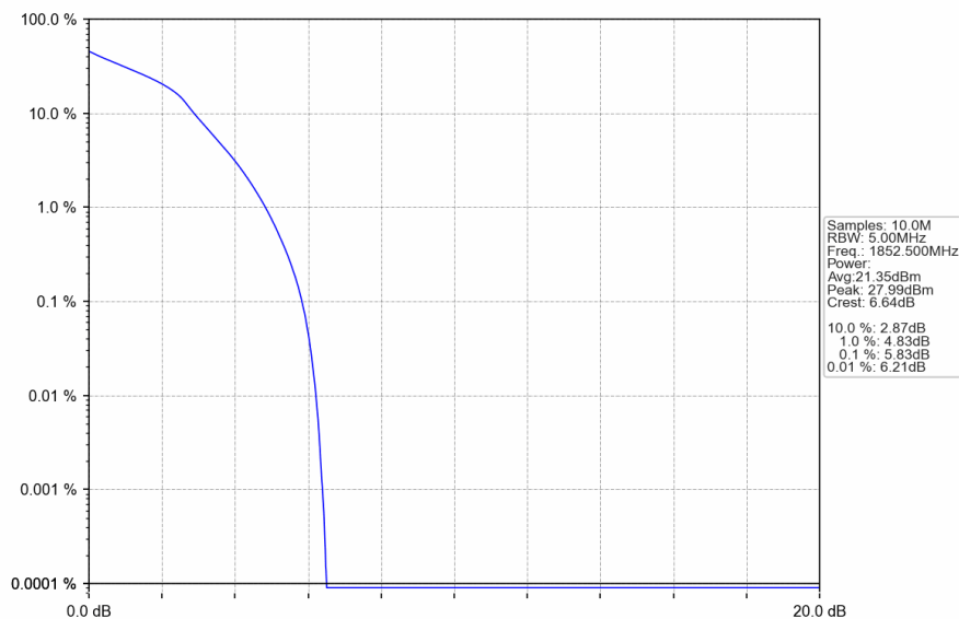
Band25_5MHz_16QAM_LCH_1852.5MHz_RB_25_0_NTNV
