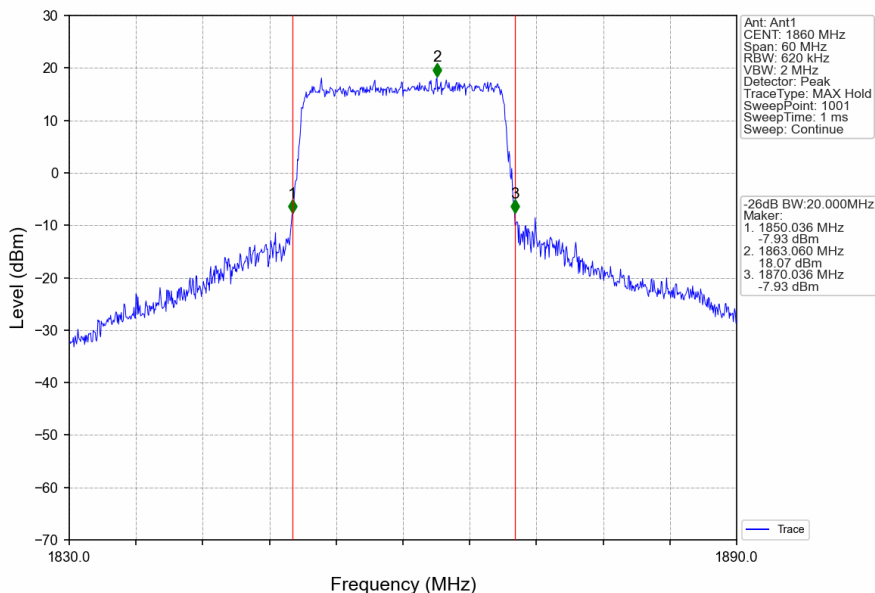
Band25_20MHz_16QAM_LCH_1860MHz_RB_100_0_NTNV
