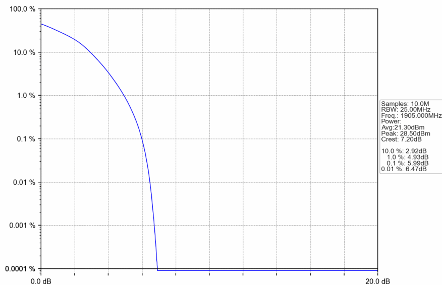
Band25_20MHz_16QAM_HCH_1905MHz_RB_100_0_NTNV
