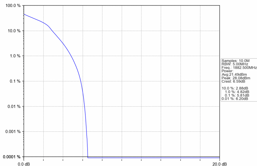
Band25_5MHz_16QAM_MCH_1882.5MHz_RB_25_0_NTNV
