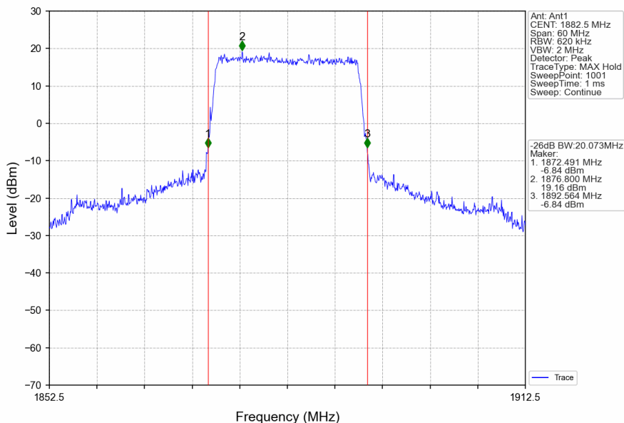
Band25_20MHz_QPSK_MCH_1882.5MHz_RB_100_0_NTNV
