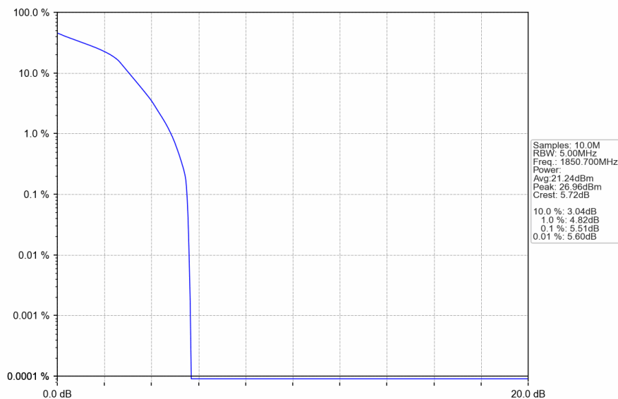
Band25_1.4MHz_16QAM_LCH_1850.7MHz_RB_6_0_NTNV
