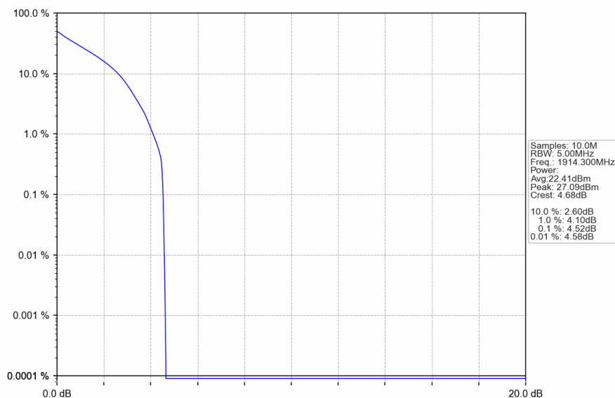
Band25_1.4MHz_QPSK_HCH_1914.3MHz_RB_6_0_NTNV
