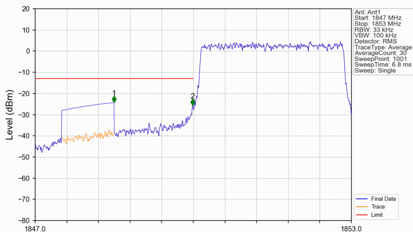
Band25_3MHz_16QAM_LCH_1851.5MHz_RB_15_0_NTNV
