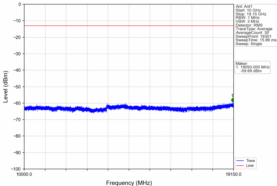
Band25_1.4MHz_QPSK_LCH_1850.7MHz_RB_6_0_NTNV
