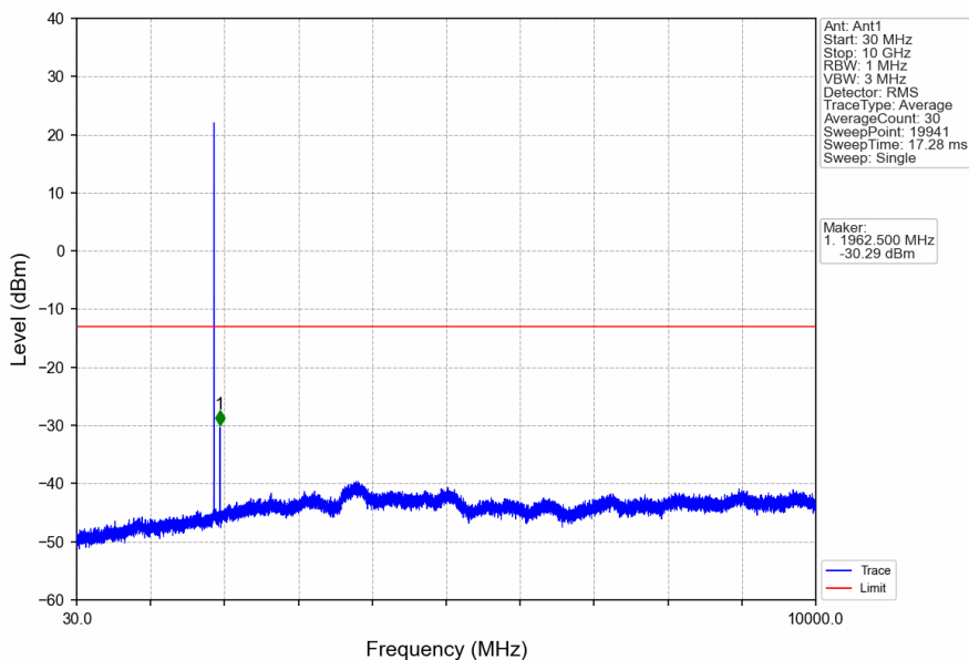
Band25_3MHz_16QAM_MCH_1882.5MHz_RB_1_0_NTNV
