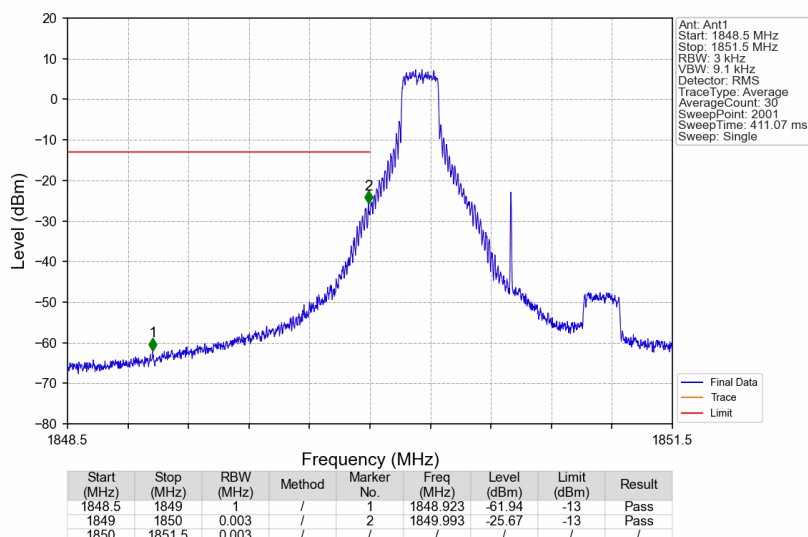
Band25_1.4MHz_QPSK_LCH_1850.7MHz_RB_1_0_NTNV
