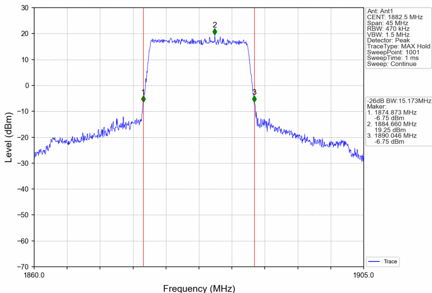
Band25_15MHz_QPSK_MCH_1882.5MHz_RB_75_0_NTNV
