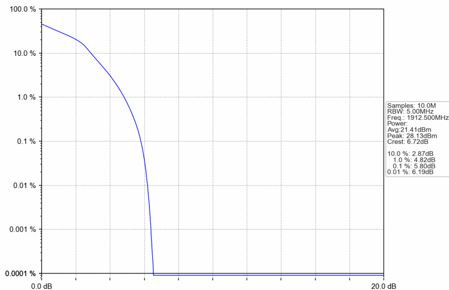
Band25_5MHz_16QAM_HCH_1912.5MHz_RB_25_0_NTNV
