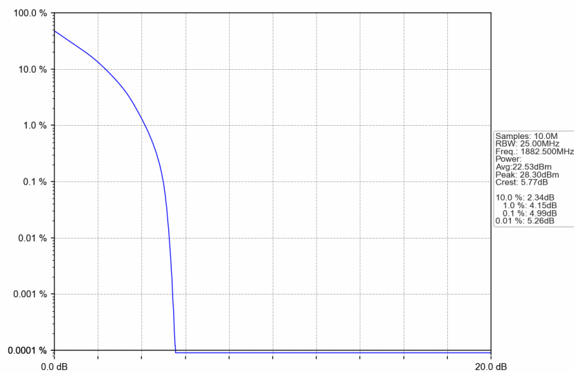
Band25_20MHz_QPSK_MCH_1882.5MHz_RB_100_0_NTNV
