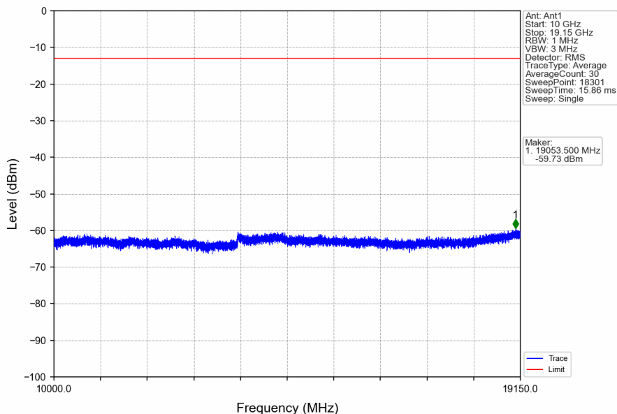
Band25_3MHz_16QAM_MCH_1882.5MHz_RB_1_0_NTNV
