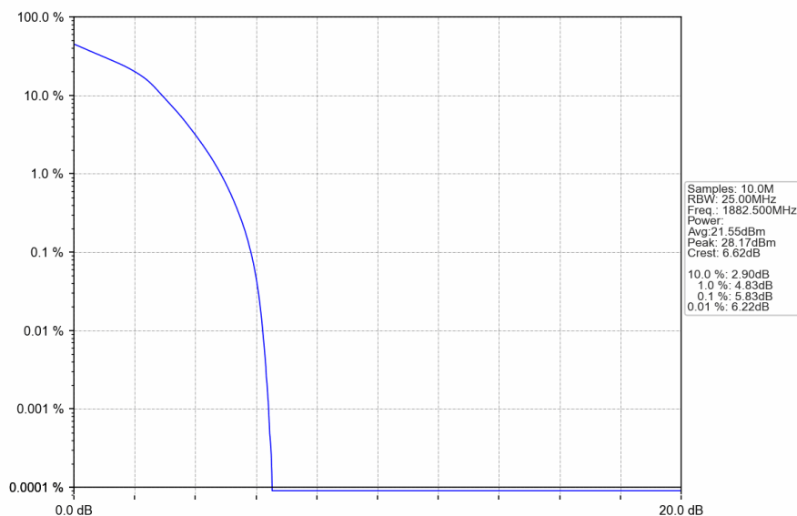
Band25_20MHz_16QAM_MCH_1882.5MHz_RB_100_0_NTNV
