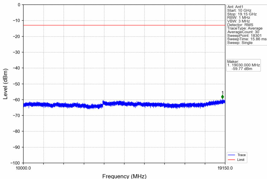
Band25_3MHz_QPSK_MCH_1882.5MHz_RB_1_0_NTNV
