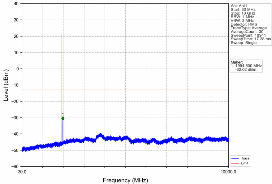
Band25_1.4MHz_16QAM_HCH_1914.3MHz_RB_1_0_NTNV
