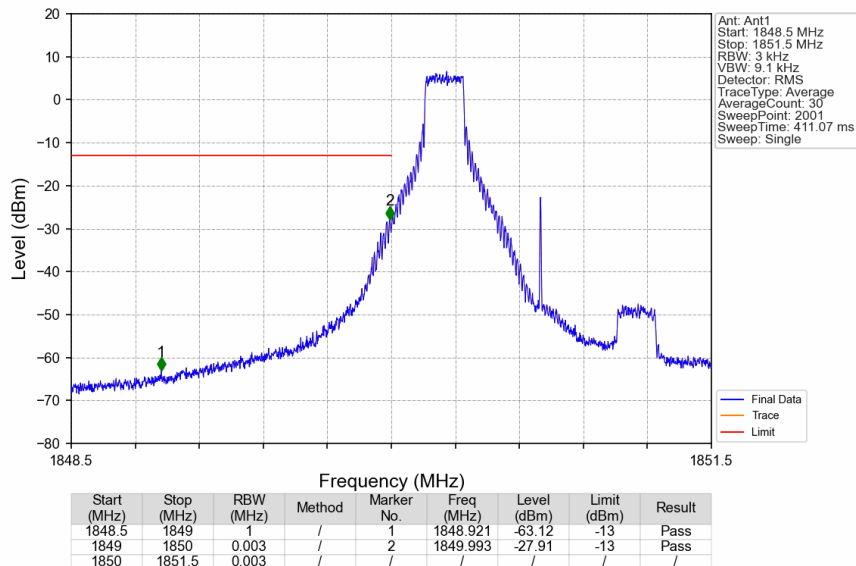
Band25_1.4MHz_16QAM_LCH_1850.7MHz_RB_1_0_NTNV
