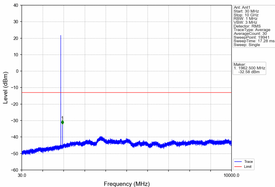
Band25_1.4MHz_16QAM_MCH_1882.5MHz_RB_1_0_NTNV
