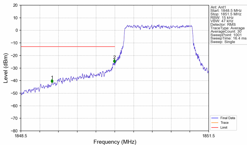
Band25_1.4MHz_16QAM_LCH_1850.7MHz_RB_6_0_NTNV
