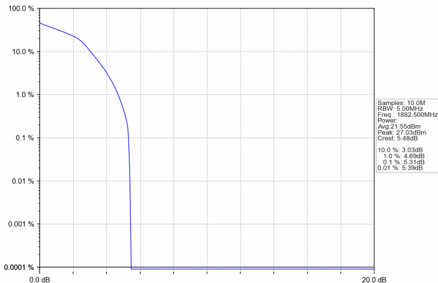
Band25_1.4MHz_16QAM_MCH_1882.5MHz_RB_6_0_NTNV
