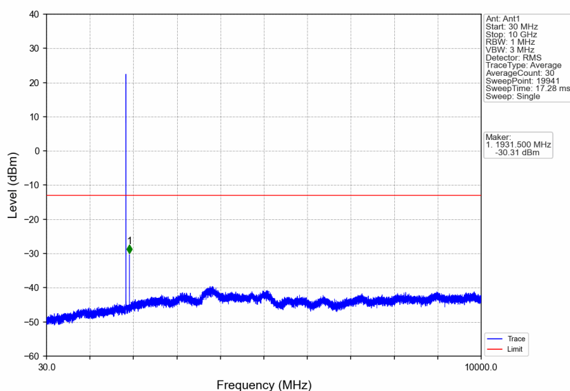
Band25_3MHz_QPSK_LCH_1851.5MHz_RB_1_0_NTNV
