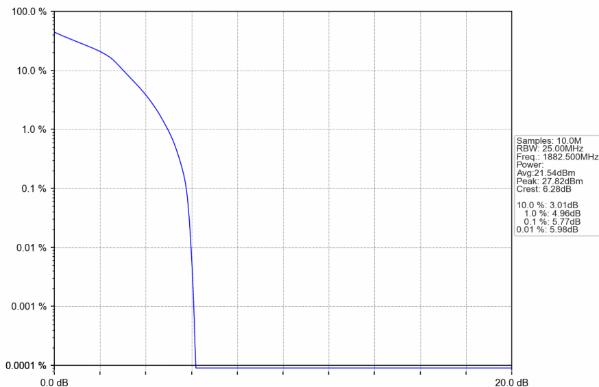
Band25_15MHz_16QAM_MCH_1882.5MHz_RB_75_0_NTNV
