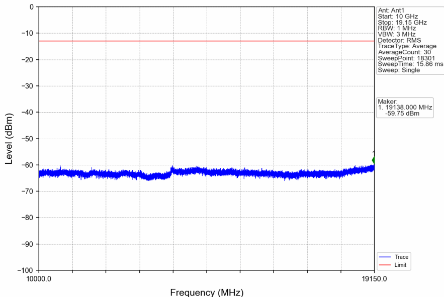
Band25_1.4MHz_QPSK_MCH_1882.5MHz_RB_1_0_NTNV
