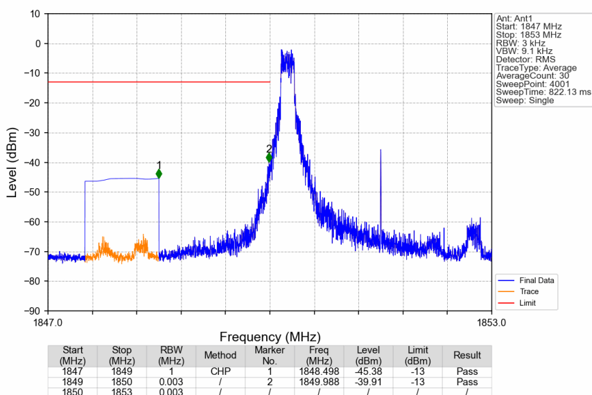
Band25_3MHz_QPSK_LCH_1851.5MHz_RB_1_0_NTNV
