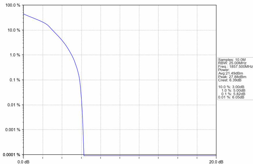
Band25_15MHz_16QAM_LCH_1857.5MHz_RB_75_0_NTNV
