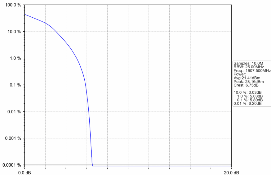
Band25_15MHz_16QAM_HCH_1907.5MHz_RB_75_0_NTNV
