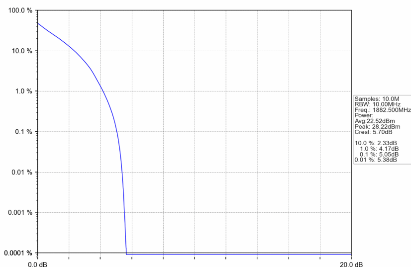
Band25_10MHz_QPSK_MCH_1882.5MHz_RB_50_0_NTNV
