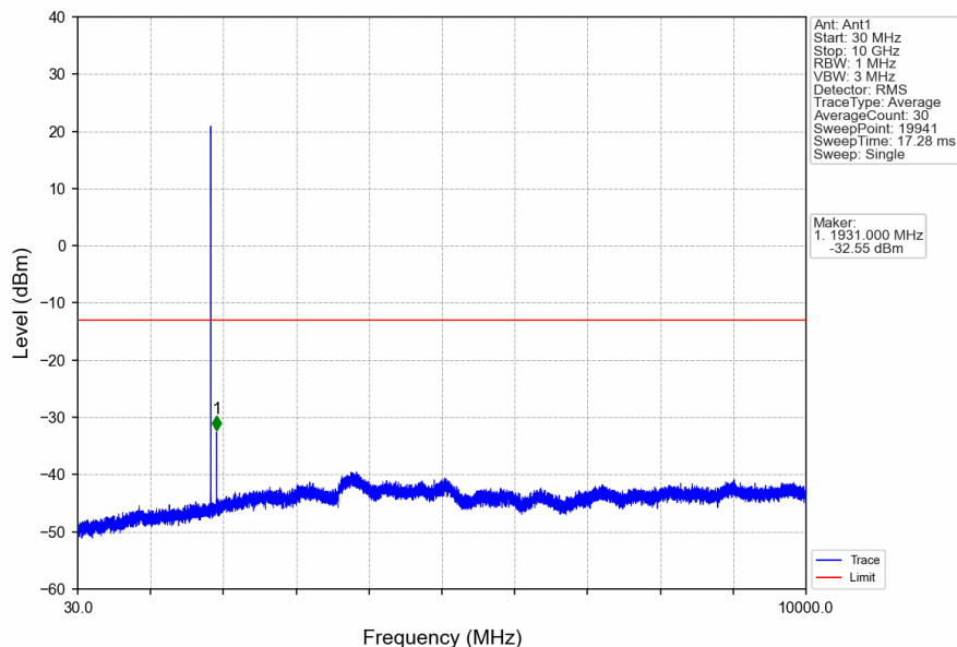
Band25_1.4MHz_16QAM_LCH_1850.7MHz_RB_1_0_NTNV
