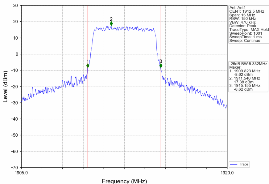
Band25_5MHz_16QAM_HCH_1912.5MHz_RB_25_0_NTNV
