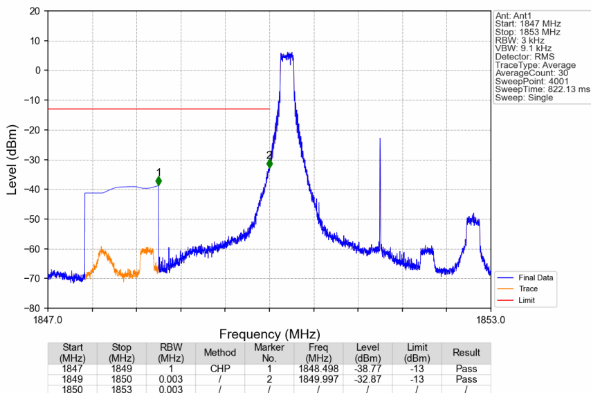
Band25_3MHz_16QAM_LCH_1851.5MHz_RB_1_0_NTNV
