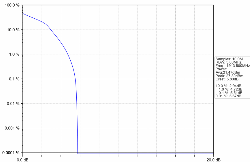
Band25_3MHz_16QAM_HCH_1913.5MHz_RB_15_0_NTNV
