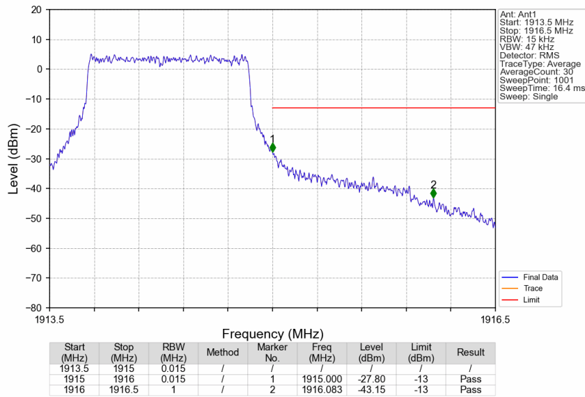
Band25_1.4MHz_16QAM_HCH_1914.3MHz_RB_6_0_NTNV
