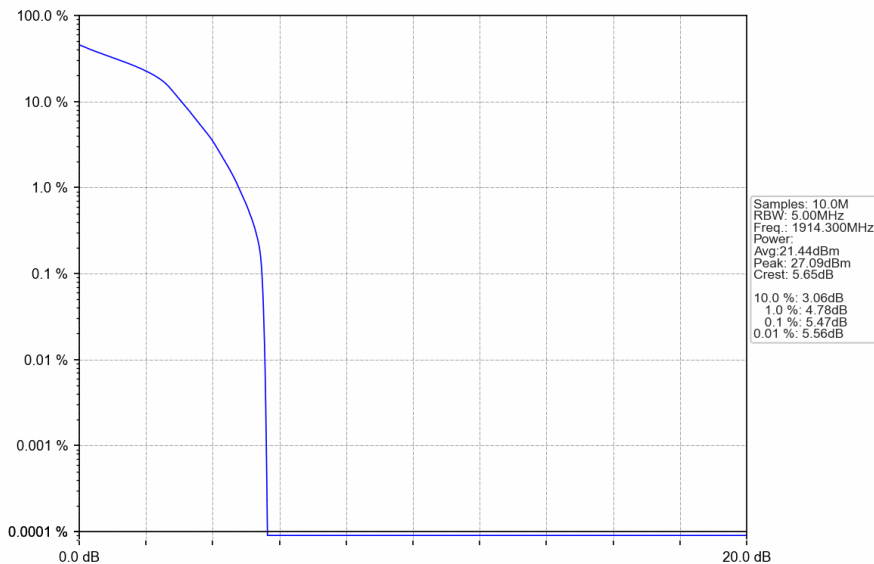
Band25_1.4MHz_16QAM_HCH_1914.3MHz_RB_6_0_NTNV
