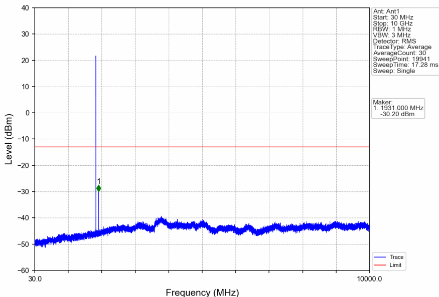
Band25_3MHz_16QAM_LCH_1851.5MHz_RB_1_0_NTNV
