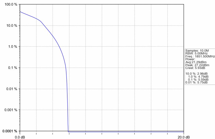
Band25_3MHz_16QAM_LCH_1851.5MHz_RB_15_0_NTNV
