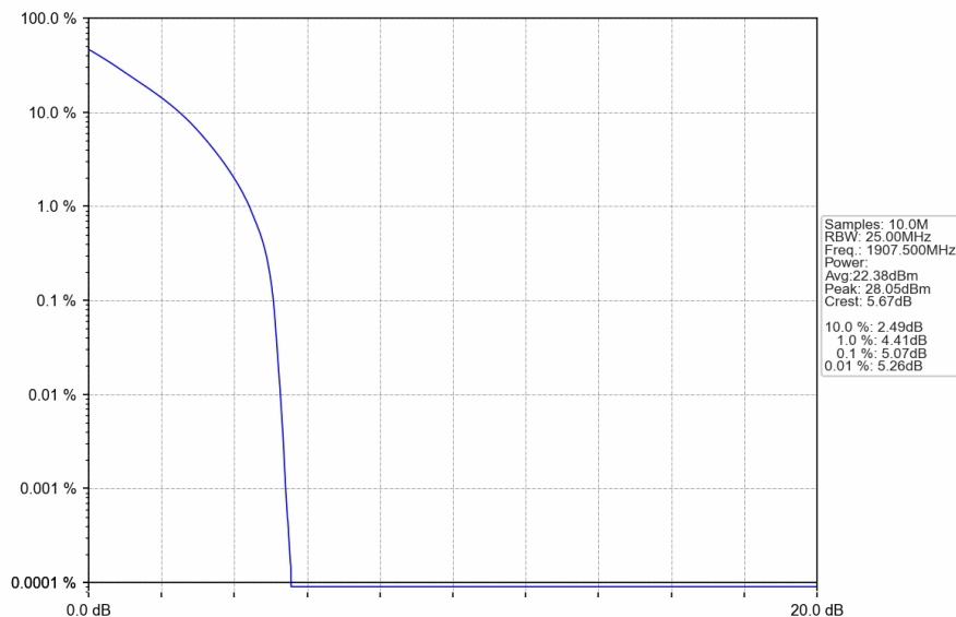
Band25_15MHz_QPSK_HCH_1907.5MHz_RB_75_0_NTNV
