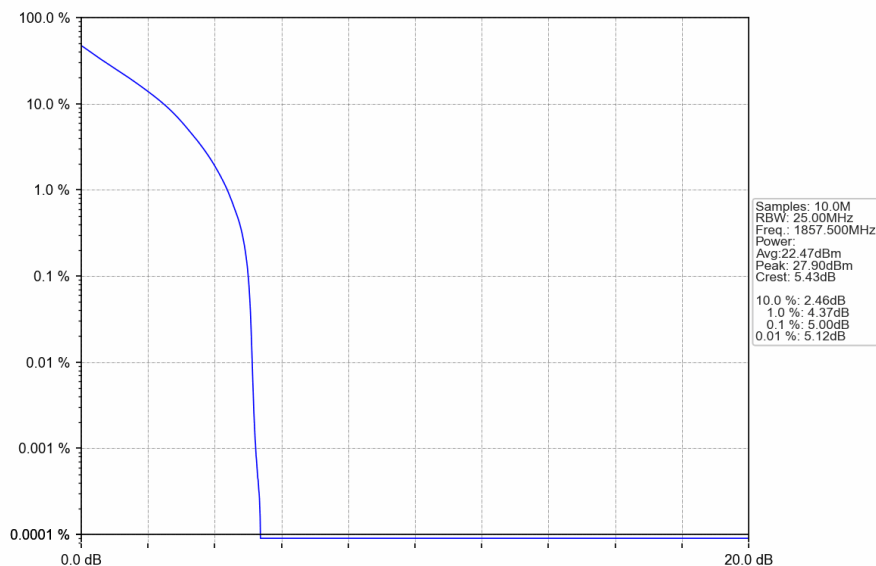
Band25_15MHz_QPSK_LCH_1857.5MHz_RB_75_0_NTNV
