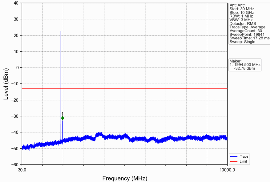
Band25_1.4MHz_QPSK_HCH_1914.3MHz_RB_1_0_NTNV
