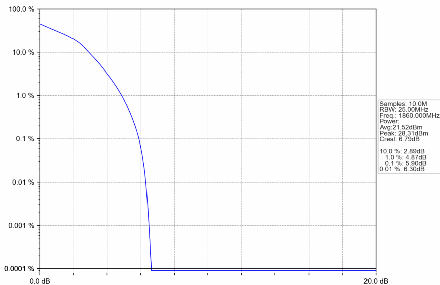
Band25_20MHz_16QAM_LCH_1860MHz_RB_100_0_NTNV
