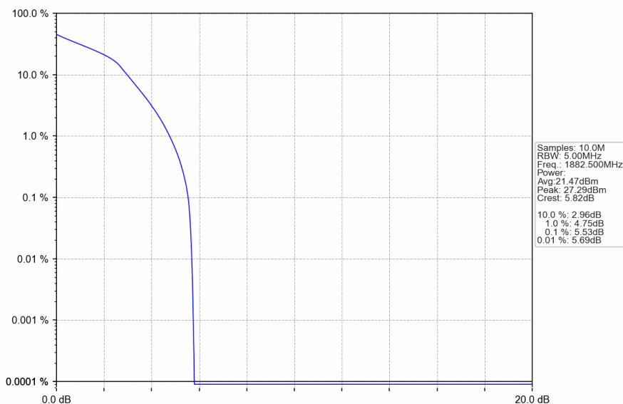
Band25_3MHz_16QAM_MCH_1882.5MHz_RB_15_0_NTNV
