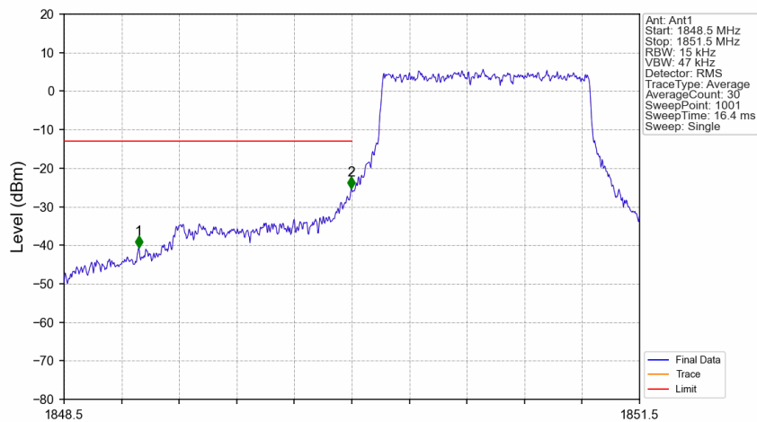
Band25_1.4MHz_QPSK_LCH_1850.7MHz_RB_6_0_NTNV
