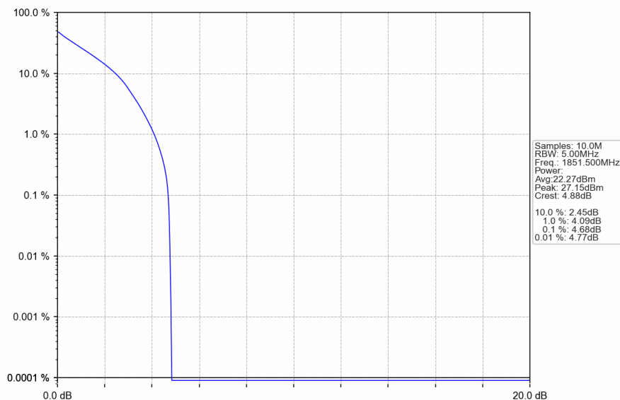
Band25_3MHz_QPSK_LCH_1851.5MHz_RB_15_0_NTNV
