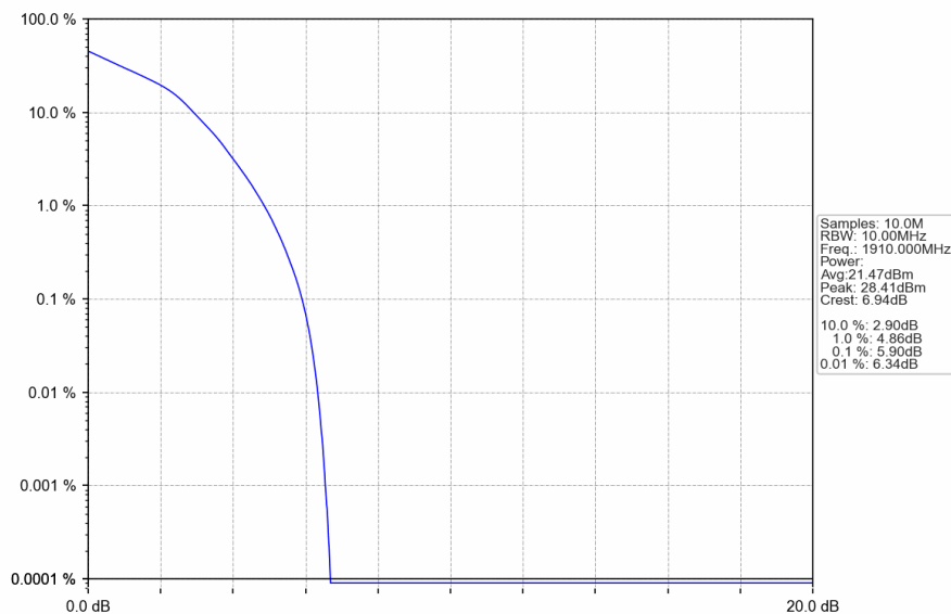
Band25_10MHz_16QAM_HCH_1910MHz_RB_50_0_NTNV
