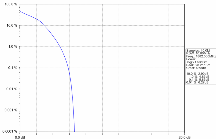
Band25_10MHz_16QAM_MCH_1882.5MHz_RB_50_0_NTNV
