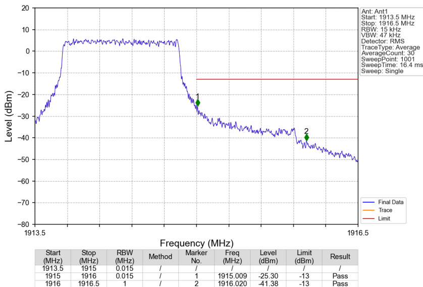
Band25_1.4MHz_QPSK_HCH_1914.3MHz_RB_6_0_NTNV
