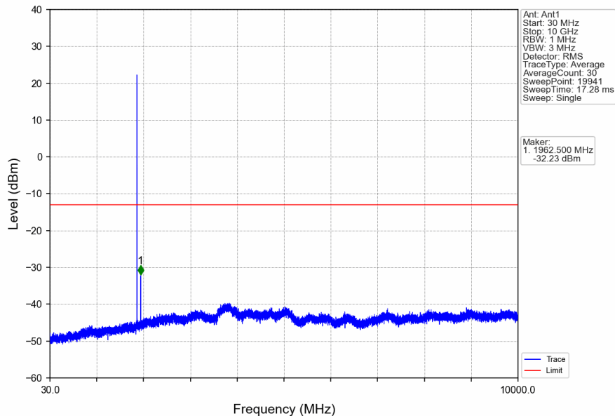
Band25_1.4MHz_QPSK_MCH_1882.5MHz_RB_1_0_NTNV
