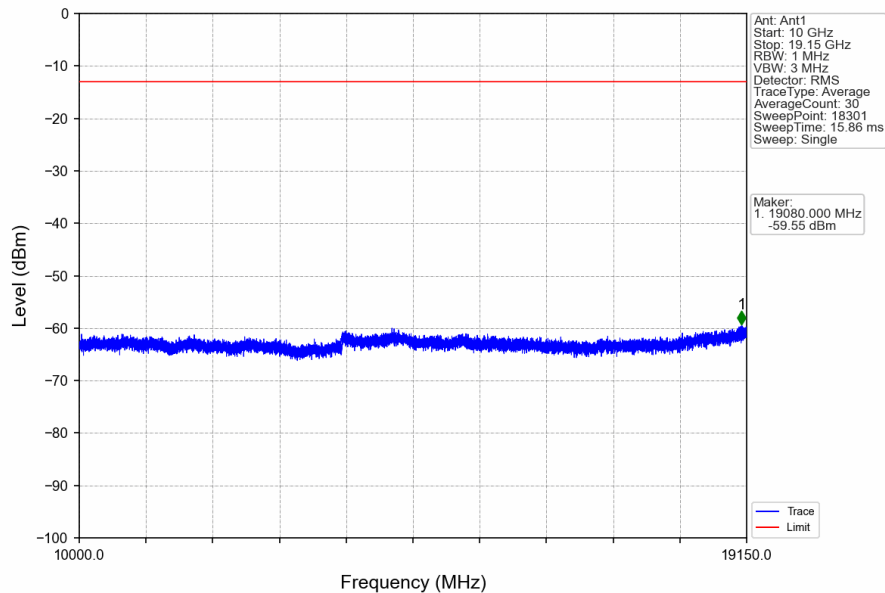
Band25_1.4MHz_QPSK_HCH_1914.3MHz_RB_1_0_NTNV
