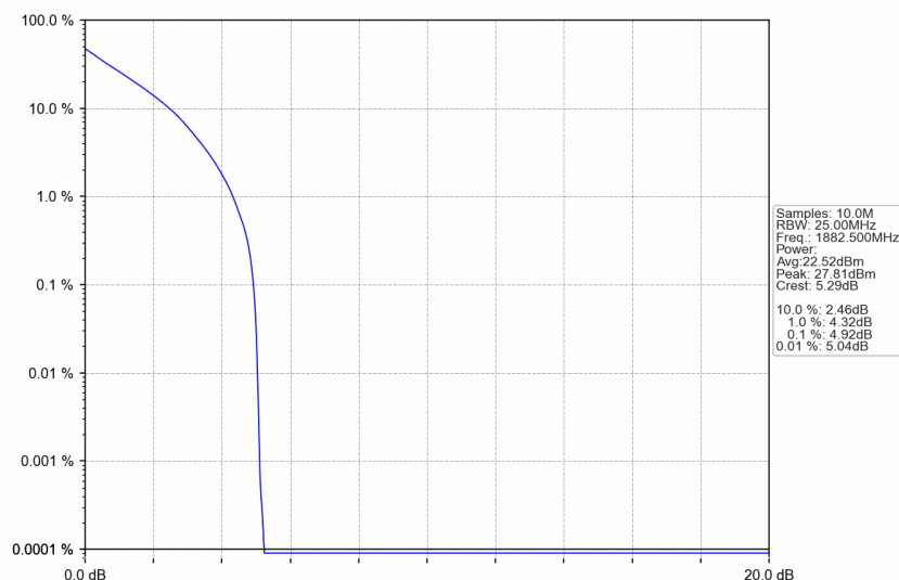
Band25_15MHz_QPSK_MCH_1882.5MHz_RB_75_0_NTNV
