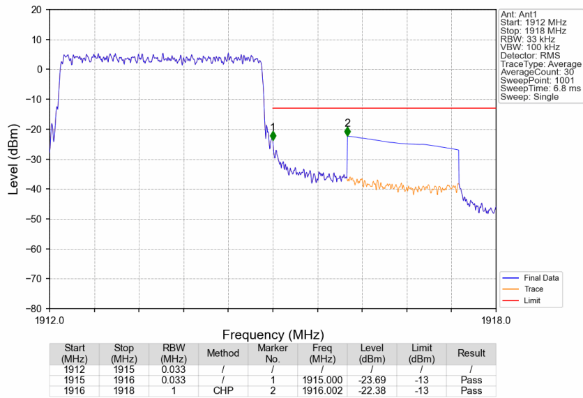
Band25_3MHz_QPSK_HCH_1913.5MHz_RB_15_0_NTNV
