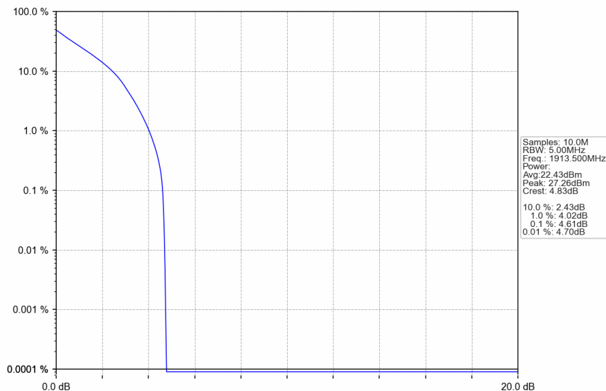
Band25_3MHz_QPSK_HCH_1913.5MHz_RB_15_0_NTNV
