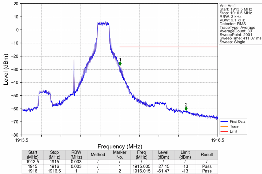
Band25_1.4MHz_16QAM_HCH_1914.3MHz_RB_1_5_NTNV
