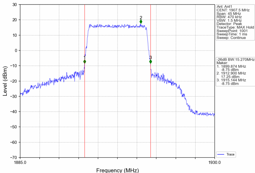
Band25_15MHz_16QAM_HCH_1907.5MHz_RB_75_0_NTNV
