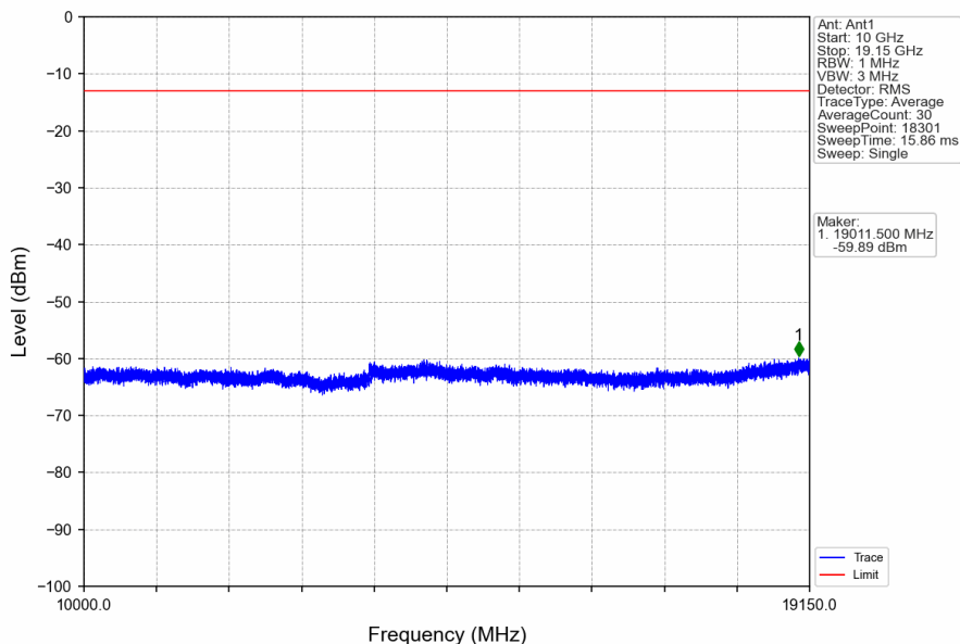
Band25_1.4MHz_16QAM_MCH_1882.5MHz_RB_1_0_NTNV
