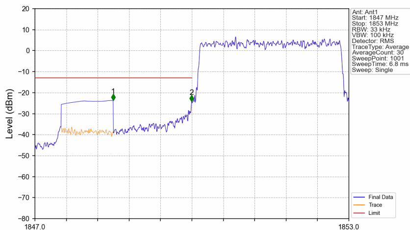
Band25_3MHz_QPSK_LCH_1851.5MHz_RB_15_0_NTNV
