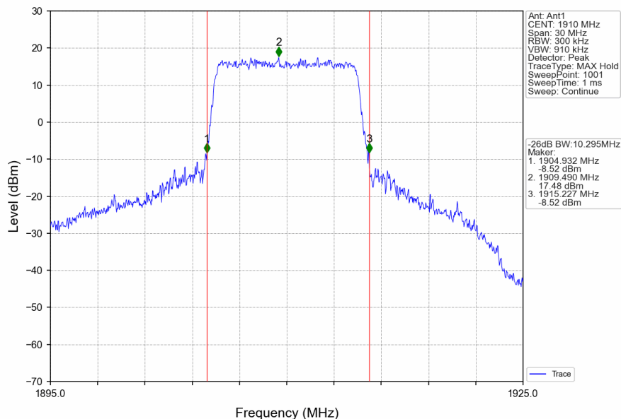
Band25_10MHz_16QAM_HCH_1910MHz_RB_50_0_NTNV
