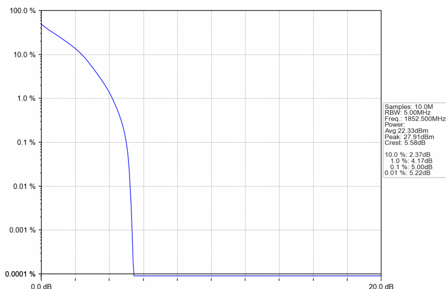
Band25_5MHz_QPSK_LCH_1852.5MHz_RB_25_0_NTNV
