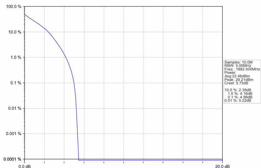
Band25_5MHz_QPSK_MCH_1882.5MHz_RB_25_0_NTNV
