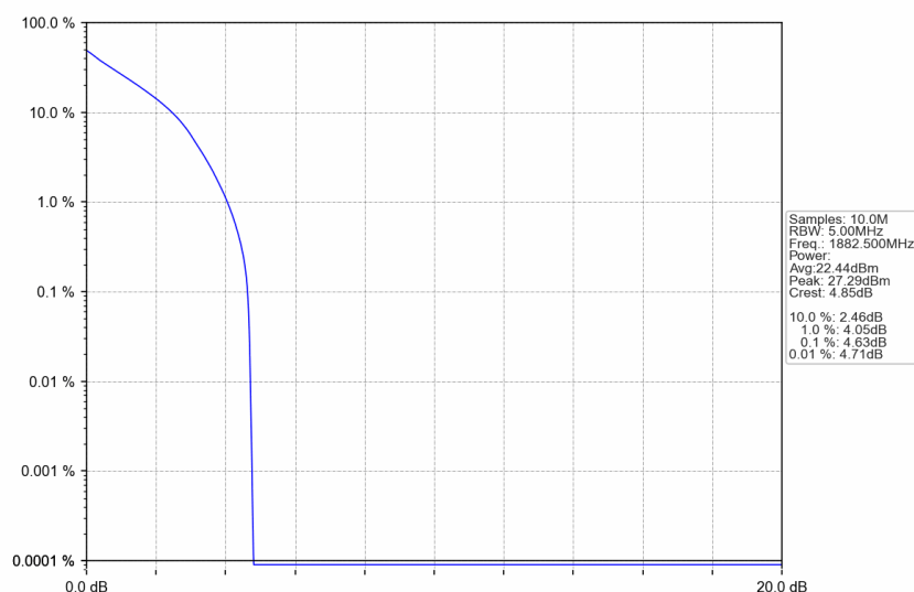
Band25_3MHz_QPSK_MCH_1882.5MHz_RB_15_0_NTNV
