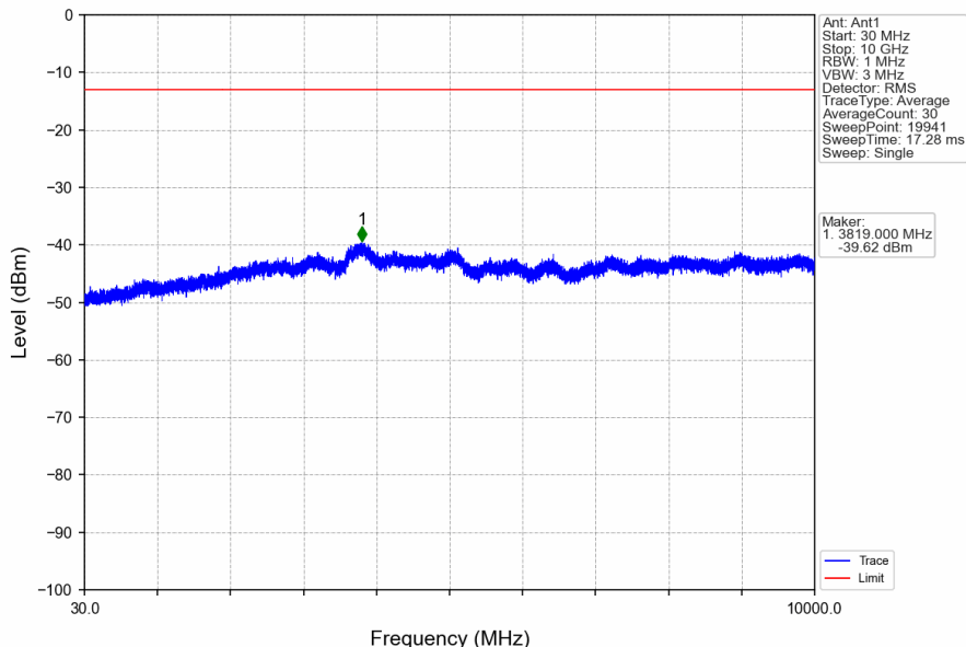
Band25_3MHz_QPSK_HCH_1913.5MHz_RB_1_0_NTNV
