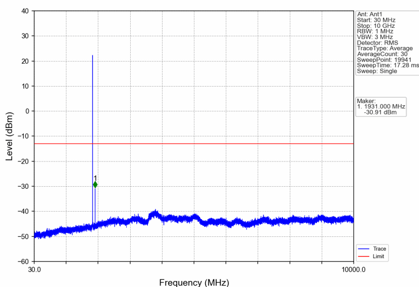
Band25_1.4MHz_QPSK_LCH_1850.7MHz_RB_1_0_NTNV
