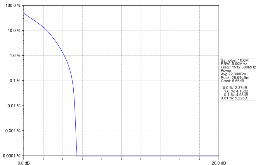
Band25_5MHz_QPSK_HCH_1912.5MHz_RB_25_0_NTNV
