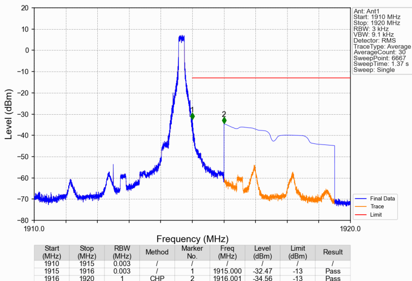
Band25_5MHz_QPSK_HCH_1912.5MHz_RB_1_24_NTNV
