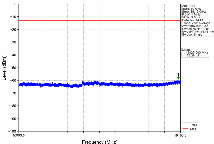
Band25_5MHz_QPSK_LCH_1852.5MHz_RB_25_0_NTNV
