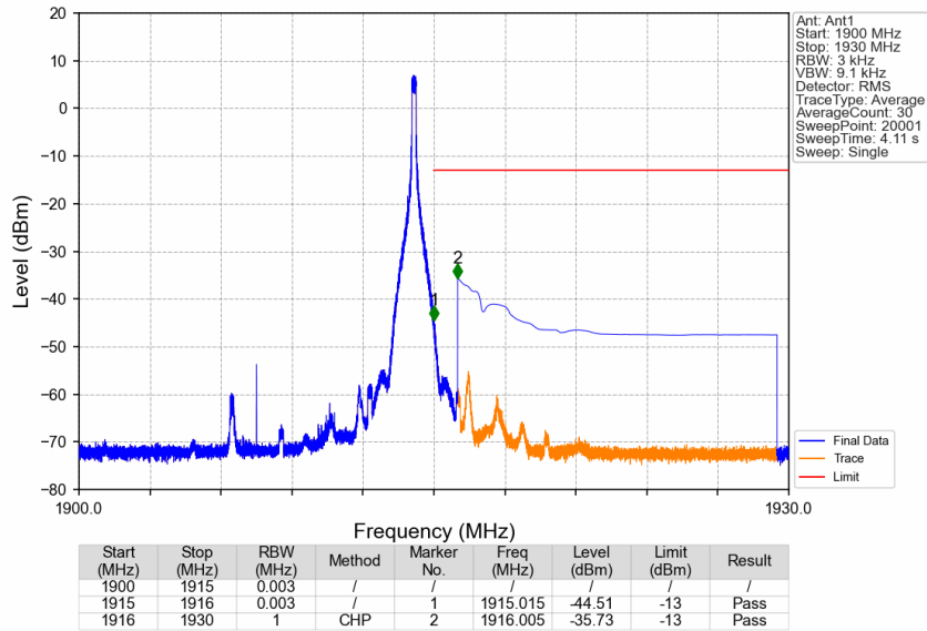
Band25_15MHz_16QAM_HCH_1907.5MHz_RB_1_74_NTNV
