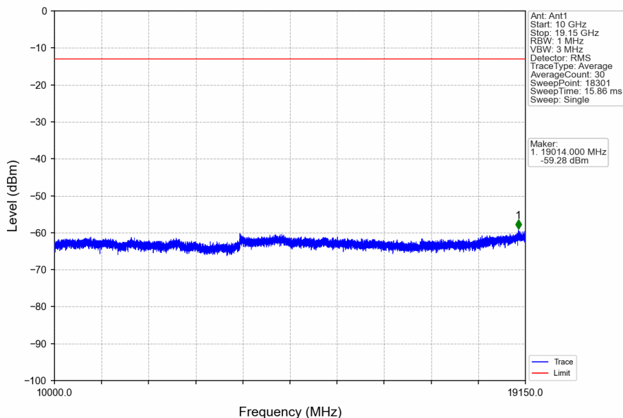
Band25_5MHz_QPSK_HCH_1912.5MHz_RB_1_0_NTNV
