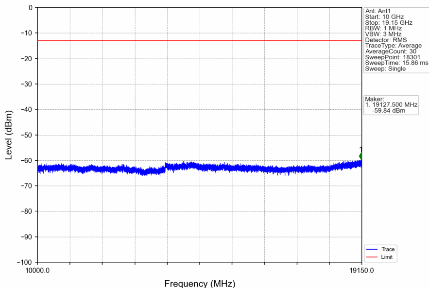
Band25_10MHz_16QAM_MCH_1882.5MHz_RB_1_0_NTNV
