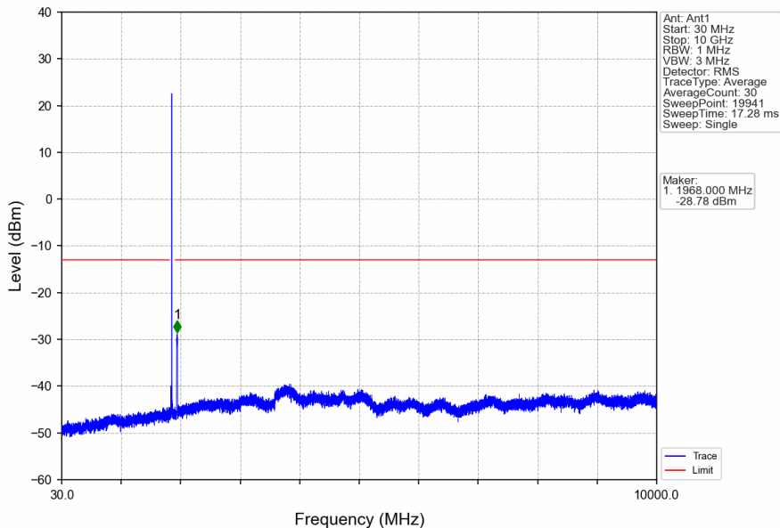
Band25_20MHz_QPSK_MCH_1882.5MHz_RB_1_0_NTNV
