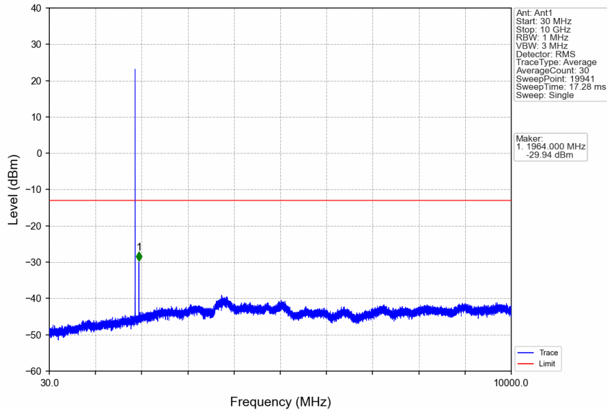
Band25_5MHz_QPSK_MCH_1882.5MHz_RB_1_0_NTNV
