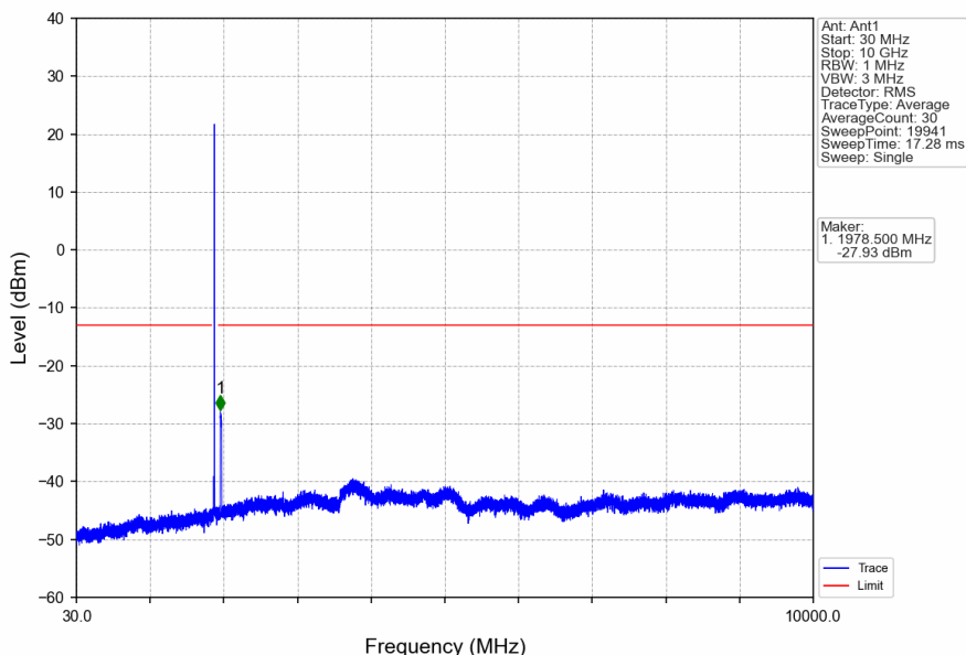
Band25_20MHz_16QAM_HCH_1905MHz_RB_1_0_NTNV
