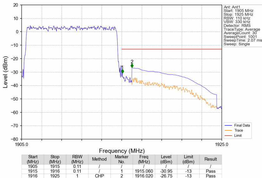
Band25_10MHz_16QAM_HCH_1910MHz_RB_50_0_NTNV
