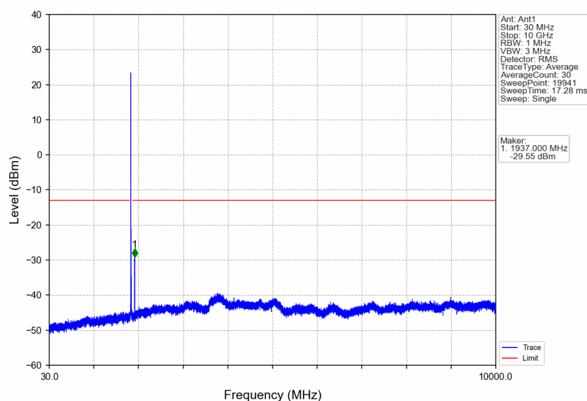
Band25_15MHz_QPSK_LCH_1857.5MHz_RB_1_0_NTNV
