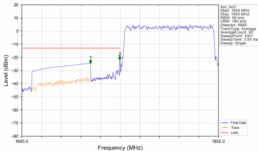
Band25_5MHz_16QAM_LCH_1852.5MHz_RB_25_0_NTNV
