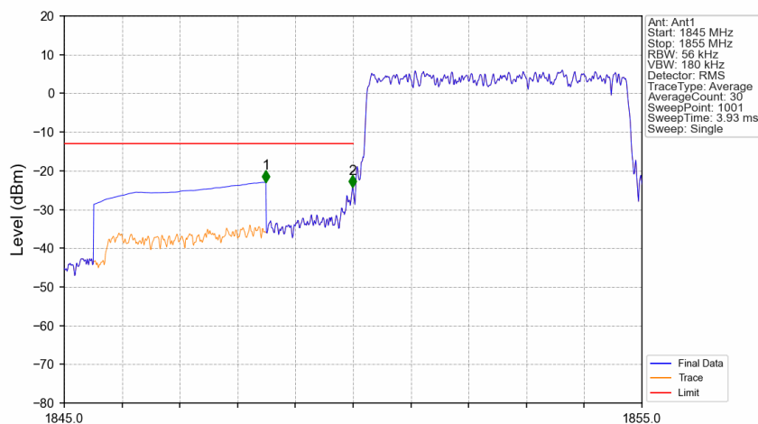
Band25_5MHz_QPSK_LCH_1852.5MHz_RB_25_0_NTNV
