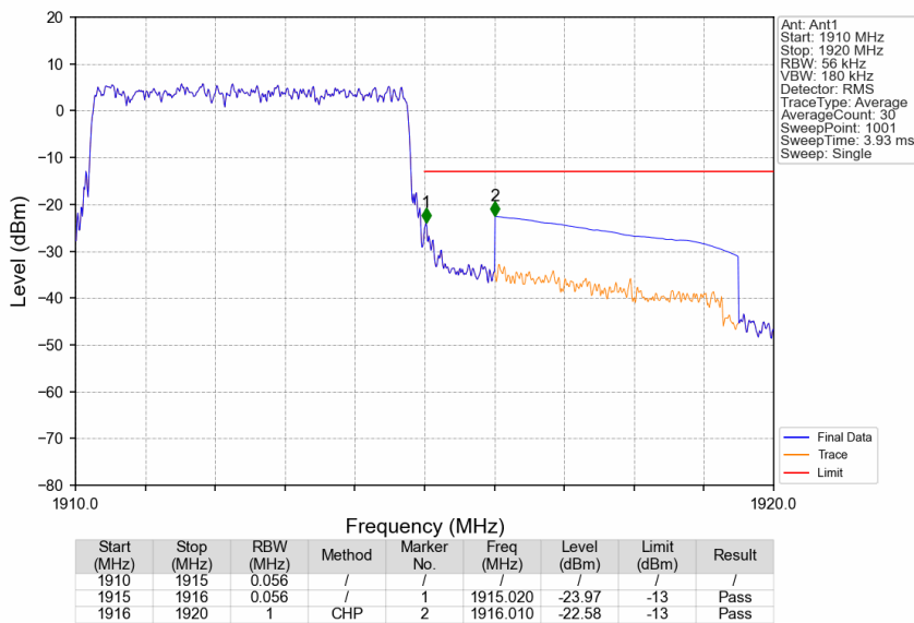
Band25_5MHz_QPSK_HCH_1912.5MHz_RB_25_0_NTNV
