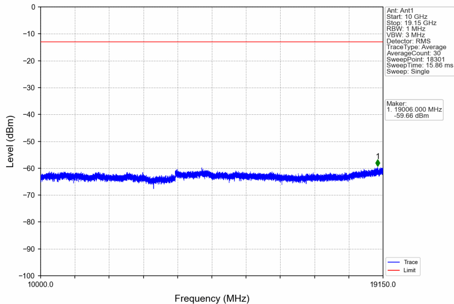
Band25_5MHz_QPSK_MCH_1882.5MHz_RB_1_0_NTNV
