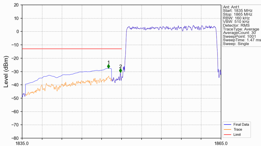
Band25_15MHz_16QAM_LCH_1857.5MHz_RB_75_0_NTNV
