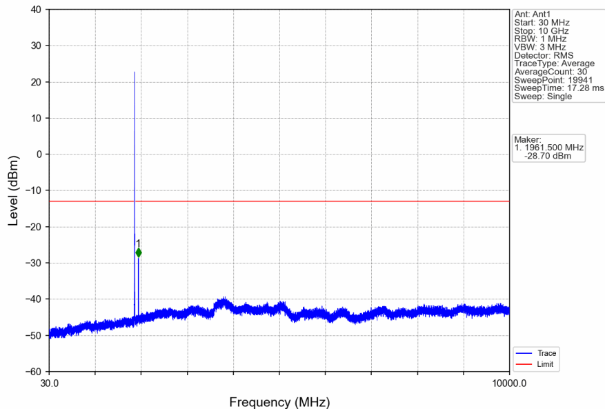
Band25_10MHz_QPSK_MCH_1882.5MHz_RB_1_0_NTNV
