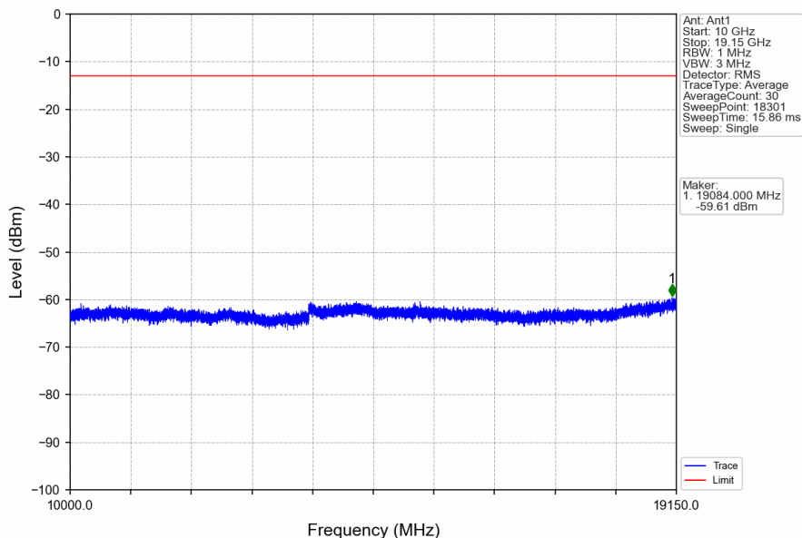
Band25_5MHz_16QAM_HCH_1912.5MHz_RB_1_0_NTNV
