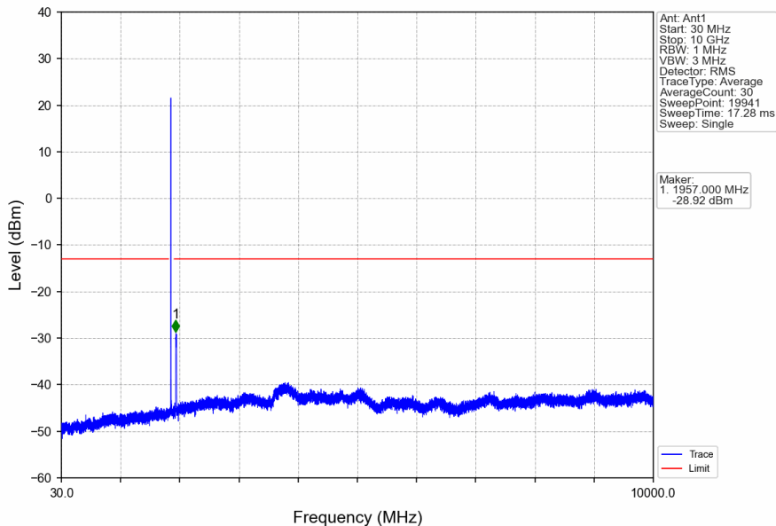
Band25_20MHz_16QAM_MCH_1882.5MHz_RB_1_0_NTNV
