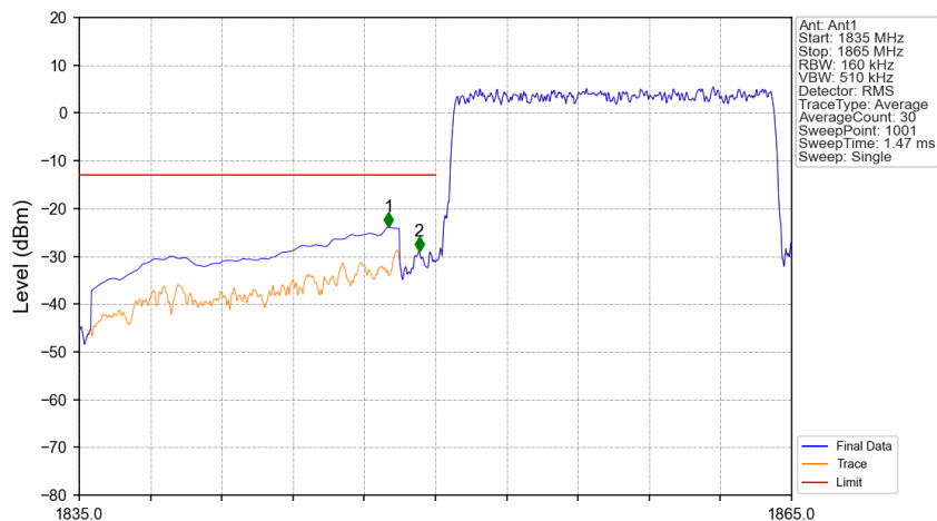
Band25_15MHz_QPSK_LCH_1857.5MHz_RB_75_0_NTNV
