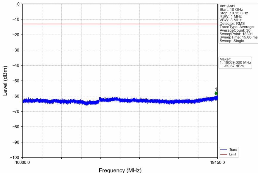
Band25_20MHz_QPSK_MCH_1882.5MHz_RB_1_0_NTNV
