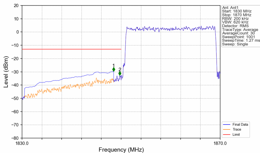
Band25_20MHz_16QAM_LCH_1860MHz_RB_100_0_NTNV
