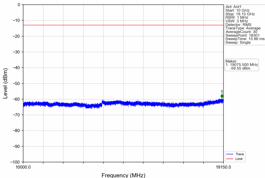
Band25_15MHz_16QAM_HCH_1907.5MHz_RB_1_0_NTNV
