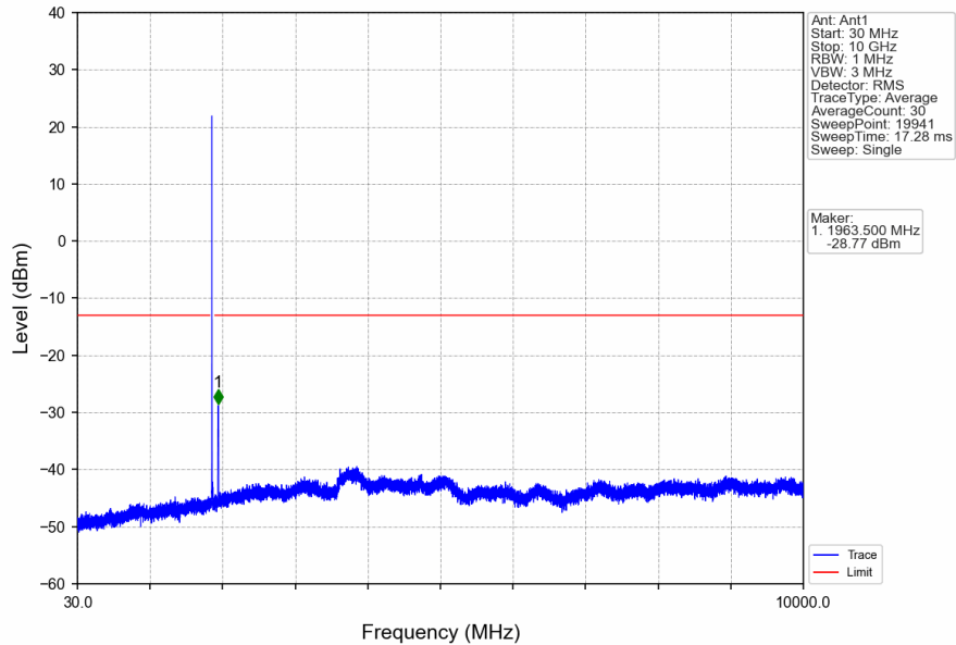
Band25_15MHz_16QAM_MCH_1882.5MHz_RB_1_0_NTNV
