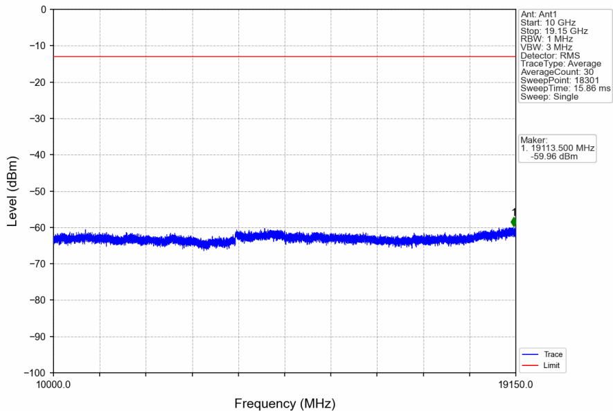
Band25_15MHz_16QAM_MCH_1882.5MHz_RB_1_0_NTNV
