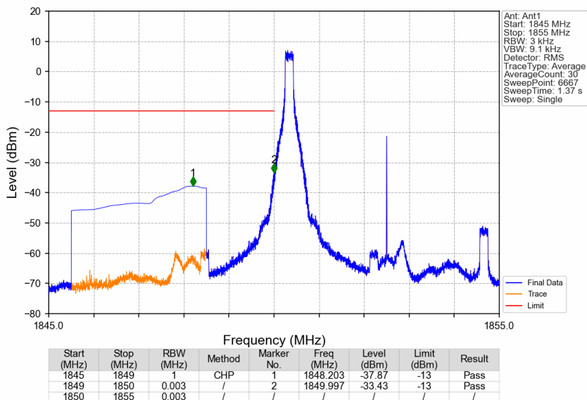
Band25_5MHz_16QAM_LCH_1852.5MHz_RB_1_0_NTNV
