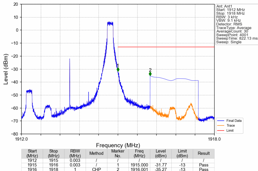
Band25_3MHz_16QAM_HCH_1913.5MHz_RB_1_14_NTNV
