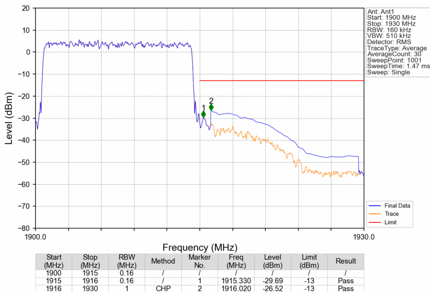
Band25_15MHz_QPSK_HCH_1907.5MHz_RB_75_0_NTNV
