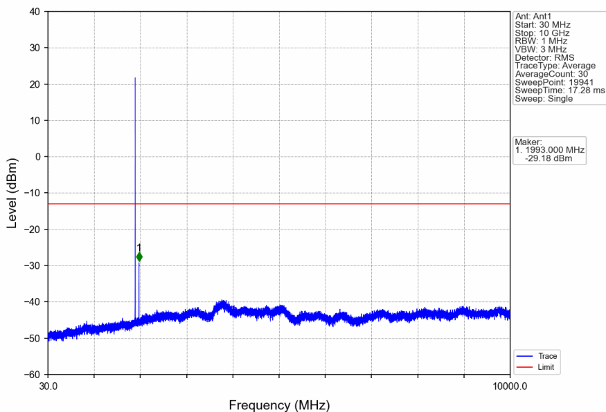
Band25_5MHz_16QAM_HCH_1912.5MHz_RB_1_0_NTNV
