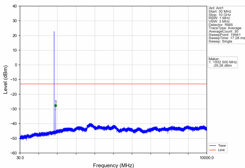
Band25_5MHz_QPSK_LCH_1852.5MHz_RB_1_0_NTNV
