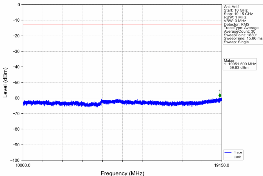
Band25_20MHz_16QAM_HCH_1905MHz_RB_1_0_NTNV
