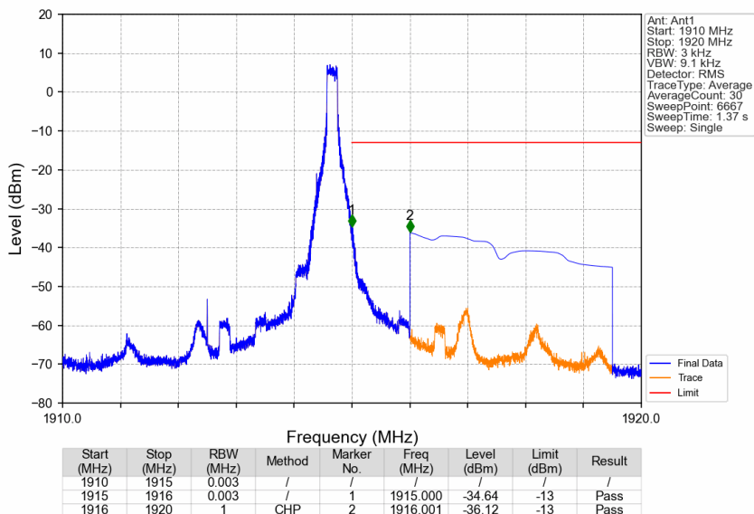
Band25_5MHz_16QAM_HCH_1912.5MHz_RB_1_24_NTNV
