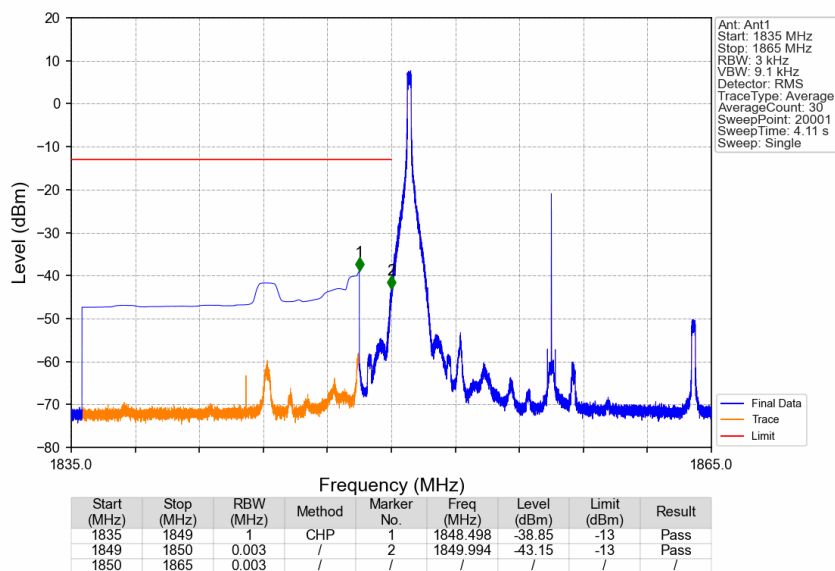
Band25_15MHz_QPSK_LCH_1857.5MHz_RB_1_0_NTNV
