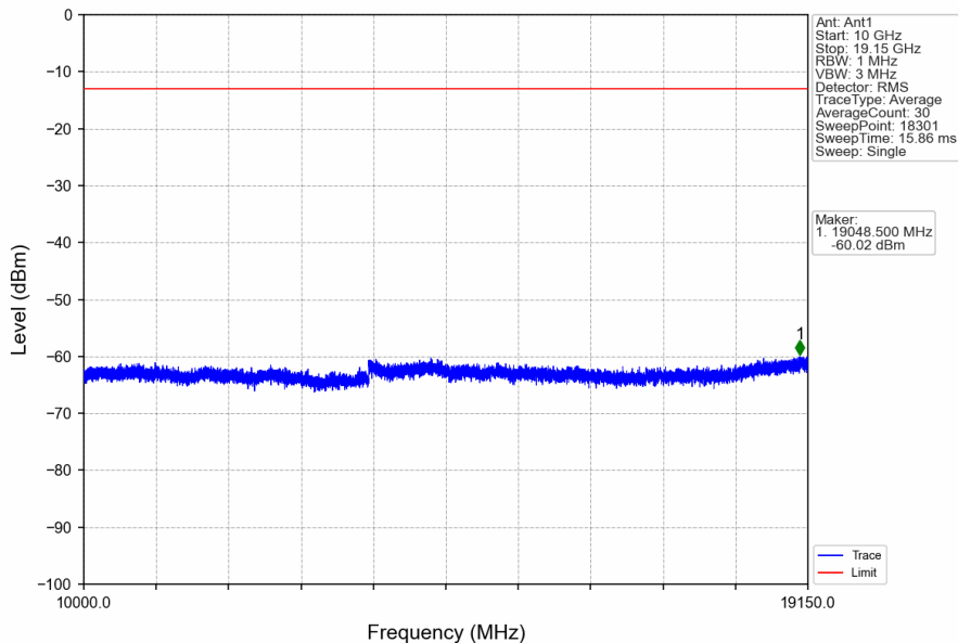
Band25_5MHz_16QAM_LCH_1852.5MHz_RB_25_0_NTNV
