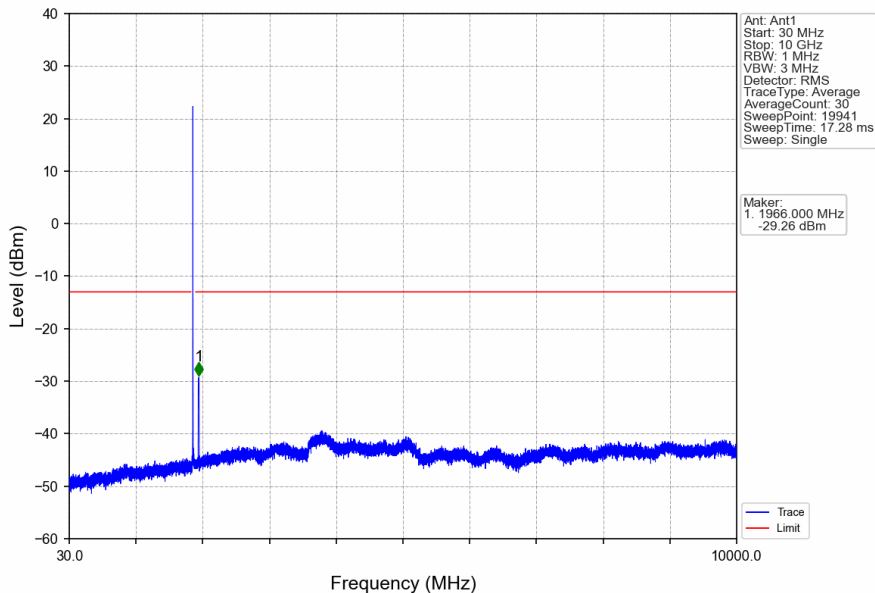
Band25_15MHz_QPSK_MCH_1882.5MHz_RB_1_0_NTNV
