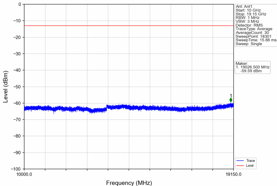
Band25_15MHz_16QAM_LCH_1857.5MHz_RB_75_0_NTNV
