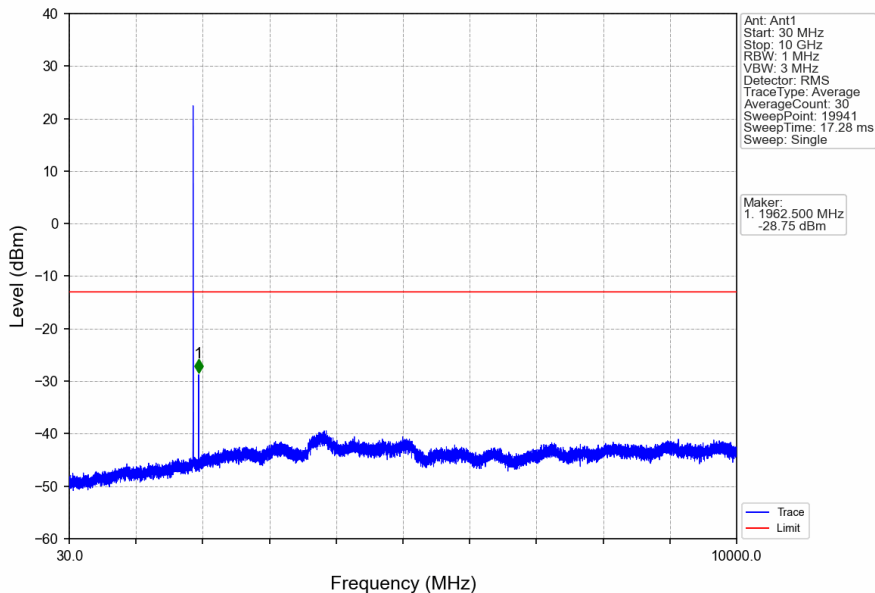
Band25_5MHz_16QAM_MCH_1882.5MHz_RB_1_0_NTNV
