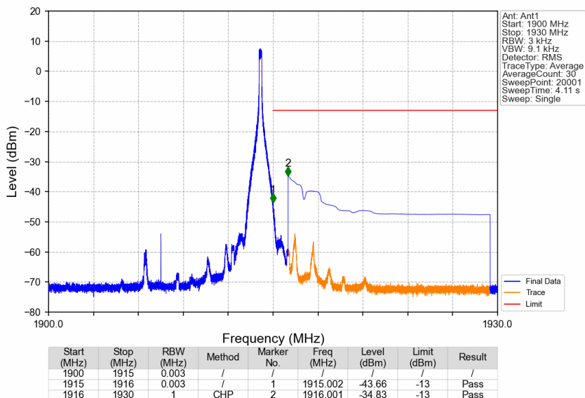
Band25_15MHz_QPSK_HCH_1907.5MHz_RB_1_74_NTNV
