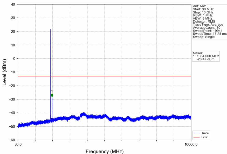
Band25_15MHz_16QAM_HCH_1907.5MHz_RB_1_0_NTNV
