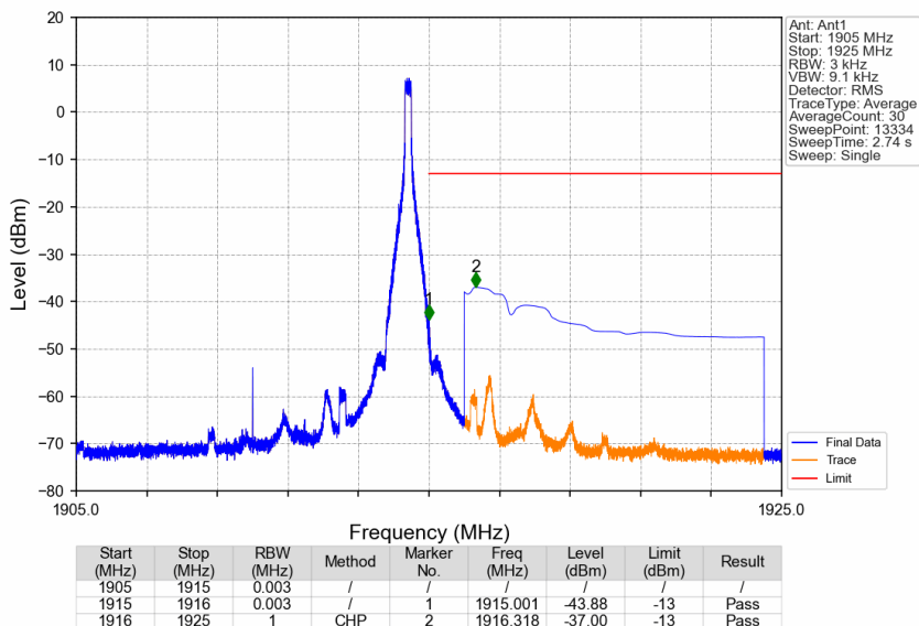
Band25_10MHz_16QAM_HCH_1910MHz_RB_1_49_NTNV
