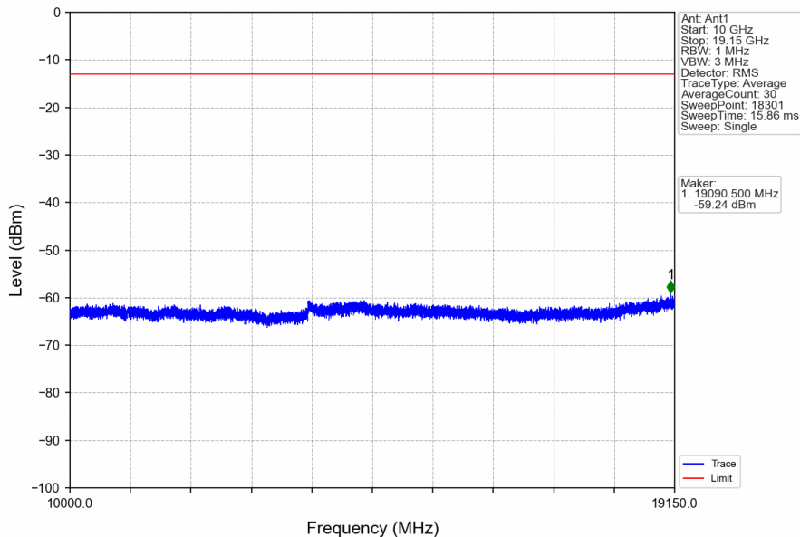
Band25_15MHz_QPSK_LCH_1857.5MHz_RB_75_0_NTNV
