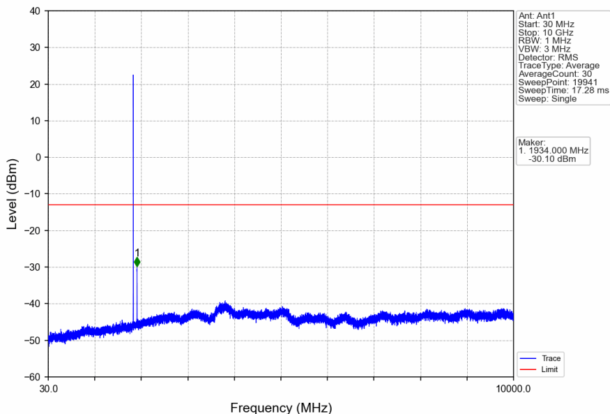
Band25_5MHz_16QAM_LCH_1852.5MHz_RB_1_0_NTNV
