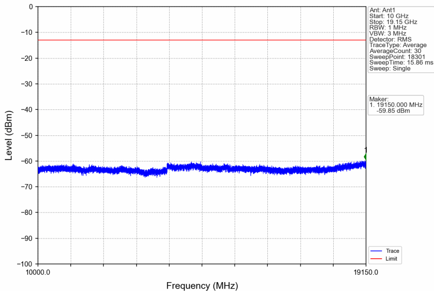
Band25_10MHz_QPSK_MCH_1882.5MHz_RB_1_0_NTNV
