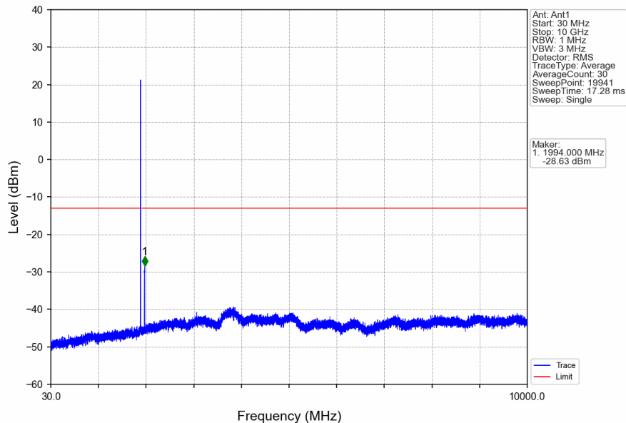
Band25_10MHz_16QAM_HCH_1910MHz_RB_1_0_NTNV
