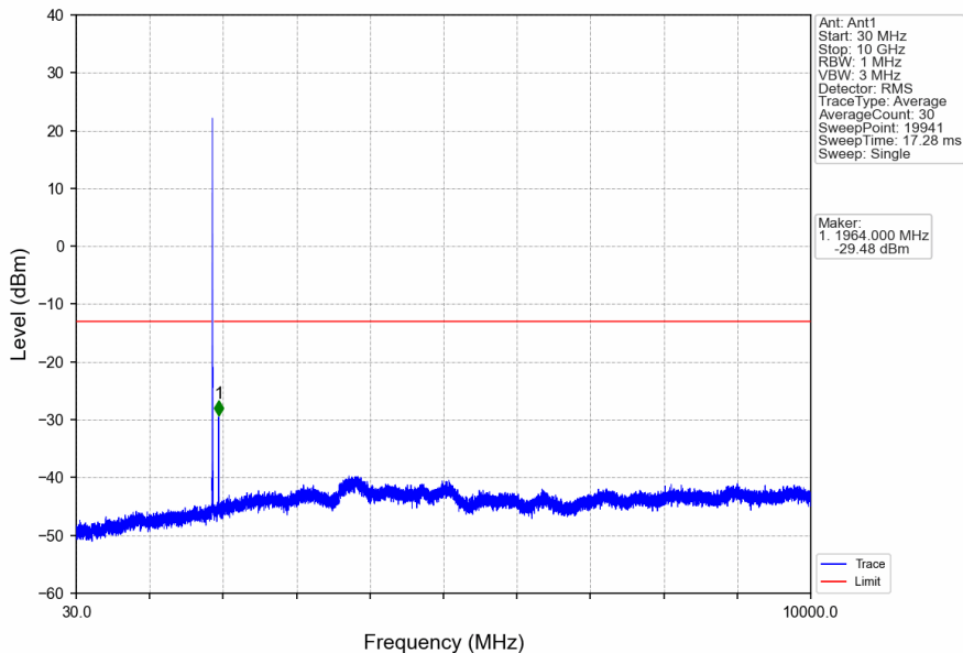
Band25_10MHz_16QAM_MCH_1882.5MHz_RB_1_0_NTNV
