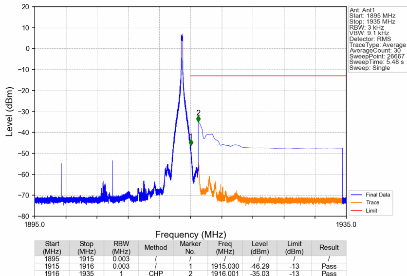
Band25_20MHz_16QAM_HCH_1905MHz_RB_1_99_NTNV
