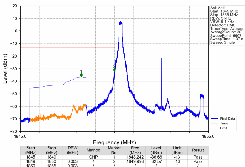
Band25_5MHz_QPSK_LCH_1852.5MHz_RB_1_0_NTNV
