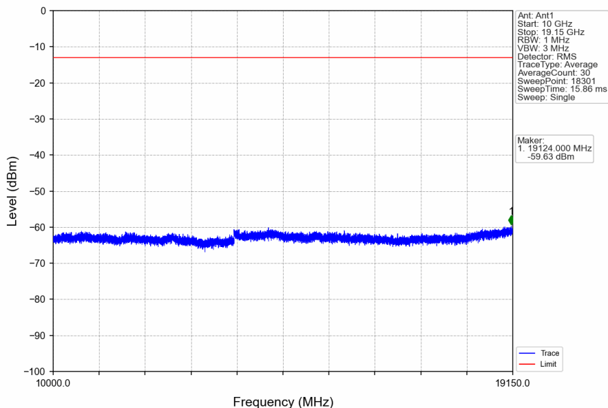
Band25_15MHz_QPSK_HCH_1907.5MHz_RB_1_0_NTNV
