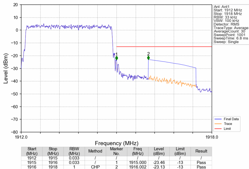
Band25_3MHz_16QAM_HCH_1913.5MHz_RB_15_0_NTNV
