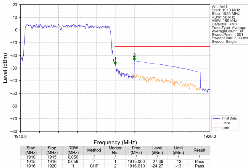
Band25_5MHz_16QAM_HCH_1912.5MHz_RB_25_0_NTNV
