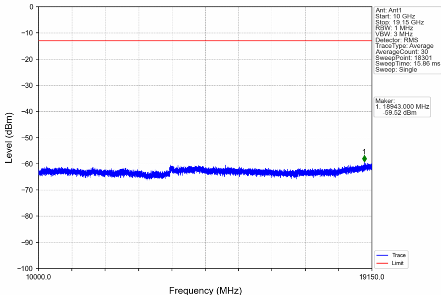
Band25_10MHz_16QAM_HCH_1910MHz_RB_1_0_NTNV
