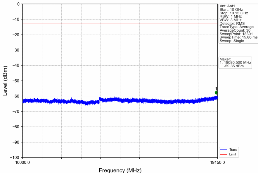
Band25_5MHz_16QAM_MCH_1882.5MHz_RB_1_0_NTNV
