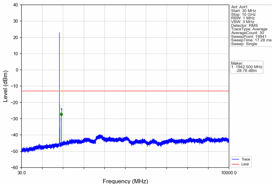
Band25_15MHz_16QAM_LCH_1857.5MHz_RB_1_0_NTNV
