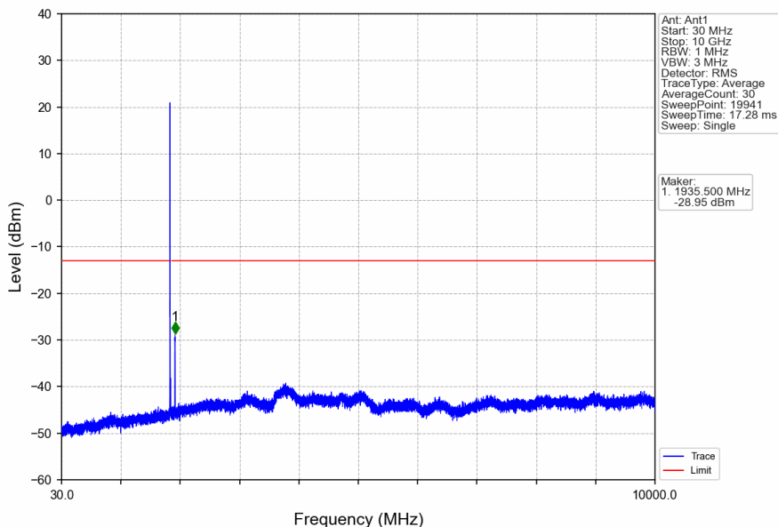
Band25_10MHz_16QAM_LCH_1855MHz_RB_1_0_NTNV
