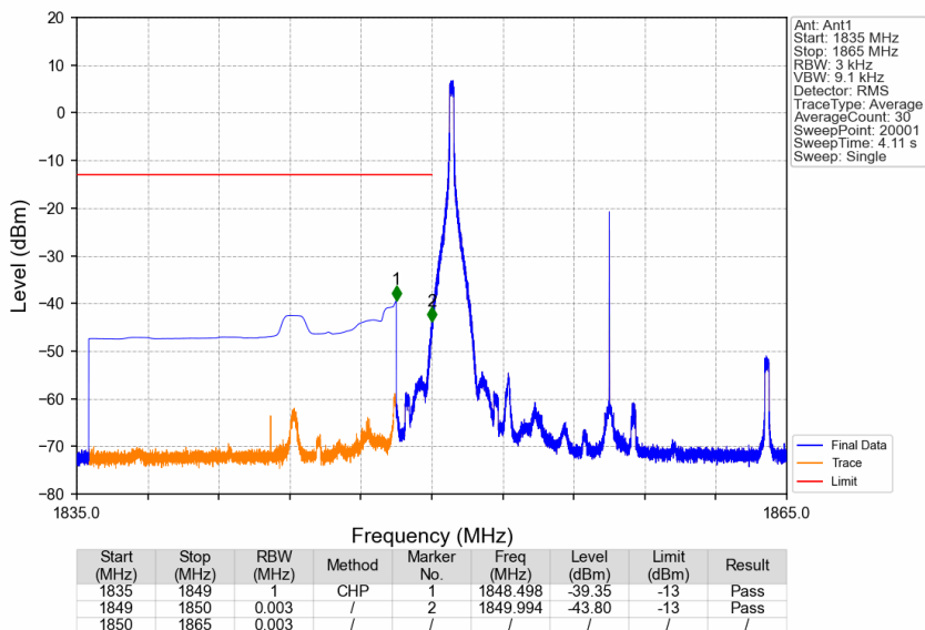
Band25_15MHz_16QAM_LCH_1857.5MHz_RB_1_0_NTNV
