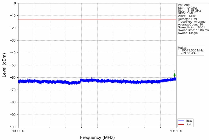
Band25_20MHz_16QAM_MCH_1882.5MHz_RB_1_0_NTNV
