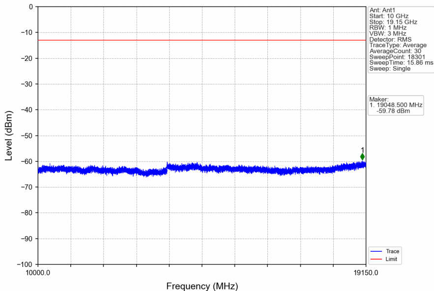
Band25_10MHz_16QAM_LCH_1855MHz_RB_50_0_NTNV
