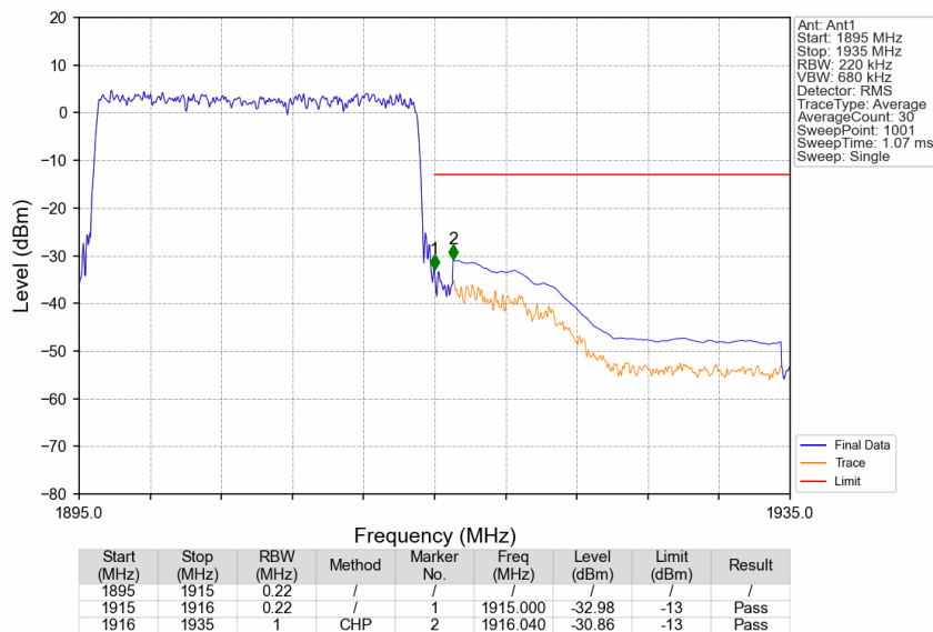
Band25_20MHz_16QAM_HCH_1905MHz_RB_100_0_NTNV
