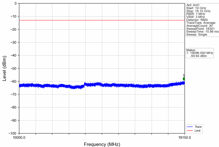
Band25_15MHz_QPSK_MCH_1882.5MHz_RB_1_0_NTNV
