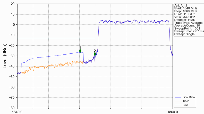
Band25_10MHz_16QAM_LCH_1855MHz_RB_50_0_NTNV
