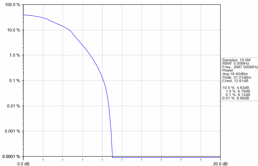
Band41_5MHz_16QAM_HCH_2687.5MHz_RB_25_0_NTNV
