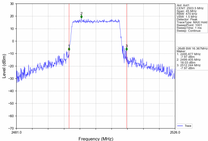
Band41_15MHz_16QAM_LCH_2503.5MHz_RB_75_0_NTNV
