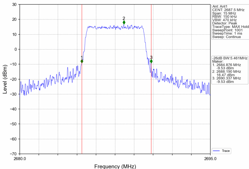
Band41_5MHz_16QAM_HCH_2687.5MHz_RB_25_0_NTNV
