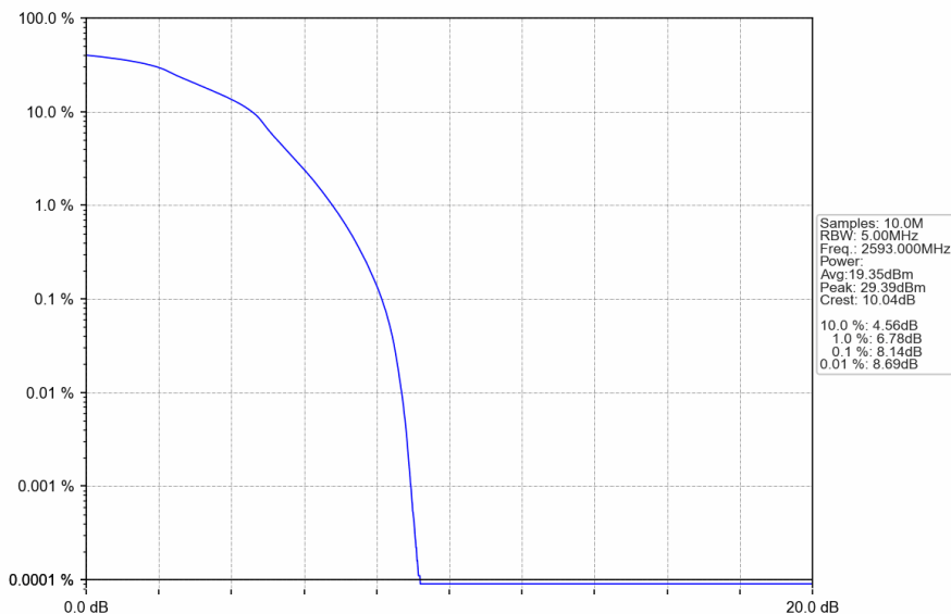
Band41_5MHz_16QAM_MCH_2593MHz_RB_25_0_NTNV
