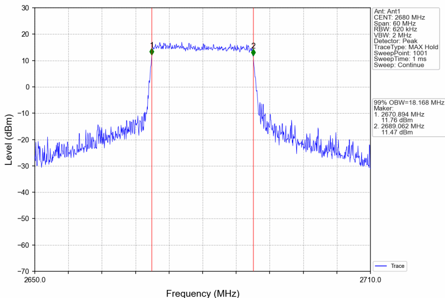
Band41_20MHz_16QAM_HCH_2680MHz_RB_100_0_NTNV
