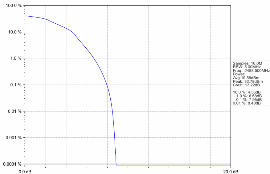
Band41_5MHz_16QAM_LCH_2498.5MHz_RB_25_0_NTNV
