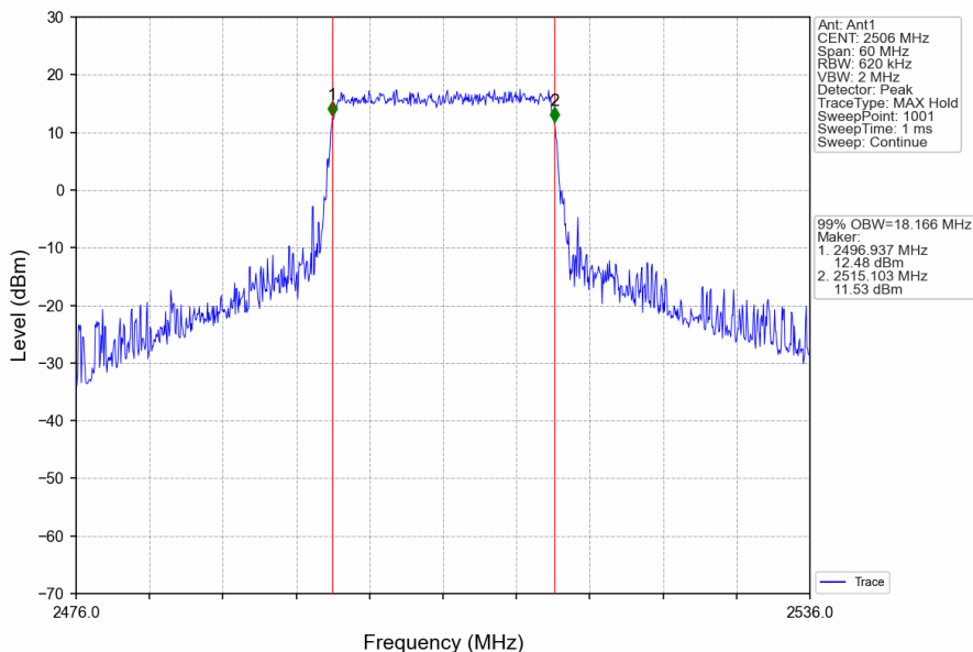
Band41_20MHz_16QAM_LCH_2506MHz_RB_100_0_NTNV
