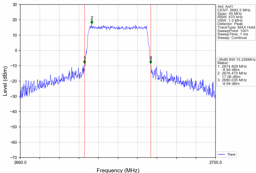
Band41_15MHz_16QAM_HCH_2682.5MHz_RB_75_0_NTNV
