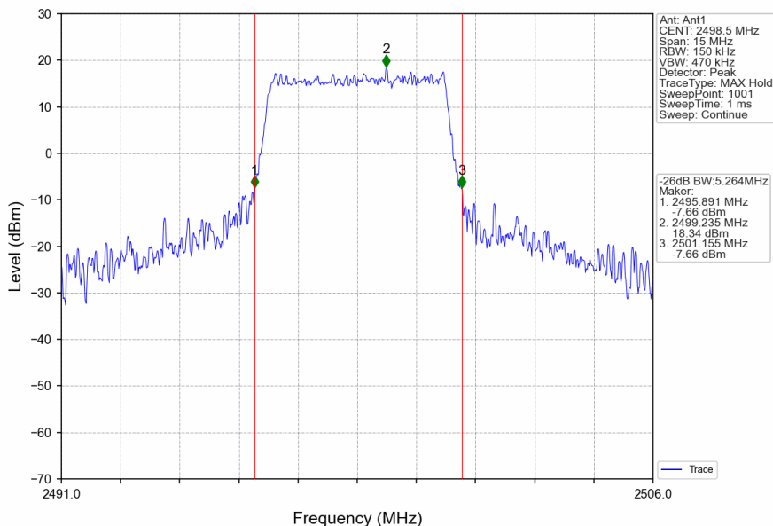
Band41_5MHz_16QAM_LCH_2498.5MHz_RB_25_0_NTNV
