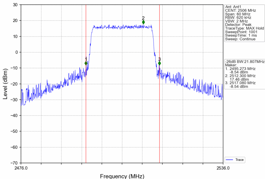
Band41_20MHz_16QAM_LCH_2506MHz_RB_100_0_NTNV
