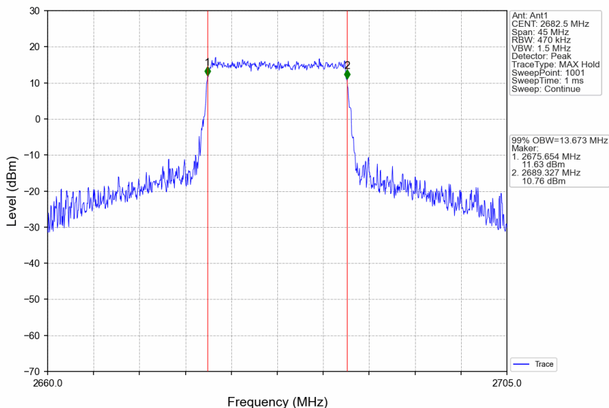
Band41_15MHz_16QAM_HCH_2682.5MHz_RB_75_0_NTNV
