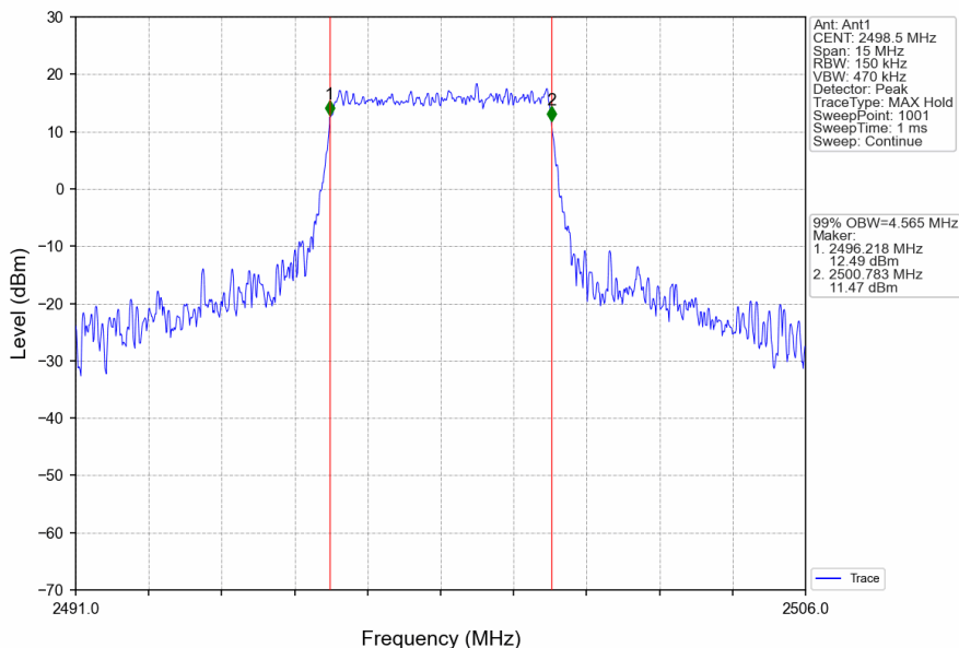
Band41_5MHz_16QAM_LCH_2498.5MHz_RB_25_0_NTNV
