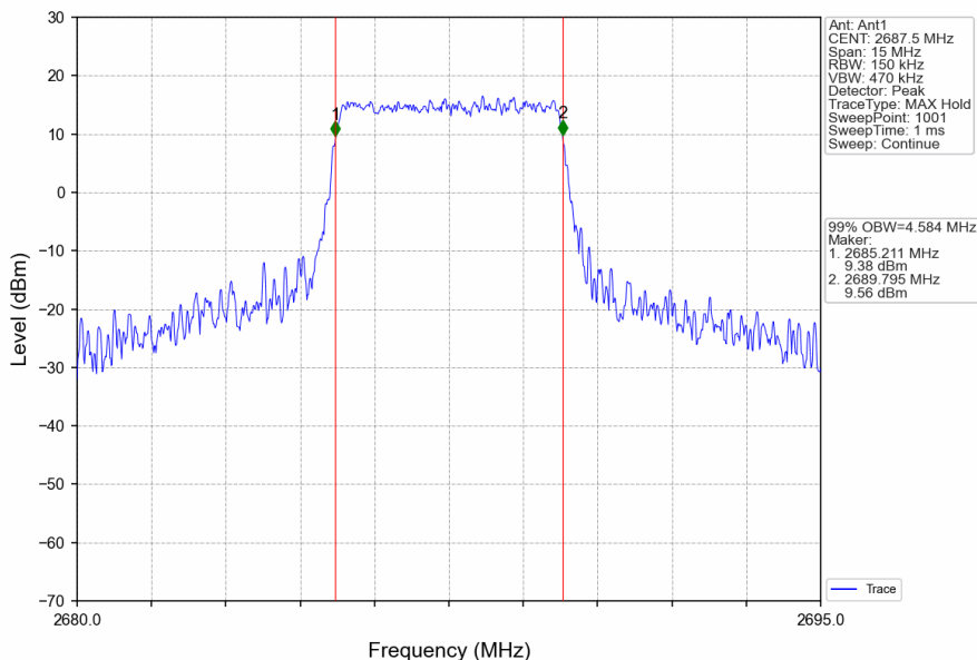
Band41_5MHz_16QAM_HCH_2687.5MHz_RB_25_0_NTNV
