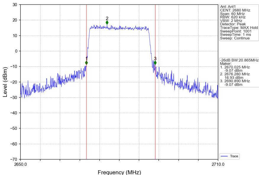
Band41_20MHz_16QAM_HCH_2680MHz_RB_100_0_NTNV
