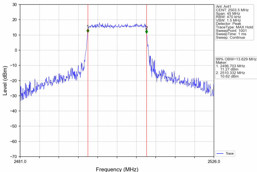
Band41_15MHz_16QAM_LCH_2503.5MHz_RB_75_0_NTNV
