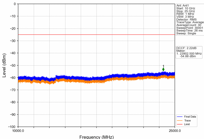
Band41_5MHz_16QAM_HCH_2687.5MHz_RB_1_0_NTNV
