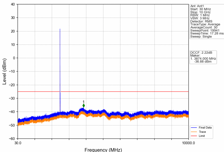
Band41_15MHz_16QAM_LCH_2503.5MHz_RB_1_0_NTNV
