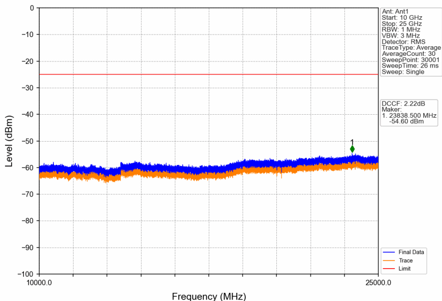
Band41_15MHz_16QAM_MCH_2593MHz_RB_1_0_NTNV
