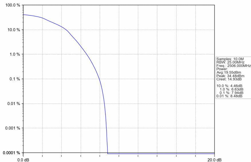
Band41_20MHz_16QAM_LCH_2506MHz_RB_100_0_NTNV
