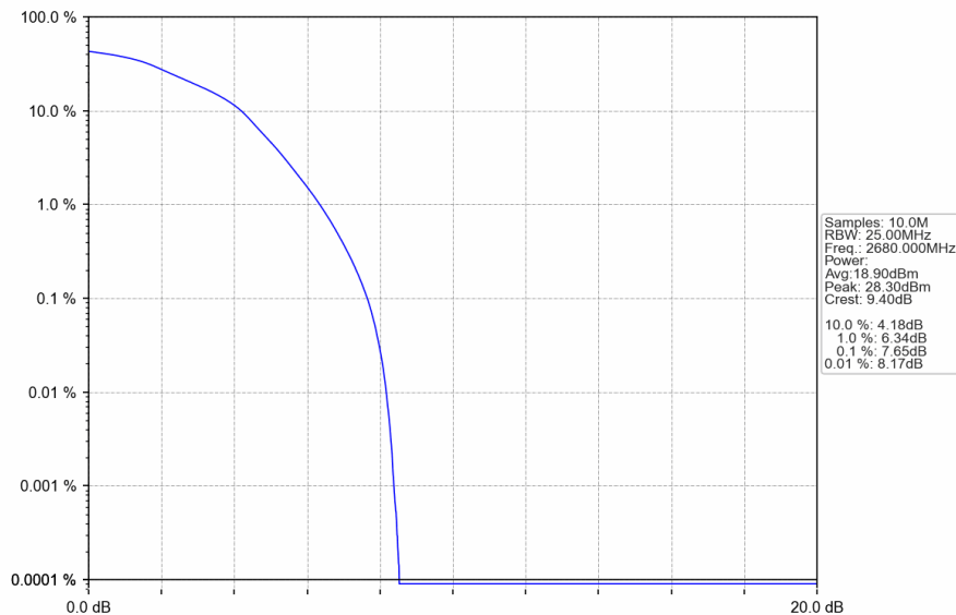
Band41_20MHz_16QAM_HCH_2680MHz_RB_100_0_NTNV
