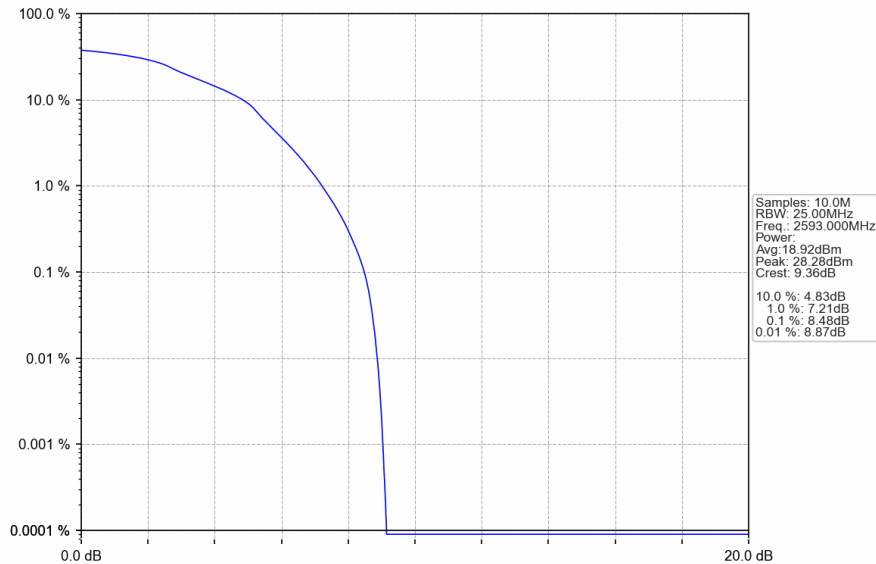
Band41_15MHz_16QAM_MCH_2593MHz_RB_75_0_NTNV
