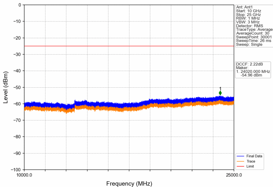
Band41_5MHz_16QAM_LCH_2498.5MHz_RB_1_0_NTNV
