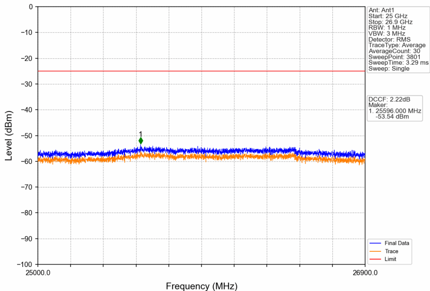
Band41_5MHz_16QAM_HCH_2687.5MHz_RB_1_0_NTNV
