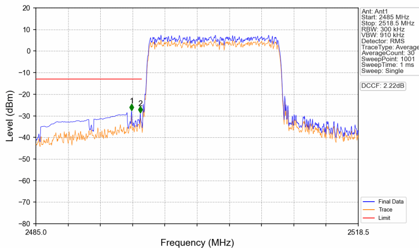
Band41_15MHz_16QAM_LCH_2503.5MHz_RB_75_0_NTNV
