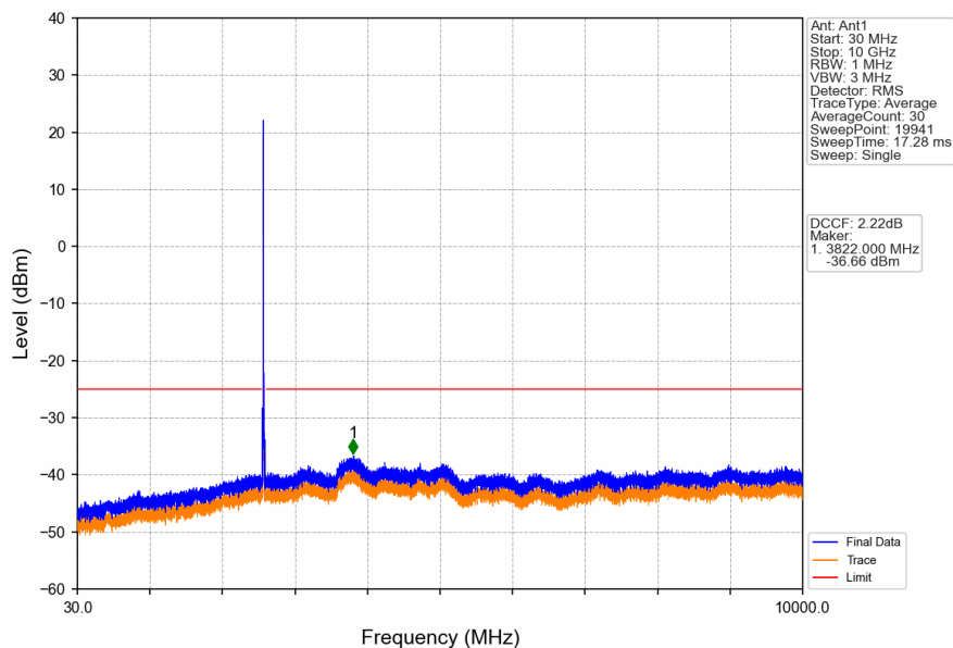
Band41_15MHz_16QAM_MCH_2593MHz_RB_1_0_NTNV
