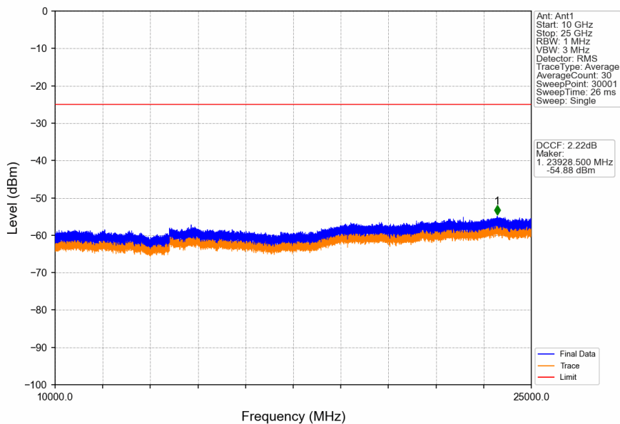
Band41_5MHz_16QAM_MCH_2593MHz_RB_1_0_NTNV
