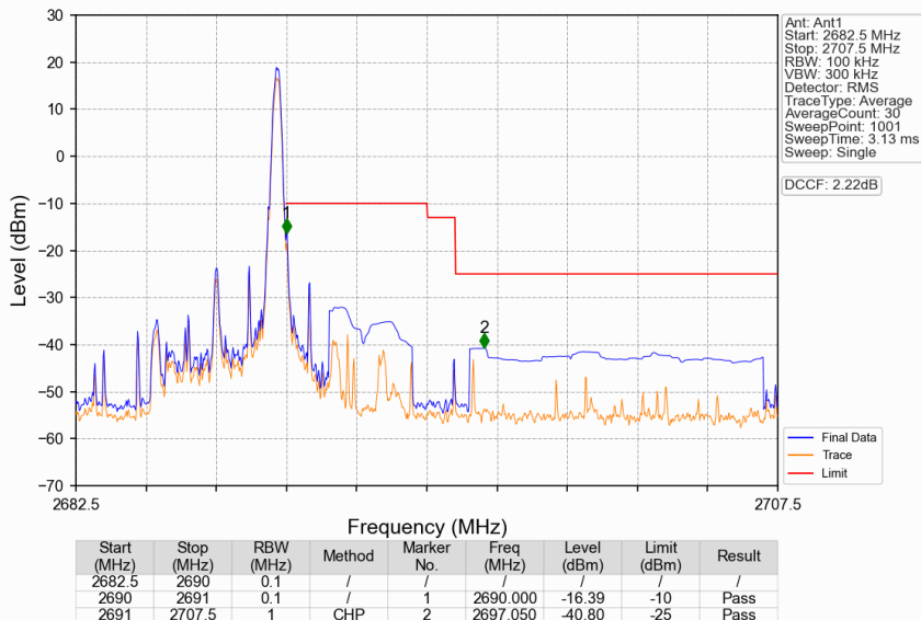
Band41_5MHz_16QAM_HCH_2687.5MHz_RB_1_24_NTNV
