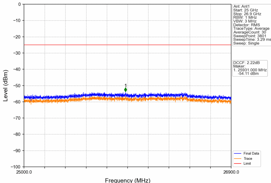
Band41_15MHz_16QAM_LCH_2503.5MHz_RB_75_0_NTNV
