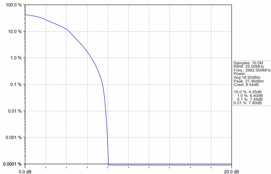
Band41_15MHz_16QAM_HCH_2682.5MHz_RB_75_0_NTNV
