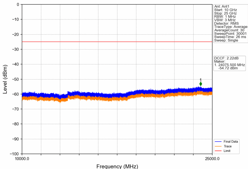
Band41_15MHz_16QAM_LCH_2503.5MHz_RB_1_0_NTNV
