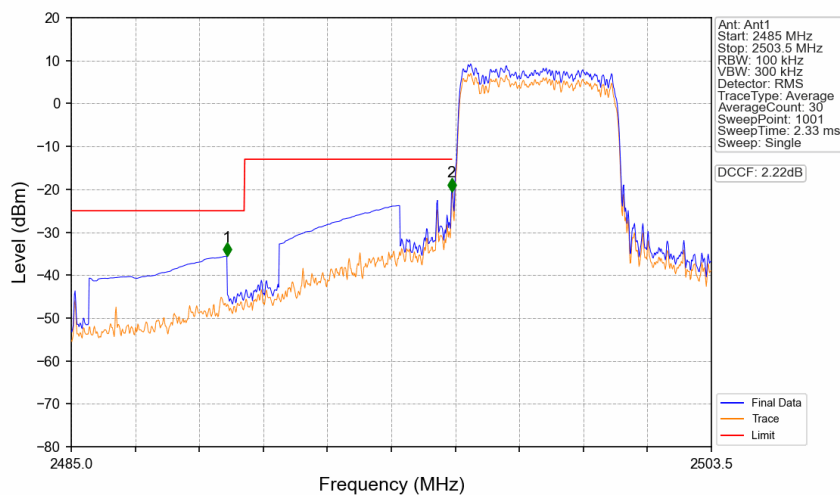
Band41_5MHz_16QAM_LCH_2498.5MHz_RB_25_0_NTNV
