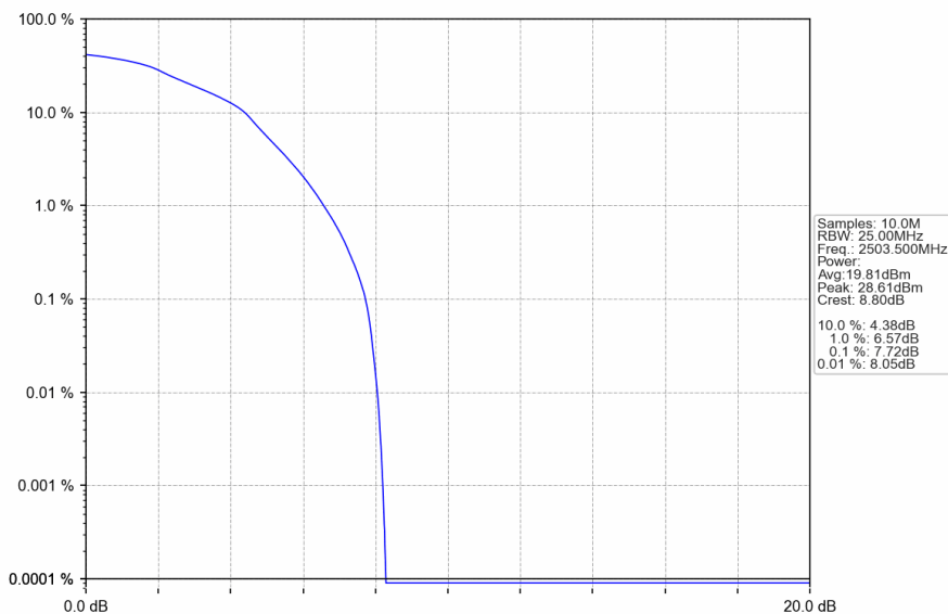
Band41_15MHz_16QAM_LCH_2503.5MHz_RB_75_0_NTNV
