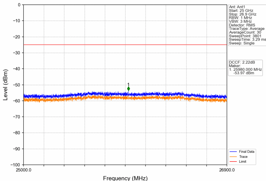
Band41_5MHz_16QAM_HCH_2687.5MHz_RB_1_0_NTNV
