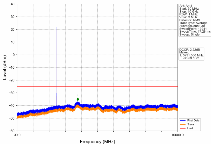
Band41_5MHz_16QAM_LCH_2498.5MHz_RB_1_0_NTNV
