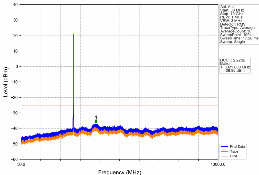
Band41_15MHz_16QAM_HCH_2682.5MHz_RB_1_0_NTNV
