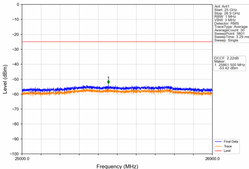
Band41_20MHz_16QAM_HCH_2680MHz_RB_1_0_NTNV
