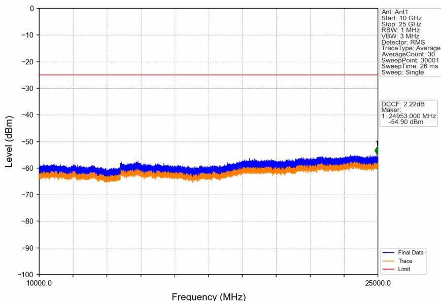
Band41_20MHz_16QAM_HCH_2680MHz_RB_1_0_NTNV
