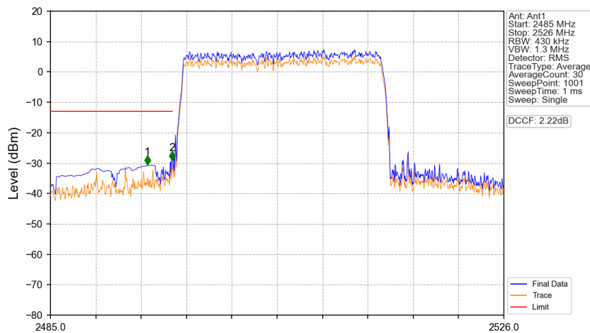
Band41_20MHz_16QAM_LCH_2506MHz_RB_100_0_NTNV
