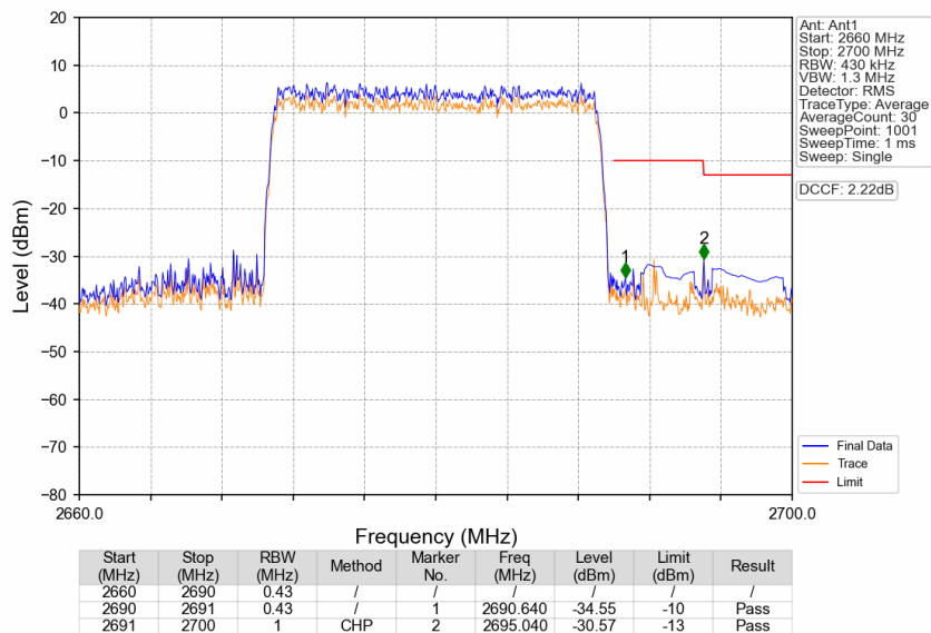
Band41_20MHz_16QAM_HCH_2680MHz_RB_100_0_NTNV
