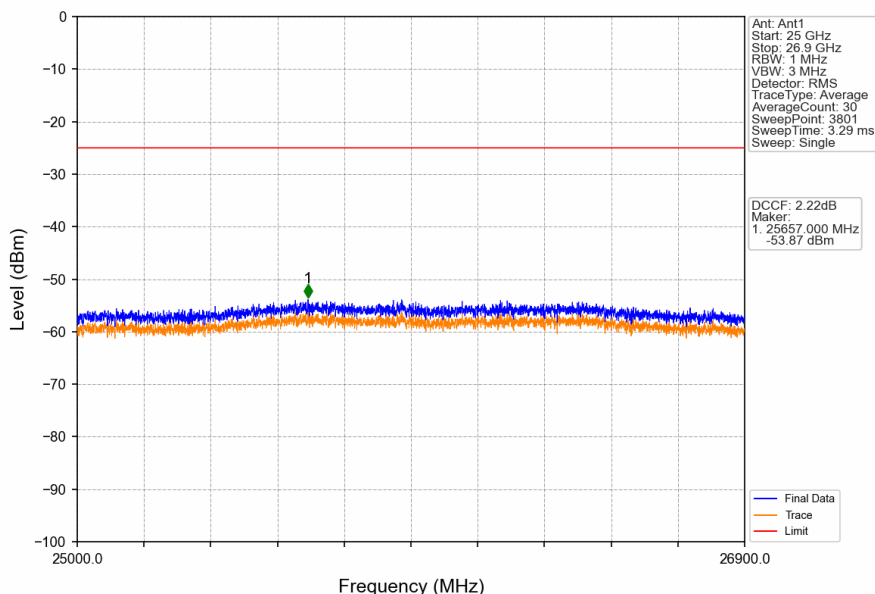
Band41_20MHz_16QAM_HCH_2680MHz_RB_1_0_NTNV
