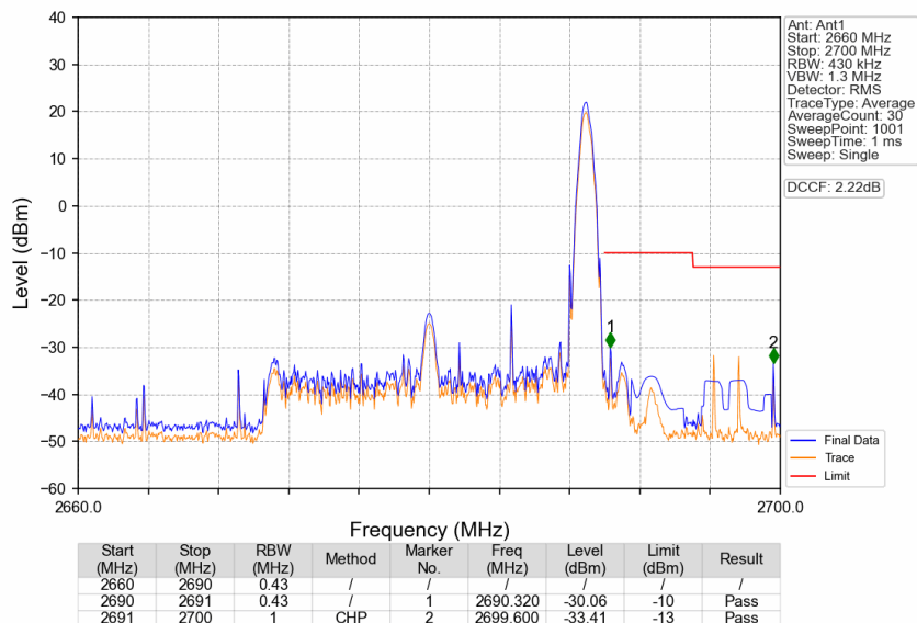
Band41_20MHz_16QAM_HCH_2680MHz_RB_1_99_NTNV
