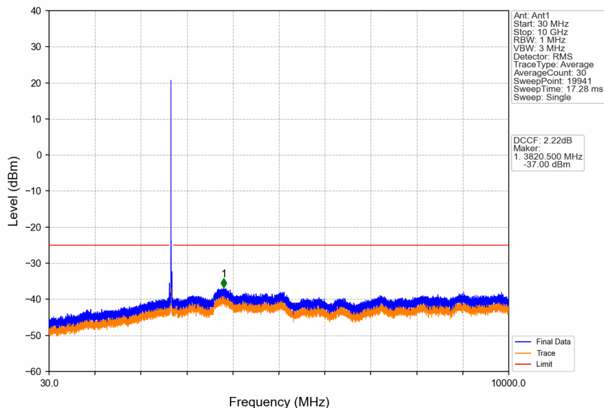
Band41_20MHz_16QAM_HCH_2680MHz_RB_1_0_NTNV
