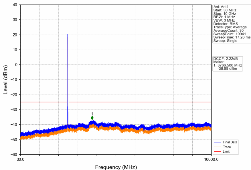
Band41_20MHz_16QAM_LCH_2506MHz_RB_1_0_NTNV
