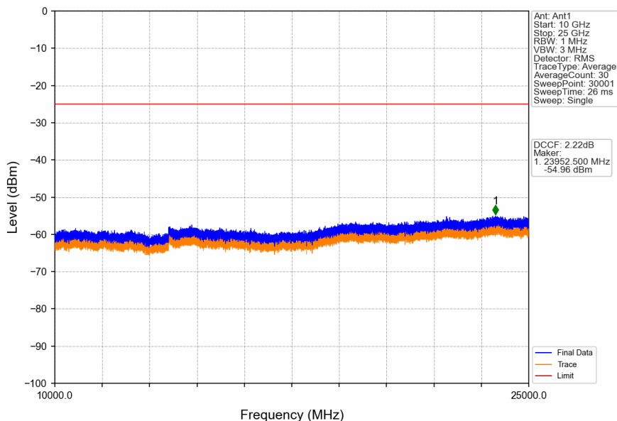
Band41_20MHz_16QAM_LCH_2506MHz_RB_1_0_NTNV
