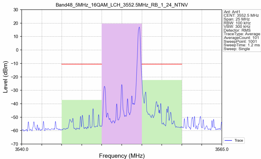
Band48_5MHz_16QAM_LCH_3552.5MHz_RB_1_24_NTNV
