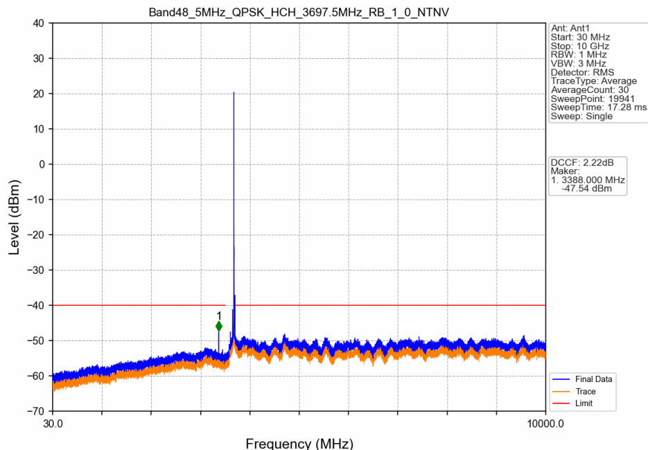
Band48_5MHz_QPSK_HCH_3697.5MHz_RB_1_0_NTNV
