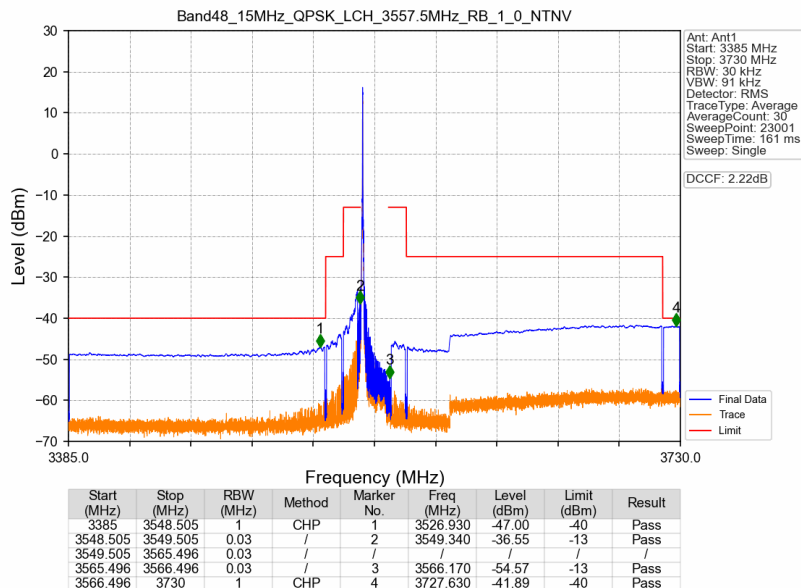
Band48_15MHz_QPSK_LCH_3557.5MHz_RB_1_0_NTNV
