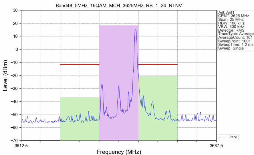
Band48_5MHz_16QAM_MCH_3625MHz_RB_1_24_NTNV
