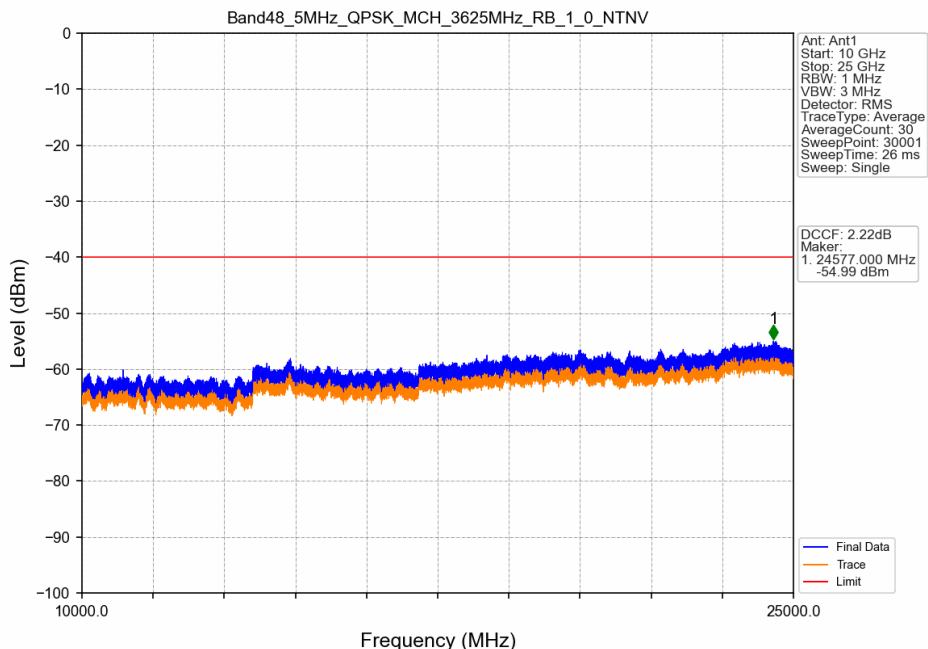
Band48_5MHz_QPSK_MCH_3625MHz_RB_1_0_NTNV
