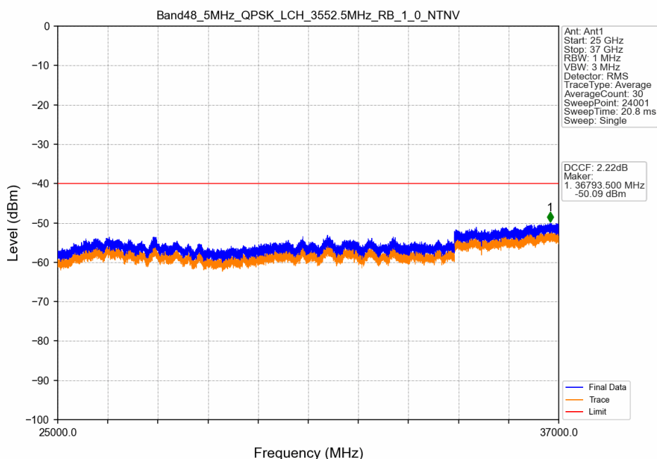
Band48_5MHz_QPSK_LCH_3552.5MHz_RB_1_0_NTNV
