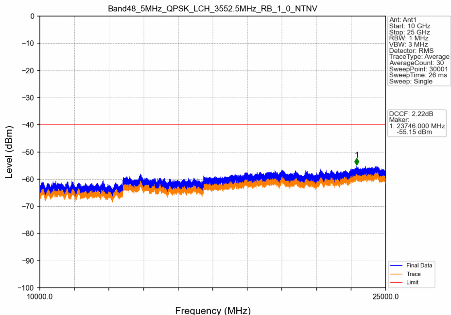
Band48_5MHz_QPSK_LCH_3552.5MHz_RB_1_0_NTNV
