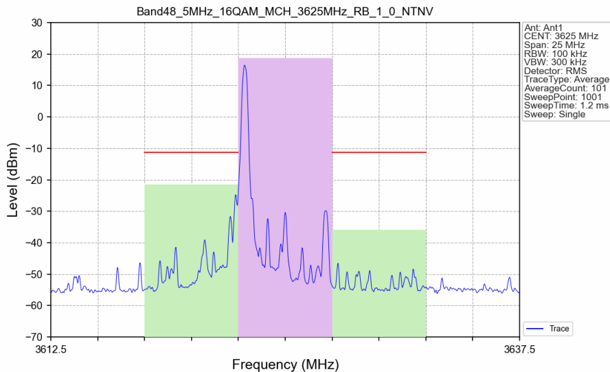
Band48_5MHz_16QAM_MCH_3625MHz_RB_1_0_NTNV
