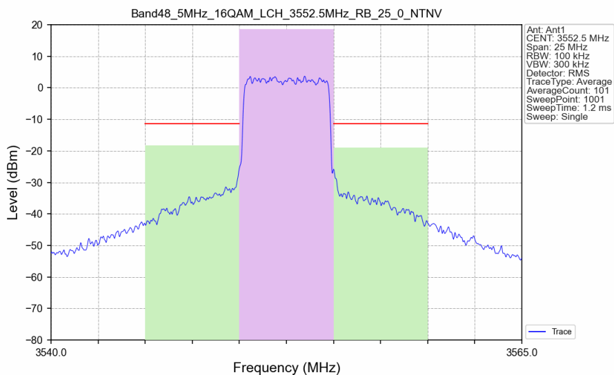
Band48_5MHz_16QAM_LCH_3552.5MHz_RB_25_0_NTNV
