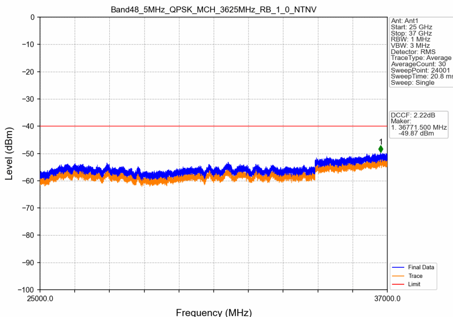
Band48_5MHz_QPSK_MCH_3625MHz_RB_1_0_NTNV
