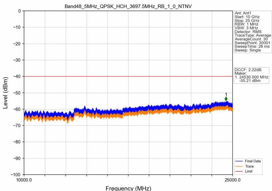
Band48_5MHz_QPSK_HCH_3697.5MHz_RB_1_0_NTNV
