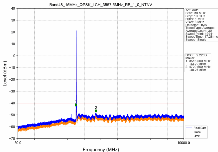
Band48_15MHz_QPSK_LCH_3557.5MHz_RB_1_0_NTNV
