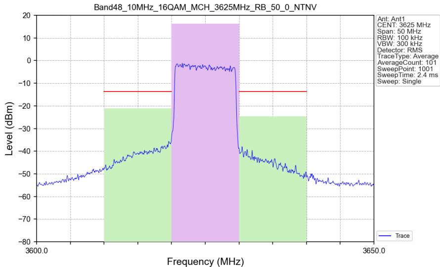
Band48_10MHz_16QAM_MCH_3625MHz_RB_50_0_NTNV
