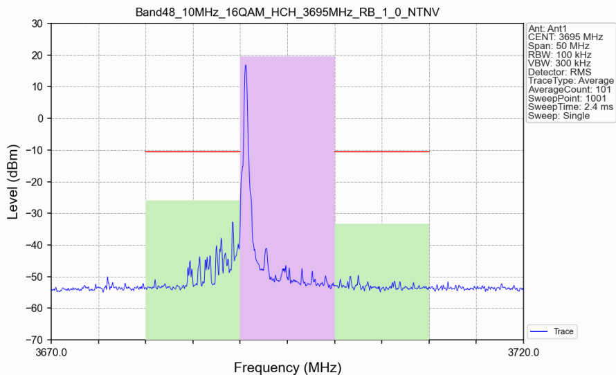
Band48_10MHz_16QAM_HCH_3695MHz_RB_1_0_NTNV
