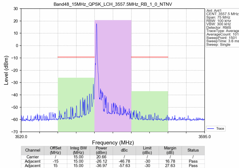
Band48_15MHz_QPSK_LCH_3557.5MHz_RB_1_0_NTNV
