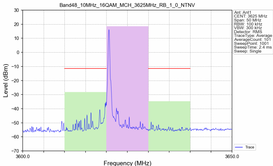
Band48_10MHz_16QAM_MCH_3625MHz_RB_1_0_NTNV
