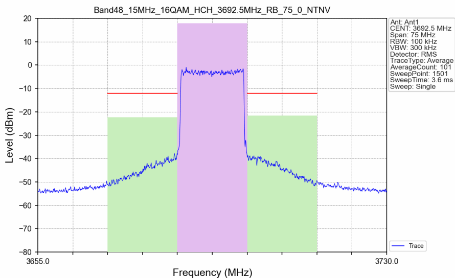
Band48_15MHz_16QAM_HCH_3692.5MHz_RB_75_0_NTNV
