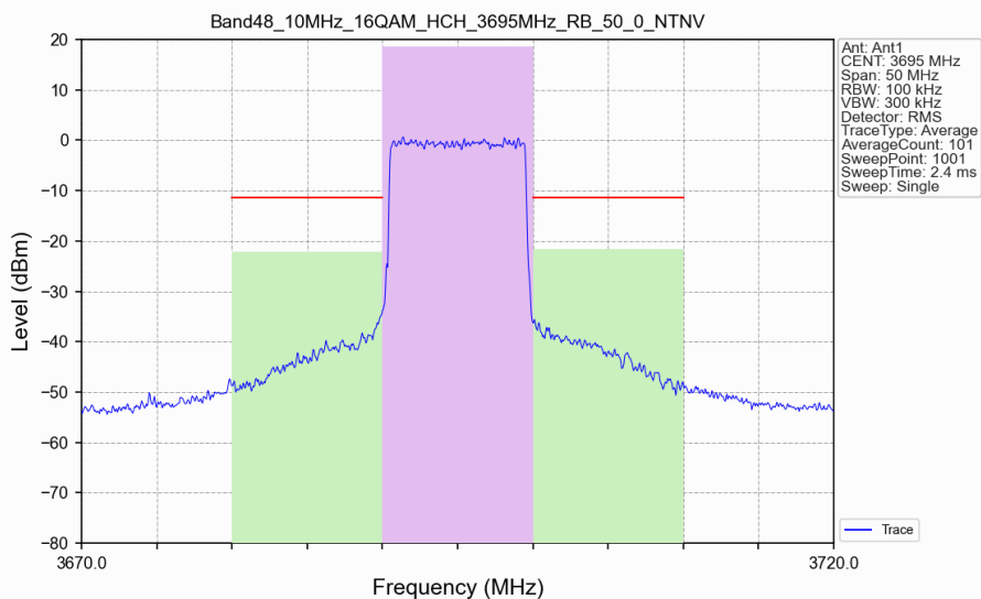
Band48_10MHz_16QAM_HCH_3695MHz_RB_50_0_NTNV
