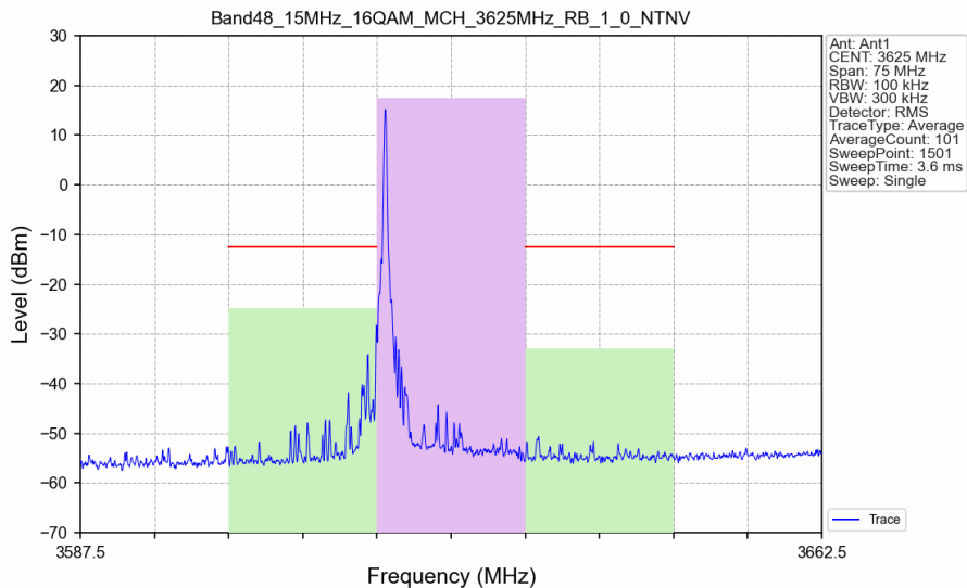
Band48_15MHz_16QAM_MCH_3625MHz_RB_1_0_NTNV
