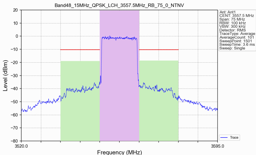
Band48_15MHz_QPSK_LCH_3557.5MHz_RB_75_0_NTNV
