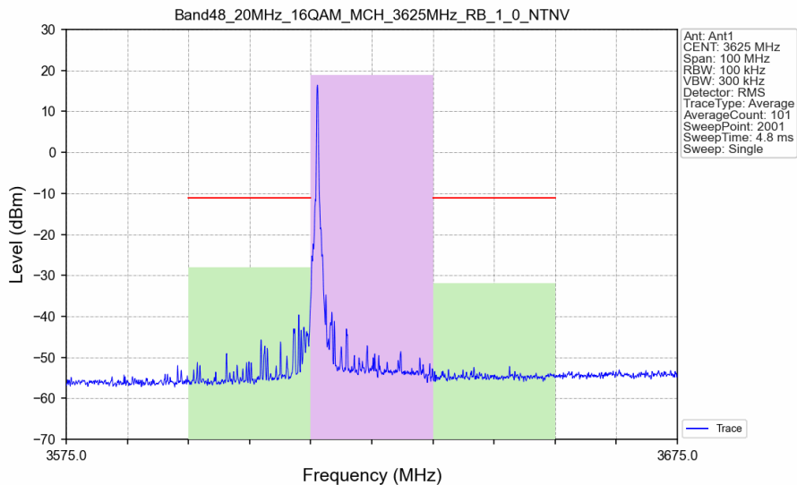
Band48_20MHz_16QAM_MCH_3625MHz_RB_1_0_NTNV
