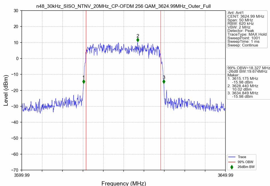
n48_30kHz_SISO_NTNV_20MHz_CP-OFDM 256 QAM_3624.99MHz_Outer_Full_Ant1
