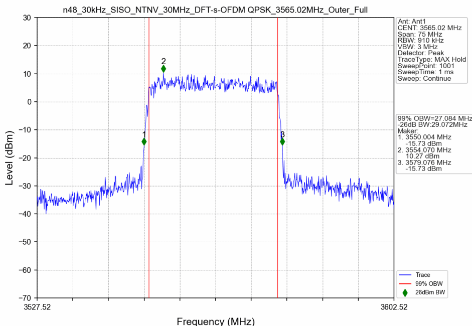
n48_30kHz_SISO_NTNV_30MHz_DFT-s-OFDM QPSK_3565.02MHz_Outer_Full_Ant1
