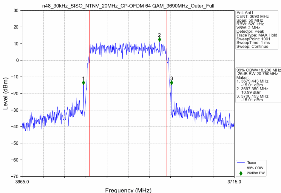
n48_30kHz_SISO_NTNV_20MHz_CP-OFDM 64 QAM_3690MHz_Outer_Full_Ant1
