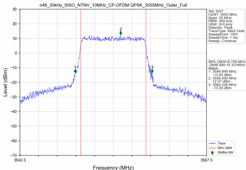
n48_30kHz_SISO_NTNV_10MHz_CP-OFDM QPSK_3555MHz_Outer_Full_Ant1
