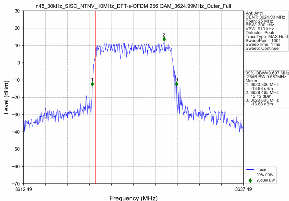
n48_30kHz_SISO_NTNV_10MHz_DFT-s-OFDM 256 QAM_3624.99MHz_Outer_Full_Ant1
