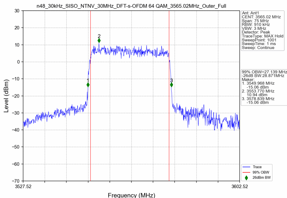
n48_30kHz_SISO_NTNV_30MHz_DFT-s-OFDM 64 QAM_3565.02MHz_Outer_Full_Ant1
