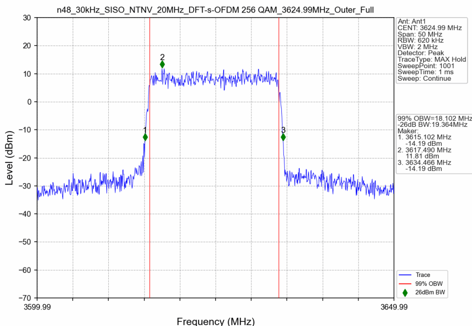
n48_30kHz_SISO_NTNV_20MHz_DFT-s-OFDM 256 QAM_3624.99MHz_Outer_Full_Ant1
