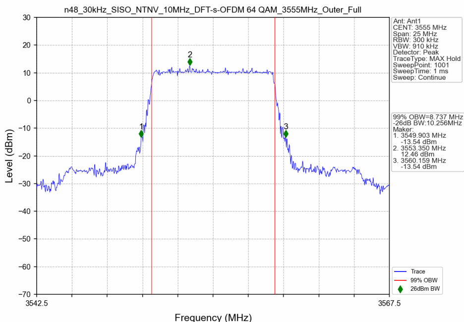
n48_30kHz_SISO_NTNV_10MHz_DFT-s-OFDM 64 QAM_3555MHz_Outer_Full_Ant1
