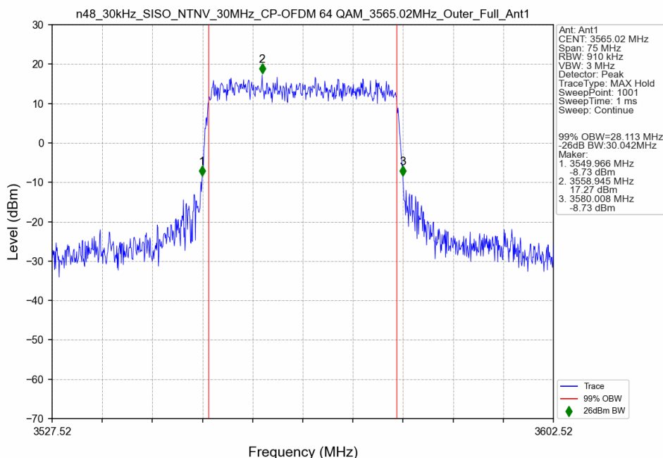
n48_30kHz_SISO_NTNV_30MHz_CP-OFDM 64 QAM_3565.02MHz_Outer_Full_Ant1
