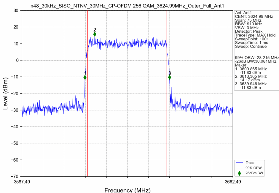
n48_30kHz_SISO_NTNV_30MHz_CP-OFDM 256 QAM_3624.99MHz_Outer_Full_Ant1
