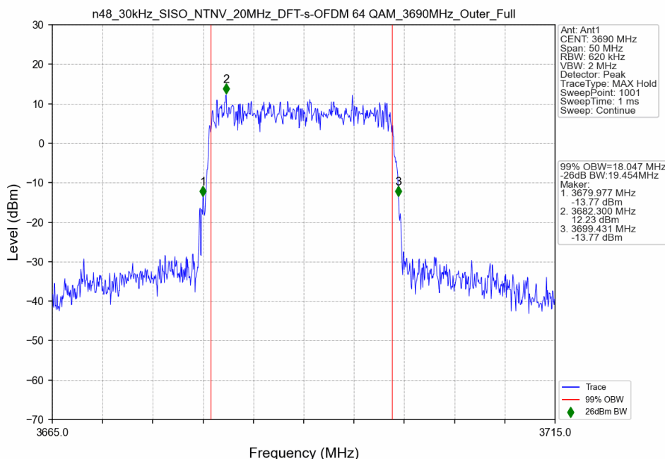
n48_30kHz_SISO_NTNV_20MHz_DFT-s-OFDM 64 QAM_3690MHz_Outer_Full_Ant1
