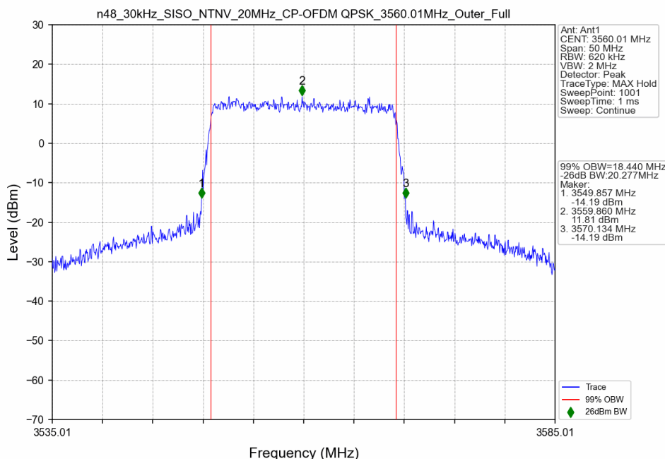
n48_30kHz_SISO_NTNV_20MHz_CP-OFDM QPSK_3560.01MHz_Outer_Full_Ant1
