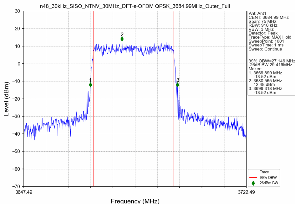
n48_30kHz_SISO_NTNV_30MHz_DFT-s-OFDM QPSK_3684.99MHz_Outer_Full_Ant1
