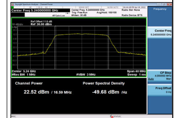
U-NII-1 Output Power-802.11a(20MHz) ,5240MHz,Ant2
