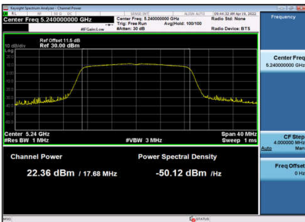
U-NII-1 Output Power-802.11n(20MHz) ,5240MHz,Ant4
