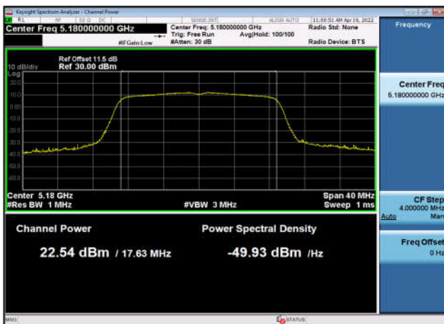
U-NII-1 Output Power-802.11ax(20MHz) ,5180MHz,Ant4
