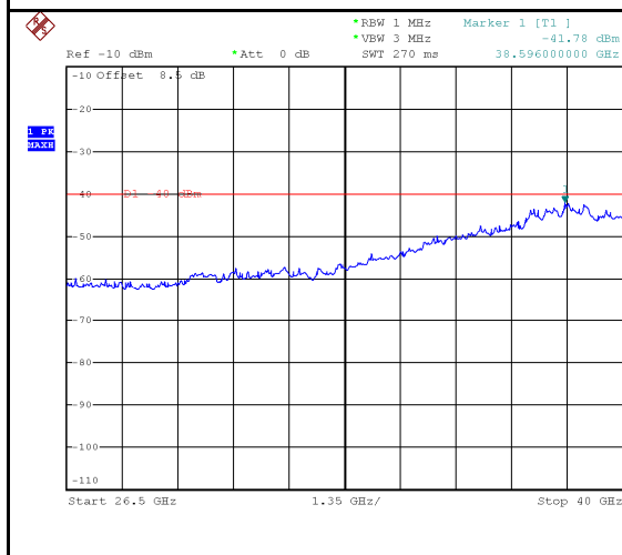
5MHz - Low CH 26.5GHz~40GHz
