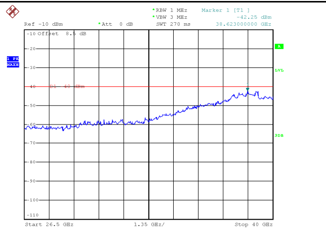
20MHz - High CH 26.5GHz~40GHz
