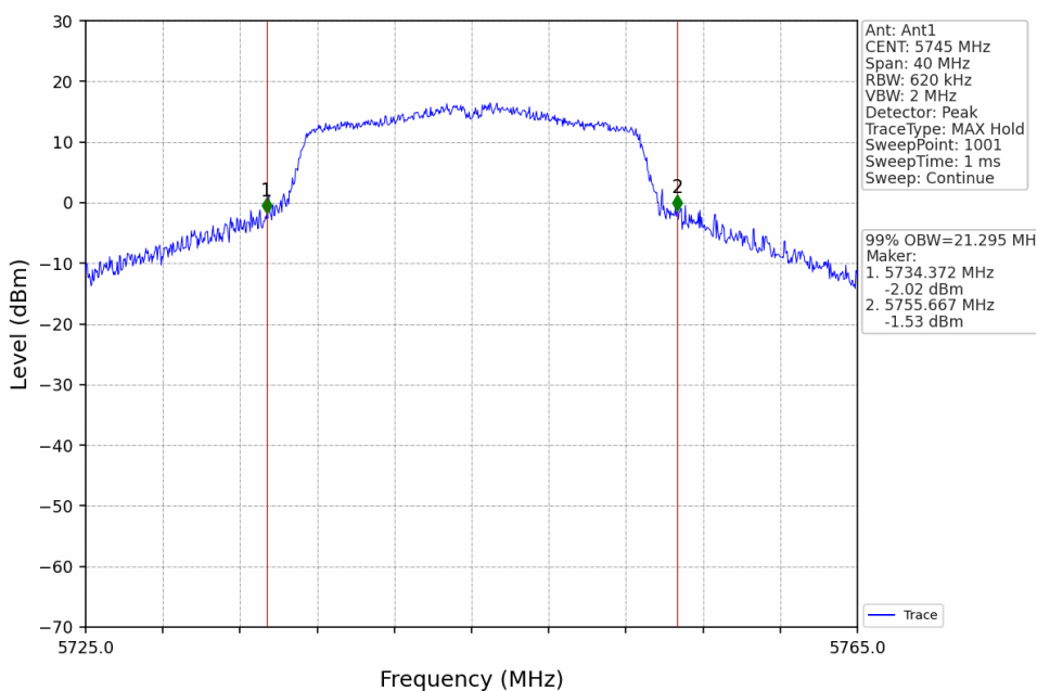
802.11ac(VHT20)_LCH_5745MHz_Ant1_NTNV
