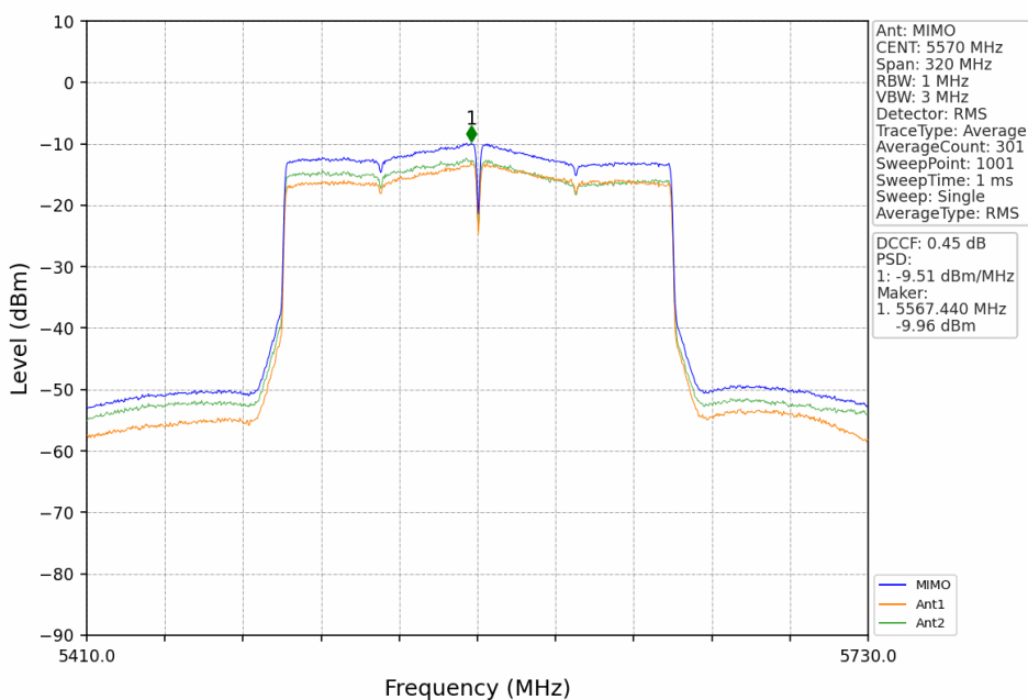
802.11ax(HEW160)_MCH_5570MHz_2xRU996_Left_MIMO_NTNV
