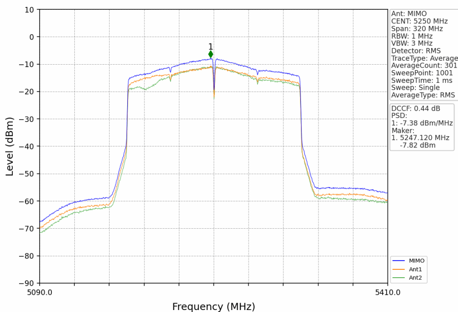
802.11ax(HEW160)_MCH_5250MHz_2xRU996_Left_MIMO_NTNV
