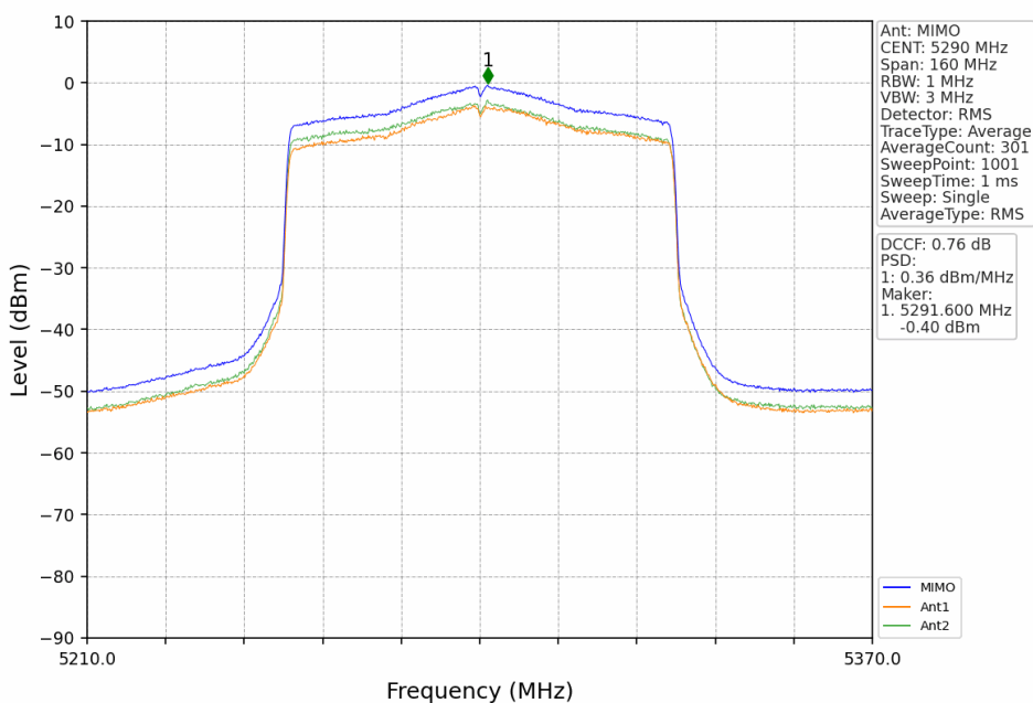
802.11ax(HEW80)_MCH_5290MHz_RU996_Left_MIMO_NTNV
