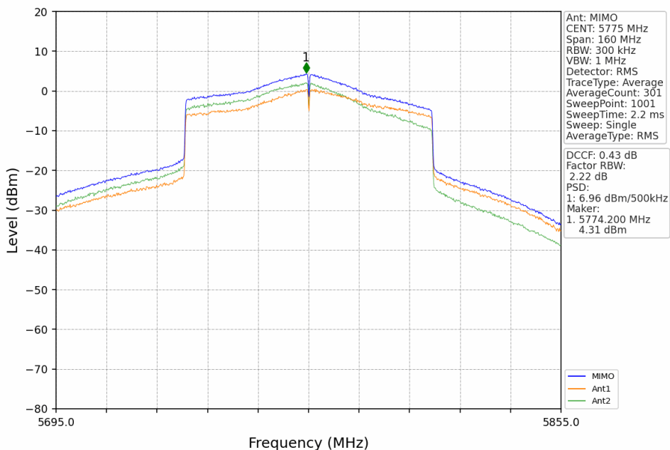
802.11ax(HEW80)_MCH_5775MHz_RU996_Left_MIMO_NTNV
