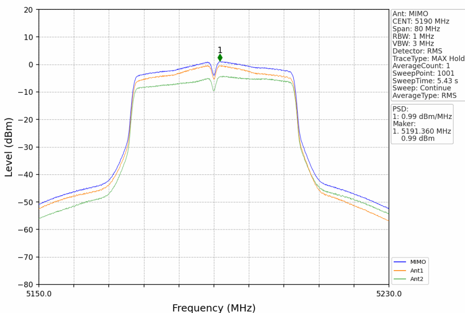
802.11n(HT40)_LCH_5190MHz_MIMO_NTNV
