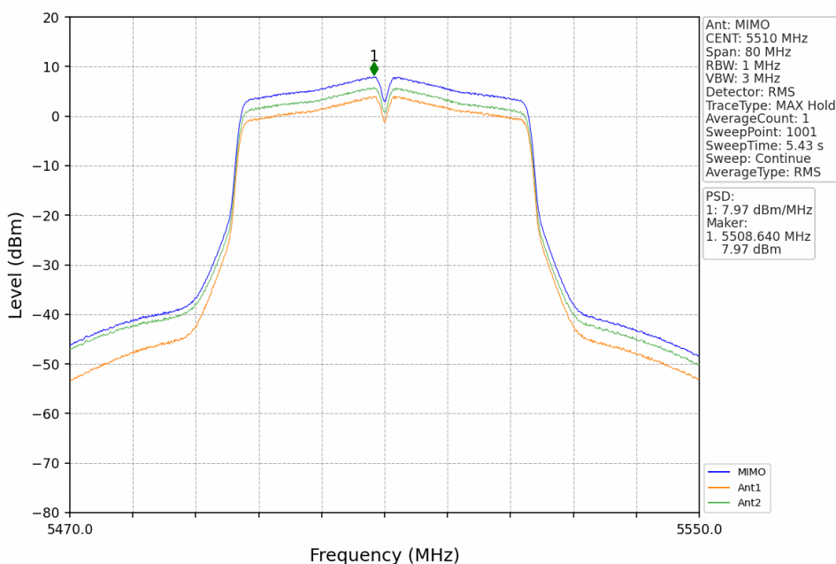
802.11n(HT40)_LCH_5510MHz_MIMO_NTNV
