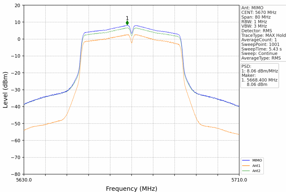
802.11ac(VHT40)_HCH_5670MHz_MIMO_NTNV
