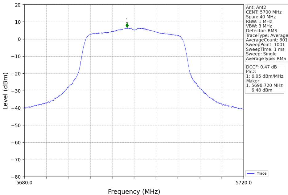
802.11ac(VHT20)_HCH_5700MHz_Ant2_NTNV
