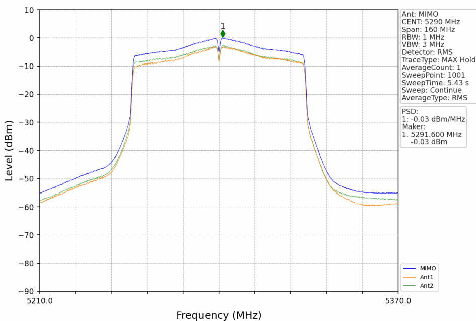
802.11ac(VHT80)_MCH_5290MHz_MIMO_NTNV
