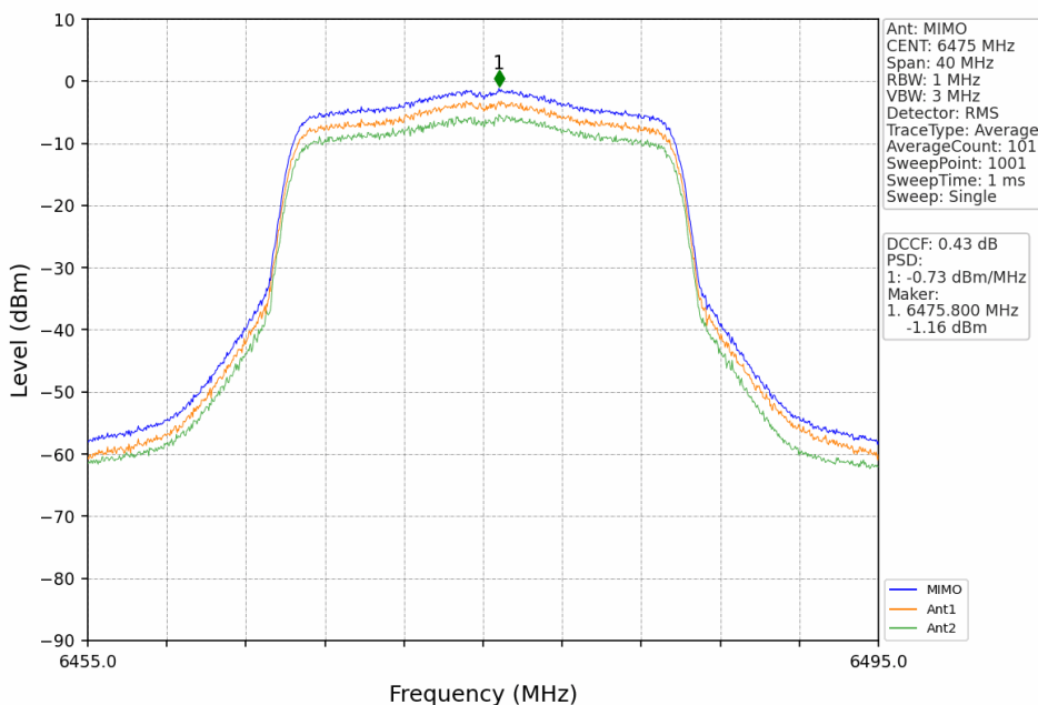
802.11ax(HEW20)_MCH_6475MHz_RU242_Left_MIMO_NTNV
