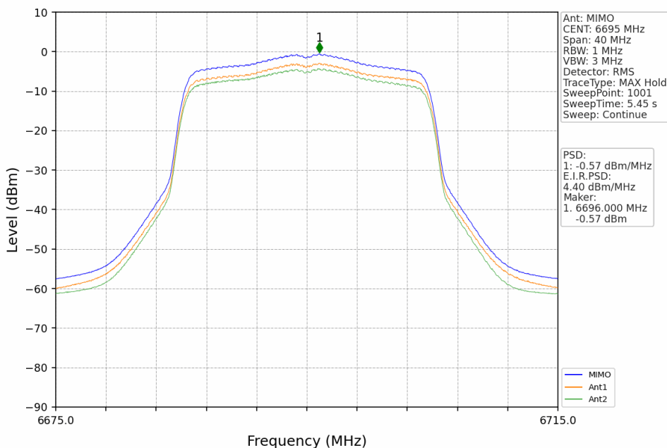
802.11ax(HEW20)_MCH_6695MHz_RU242_Left_MIMO_NTNV
