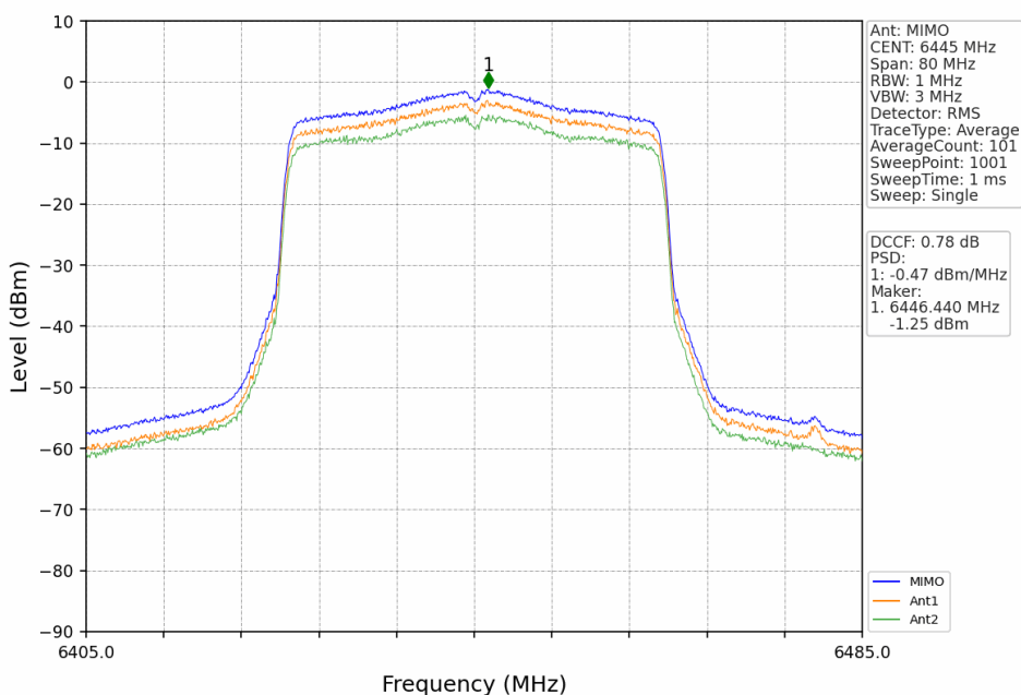
802.11ax(HEW40)_LCH_6445MHz_RU484_Left_MIMO_NTNV
