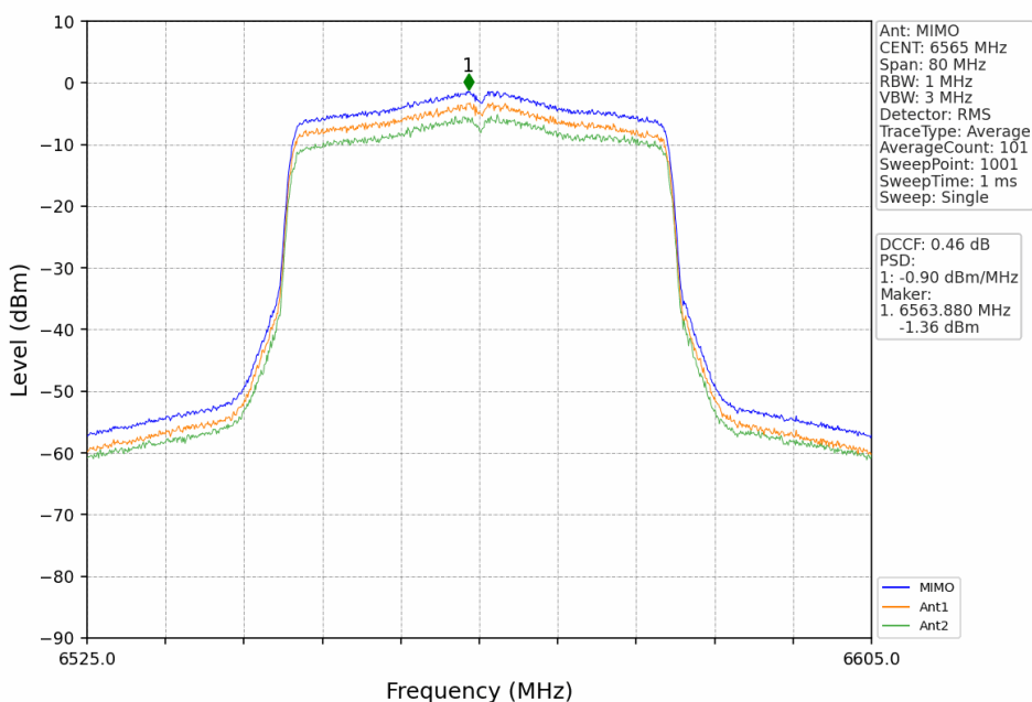
802.11ax(HEW40)_LCH_6565MHz_RU484_Left_MIMO_NTNV
