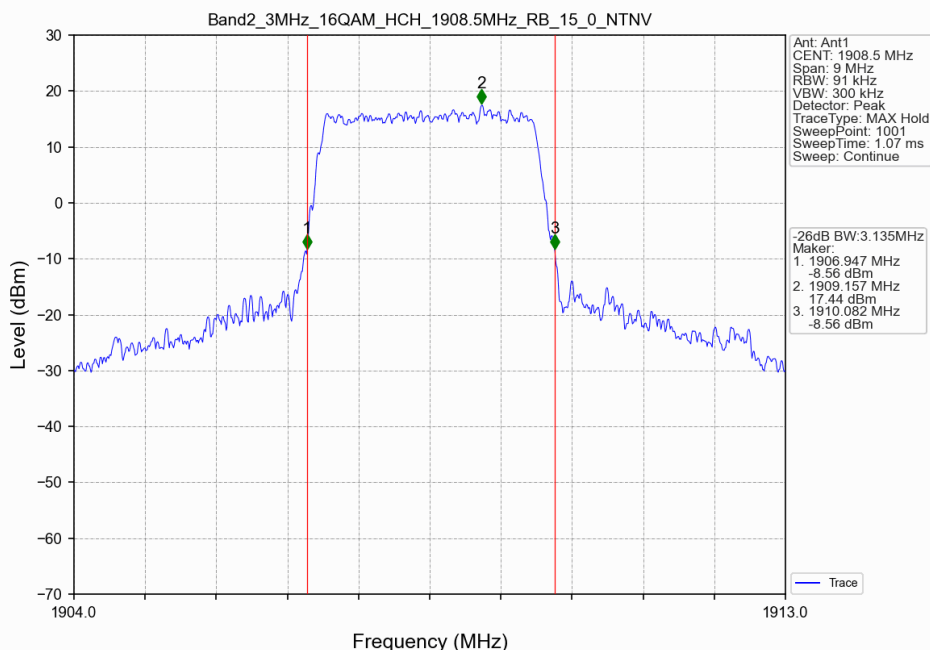
Band2_3MHz_16QAM_HCH_1908.5MHz_RB_15_0_NTNV
