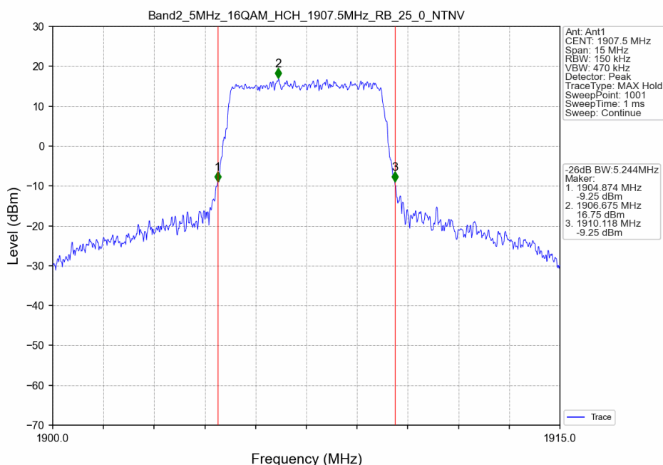
Band2_5MHz_16QAM_HCH_1907.5MHz_RB_25_0_NTNV
