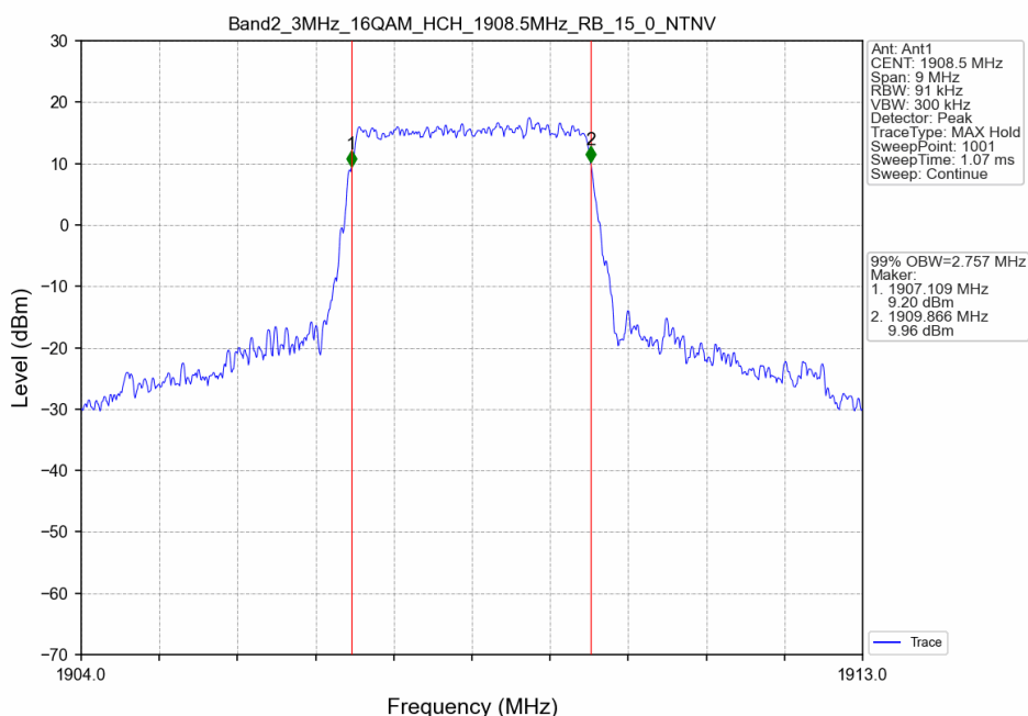
Band2_3MHz_16QAM_HCH_1908.5MHz_RB_15_0_NTNV
