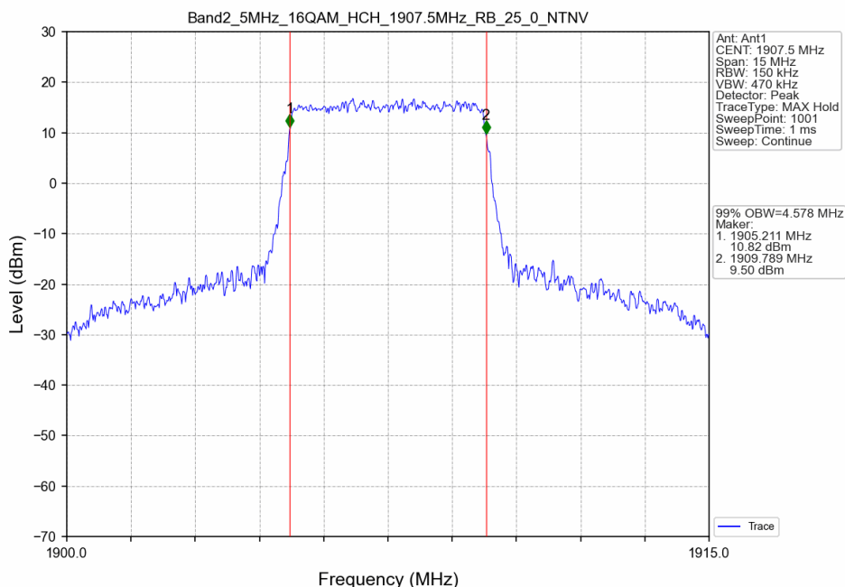
Band2_5MHz_16QAM_HCH_1907.5MHz_RB_25_0_NTNV
