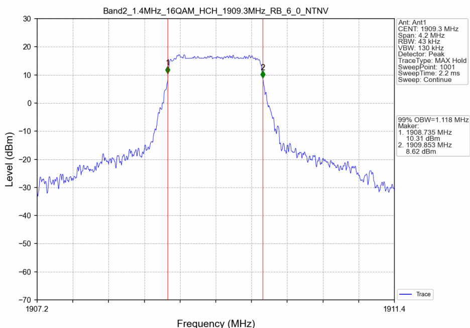
Band2_1.4MHz_16QAM_HCH_1909.3MHz_RB_6_0_NTNV
