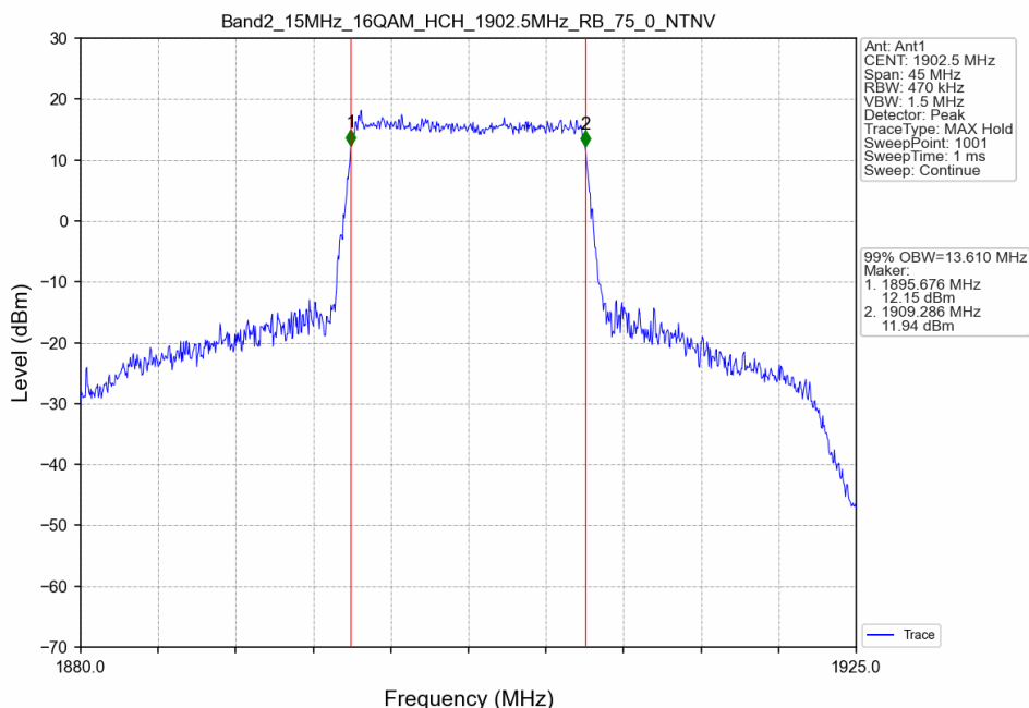
Band2_15MHz_16QAM_HCH_1902.5MHz_RB_75_0_NTNV
