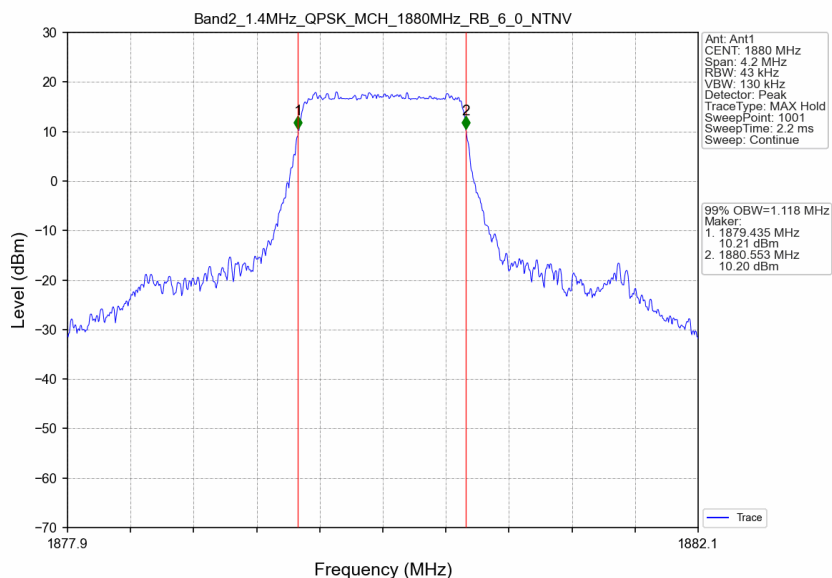
Band2_1.4MHz_QPSK_MCH_1880MHz_RB_6_0_NTNV
