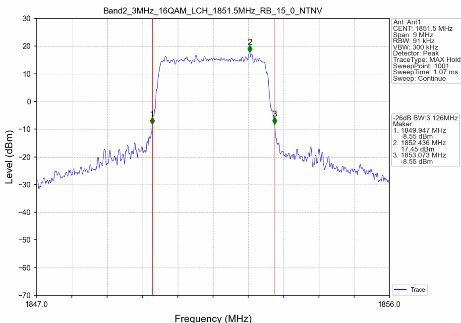
Band2_3MHz_16QAM_LCH_1851.5MHz_RB_15_0_NTNV
