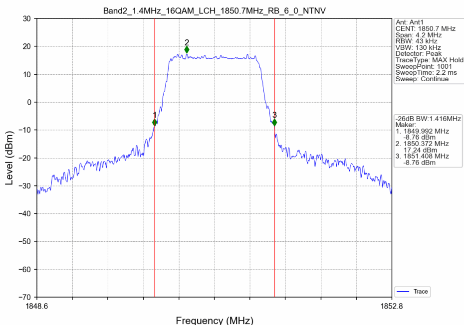
Band2_1.4MHz_16QAM_LCH_1850.7MHz_RB_6_0_NTNV
