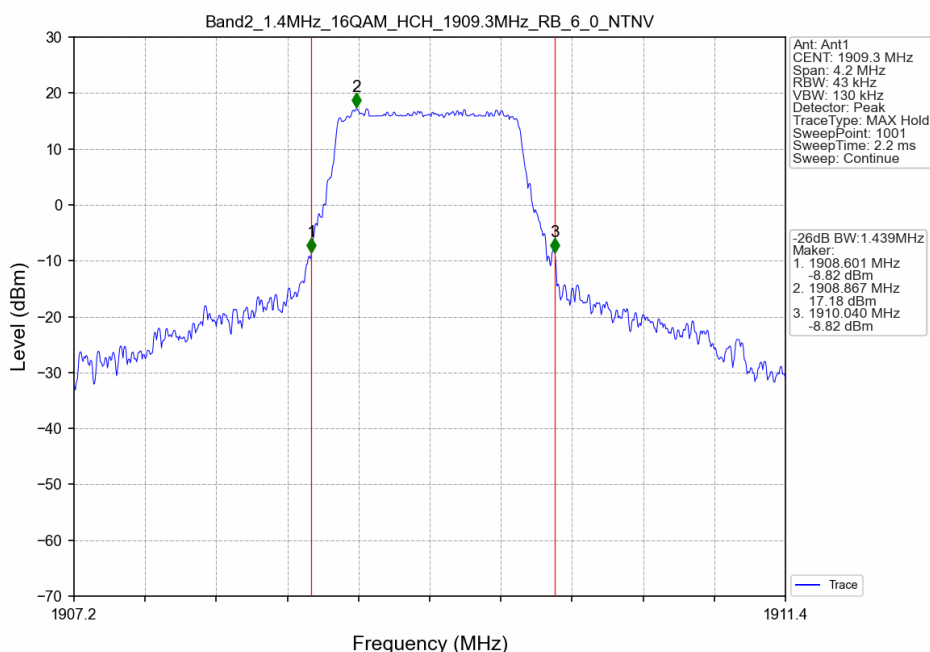
Band2_1.4MHz_16QAM_HCH_1909.3MHz_RB_6_0_NTNV
