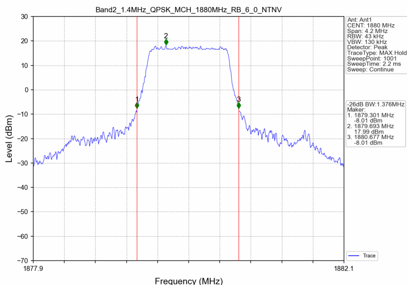
Band2_1.4MHz_QPSK_MCH_1880MHz_RB_6_0_NTNV
