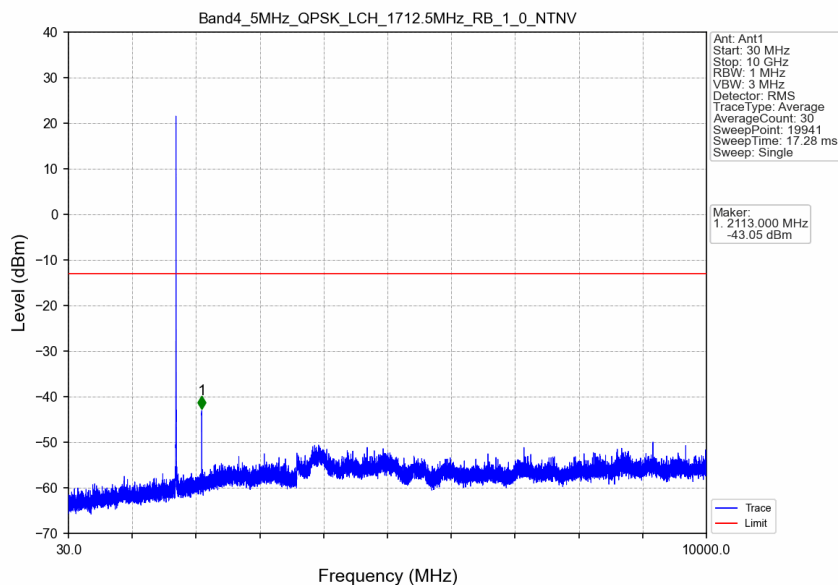
Band4_5MHz_QPSK_LCH_1712.5MHz_RB_1_0_NTNV
