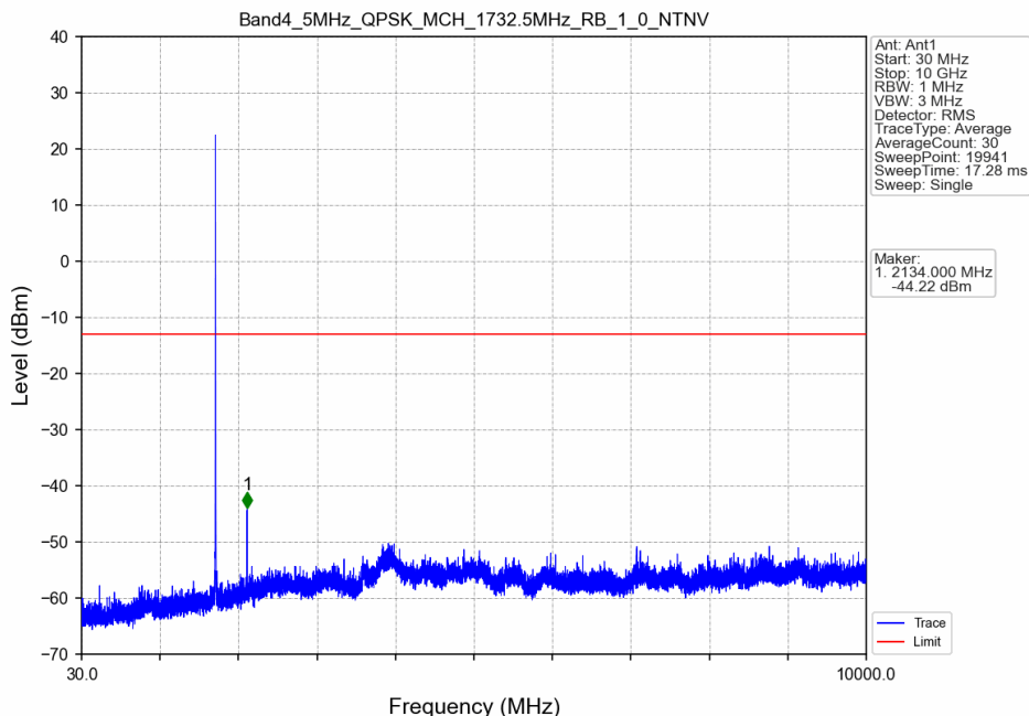
Band4_5MHz_QPSK_MCH_1732.5MHz_RB_1_0_NTNV
