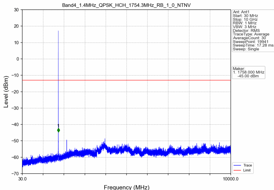
Band4_1.4MHz_QPSK_HCH_1754.3MHz_RB_1_0_NTNV
