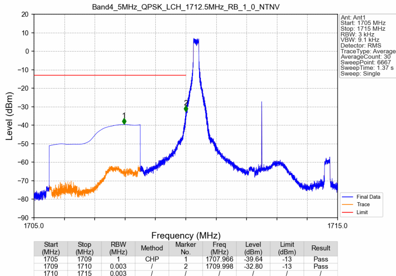
Band4_5MHz_QPSK_LCH_1712.5MHz_RB_1_0_NTNV
