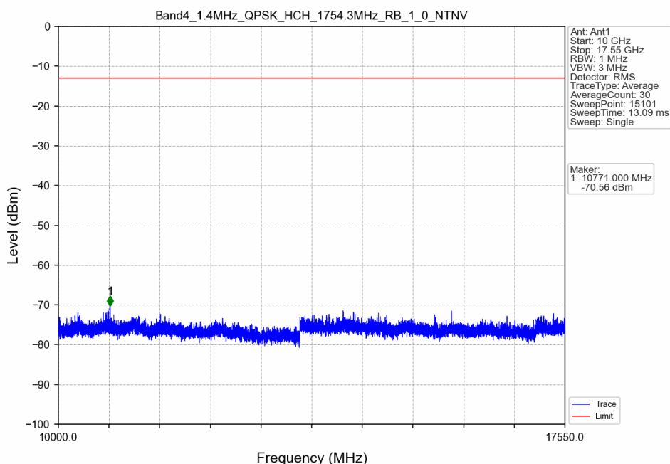
Band4_1.4MHz_QPSK_HCH_1754.3MHz_RB_1_0_NTNV
