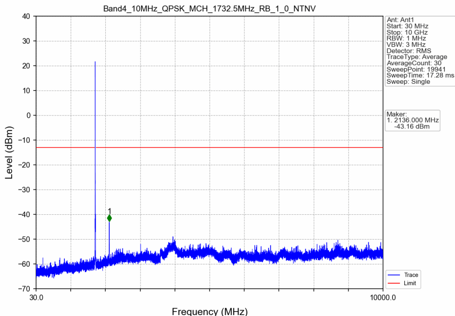
Band4_10MHz_QPSK_MCH_1732.5MHz_RB_1_0_NTNV
