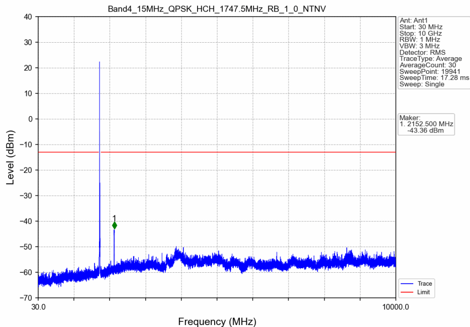
Band4_15MHz_QPSK_HCH_1747.5MHz_RB_1_0_NTNV
