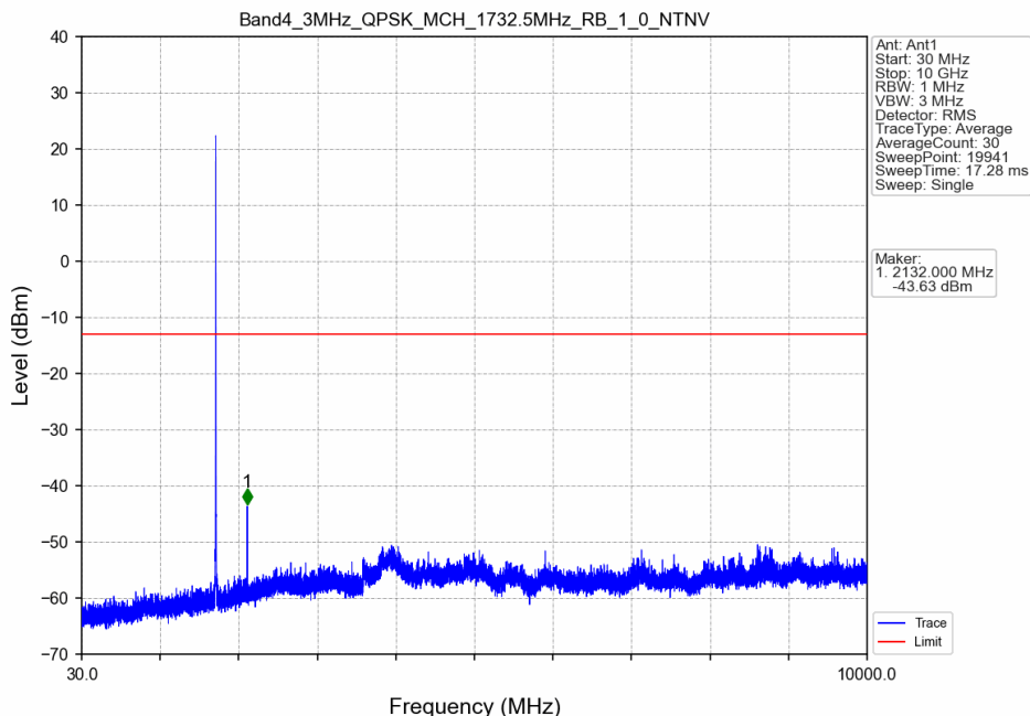
Band4_3MHz_QPSK_MCH_1732.5MHz_RB_1_0_NTNV
