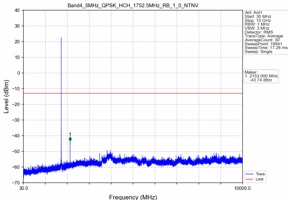
Band4_5MHz_QPSK_HCH_1752.5MHz_RB_1_0_NTNV
