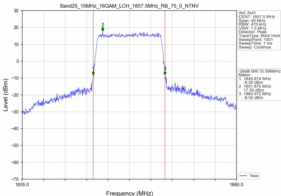
Band25_15MHz_16QAM_LCH_1857.5MHz_RB_75_0_NTNV
