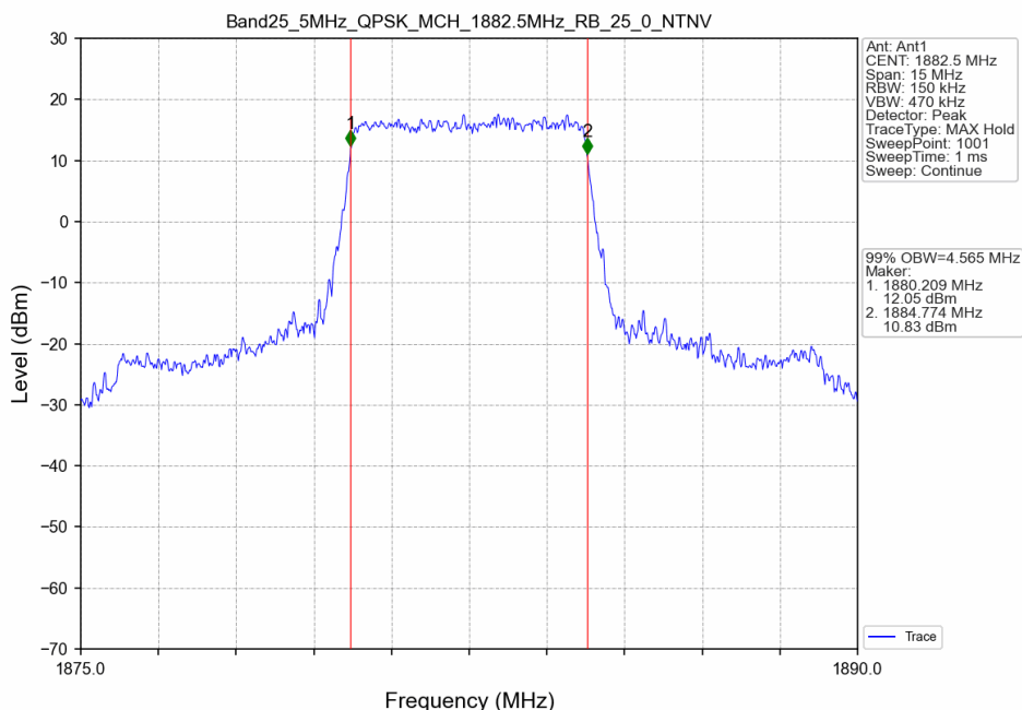
Band25_5MHz_QPSK_MCH_1882.5MHz_RB_25_0_NTNV
