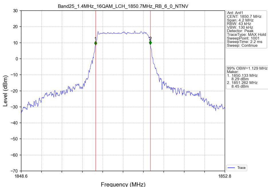
Band25_1.4MHz_16QAM_LCH_1850.7MHz_RB_6_0_NTNV
