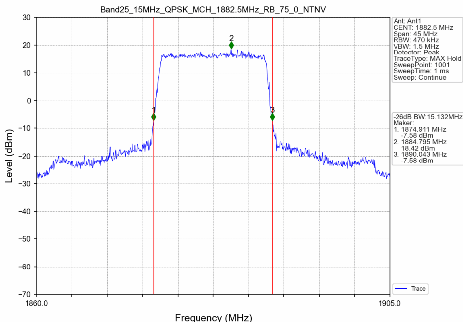
Band25_15MHz_QPSK_MCH_1882.5MHz_RB_75_0_NTNV
