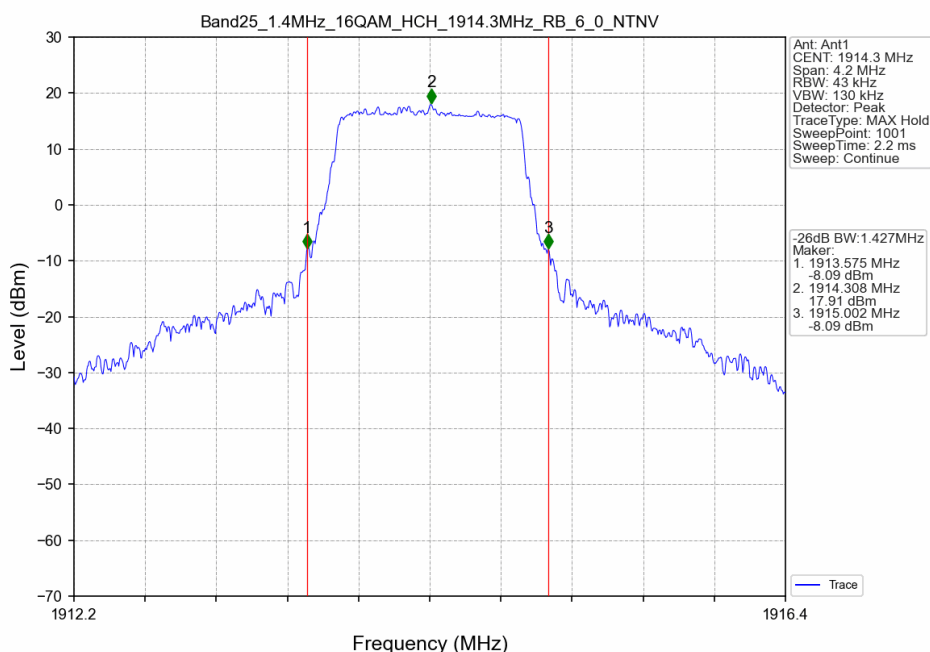
Band25_1.4MHz_16QAM_HCH_1914.3MHz_RB_6_0_NTNV
