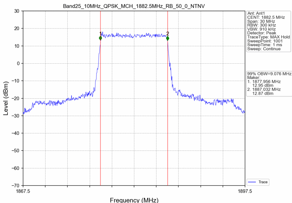
Band25_10MHz_QPSK_MCH_1882.5MHz_RB_50_0_NTNV
