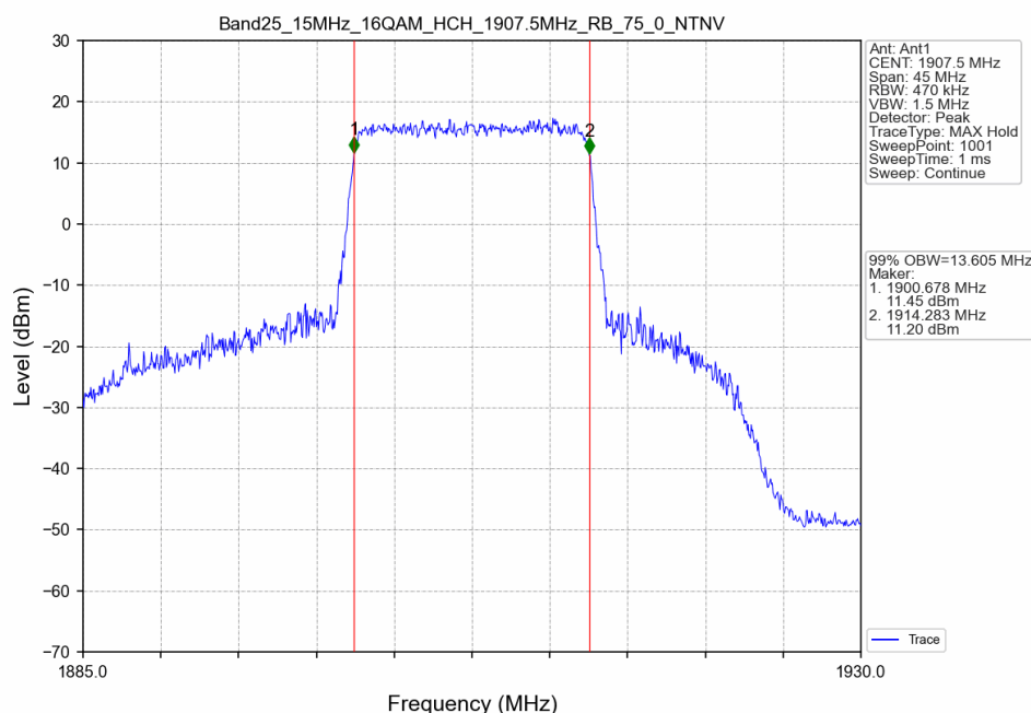
Band25_15MHz_16QAM_HCH_1907.5MHz_RB_75_0_NTNV
