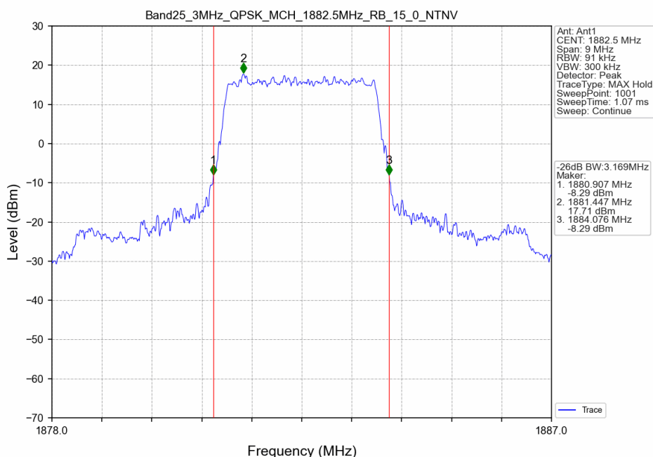
Band25_3MHz_QPSK_MCH_1882.5MHz_RB_15_0_NTNV
