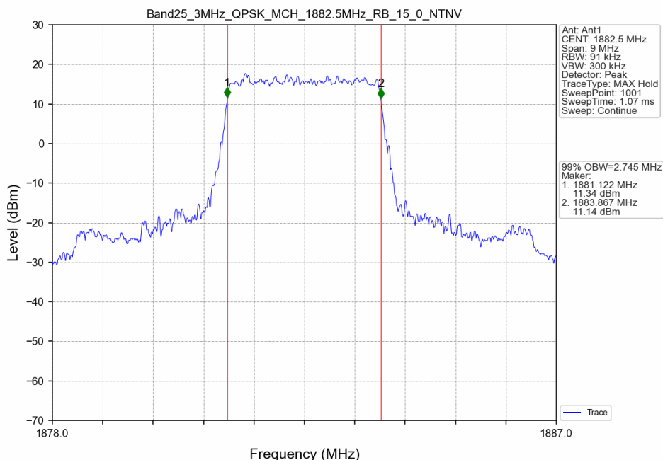
Band25_3MHz_QPSK_MCH_1882.5MHz_RB_15_0_NTNV
