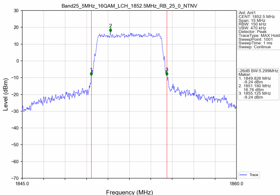
Band25_5MHz_16QAM_LCH_1852.5MHz_RB_25_0_NTNV
