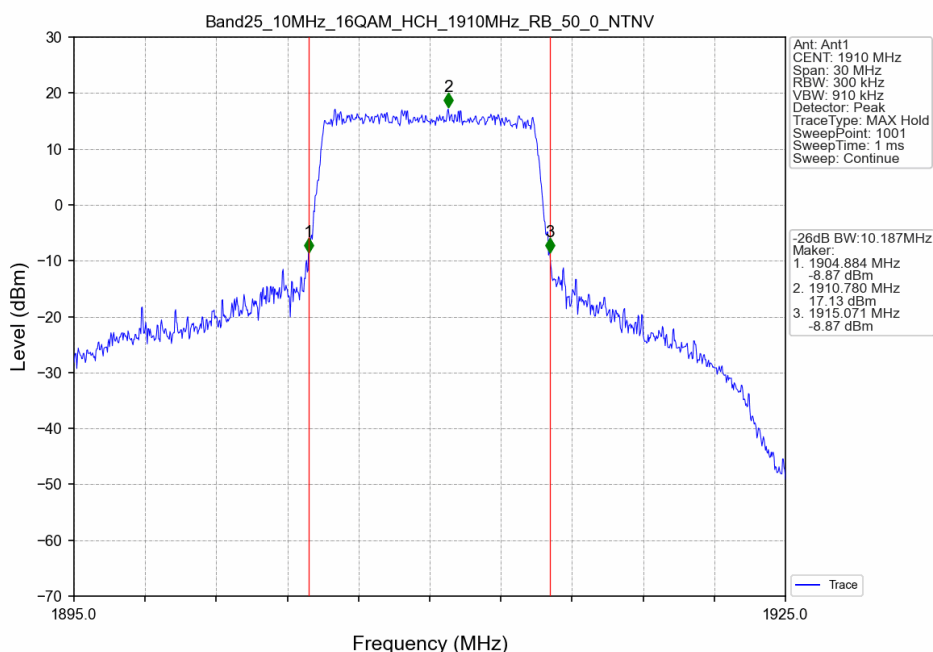
Band25_10MHz_16QAM_HCH_1910MHz_RB_50_0_NTNV
