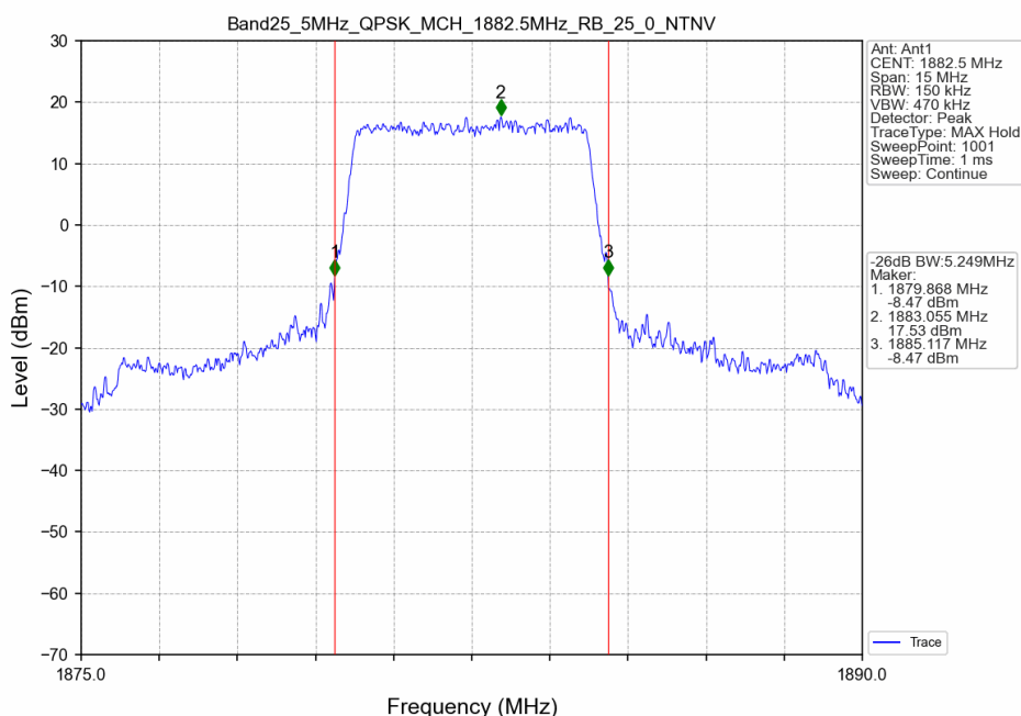
Band25_5MHz_QPSK_MCH_1882.5MHz_RB_25_0_NTNV
