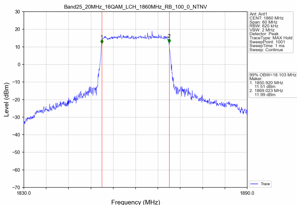
Band25_20MHz_16QAM_LCH_1860MHz_RB_100_0_NTNV
