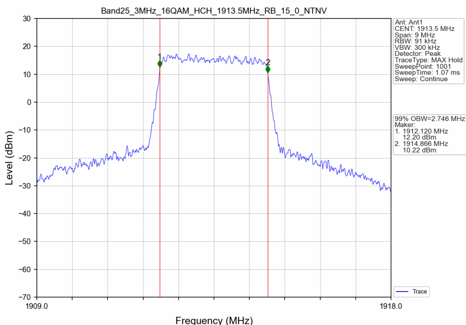
Band25_3MHz_16QAM_HCH_1913.5MHz_RB_15_0_NTNV
