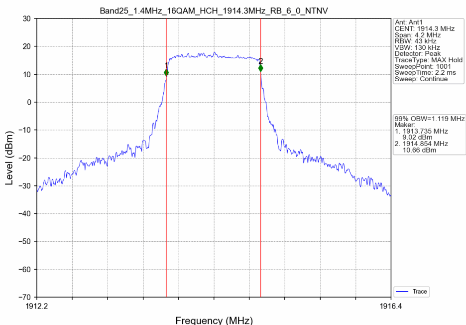
Band25_1.4MHz_16QAM_HCH_1914.3MHz_RB_6_0_NTNV
