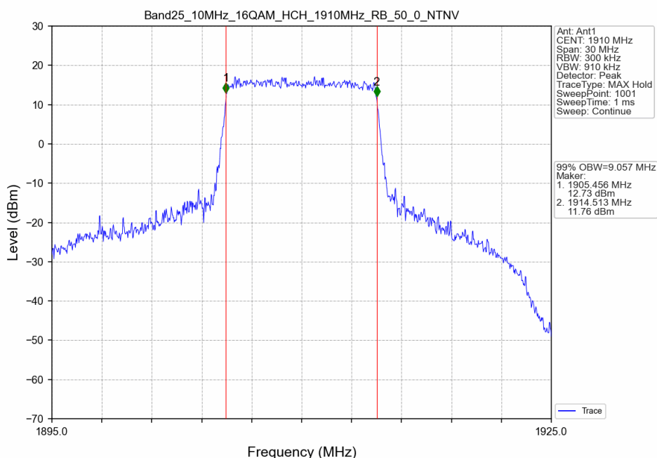
Band25_10MHz_16QAM_HCH_1910MHz_RB_50_0_NTNV
