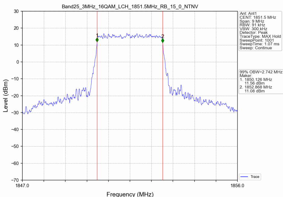
Band25_3MHz_16QAM_LCH_1851.5MHz_RB_15_0_NTNV
