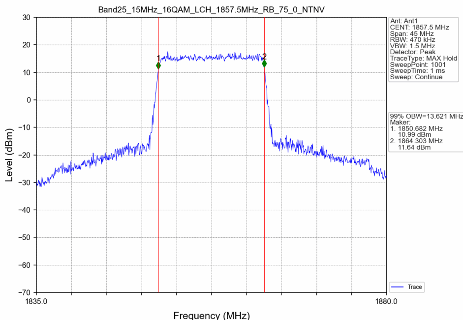
Band25_15MHz_16QAM_LCH_1857.5MHz_RB_75_0_NTNV
