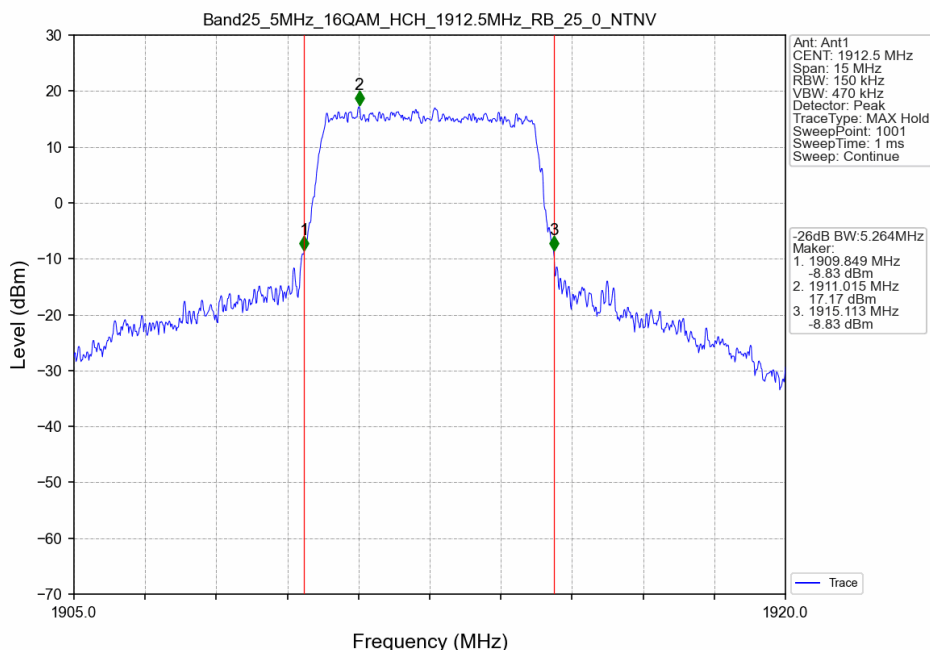
Band25_5MHz_16QAM_HCH_1912.5MHz_RB_25_0_NTNV
