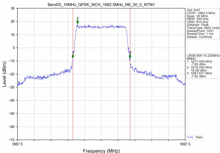
Band25_10MHz_QPSK_MCH_1882.5MHz_RB_50_0_NTNV
