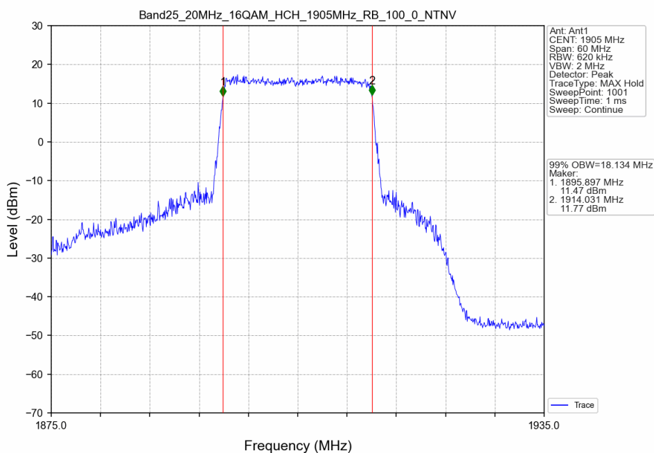
Band25_20MHz_16QAM_HCH_1905MHz_RB_100_0_NTNV
