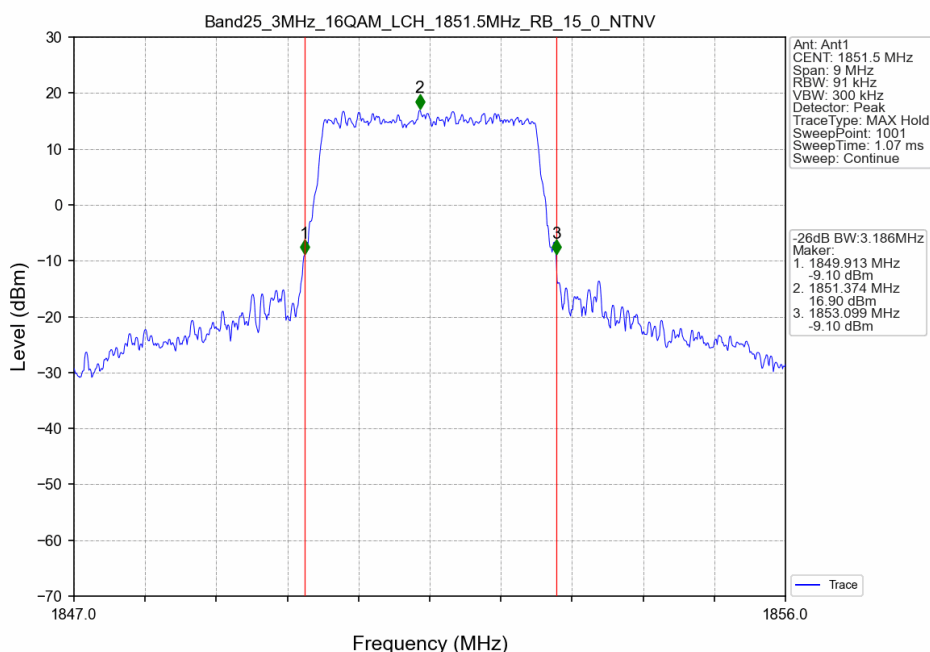
Band25_3MHz_16QAM_LCH_1851.5MHz_RB_15_0_NTNV
