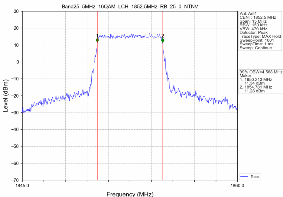
Band25_5MHz_16QAM_LCH_1852.5MHz_RB_25_0_NTNV
