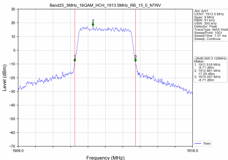
Band25_3MHz_16QAM_HCH_1913.5MHz_RB_15_0_NTNV
