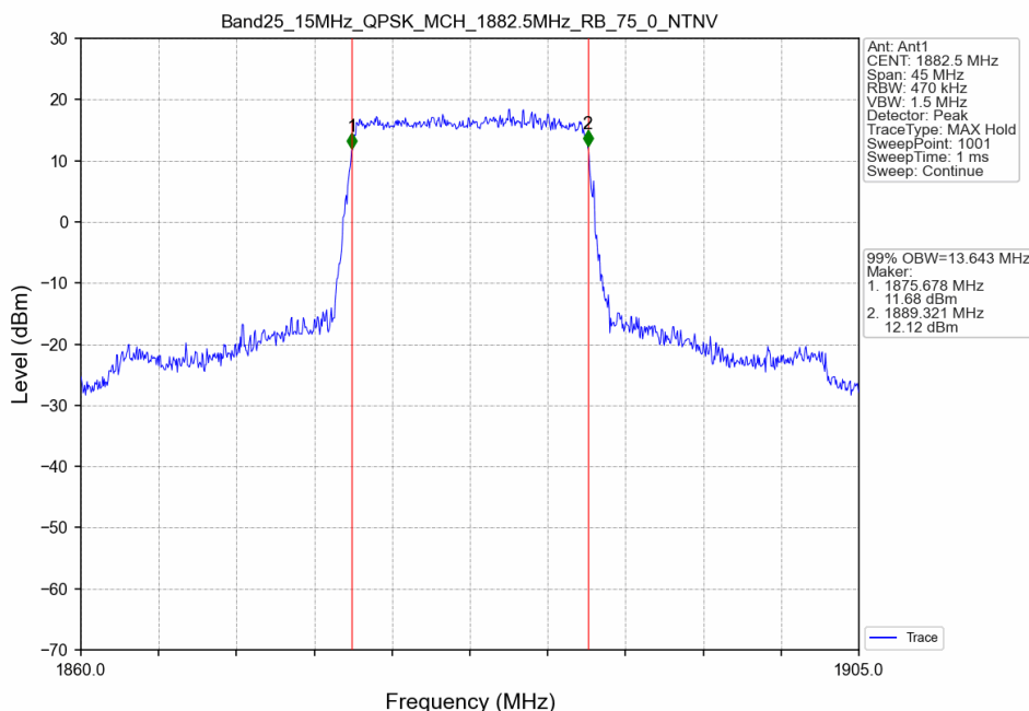
Band25_15MHz_QPSK_MCH_1882.5MHz_RB_75_0_NTNV
