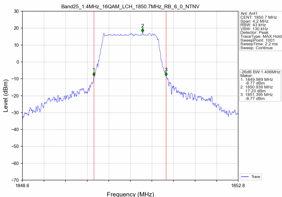
Band25_1.4MHz_16QAM_LCH_1850.7MHz_RB_6_0_NTNV
