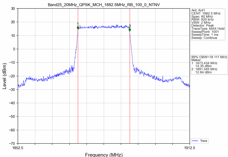
Band25_20MHz_QPSK_MCH_1882.5MHz_RB_100_0_NTNV
