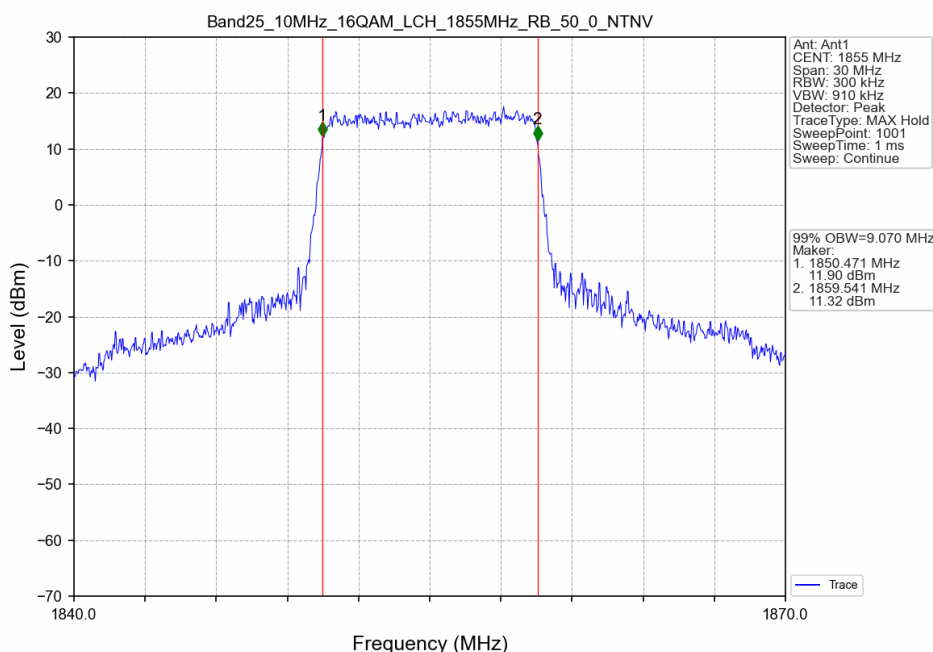
Band25_10MHz_16QAM_LCH_1855MHz_RB_50_0_NTNV
