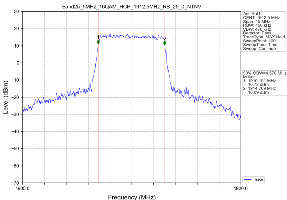
Band25_5MHz_16QAM_HCH_1912.5MHz_RB_25_0_NTNV
