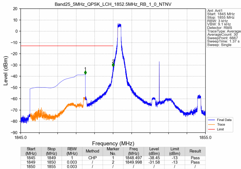
Band25_5MHz_QPSK_LCH_1852.5MHz_RB_1_0_NTNV
