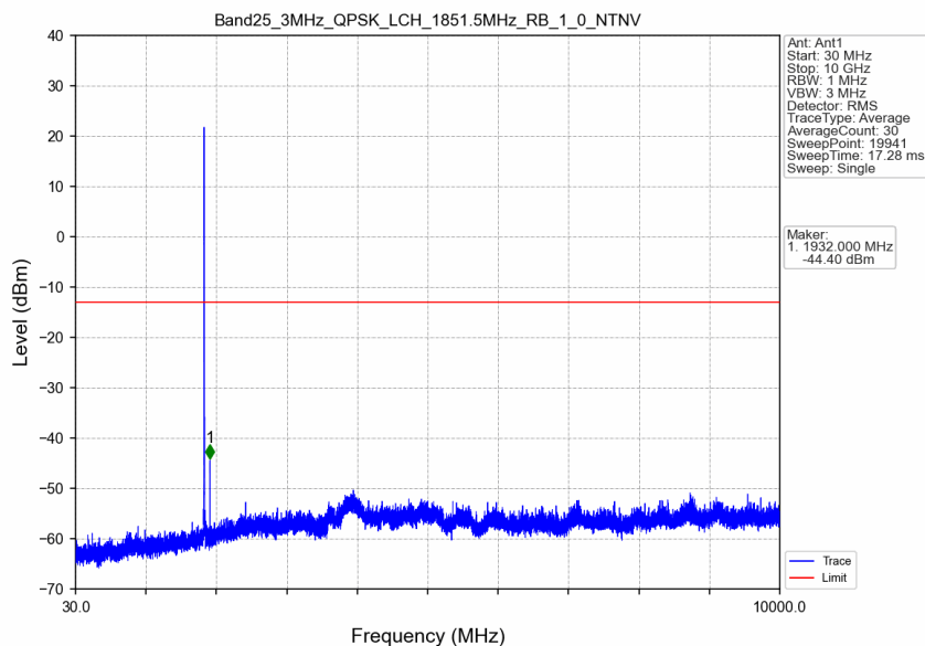
Band25_3MHz_QPSK_LCH_1851.5MHz_RB_1_0_NTNV
