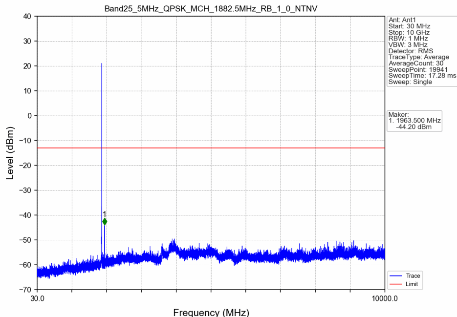
Band25_5MHz_QPSK_MCH_1882.5MHz_RB_1_0_NTNV
