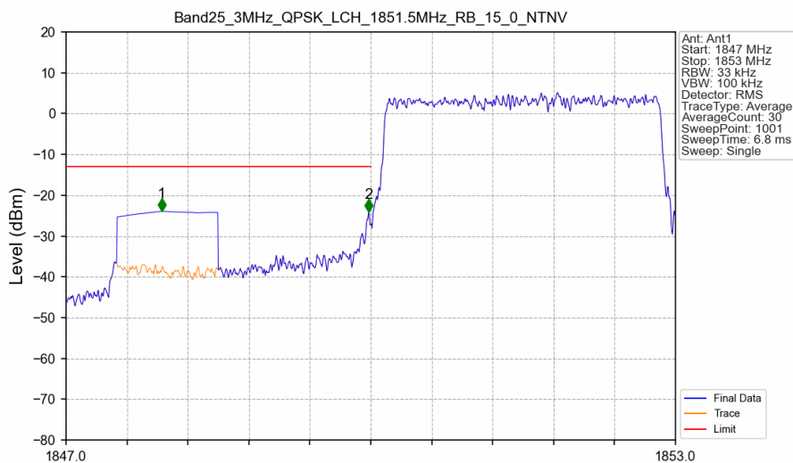
Band25_3MHz_QPSK_LCH_1851.5MHz_RB_15_0_NTNV
