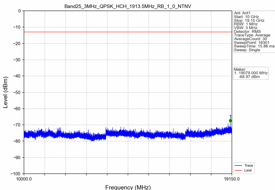
Band25_3MHz_QPSK_HCH_1913.5MHz_RB_1_0_NTNV
