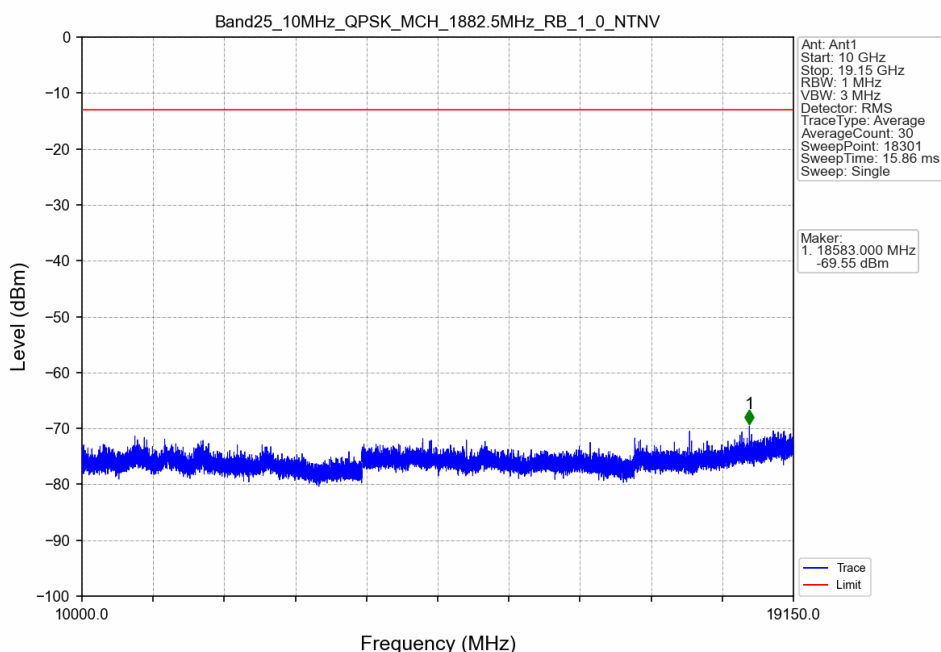
Band25_10MHz_QPSK_MCH_1882.5MHz_RB_1_0_NTNV
