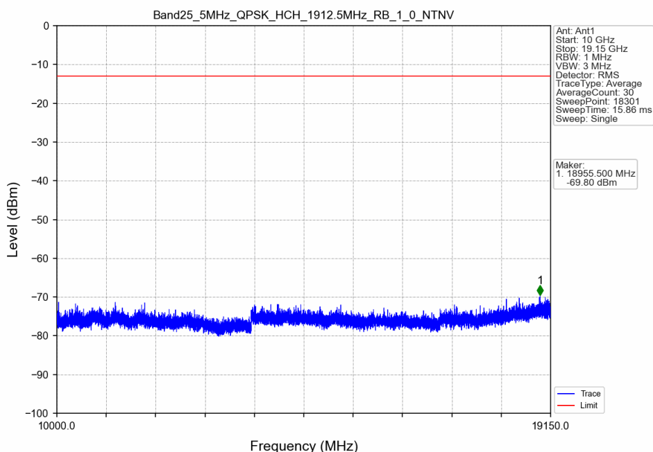
Band25_5MHz_QPSK_HCH_1912.5MHz_RB_1_0_NTNV
