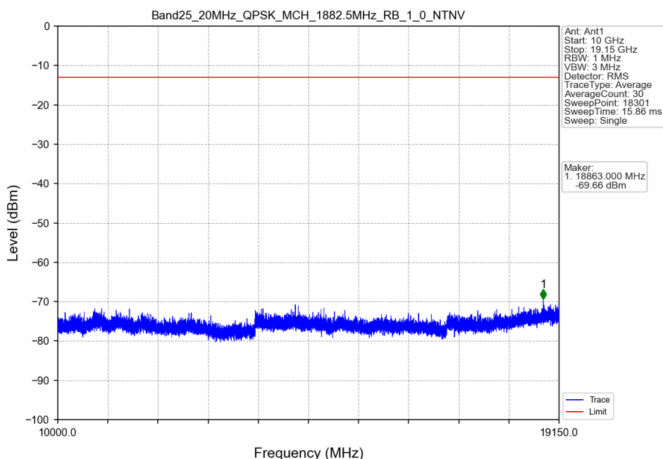
Band25_20MHz_QPSK_MCH_1882.5MHz_RB_1_0_NTNV
