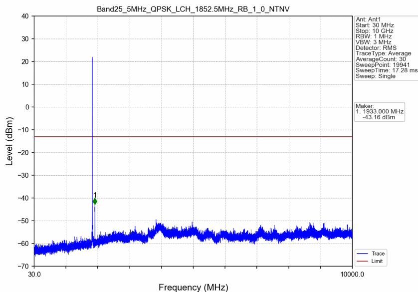
Band25_5MHz_QPSK_LCH_1852.5MHz_RB_1_0_NTNV
