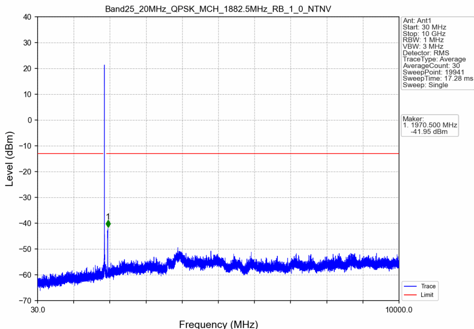
Band25_20MHz_QPSK_MCH_1882.5MHz_RB_1_0_NTNV
