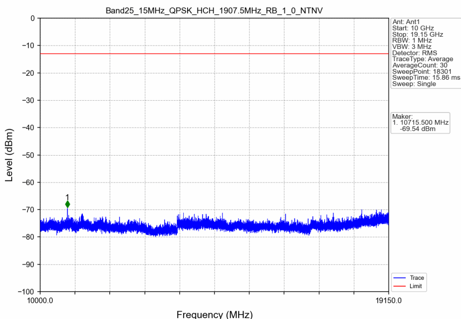
Band25_15MHz_QPSK_HCH_1907.5MHz_RB_1_0_NTNV
