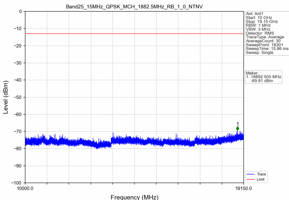
Band25_15MHz_QPSK_MCH_1882.5MHz_RB_1_0_NTNV
