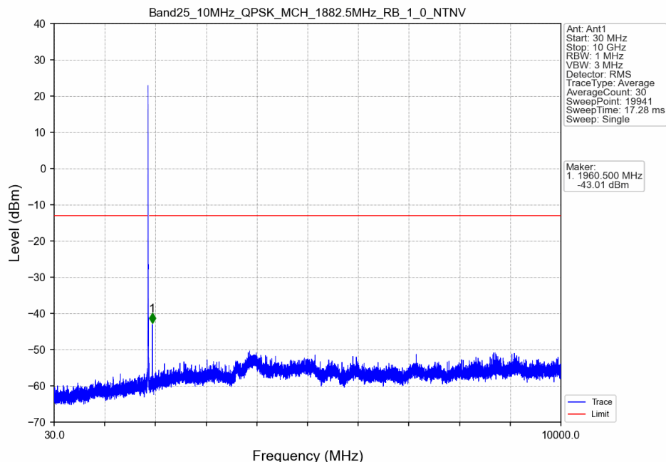
Band25_10MHz_QPSK_MCH_1882.5MHz_RB_1_0_NTNV
