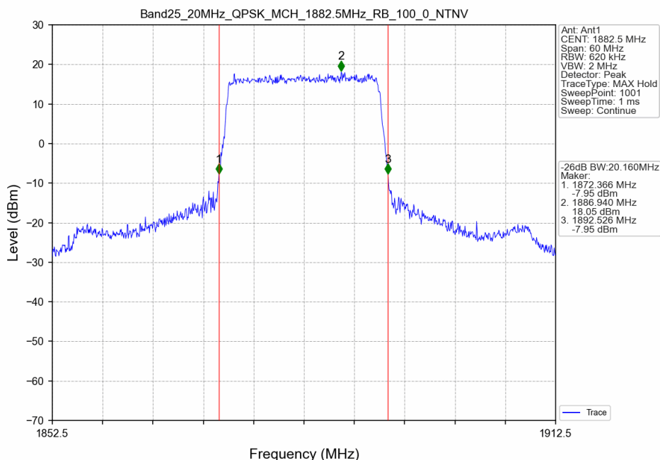
Band25_20MHz_QPSK_MCH_1882.5MHz_RB_100_0_NTNV
