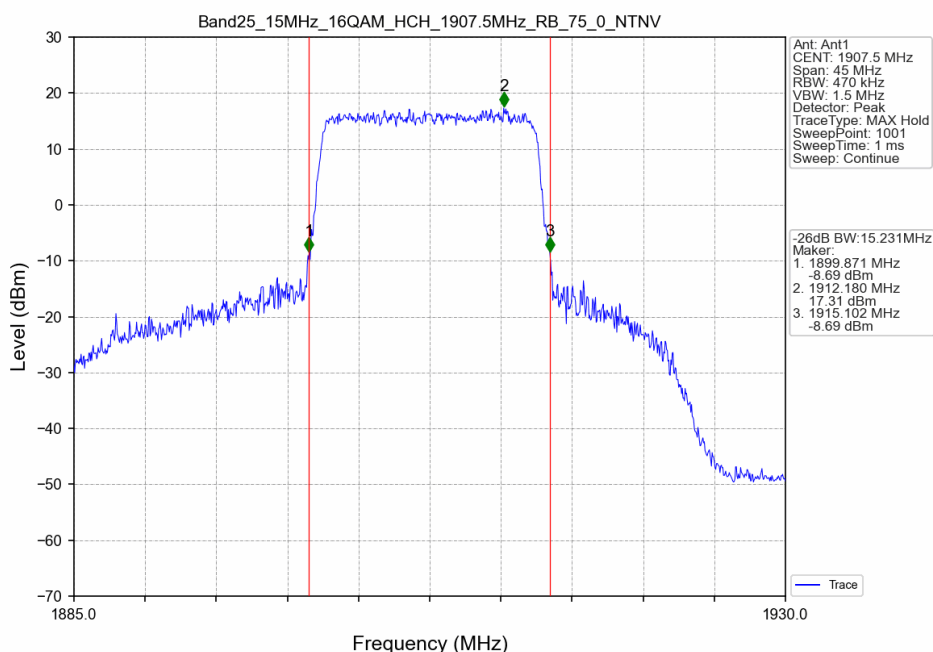
Band25_15MHz_16QAM_HCH_1907.5MHz_RB_75_0_NTNV
