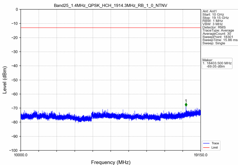
Band25_1.4MHz_QPSK_HCH_1914.3MHz_RB_1_0_NTNV
