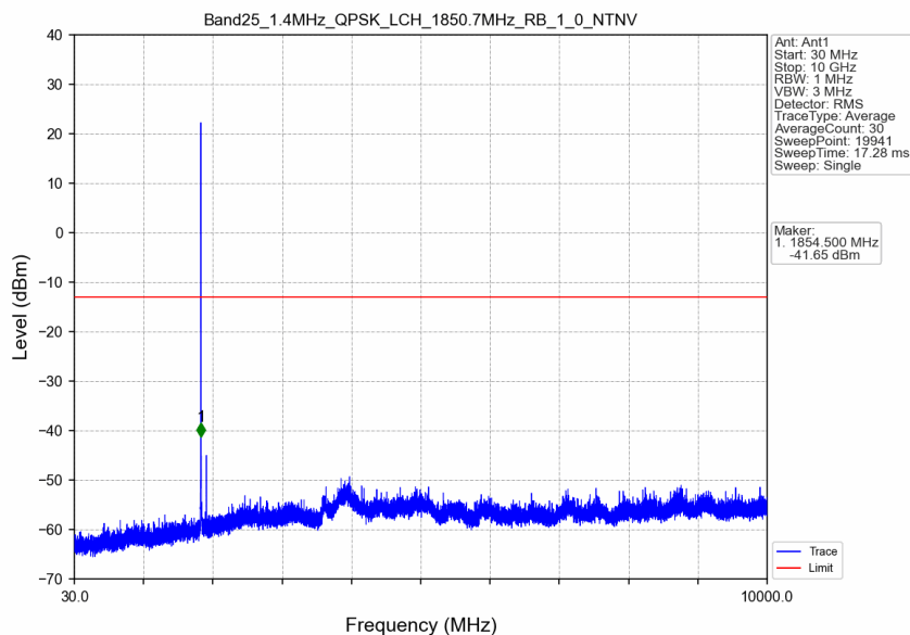
Band25_1.4MHz_QPSK_LCH_1850.7MHz_RB_1_0_NTNV
