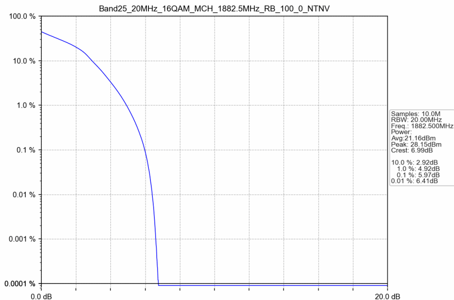
Band25_20MHz_16QAM_MCH_1882.5MHz_RB_100_0_NTNV
