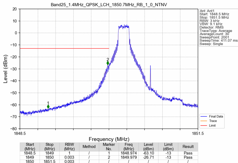
Band25_1.4MHz_QPSK_LCH_1850.7MHz_RB_1_0_NTNV
