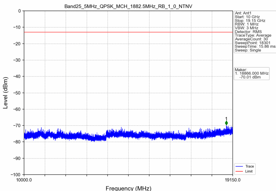
Band25_5MHz_QPSK_MCH_1882.5MHz_RB_1_0_NTNV
