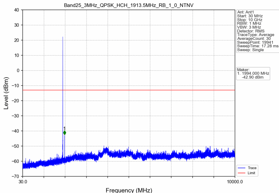
Band25_3MHz_QPSK_HCH_1913.5MHz_RB_1_0_NTNV
