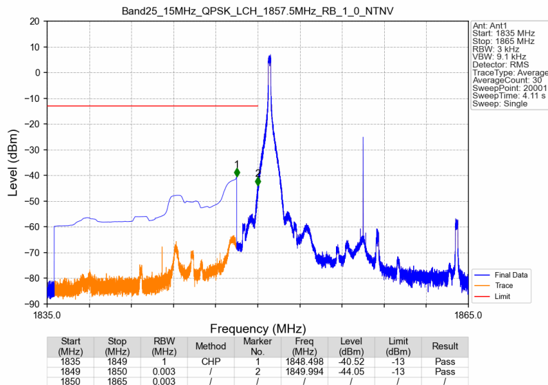
Band25_15MHz_QPSK_LCH_1857.5MHz_RB_1_0_NTNV
