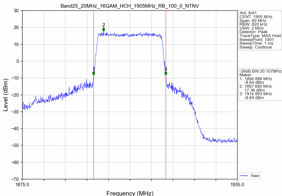
Band25_20MHz_16QAM_HCH_1905MHz_RB_100_0_NTNV
