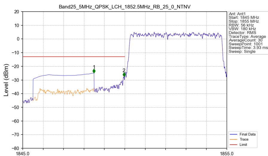
Band25_5MHz_QPSK_LCH_1852.5MHz_RB_25_0_NTNV
