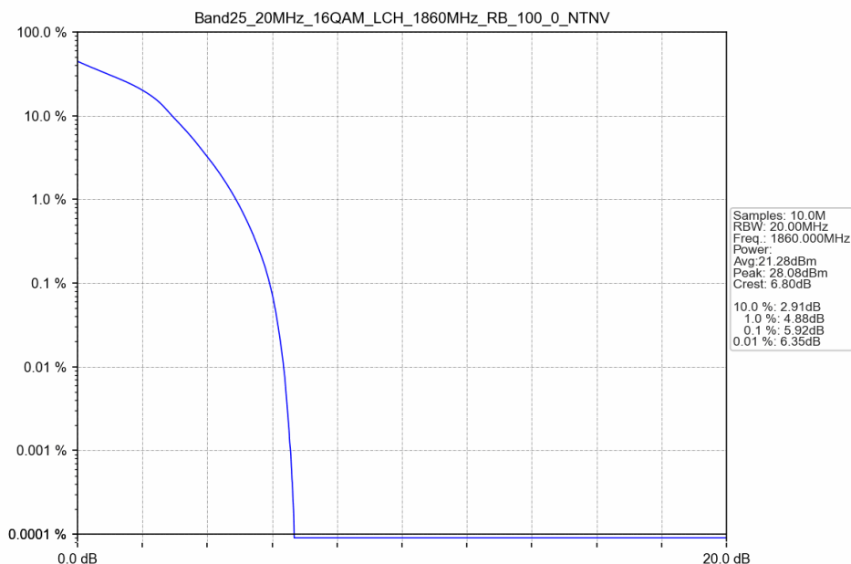
Band25_20MHz_16QAM_LCH_1860MHz_RB_100_0_NTNV
