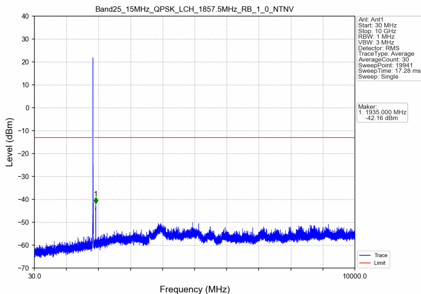
Band25_15MHz_QPSK_LCH_1857.5MHz_RB_1_0_NTNV
