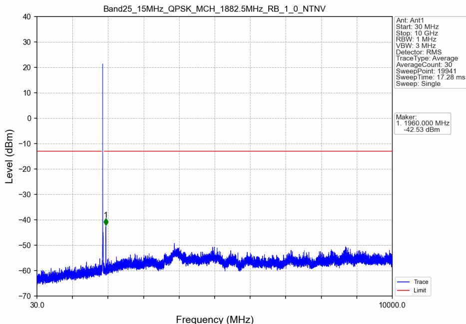
Band25_15MHz_QPSK_MCH_1882.5MHz_RB_1_0_NTNV
