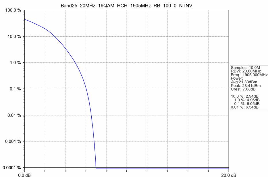
Band25_20MHz_16QAM_HCH_1905MHz_RB_100_0_NTNV
