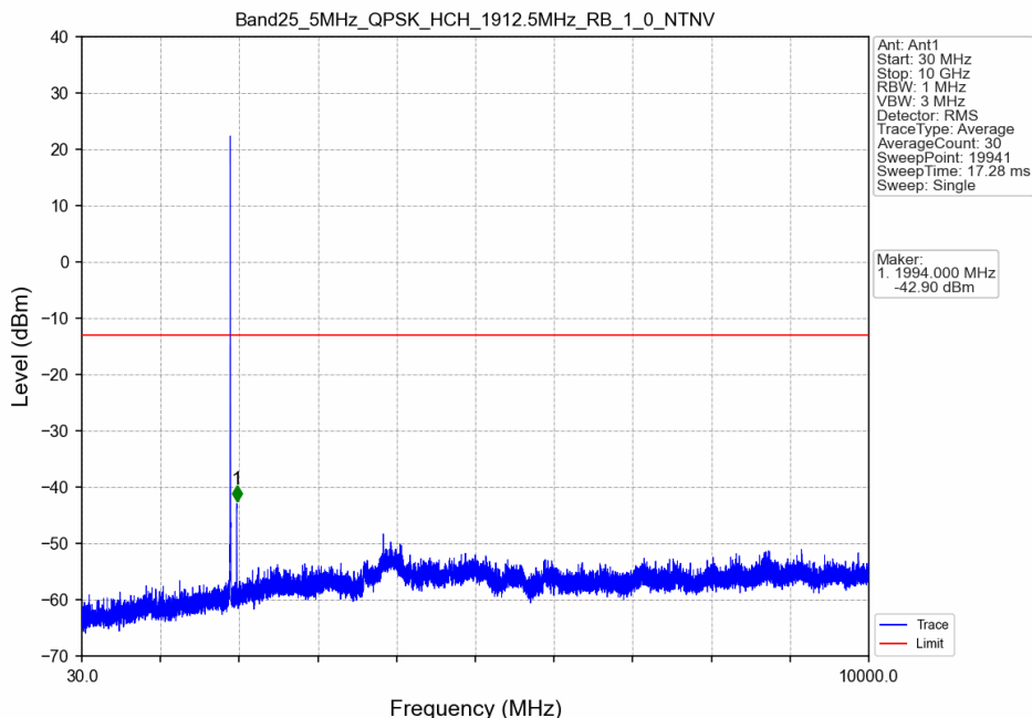
Band25_5MHz_QPSK_HCH_1912.5MHz_RB_1_0_NTNV
