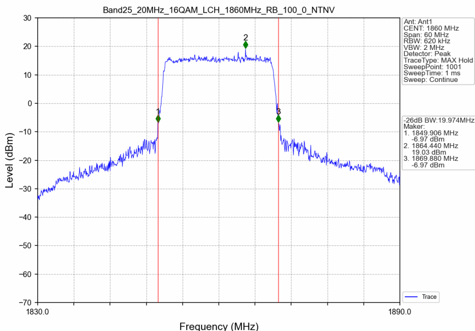
Band25_20MHz_16QAM_LCH_1860MHz_RB_100_0_NTNV
