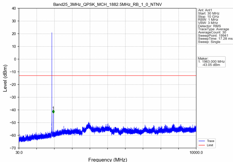
Band25_3MHz_QPSK_MCH_1882.5MHz_RB_1_0_NTNV
