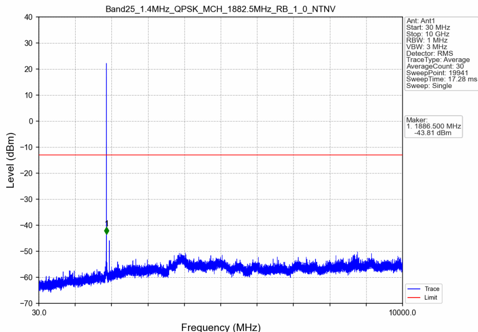
Band25_1.4MHz_QPSK_MCH_1882.5MHz_RB_1_0_NTNV
