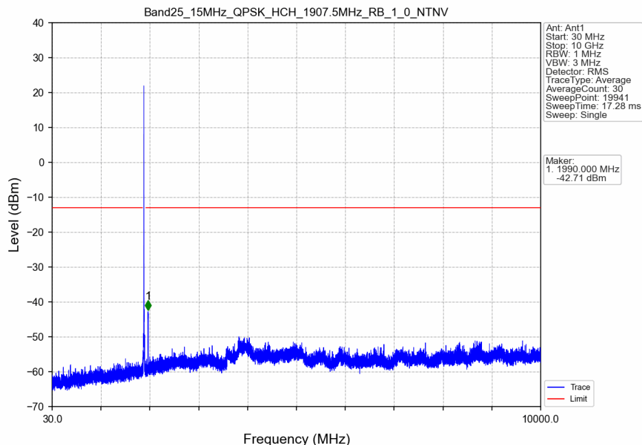
Band25_15MHz_QPSK_HCH_1907.5MHz_RB_1_0_NTNV
