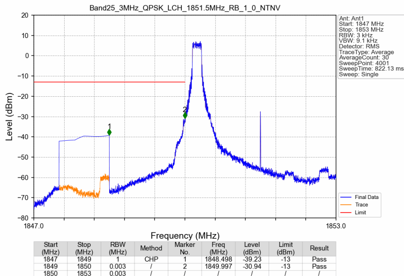
Band25_3MHz_QPSK_LCH_1851.5MHz_RB_1_0_NTNV
