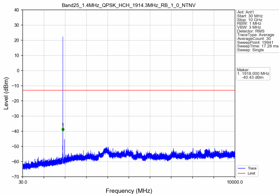
Band25_1.4MHz_QPSK_HCH_1914.3MHz_RB_1_0_NTNV
