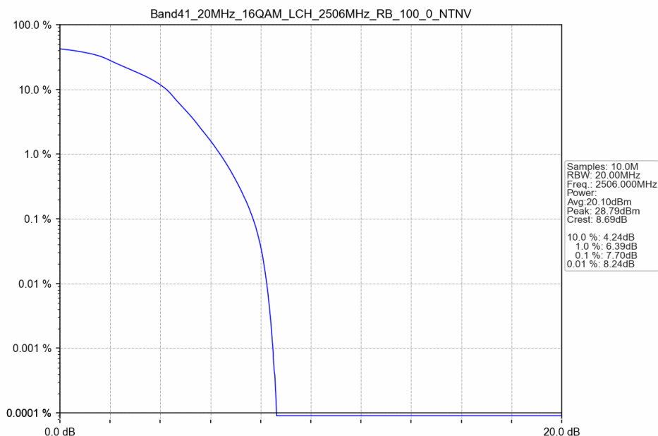
Band41_20MHz_16QAM_LCH_2506MHz_RB_100_0_NTNV
