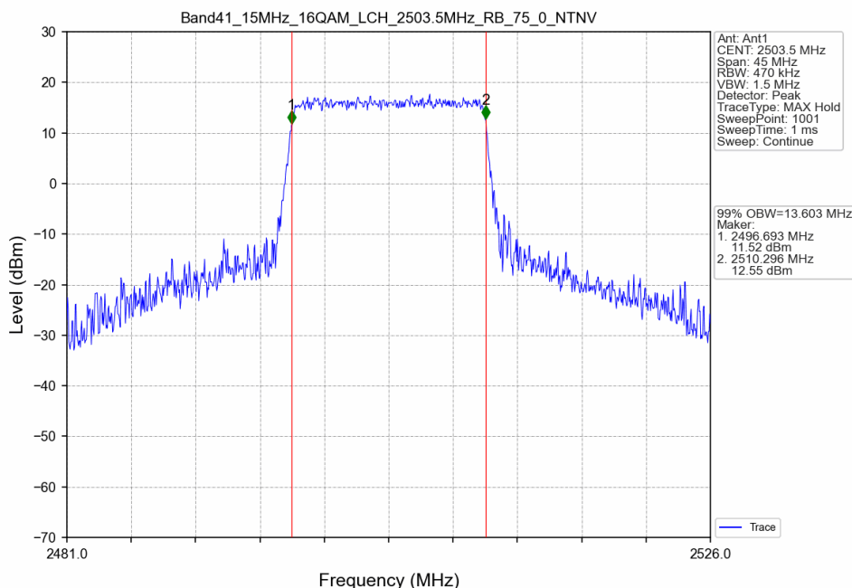
Band41_15MHz_16QAM_LCH_2503.5MHz_RB_75_0_NTNV
