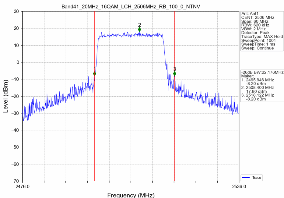
Band41_20MHz_16QAM_LCH_2506MHz_RB_100_0_NTNV
