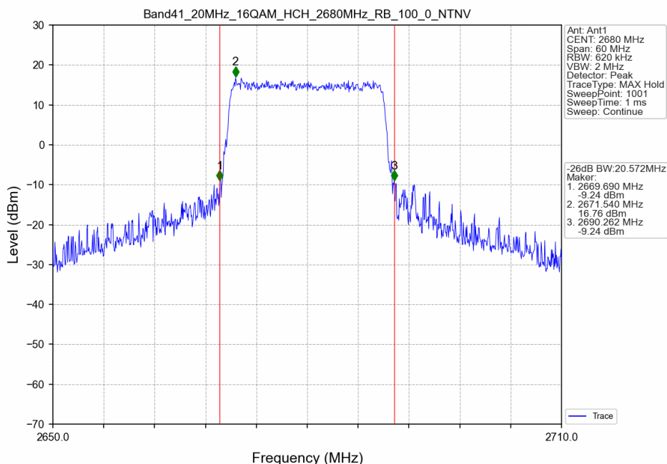
Band41_20MHz_16QAM_HCH_2680MHz_RB_100_0_NTNV
