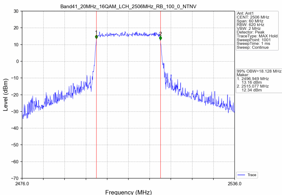
Band41_20MHz_16QAM_LCH_2506MHz_RB_100_0_NTNV
