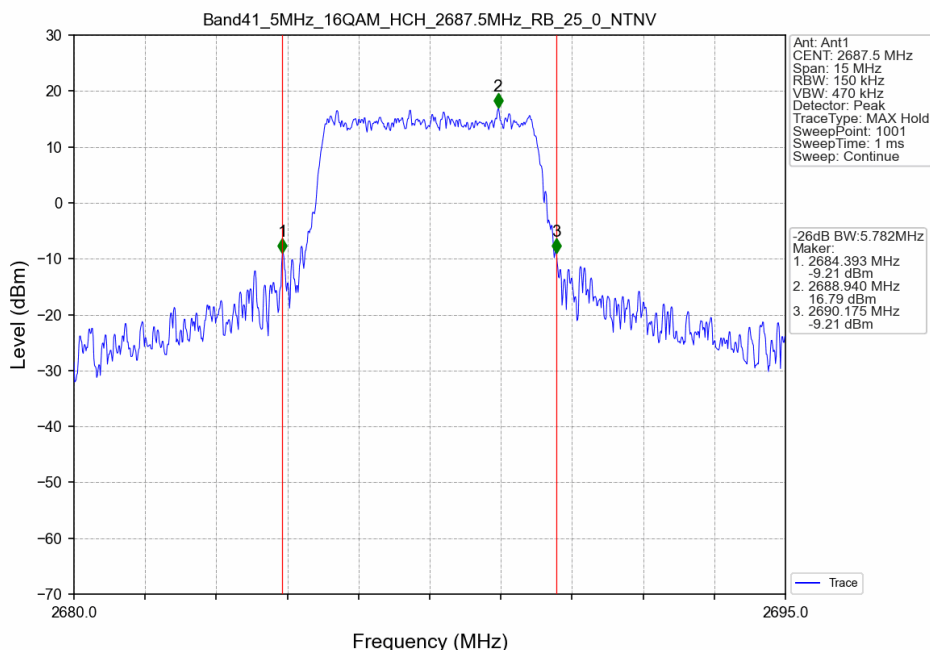
Band41_5MHz_16QAM_HCH_2687.5MHz_RB_25_0_NTNV
