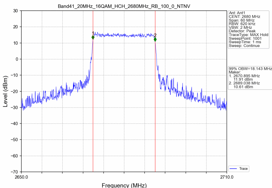
Band41_20MHz_16QAM_HCH_2680MHz_RB_100_0_NTNV
