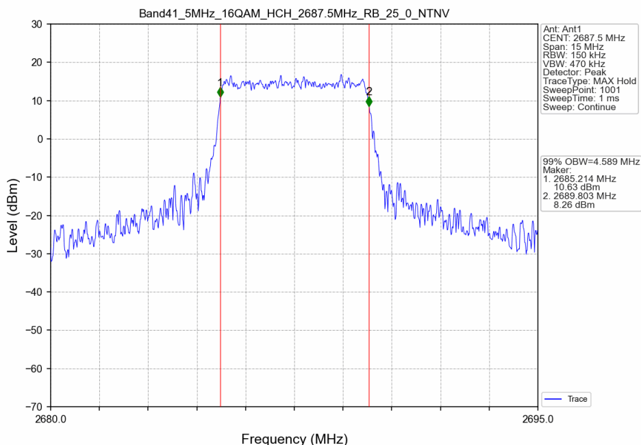
Band41_5MHz_16QAM_HCH_2687.5MHz_RB_25_0_NTNV
