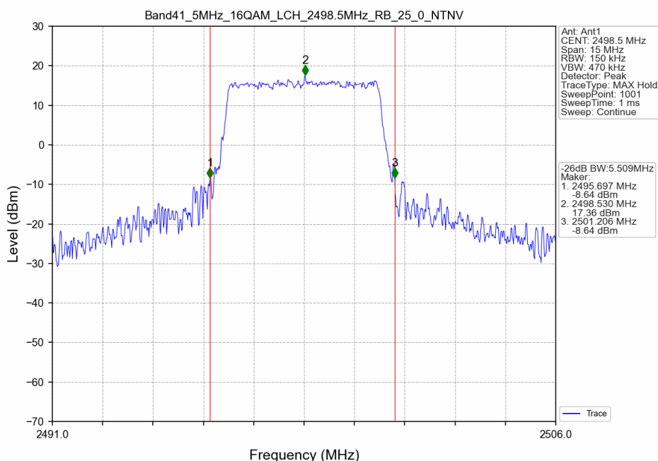
Band41_5MHz_16QAM_LCH_2498.5MHz_RB_25_0_NTNV
