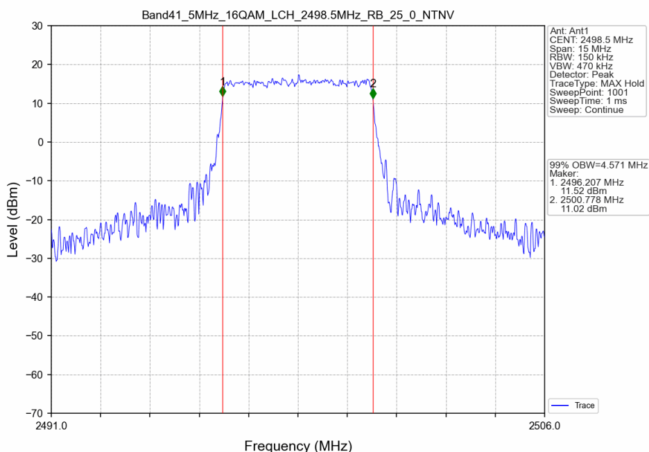
Band41_5MHz_16QAM_LCH_2498.5MHz_RB_25_0_NTNV
