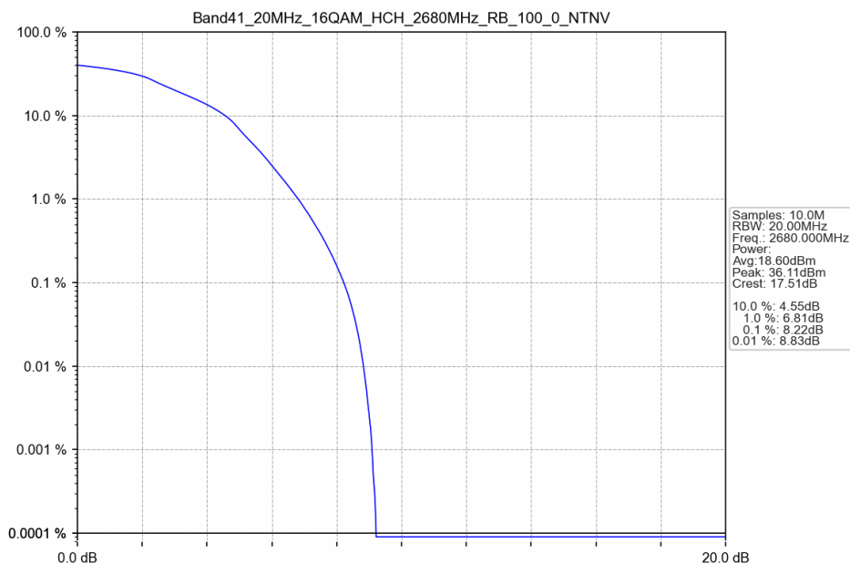
Band41_20MHz_16QAM_HCH_2680MHz_RB_100_0_NTNV
