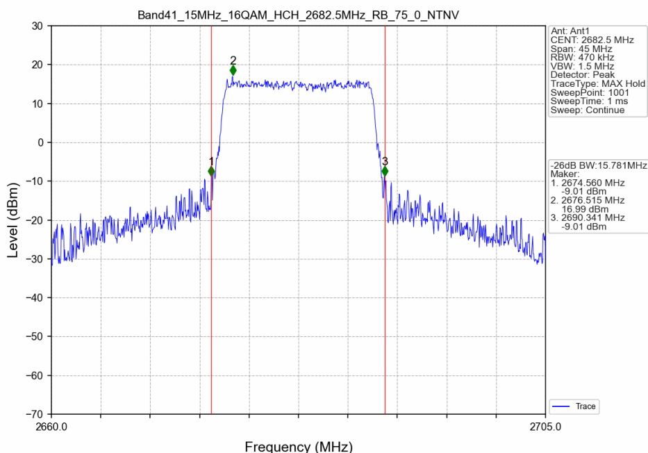
Band41_15MHz_16QAM_HCH_2682.5MHz_RB_75_0_NTNV
