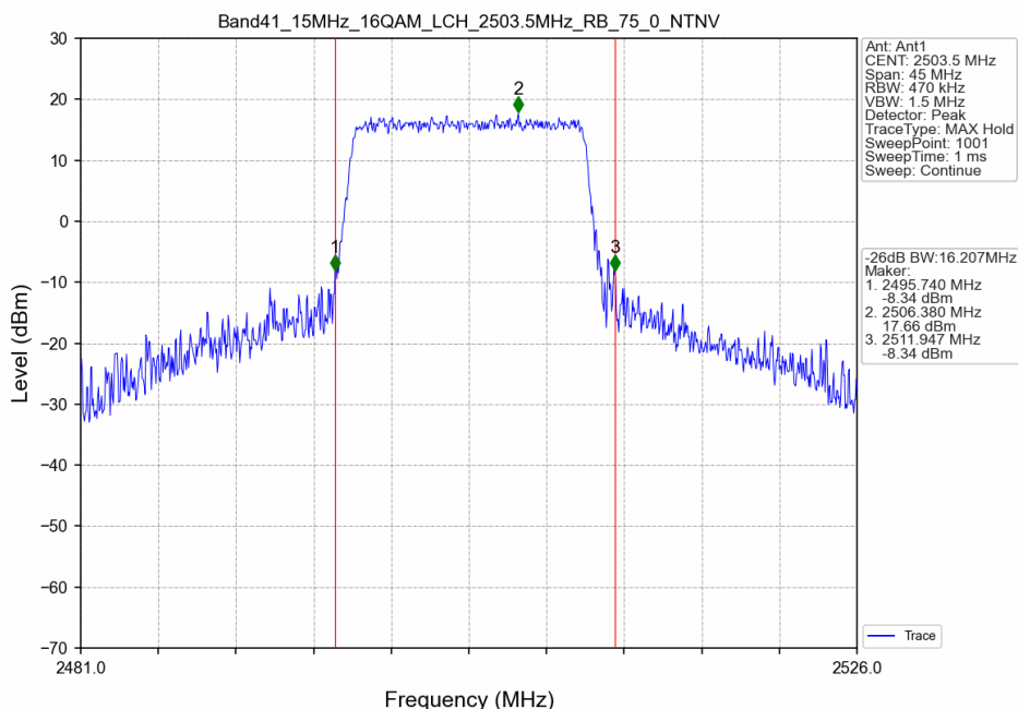
Band41_15MHz_16QAM_LCH_2503.5MHz_RB_75_0_NTNV
