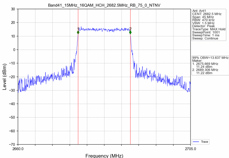
Band41_15MHz_16QAM_HCH_2682.5MHz_RB_75_0_NTNV
