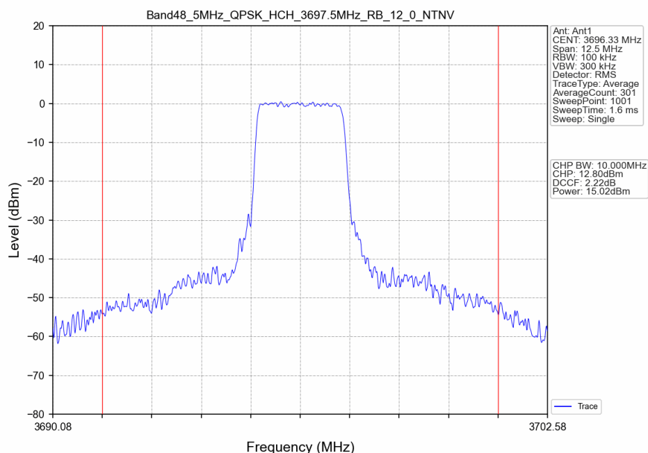
Band48_5MHz_QPSK_HCH_3697.5MHz_RB_12_0_NTNV
