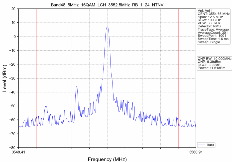
Band48_5MHz_16QAM_LCH_3552.5MHz_RB_1_24_NTNV
