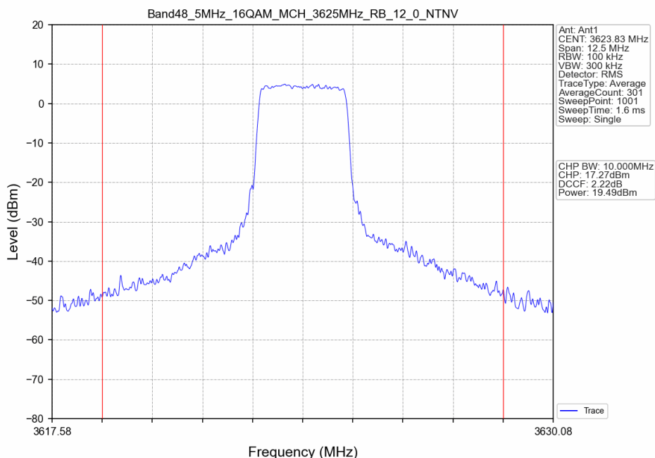
Band48_5MHz_16QAM_MCH_3625MHz_RB_12_0_NTNV
