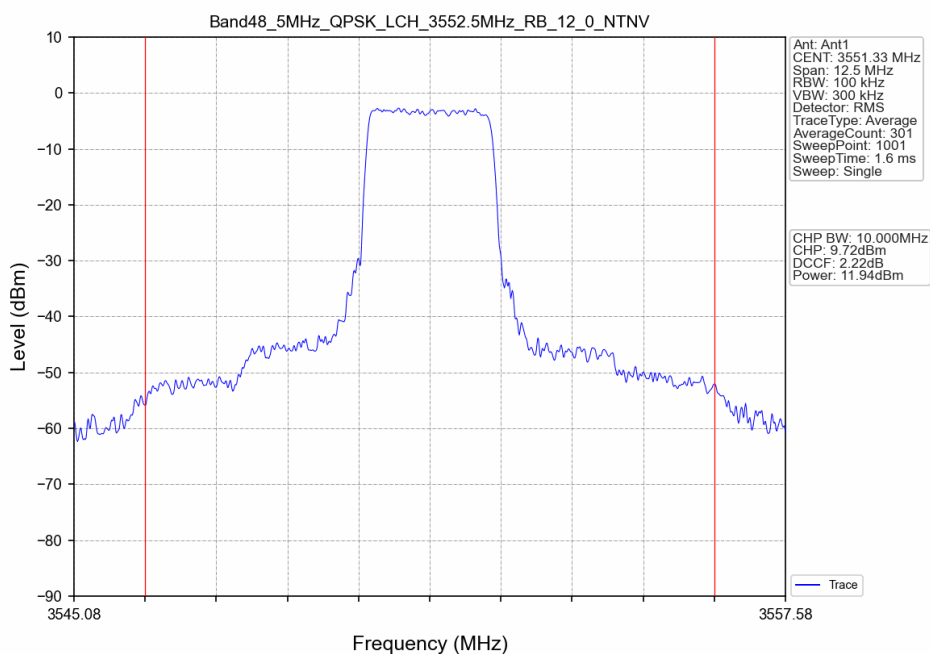
Band48_5MHz_QPSK_LCH_3552.5MHz_RB_12_0_NTNV
