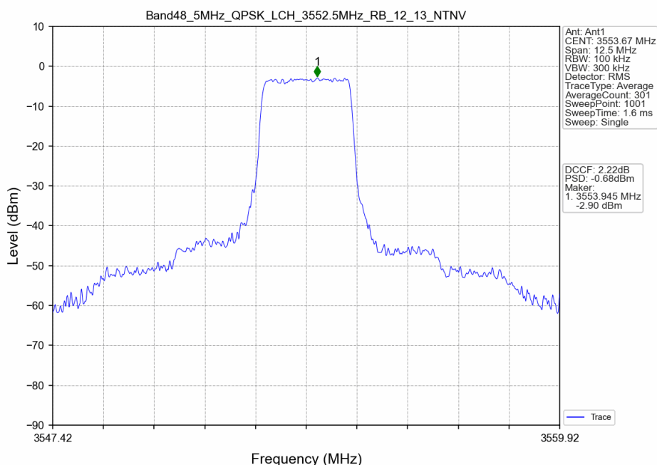
Band48_5MHz_QPSK_LCH_3552.5MHz_RB_12_13_NTNV
