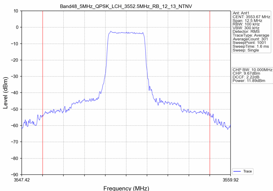
Band48_5MHz_QPSK_LCH_3552.5MHz_RB_12_13_NTNV
