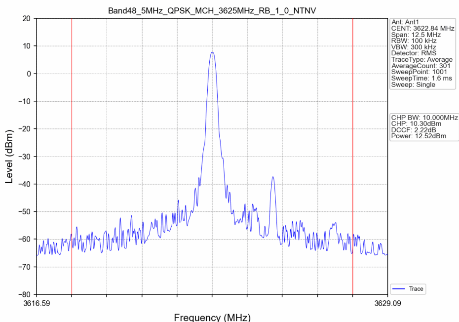
Band48_5MHz_QPSK_MCH_3625MHz_RB_1_0_NTNV
