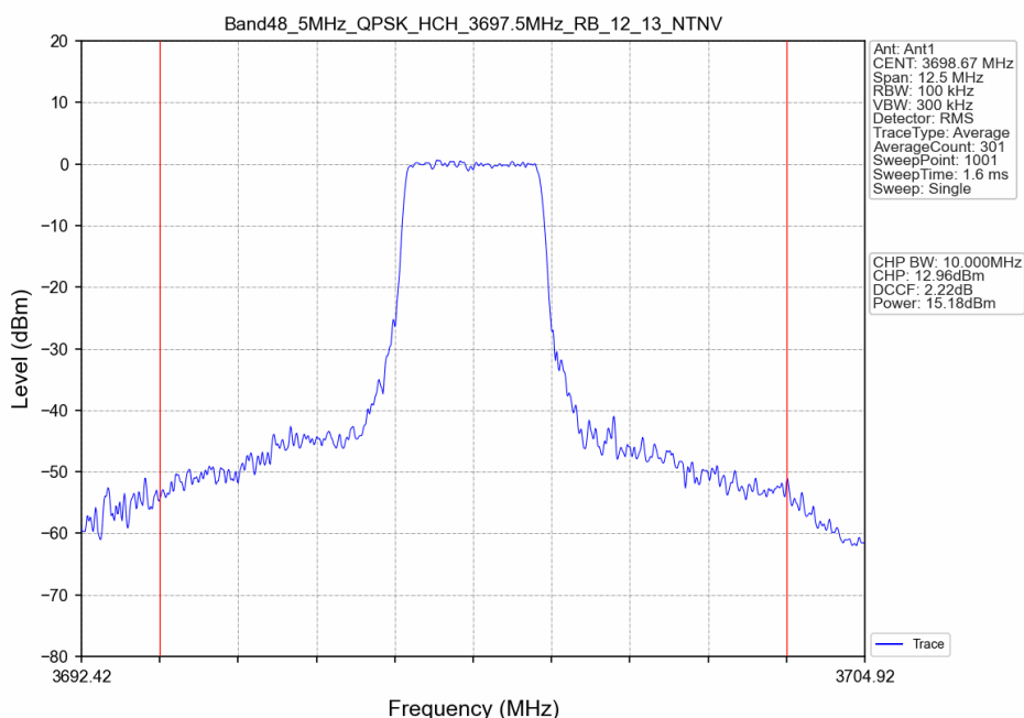
Band48_5MHz_QPSK_HCH_3697.5MHz_RB_12_13_NTNV
