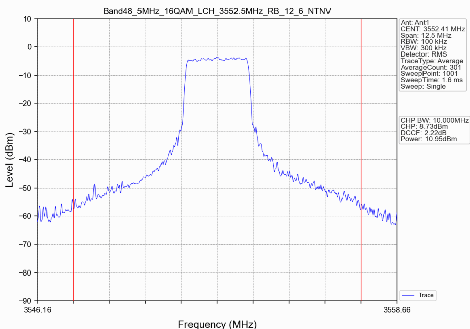
Band48_5MHz_16QAM_LCH_3552.5MHz_RB_12_6_NTNV
