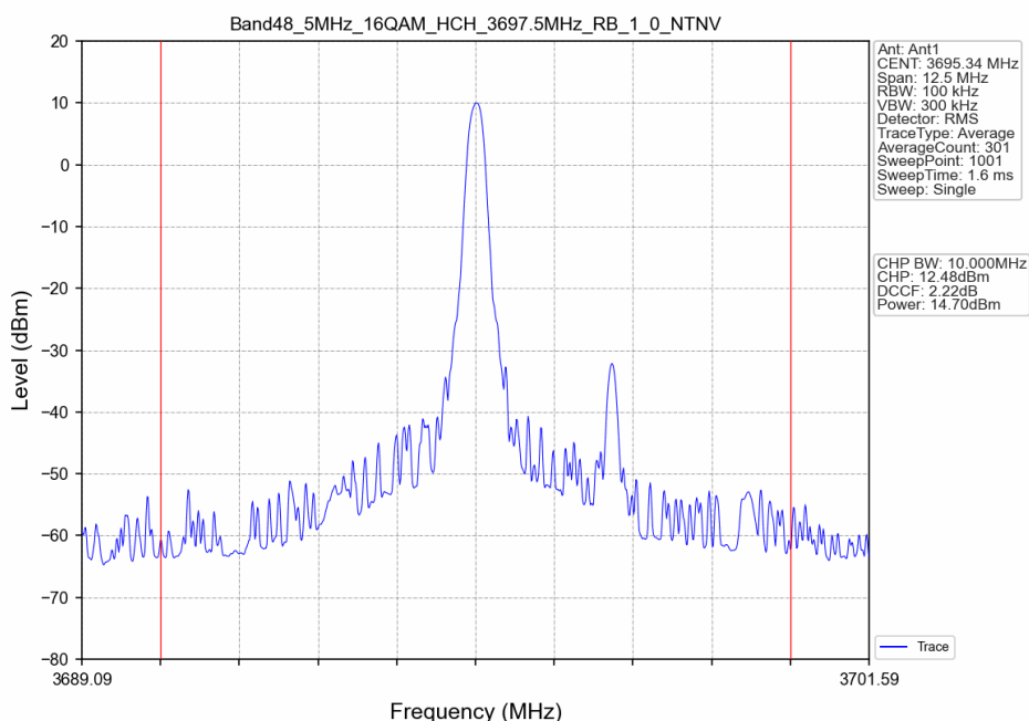
Band48_5MHz_16QAM_HCH_3697.5MHz_RB_1_0_NTNV
