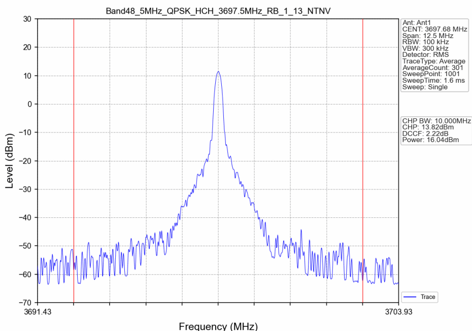
Band48_5MHz_QPSK_HCH_3697.5MHz_RB_1_13_NTNV
