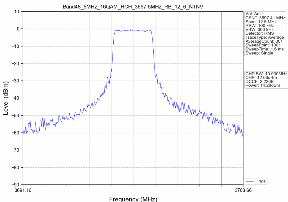
Band48_5MHz_16QAM_HCH_3697.5MHz_RB_12_6_NTNV
