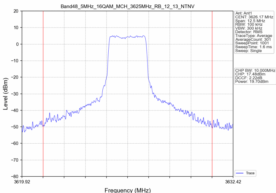
Band48_5MHz_16QAM_MCH_3625MHz_RB_12_13_NTNV
