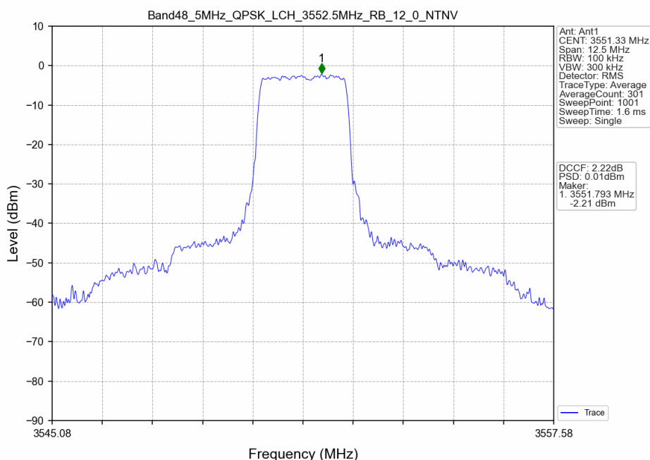
Band48_5MHz_QPSK_LCH_3552.5MHz_RB_12_0_NTNV
