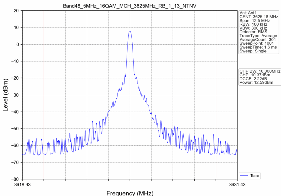
Band48_5MHz_16QAM_MCH_3625MHz_RB_1_13_NTNV
