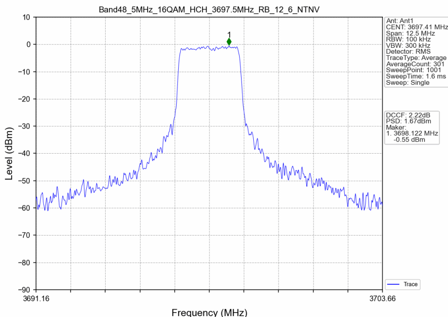
Band48_5MHz_16QAM_HCH_3697.5MHz_RB_12_6_NTNV
