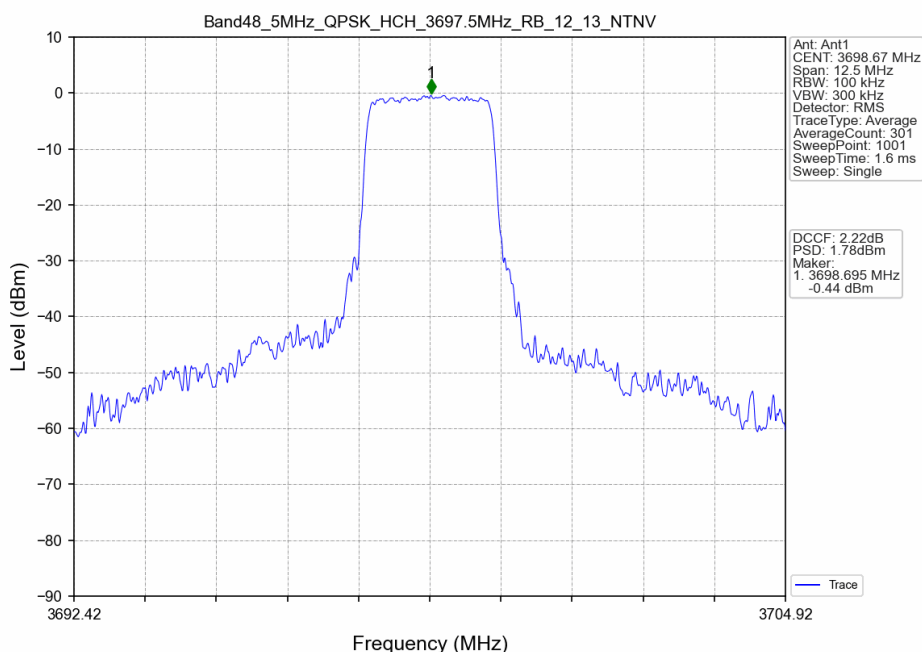
Band48_5MHz_QPSK_HCH_3697.5MHz_RB_12_13_NTNV
