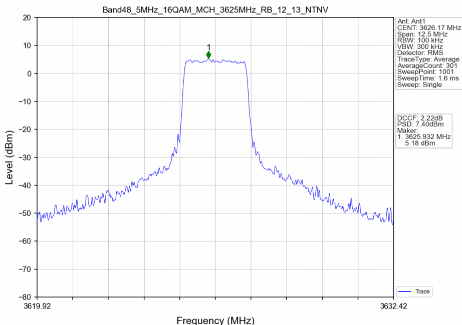
Band48_5MHz_16QAM_MCH_3625MHz_RB_12_13_NTNV
