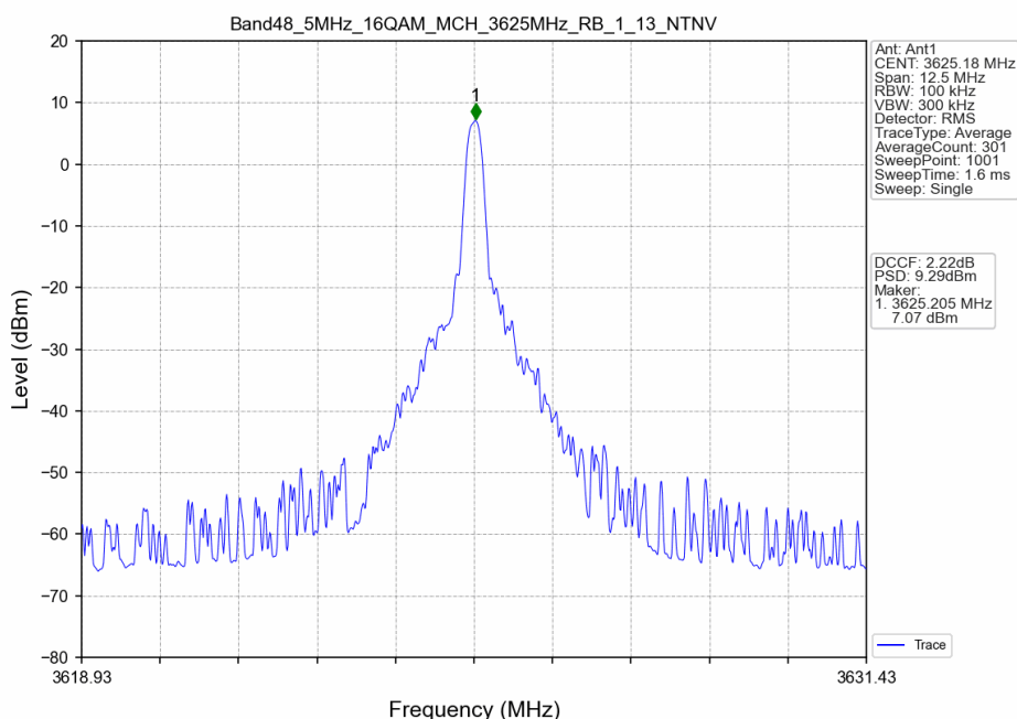
Band48_5MHz_16QAM_MCH_3625MHz_RB_1_13_NTNV
