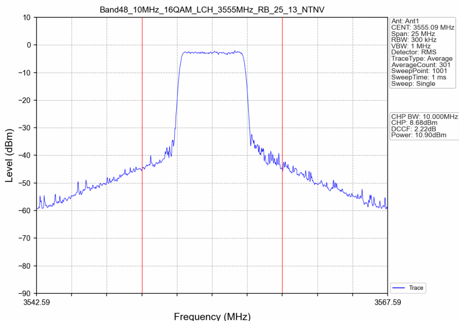
Band48_10MHz_16QAM_LCH_3555MHz_RB_25_13_NTNV
