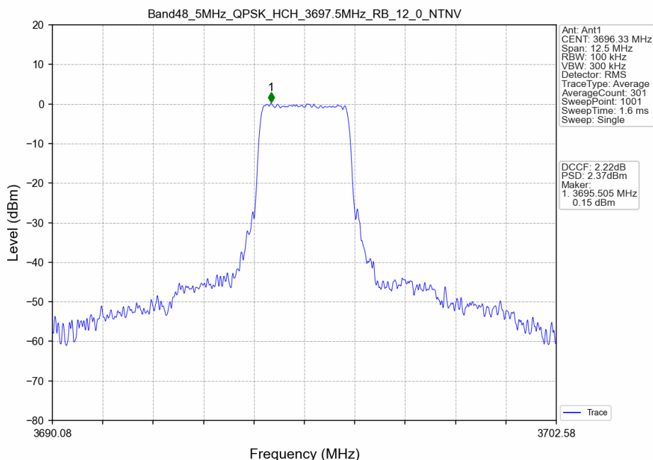
Band48_5MHz_QPSK_HCH_3697.5MHz_RB_12_0_NTNV
