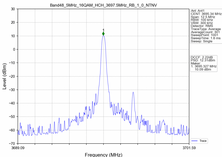
Band48_5MHz_16QAM_HCH_3697.5MHz_RB_1_0_NTNV
