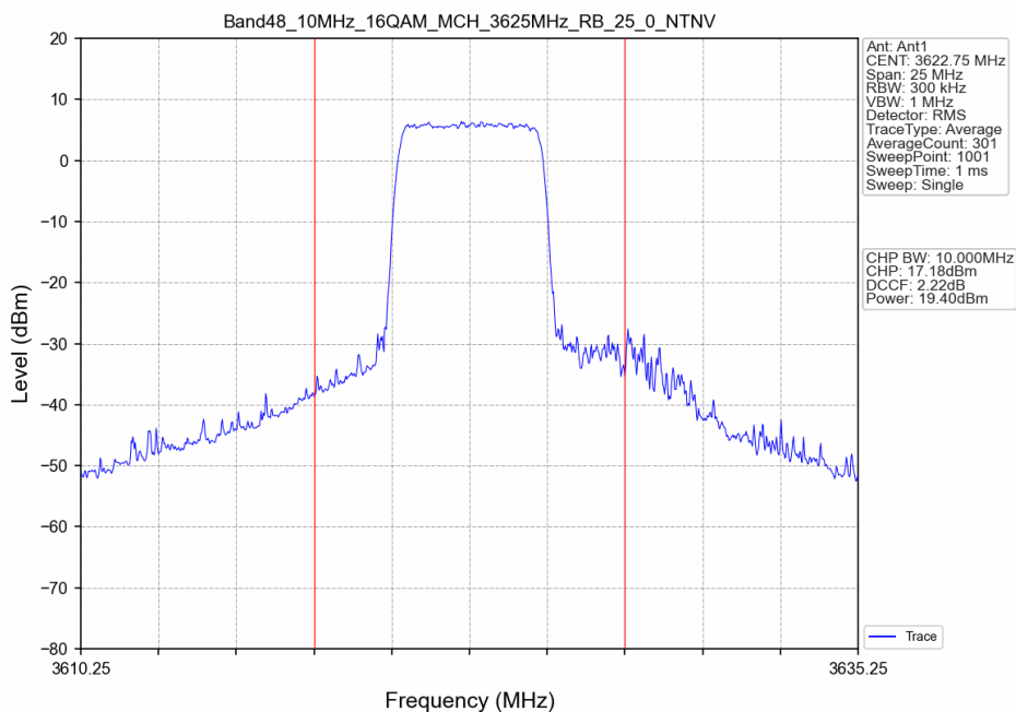
Band48_10MHz_16QAM_MCH_3625MHz_RB_25_0_NTNV
