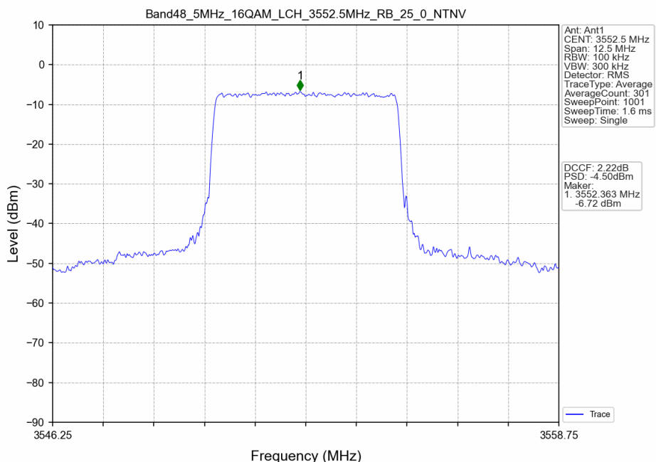
Band48_5MHz_16QAM_LCH_3552.5MHz_RB_25_0_NTNV
