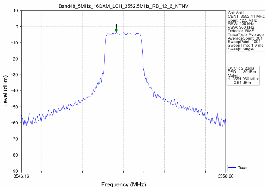
Band48_5MHz_16QAM_LCH_3552.5MHz_RB_12_6_NTNV
