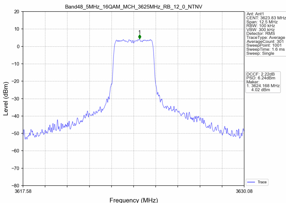
Band48_5MHz_16QAM_MCH_3625MHz_RB_12_0_NTNV
