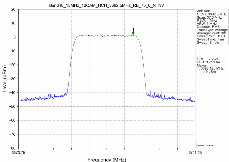
Band48_15MHz_16QAM_HCH_3692.5MHz_RB_75_0_NTNV
