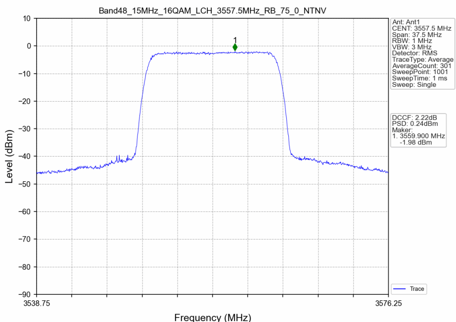
Band48_15MHz_16QAM_LCH_3557.5MHz_RB_75_0_NTNV
