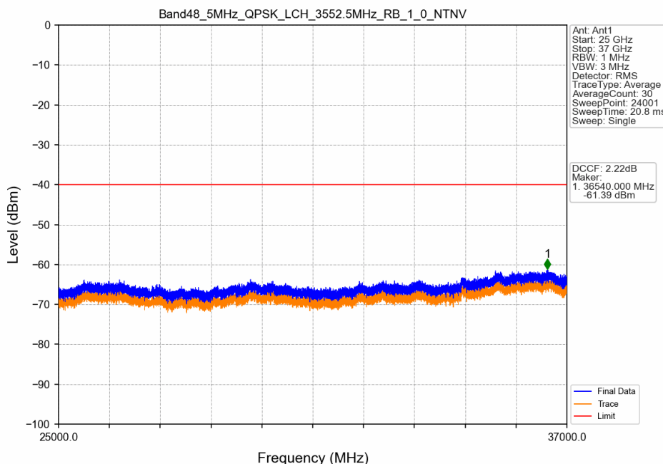
Band48_5MHz_QPSK_LCH_3552.5MHz_RB_1_0_NTNV
