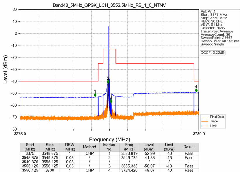
Band48_5MHz_QPSK_LCH_3552.5MHz_RB_1_0_NTNV
