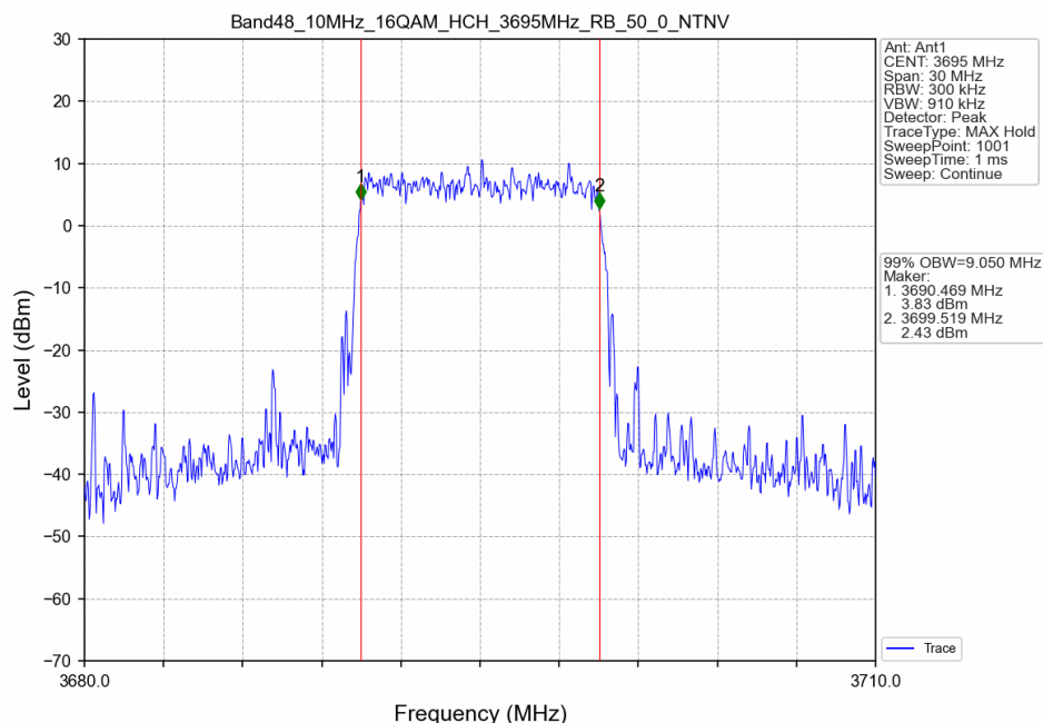
Band48_10MHz_16QAM_HCH_3695MHz_RB_50_0_NTNV
