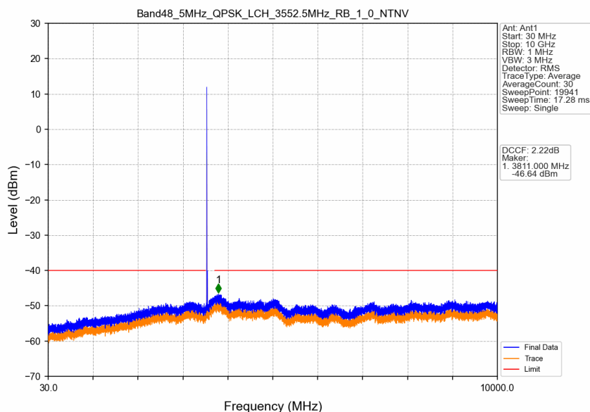
Band48_5MHz_QPSK_LCH_3552.5MHz_RB_1_0_NTNV
