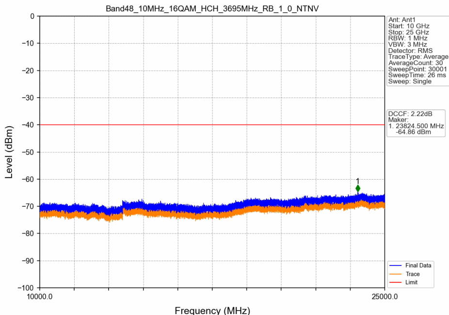
Band48_10MHz_16QAM_HCH_3695MHz_RB_1_0_NTNV
