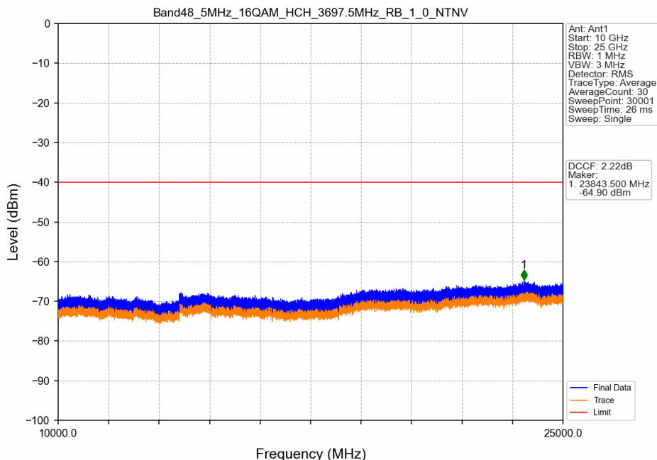
Band48_5MHz_16QAM_HCH_3697.5MHz_RB_1_0_NTNV
