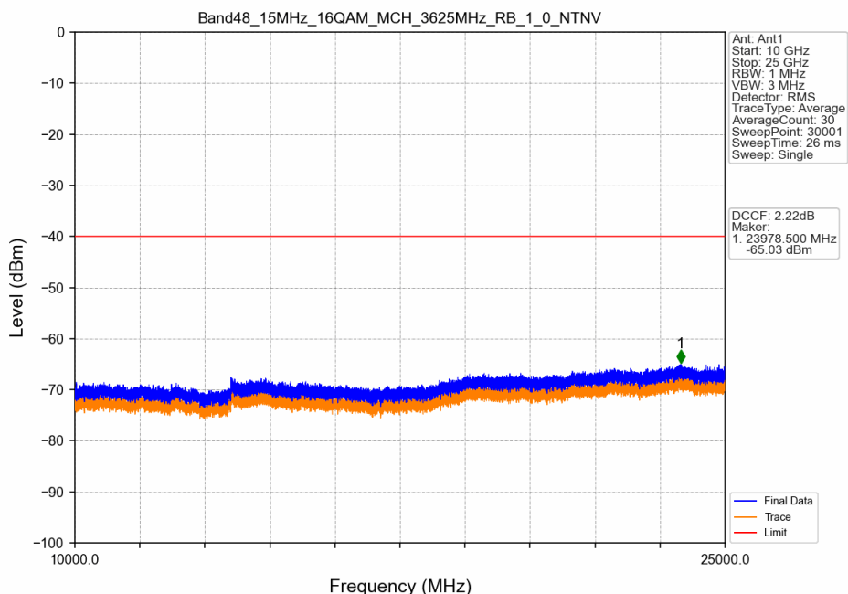
Band48_15MHz_16QAM_MCH_3625MHz_RB_1_0_NTNV
