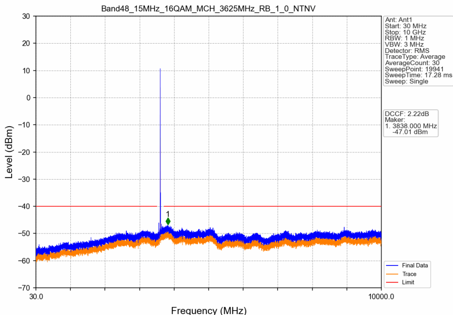
Band48_15MHz_16QAM_MCH_3625MHz_RB_1_0_NTNV
