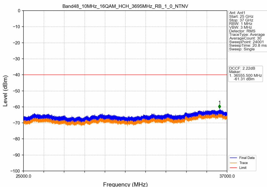
Band48_10MHz_16QAM_HCH_3695MHz_RB_1_0_NTNV
