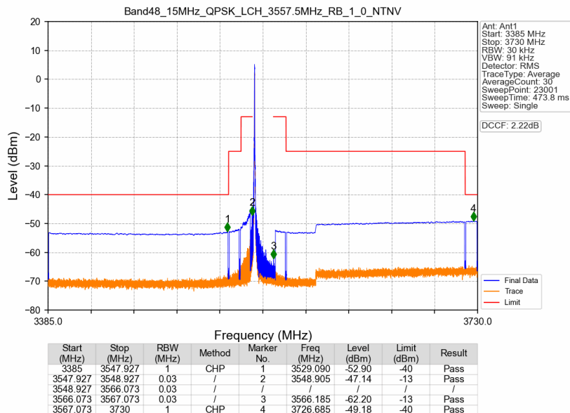
Band48_15MHz_QPSK_LCH_3557.5MHz_RB_1_0_NTNV
