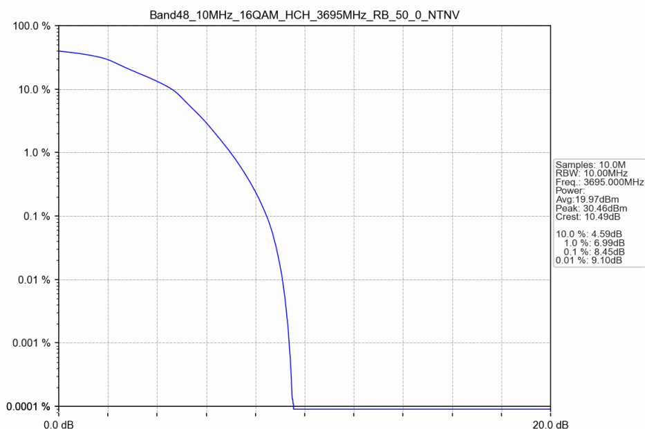
Band48_10MHz_16QAM_HCH_3695MHz_RB_50_0_NTNV
