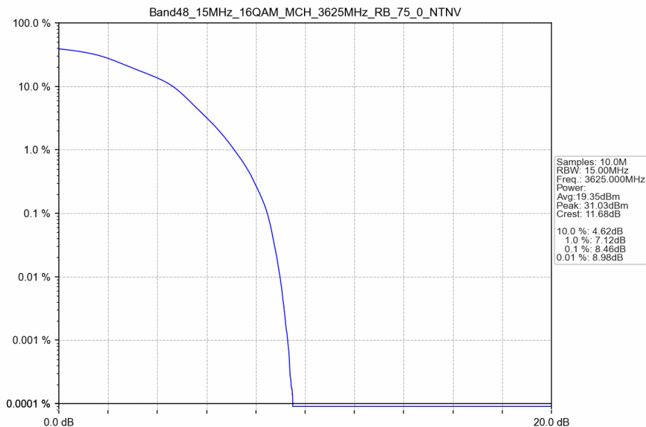
Band48_15MHz_16QAM_MCH_3625MHz_RB_75_0_NTNV
