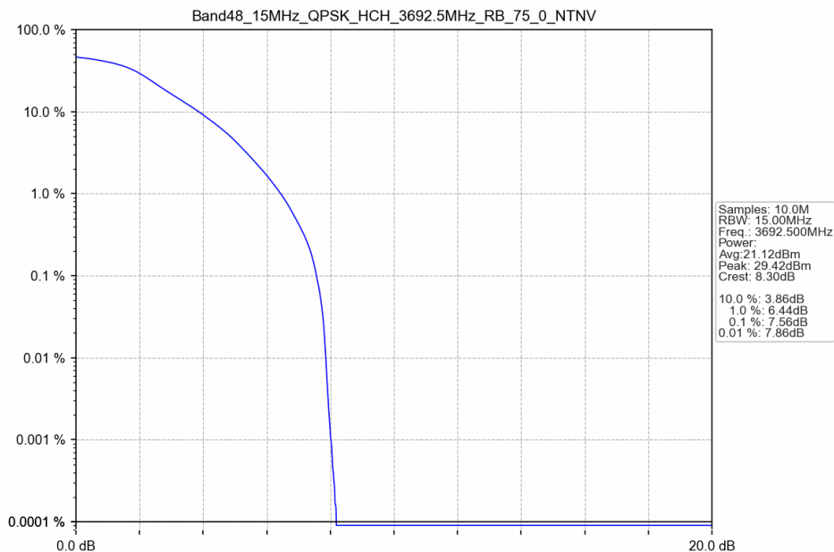
Band48_15MHz_QPSK_HCH_3692.5MHz_RB_75_0_NTNV
