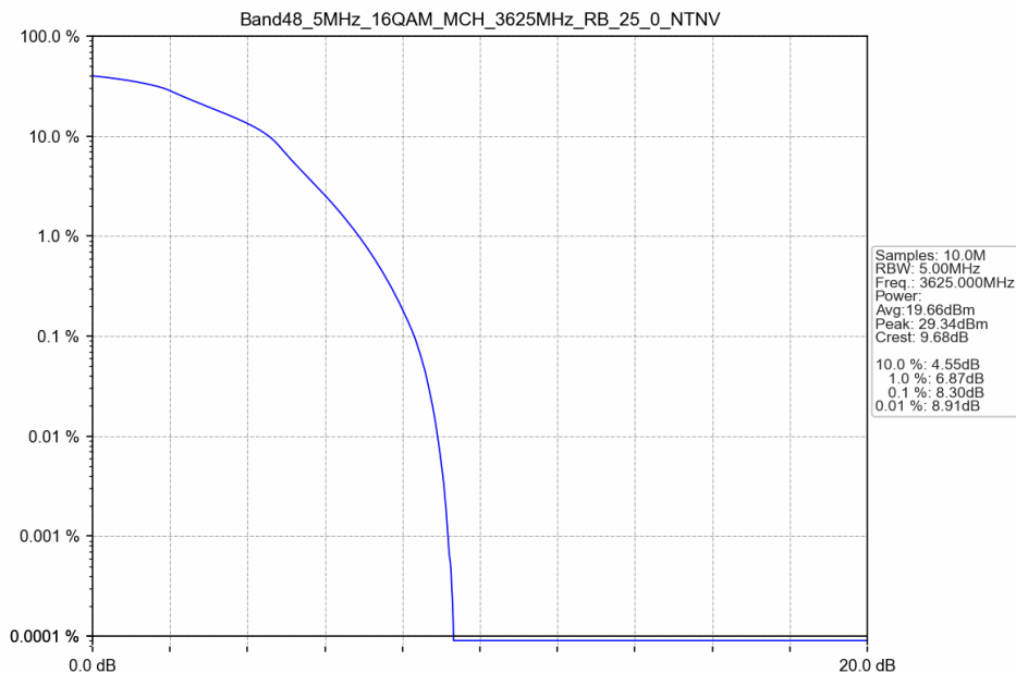
Band48_5MHz_16QAM_MCH_3625MHz_RB_25_0_NTNV
