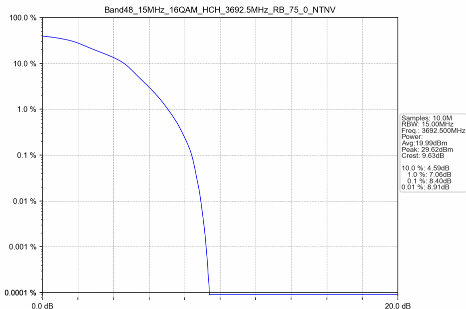
Band48_15MHz_16QAM_HCH_3692.5MHz_RB_75_0_NTNV
