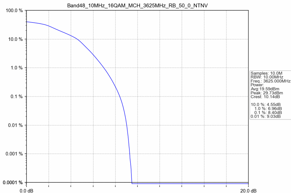
Band48_10MHz_16QAM_MCH_3625MHz_RB_50_0_NTNV
