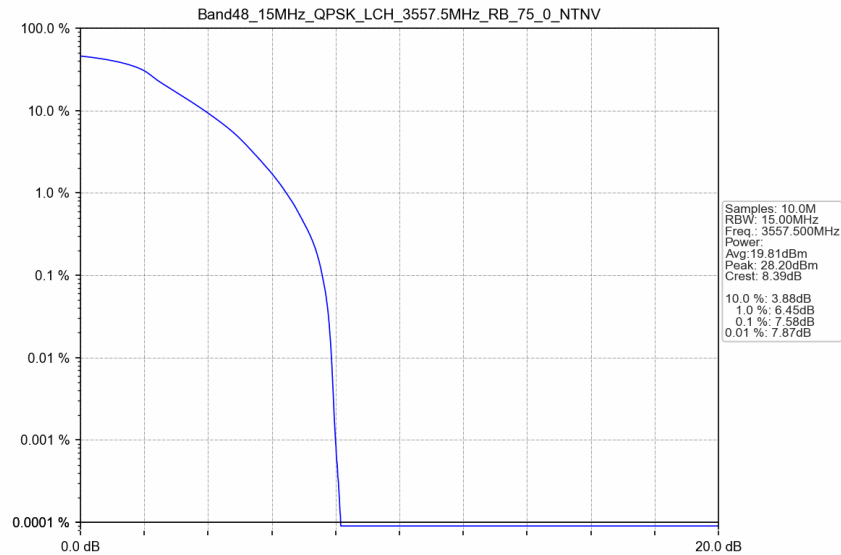
Band48_15MHz_QPSK_LCH_3557.5MHz_RB_75_0_NTNV
