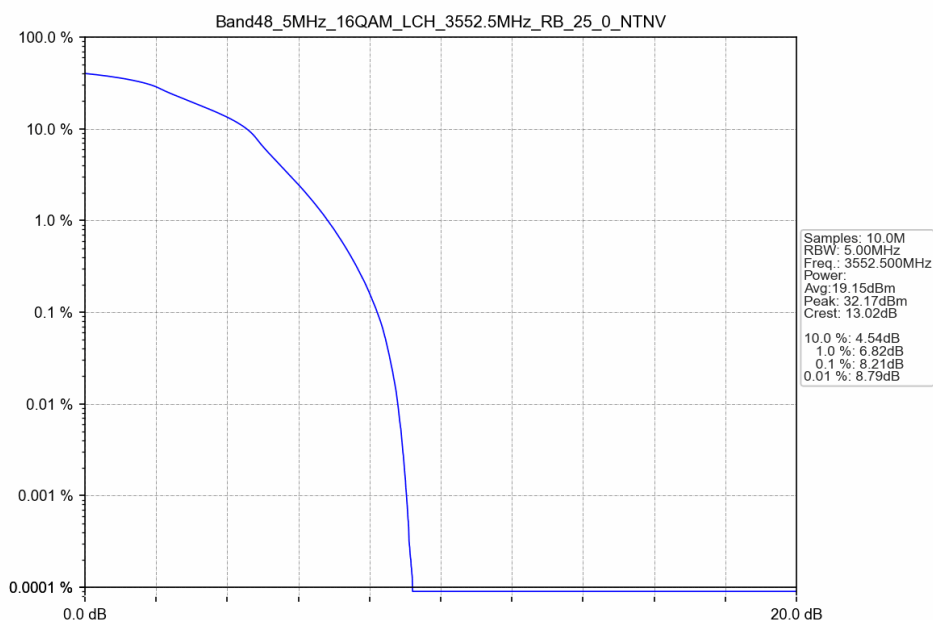
Band48_5MHz_16QAM_LCH_3552.5MHz_RB_25_0_NTNV
