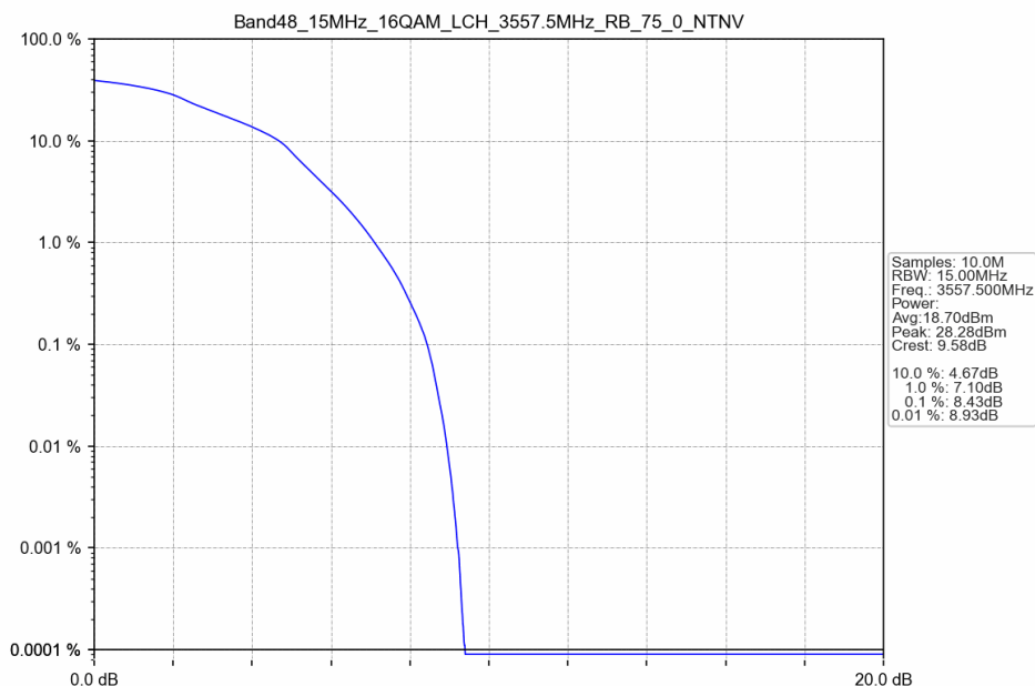
Band48_15MHz_16QAM_LCH_3557.5MHz_RB_75_0_NTNV
