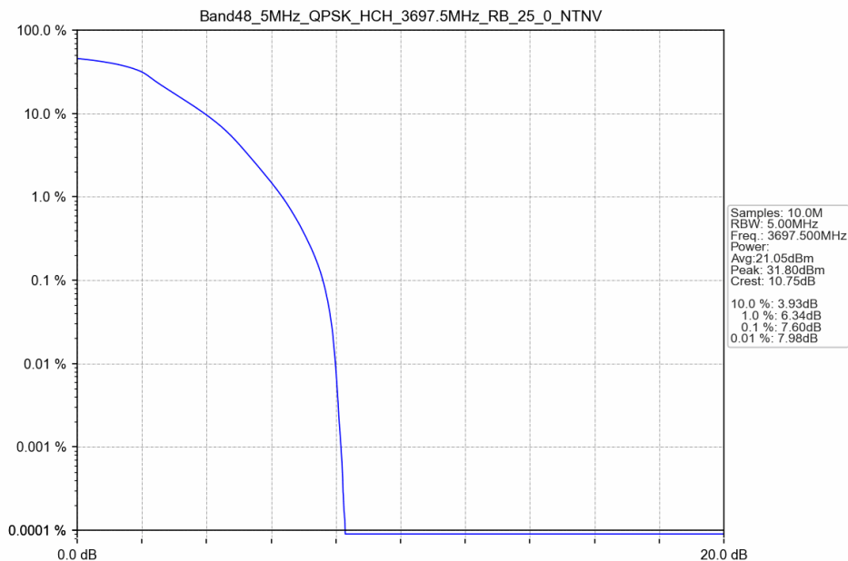
Band48_5MHz_QPSK_HCH_3697.5MHz_RB_25_0_NTNV
