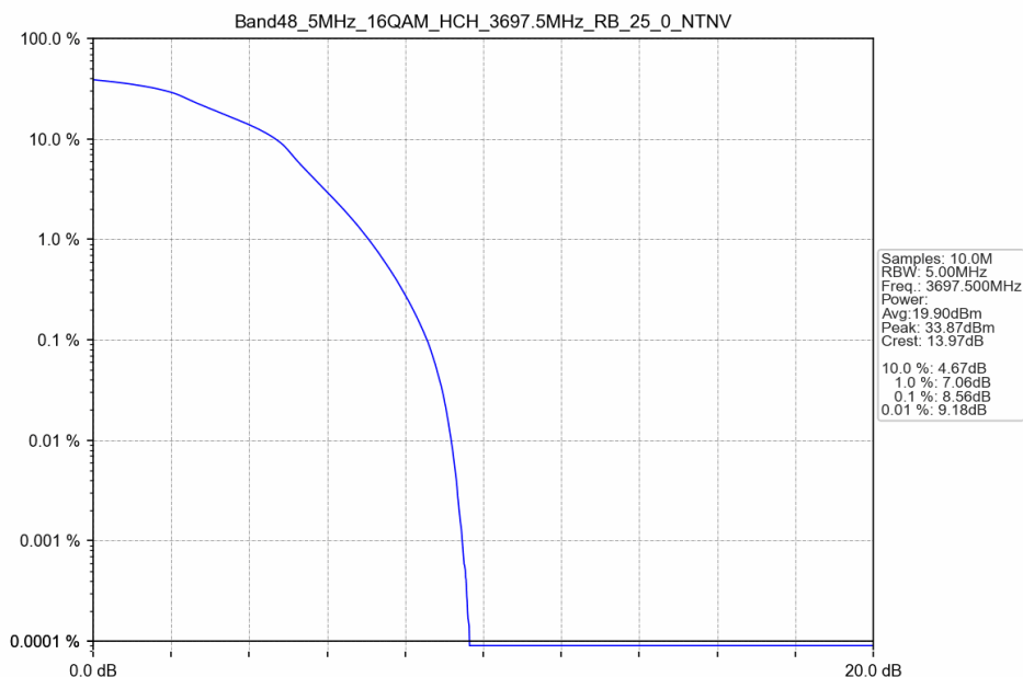
Band48_5MHz_16QAM_HCH_3697.5MHz_RB_25_0_NTNV
