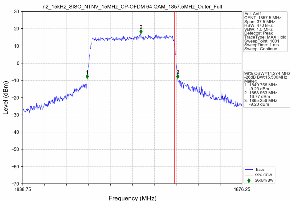
n2_15kHz_SISO_NTNV_15MHz_CP-OFDM 64 QAM_1857.5MHz_Outer_Full
