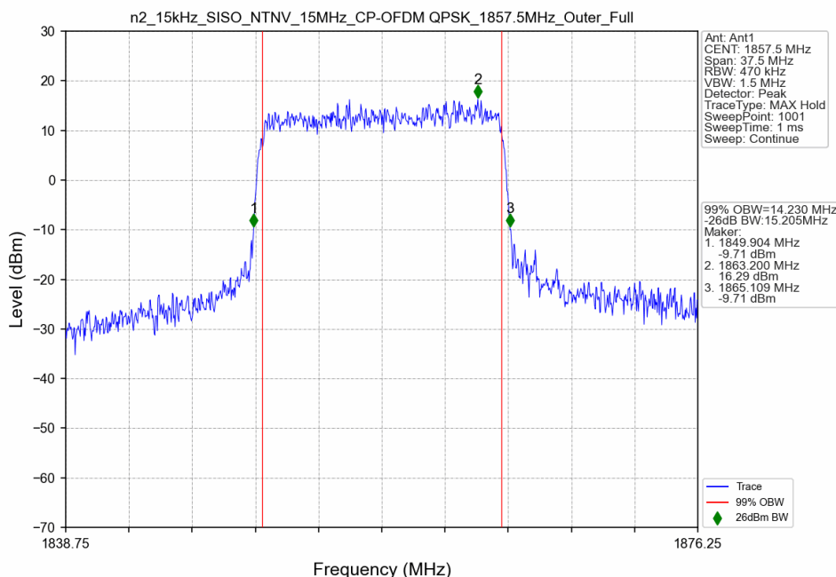
n2_15kHz_SISO_NTNV_15MHz_CP-OFDM QPSK_1857.5MHz_Outer_Full
