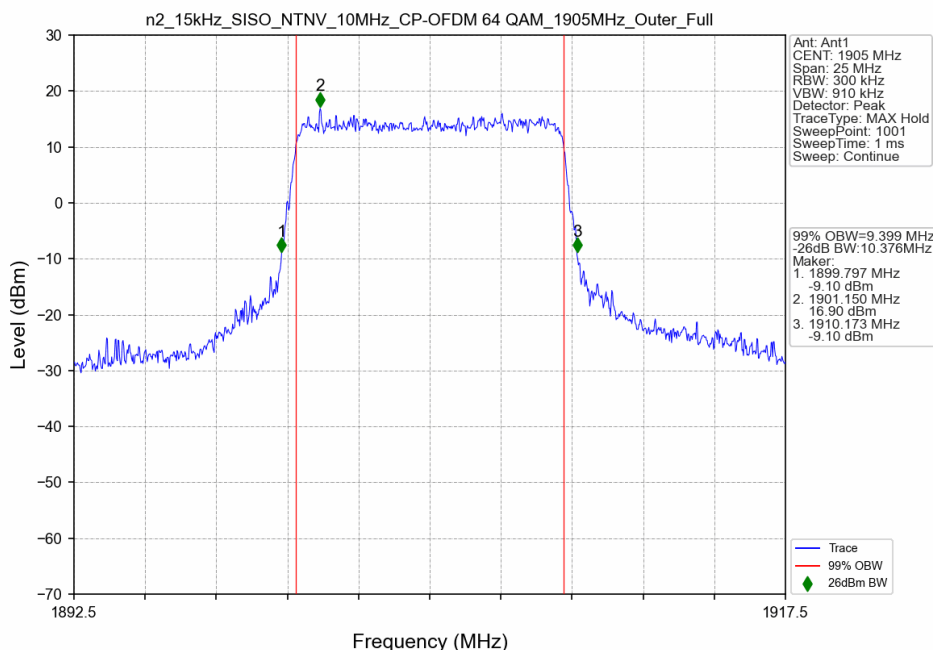
n2_15kHz_SISO_NTNV_10MHz_CP-OFDM 64 QAM_1905MHz_Outer_Full
