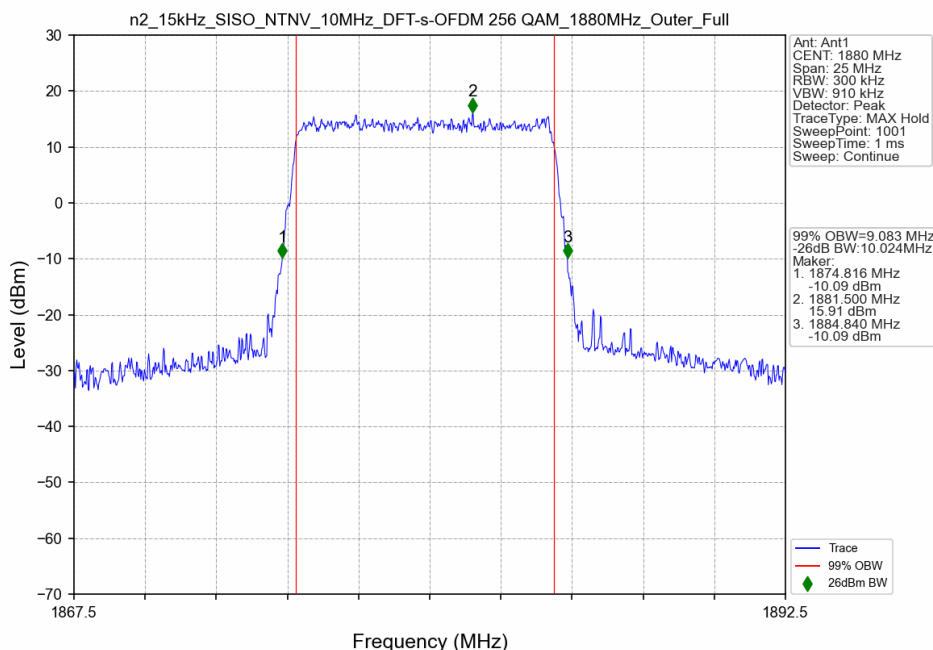
n2_15kHz_SISO_NTNV_10MHz_DFT-s-OFDM 256 QAM_1880MHz_Outer_Full
