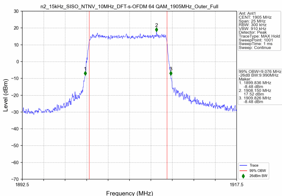
n2_15kHz_SISO_NTNV_10MHz_DFT-s-OFDM 64 QAM_1905MHz_Outer_Full
