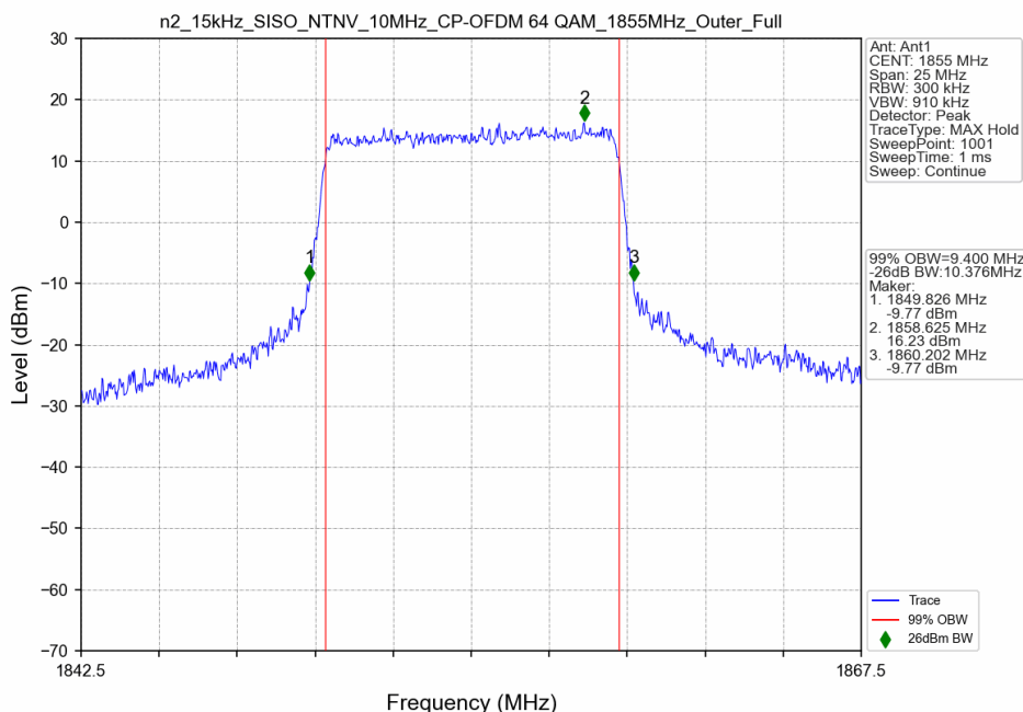
n2_15kHz_SISO_NTNV_10MHz_CP-OFDM 64 QAM_1855MHz_Outer_Full
