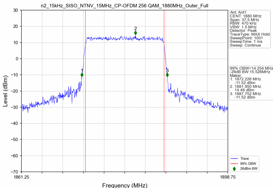
n2_15kHz_SISO_NTNV_15MHz_CP-OFDM 256 QAM_1880MHz_Outer_Full
