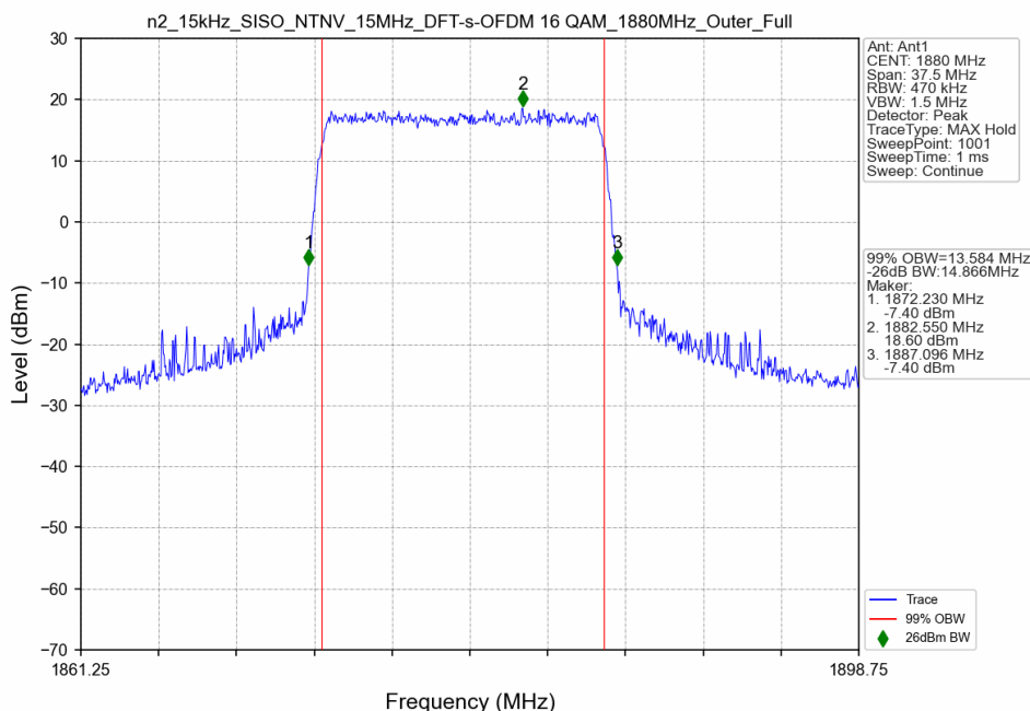
n2_15kHz_SISO_NTNV_15MHz_DFT-s-OFDM 16 QAM_1880MHz_Outer_Full
