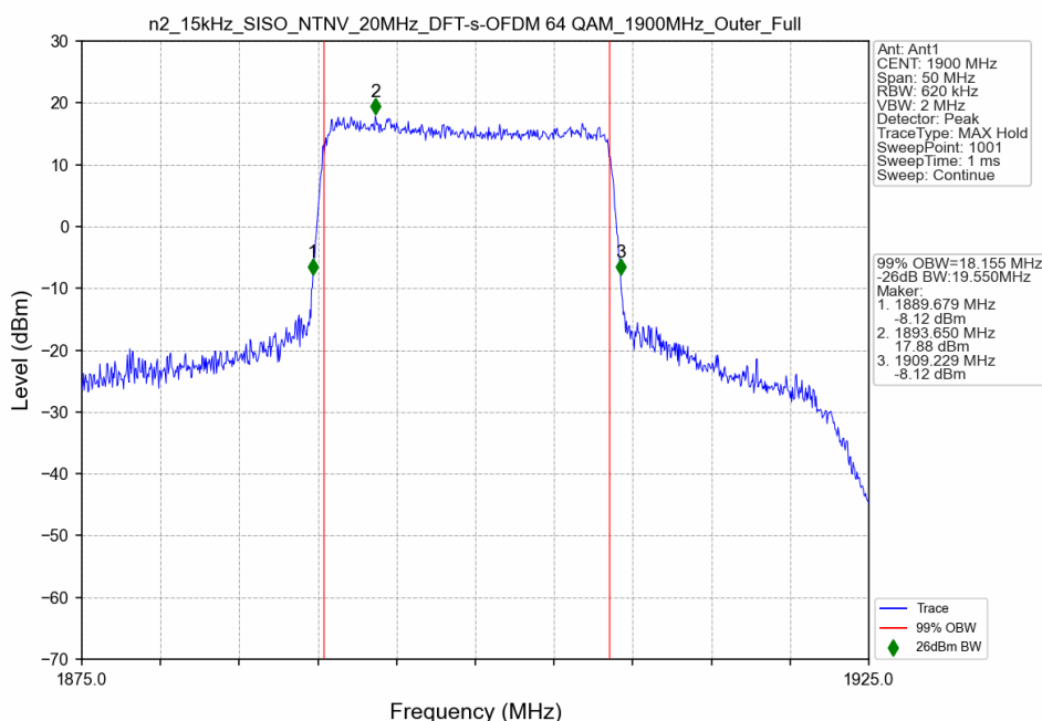
n2_15kHz_SISO_NTNV_20MHz_DFT-s-OFDM 64 QAM_1900MHz_Outer_Full
