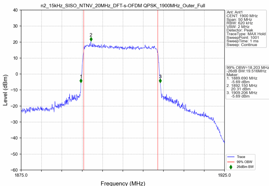
n2_15kHz_SISO_NTNV_20MHz_DFT-s-OFDM QPSK_1900MHz_Outer_Full
