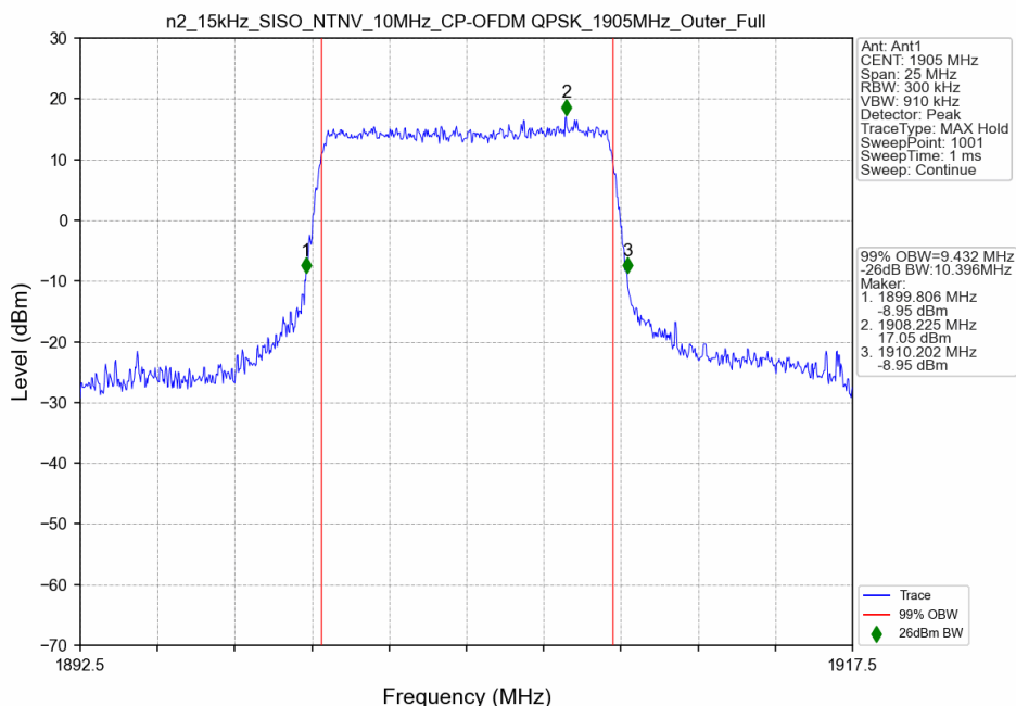
n2_15kHz_SISO_NTNV_10MHz_CP-OFDM QPSK_1905MHz_Outer_Full
