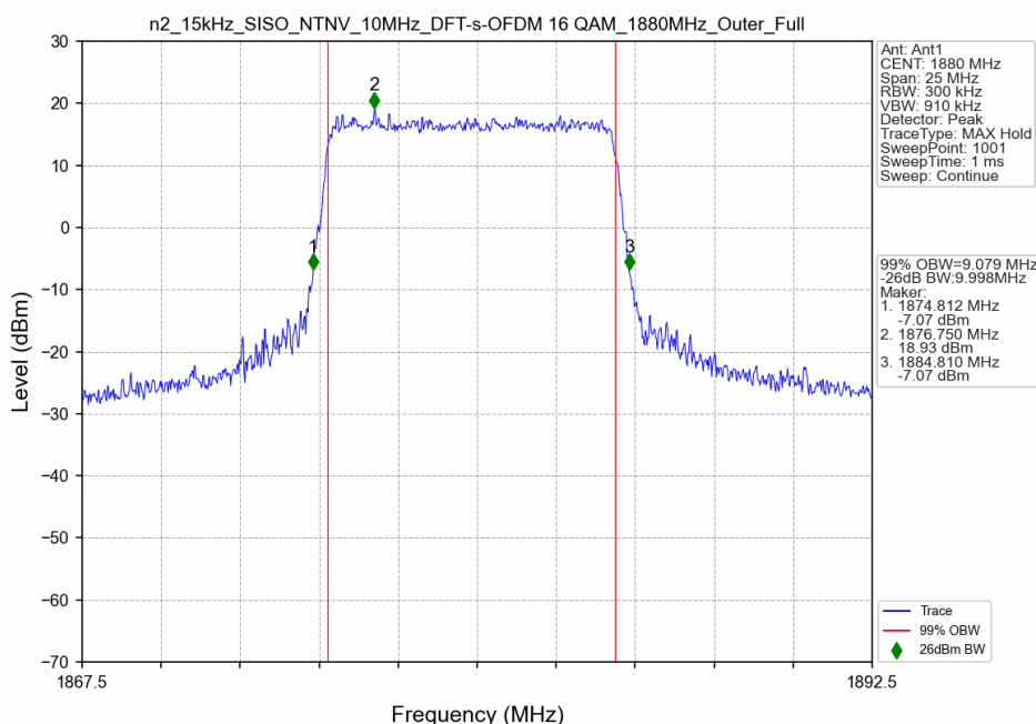
n2_15kHz_SISO_NTNV_10MHz_DFT-s-OFDM 16 QAM_1880MHz_Outer_Full
