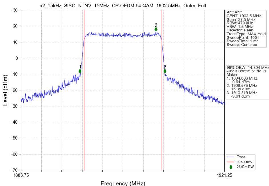
n2_15kHz_SISO_NTNV_15MHz_CP-OFDM 64 QAM_1902.5MHz_Outer_Full
