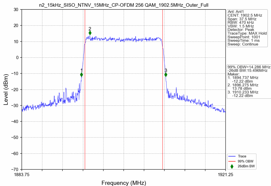
n2_15kHz_SISO_NTNV_15MHz_CP-OFDM 256 QAM_1902.5MHz_Outer_Full
