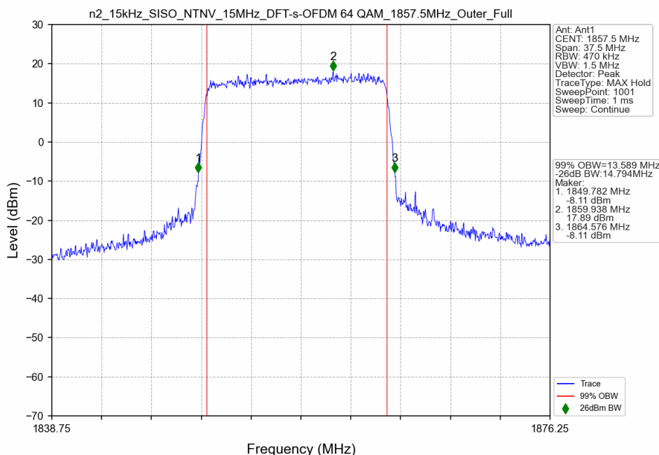
n2_15kHz_SISO_NTNV_15MHz_DFT-s-OFDM 64 QAM_1857.5MHz_Outer_Full
