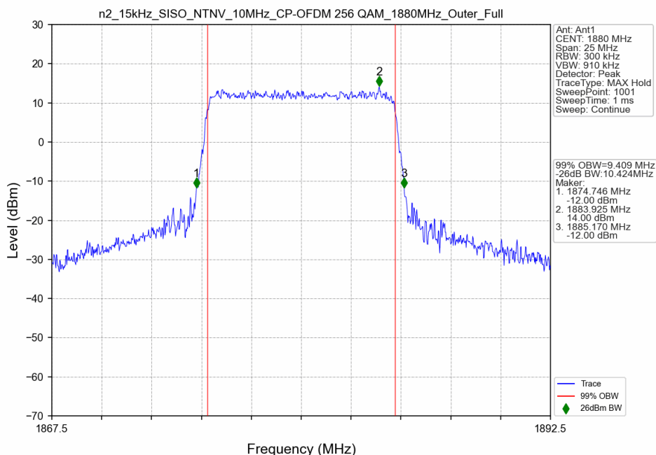
n2_15kHz_SISO_NTNV_10MHz_CP-OFDM 256 QAM_1880MHz_Outer_Full
