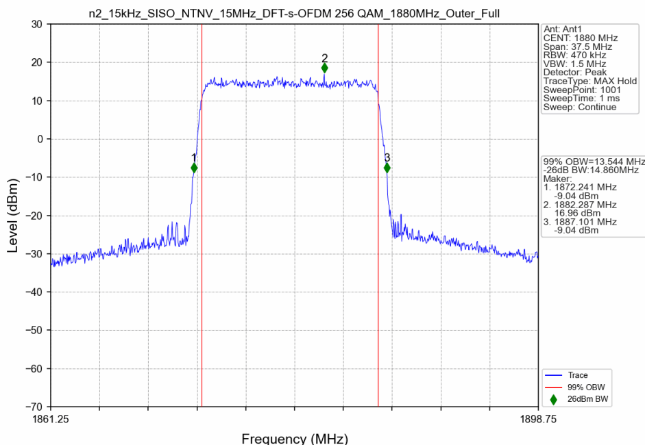
n2_15kHz_SISO_NTNV_15MHz_DFT-s-OFDM 256 QAM_1880MHz_Outer_Full
