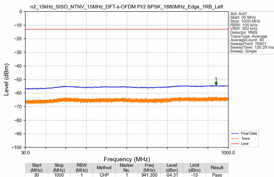
n2_15kHz_SISO_NTNV_15MHz_DFT-s-OFDM PI/2 BPSK_1880MHz_Edge_1RB_Left
