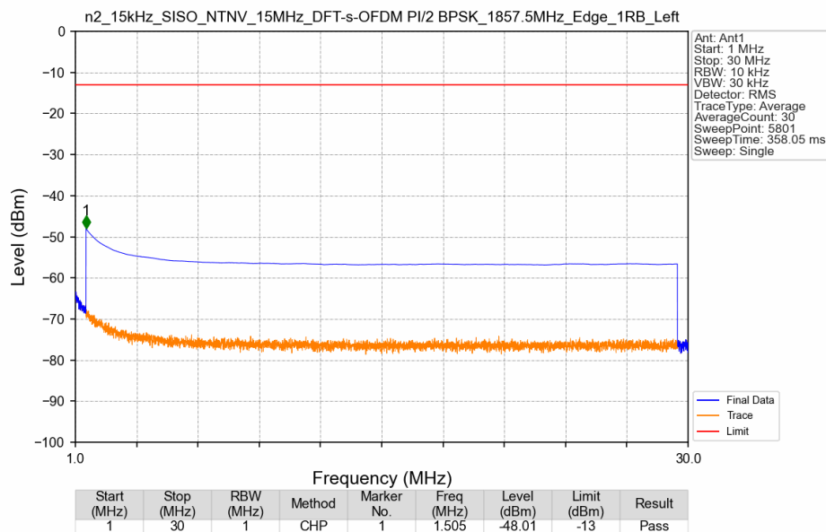
n2_15kHz_SISO_NTNV_15MHz_DFT-s-OFDM PI/2 BPSK_1857.5MHz_Edge_1RB_Left
