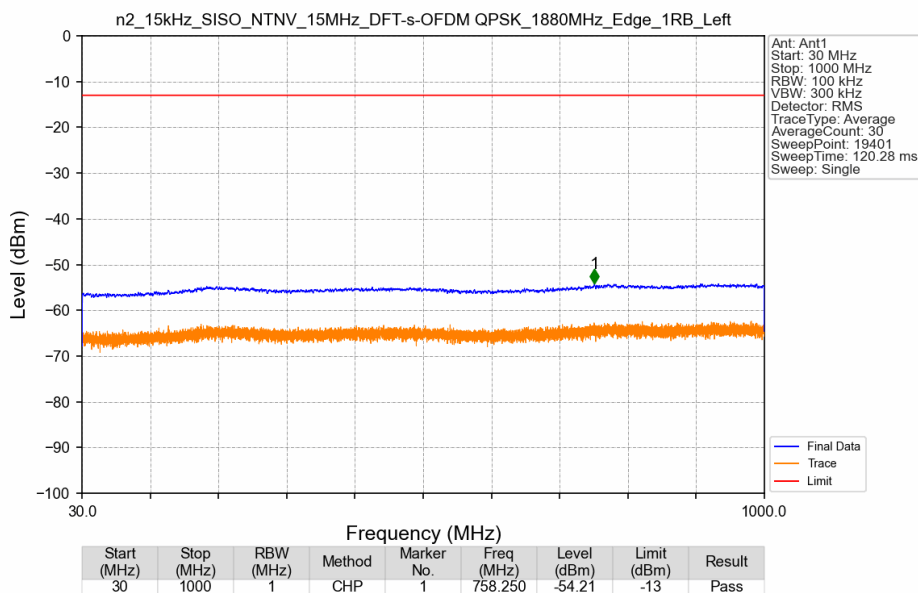
n2_15kHz_SISO_NTNV_15MHz_DFT-s-OFDM QPSK_1880MHz_Edge_1RB_Left
