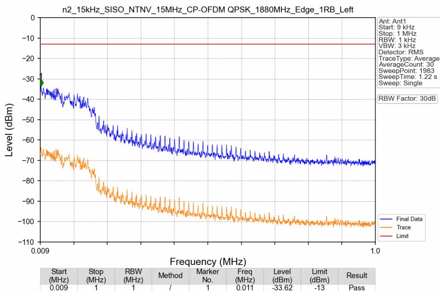
n2_15kHz_SISO_NTNV_15MHz_CP-OFDM QPSK_1880MHz_Edge_1RB_Left
