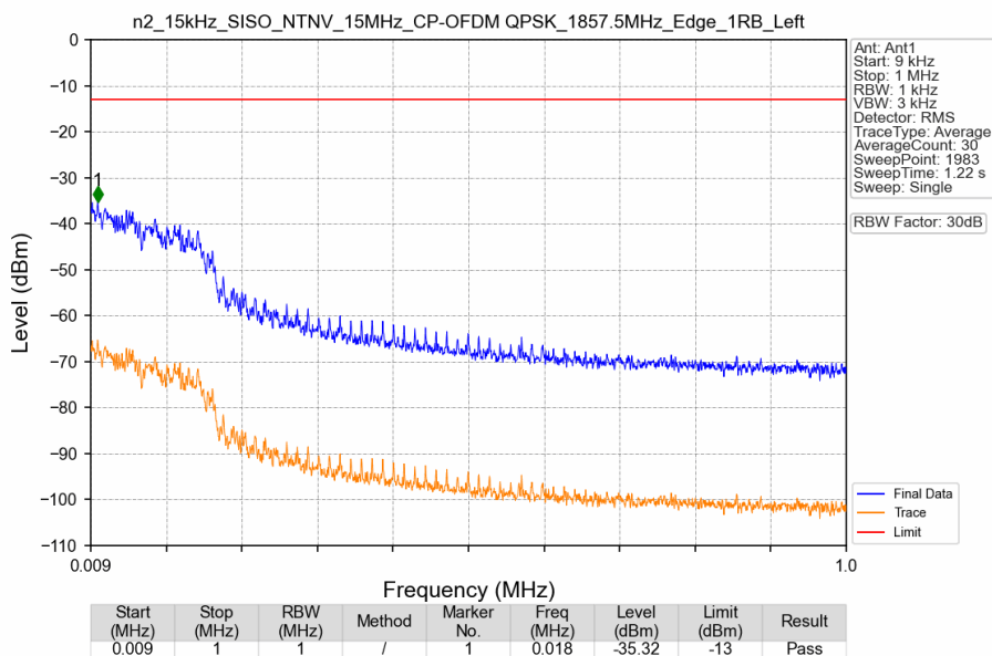
n2_15kHz_SISO_NTNV_15MHz_CP-OFDM QPSK_1857.5MHz_Edge_1RB_Left
