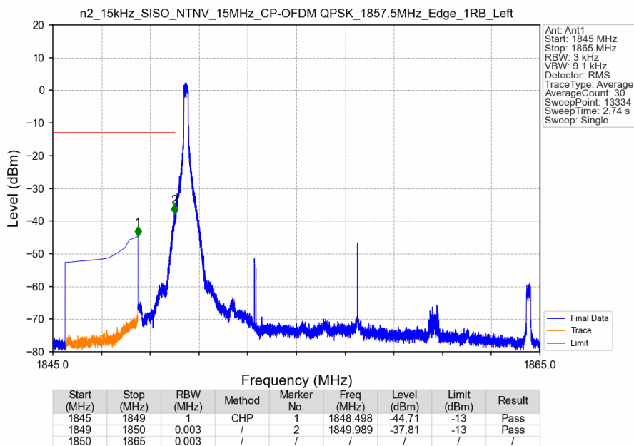
n2_15kHz_SISO_NTNV_15MHz_CP-OFDM QPSK_1857.5MHz_Edge_1RB_Left
