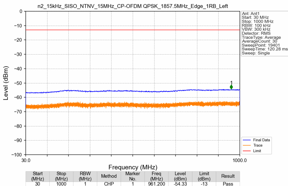
n2_15kHz_SISO_NTNV_15MHz_CP-OFDM QPSK_1857.5MHz_Edge_1RB_Left
