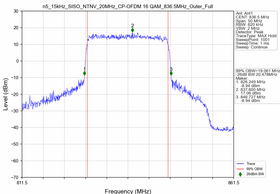
n5_15kHz_SISO_NTNV_20MHz_CP-OFDM 16 QAM_836.5MHz_Outer_Full
