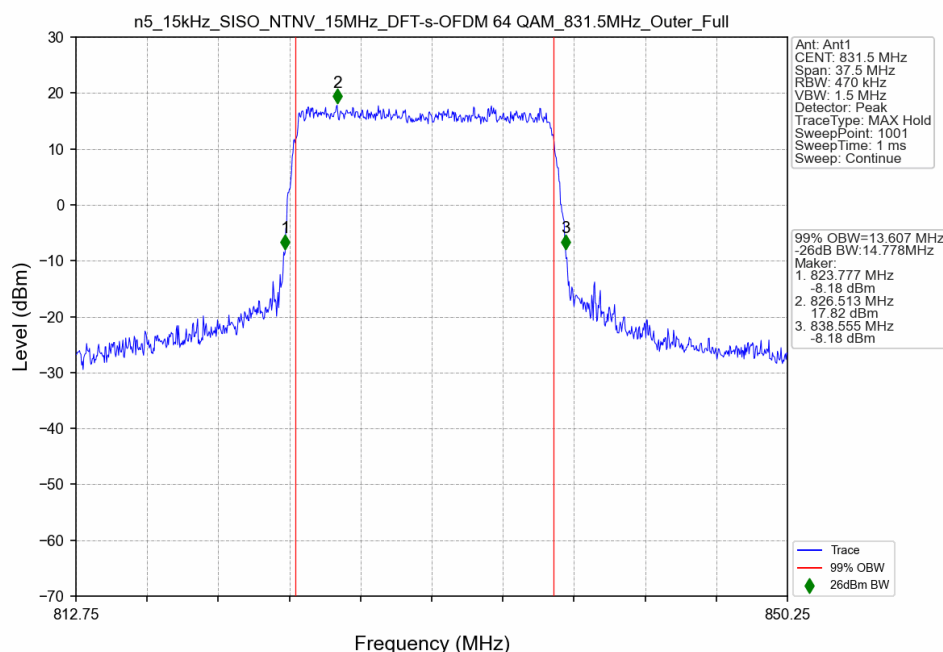
n5_15kHz_SISO_NTNV_15MHz_DFT-s-OFDM 64 QAM_831.5MHz_Outer_Full
