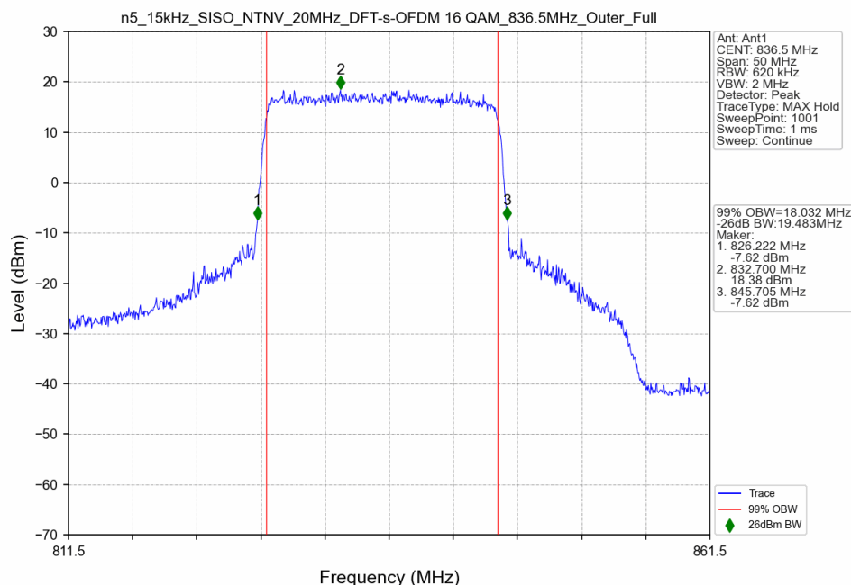
n5_15kHz_SISO_NTNV_20MHz_DFT-s-OFDM 16 QAM_836.5MHz_Outer_Full
