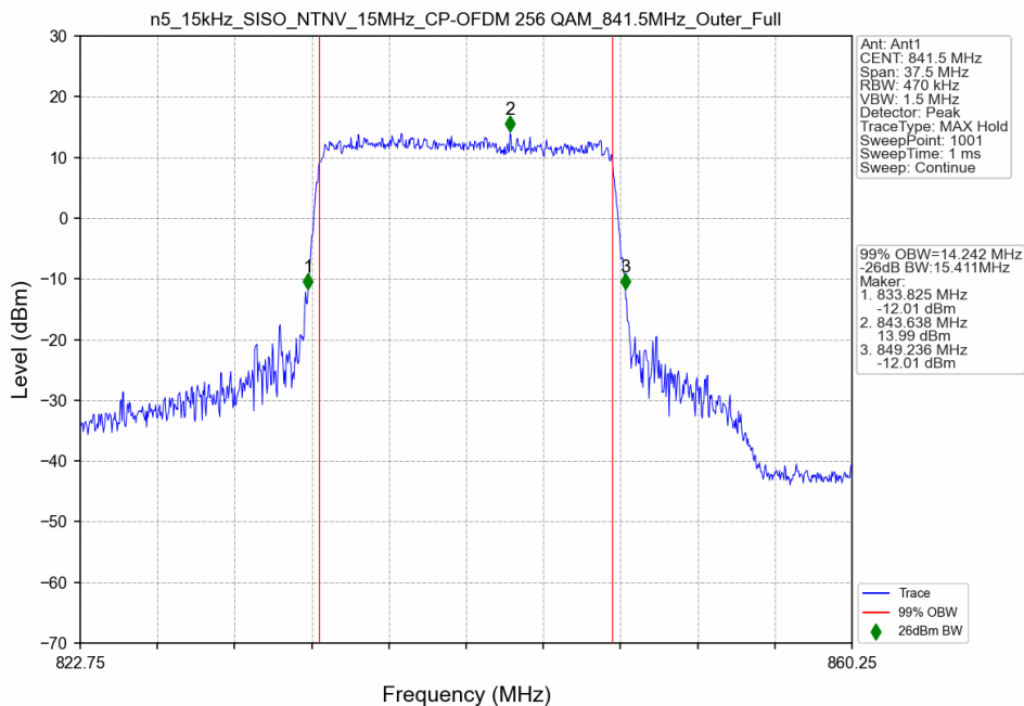
n5_15kHz_SISO_NTNV_15MHz_CP-OFDM 256 QAM_841.5MHz_Outer_Full
