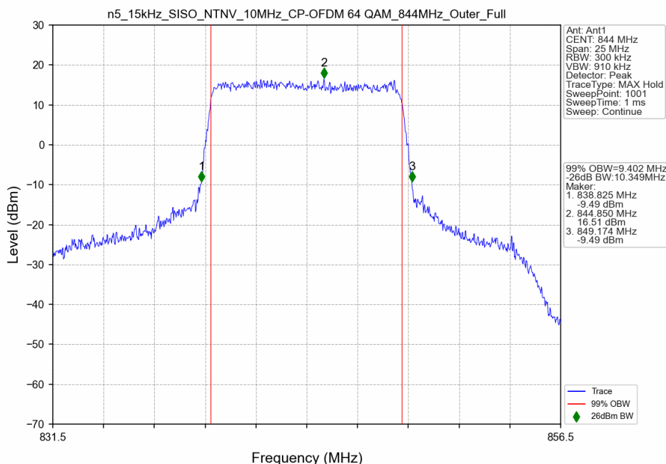
n5_15kHz_SISO_NTNV_10MHz_CP-OFDM 64 QAM_844MHz_Outer_Full
