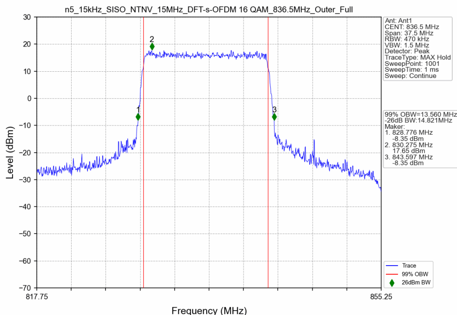
n5_15kHz_SISO_NTNV_15MHz_DFT-s-OFDM 16 QAM_836.5MHz_Outer_Full
