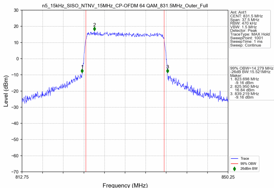
n5_15kHz_SISO_NTNV_15MHz_CP-OFDM 64 QAM_831.5MHz_Outer_Full
