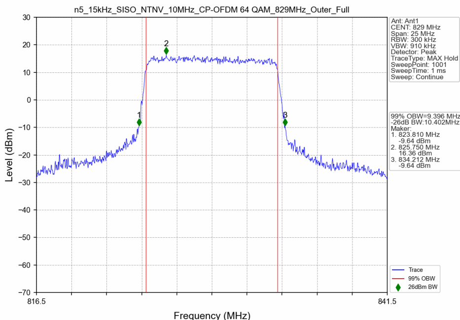
n5_15kHz_SISO_NTNV_10MHz_CP-OFDM 64 QAM_829MHz_Outer_Full
