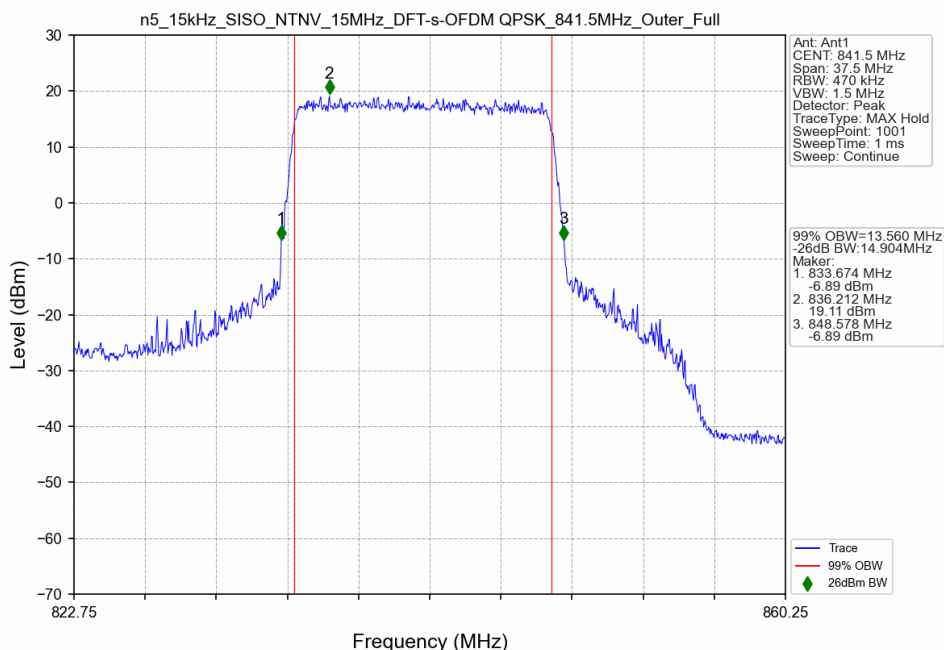
n5_15kHz_SISO_NTNV_15MHz_DFT-s-OFDM QPSK_841.5MHz_Outer_Full
