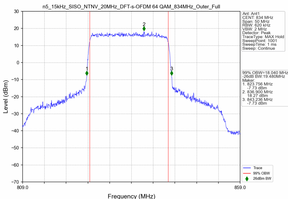
n5_15kHz_SISO_NTNV_20MHz_DFT-s-OFDM 64 QAM_834MHz_Outer_Full
