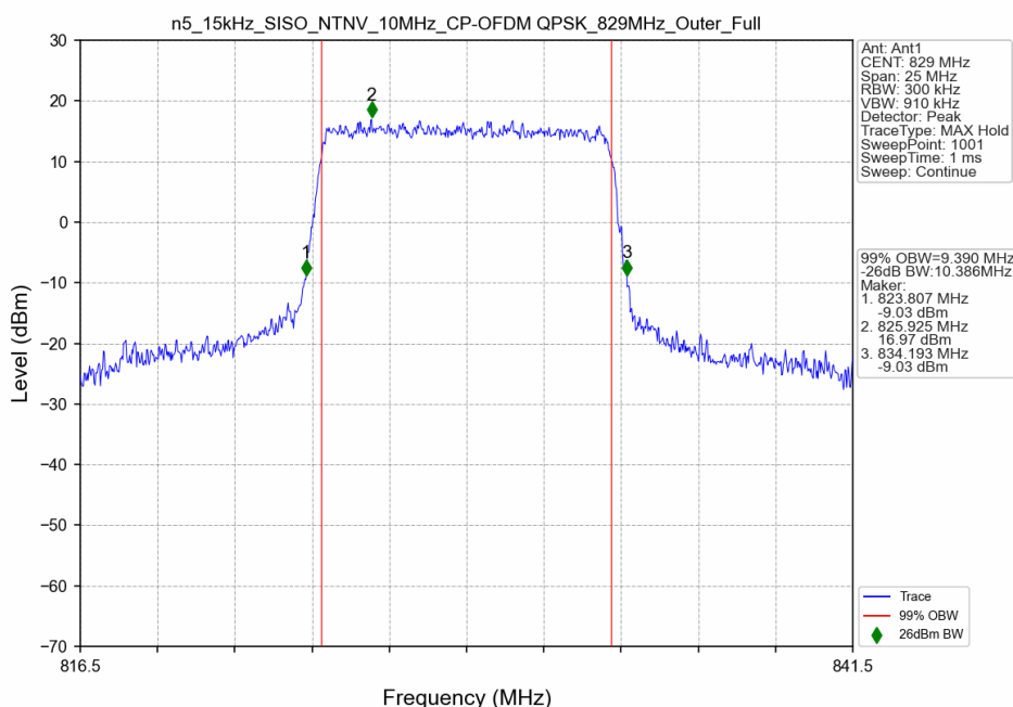
n5_15kHz_SISO_NTNV_10MHz_CP-OFDM QPSK_829MHz_Outer_Full
