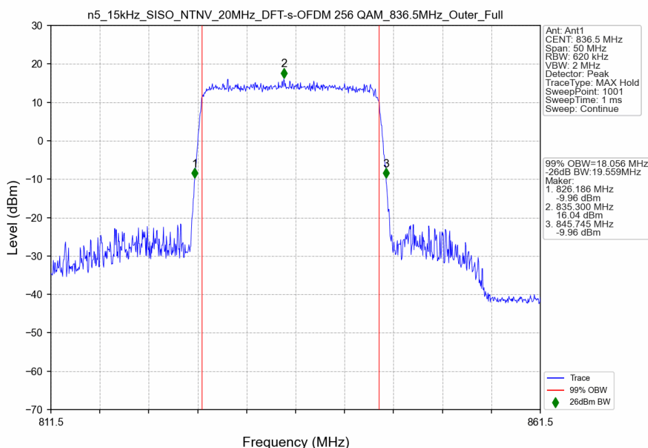
n5_15kHz_SISO_NTNV_20MHz_DFT-s-OFDM 256 QAM_836.5MHz_Outer_Full
