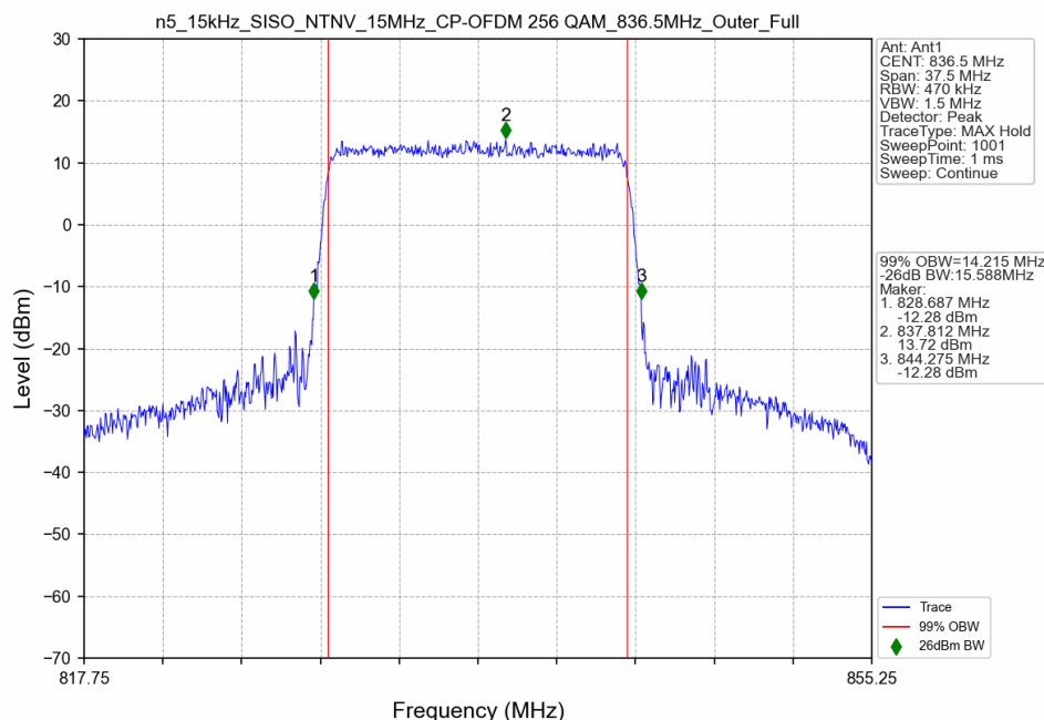
n5_15kHz_SISO_NTNV_15MHz_CP-OFDM 256 QAM_836.5MHz_Outer_Full
