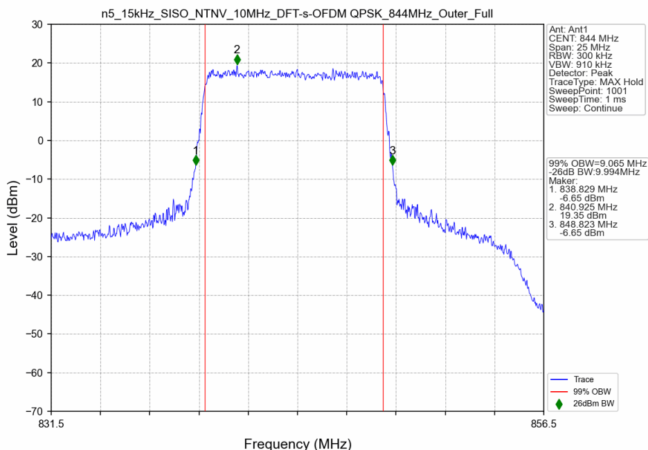
n5_15kHz_SISO_NTNV_10MHz_DFT-s-OFDM QPSK_844MHz_Outer_Full
