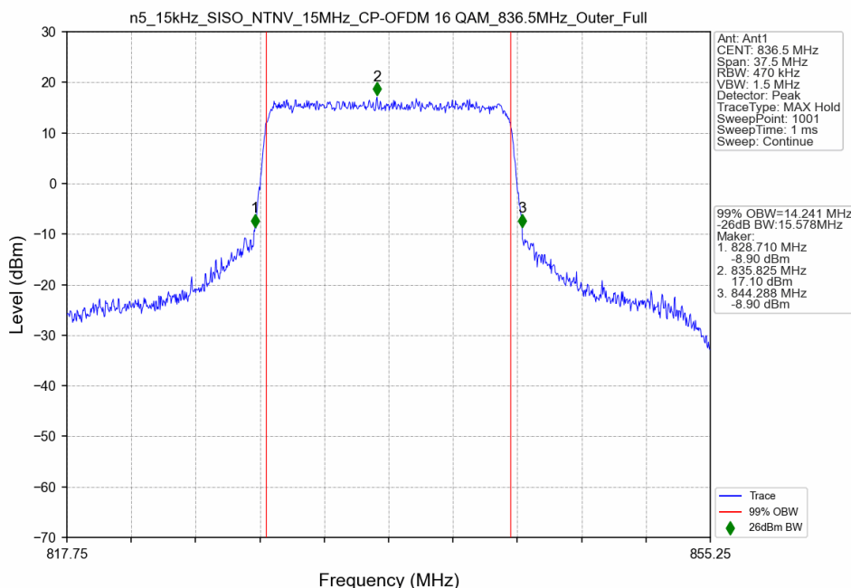
n5_15kHz_SISO_NTNV_15MHz_CP-OFDM 16 QAM_836.5MHz_Outer_Full
