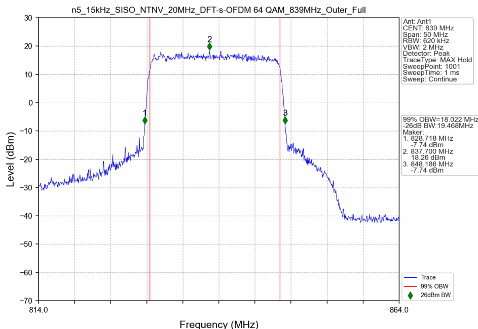
n5_15kHz_SISO_NTNV_20MHz_DFT-s-OFDM 64 QAM_839MHz_Outer_Full
