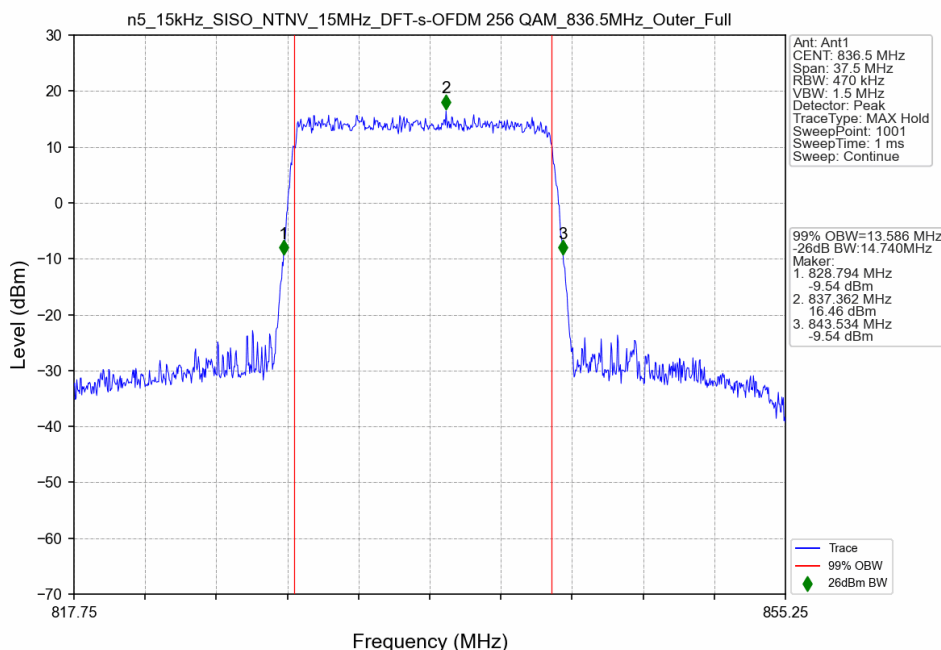
n5_15kHz_SISO_NTNV_15MHz_DFT-s-OFDM 256 QAM_836.5MHz_Outer_Full
