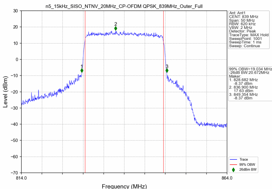
n5_15kHz_SISO_NTNV_20MHz_CP-OFDM QPSK_839MHz_Outer_Full
