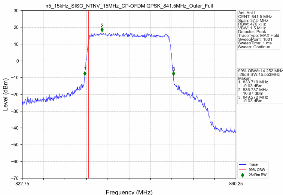
n5_15kHz_SISO_NTNV_15MHz_CP-OFDM QPSK_841.5MHz_Outer_Full
