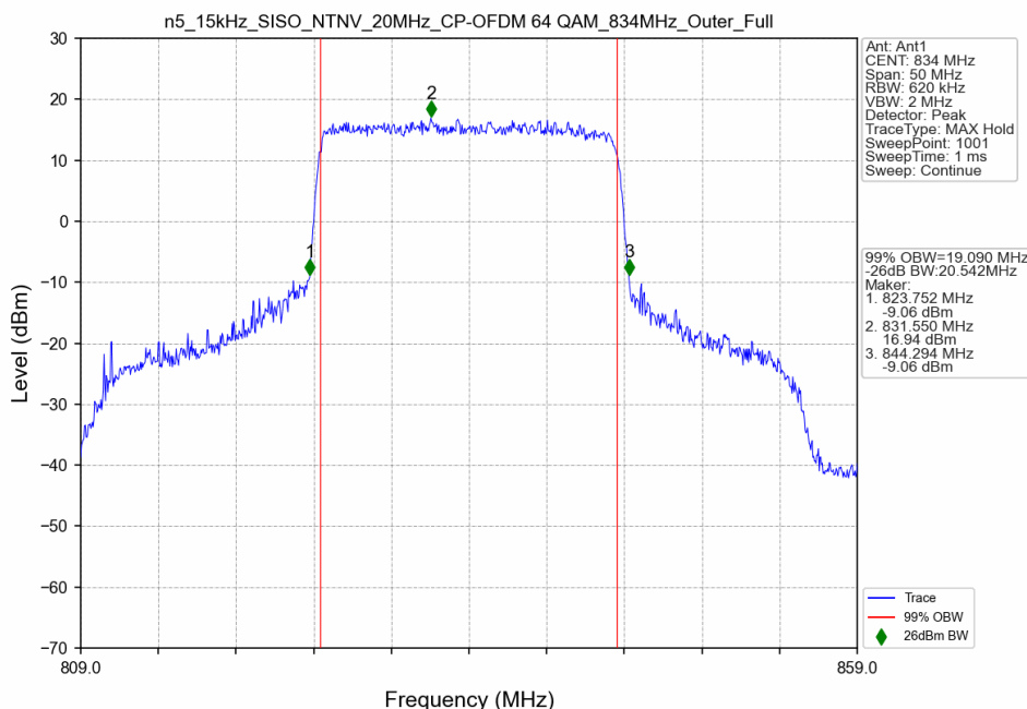
n5_15kHz_SISO_NTNV_20MHz_CP-OFDM 64 QAM_834MHz_Outer_Full
