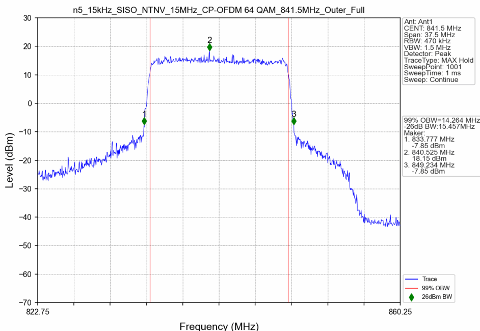
n5_15kHz_SISO_NTNV_15MHz_CP-OFDM 64 QAM_841.5MHz_Outer_Full
