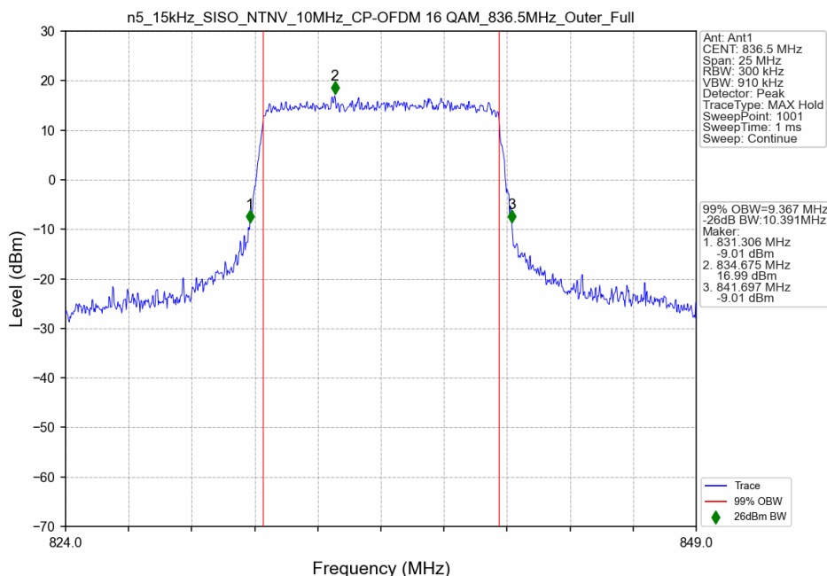
n5_15kHz_SISO_NTNV_10MHz_CP-OFDM 16 QAM_836.5MHz_Outer_Full
