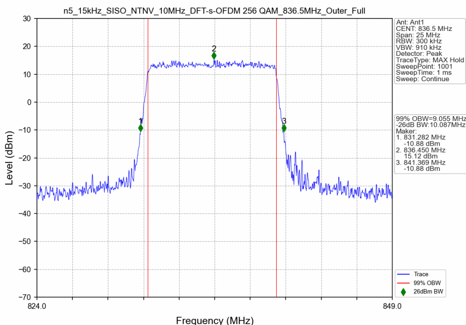
n5_15kHz_SISO_NTNV_10MHz_DFT-s-OFDM 256 QAM_836.5MHz_Outer_Full
