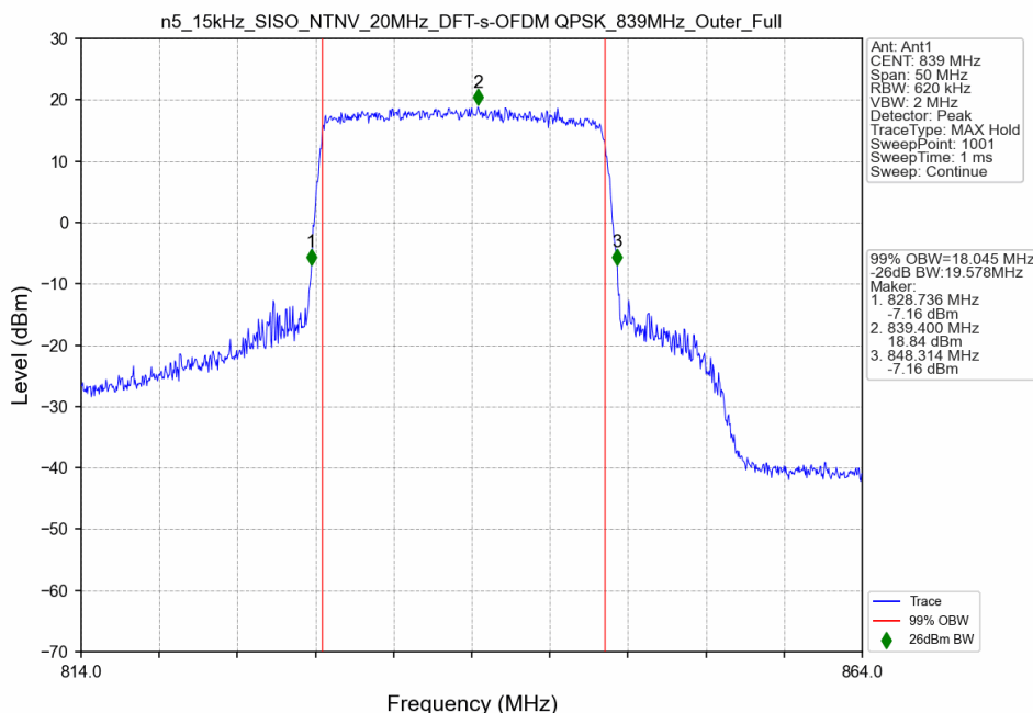
n5_15kHz_SISO_NTNV_20MHz_DFT-s-OFDM QPSK_839MHz_Outer_Full
