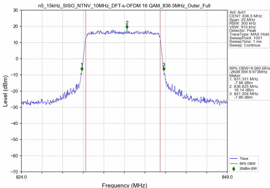
n5_15kHz_SISO_NTNV_10MHz_DFT-s-OFDM 16 QAM_836.5MHz_Outer_Full
