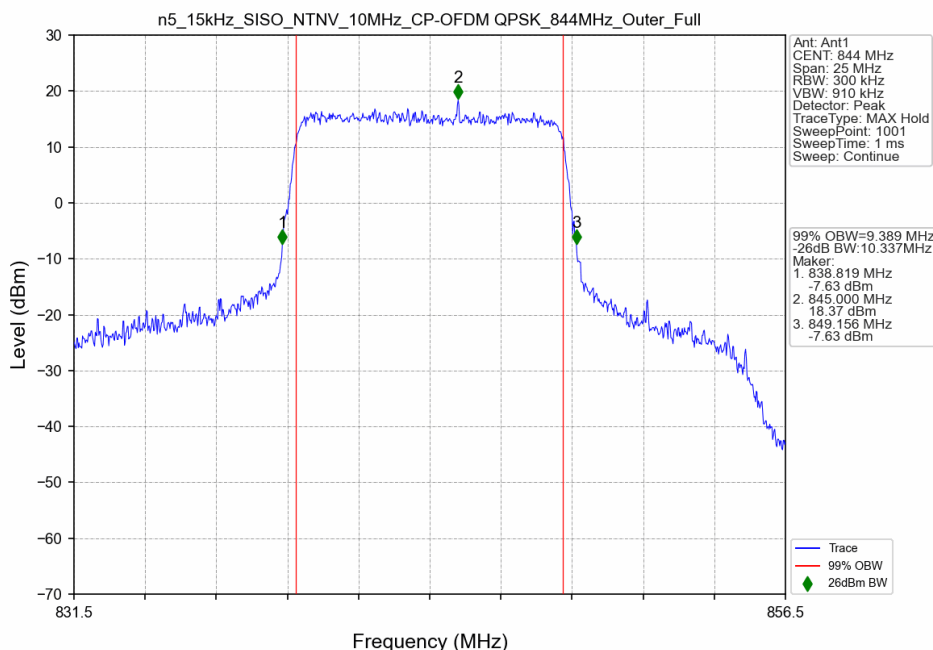
n5_15kHz_SISO_NTNV_10MHz_CP-OFDM QPSK_844MHz_Outer_Full
