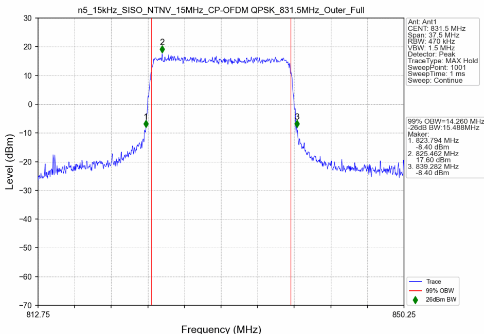
n5_15kHz_SISO_NTNV_15MHz_CP-OFDM QPSK_831.5MHz_Outer_Full
