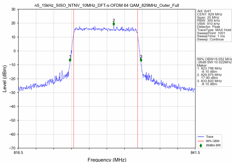
n5_15kHz_SISO_NTNV_10MHz_DFT-s-OFDM 64 QAM_829MHz_Outer_Full
