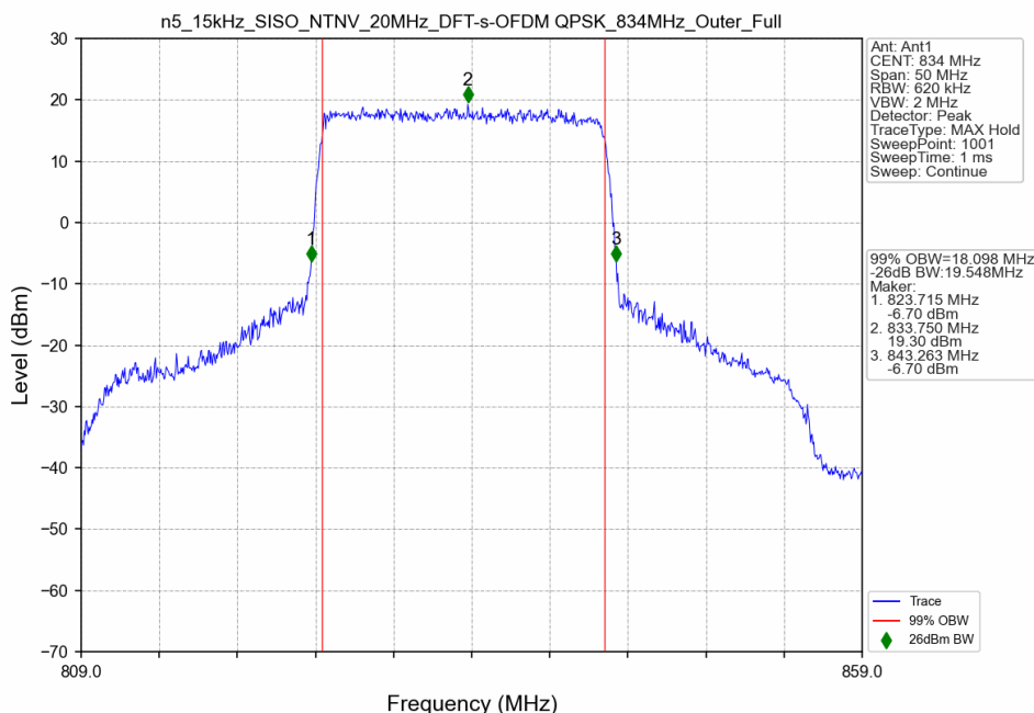
n5_15kHz_SISO_NTNV_20MHz_DFT-s-OFDM QPSK_834MHz_Outer_Full
