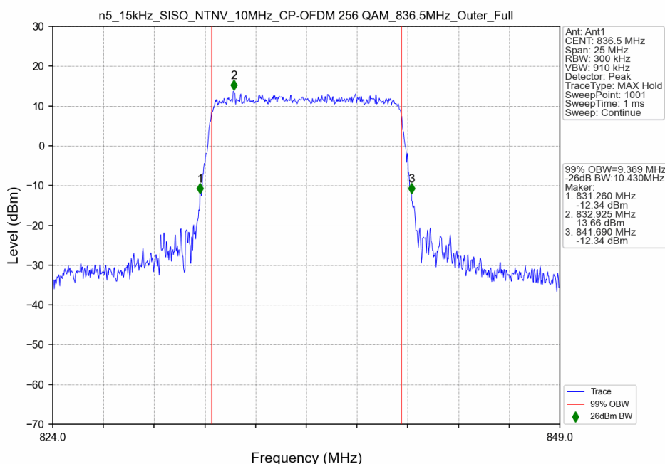
n5_15kHz_SISO_NTNV_10MHz_CP-OFDM 256 QAM_836.5MHz_Outer_Full
