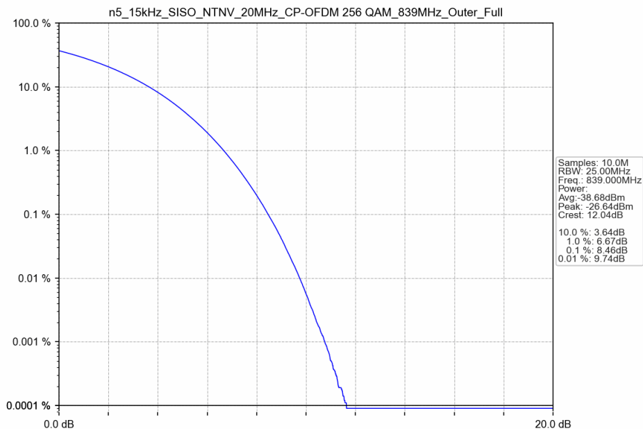
n5_15kHz_SISO_NTNV_20MHz_CP-OFDM 256 QAM_839MHz_Outer_Full
