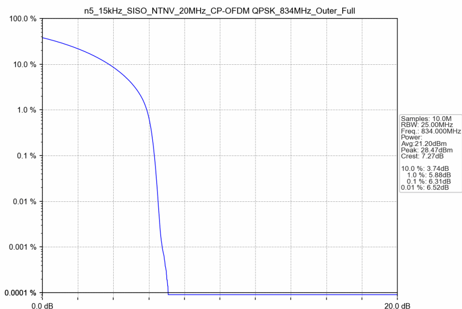
n5_15kHz_SISO_NTNV_20MHz_CP-OFDM QPSK_834MHz_Outer_Full
