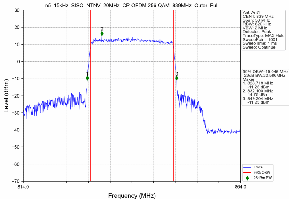
n5_15kHz_SISO_NTNV_20MHz_CP-OFDM 256 QAM_839MHz_Outer_Full
