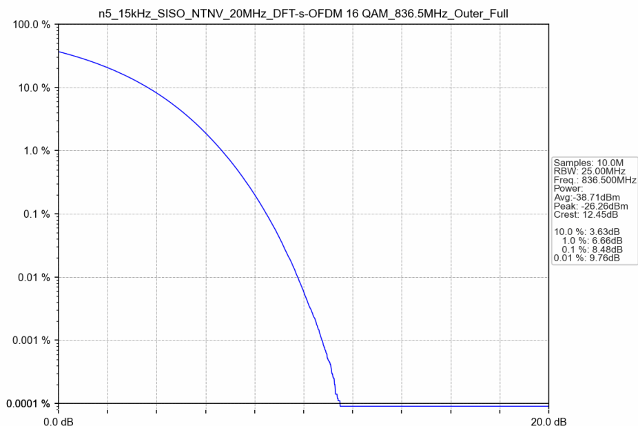
n5_15kHz_SISO_NTNV_20MHz_DFT-s-OFDM 16 QAM_836.5MHz_Outer_Full
