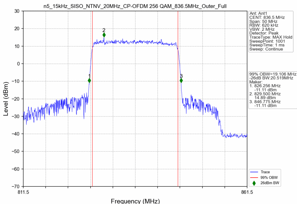
n5_15kHz_SISO_NTNV_20MHz_CP-OFDM 256 QAM_836.5MHz_Outer_Full
