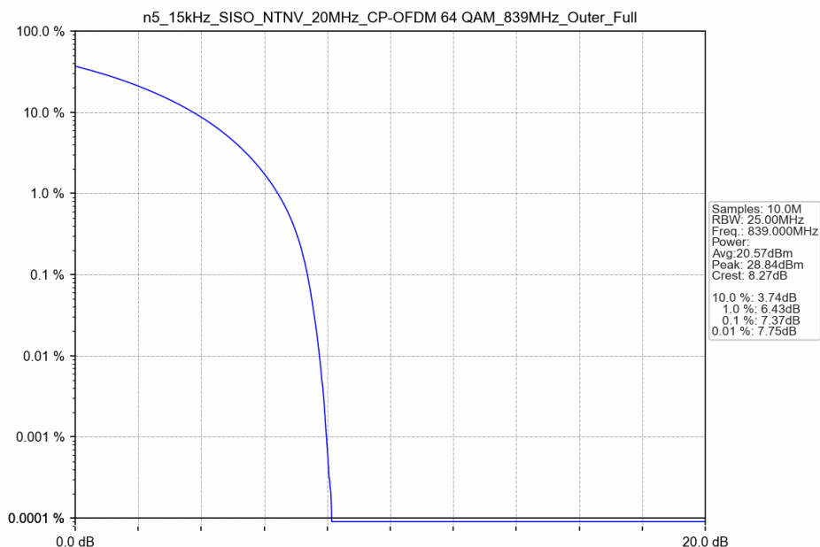
n5_15kHz_SISO_NTNV_20MHz_CP-OFDM 64 QAM_839MHz_Outer_Full
