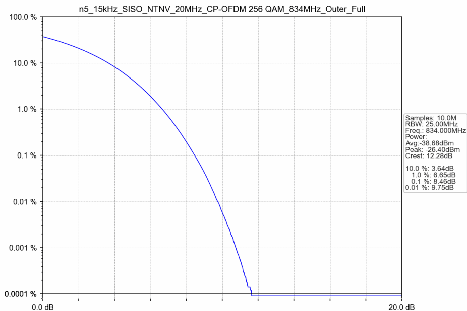
n5_15kHz_SISO_NTNV_20MHz_CP-OFDM 256 QAM_834MHz_Outer_Full
