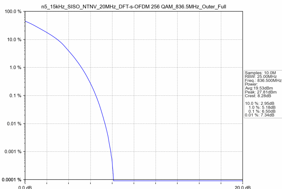
n5_15kHz_SISO_NTNV_20MHz_DFT-s-OFDM 256 QAM_836.5MHz_Outer_Full
