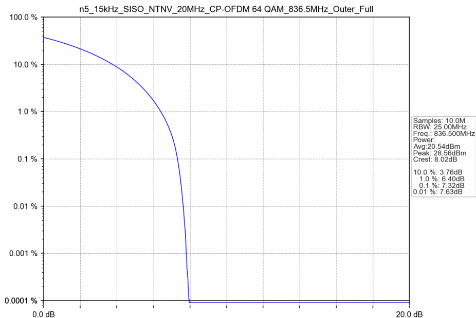
n5_15kHz_SISO_NTNV_20MHz_CP-OFDM 64 QAM_836.5MHz_Outer_Full
