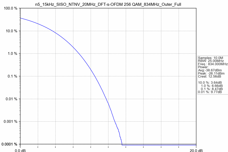
n5_15kHz_SISO_NTNV_20MHz_DFT-s-OFDM 256 QAM_834MHz_Outer_Full
