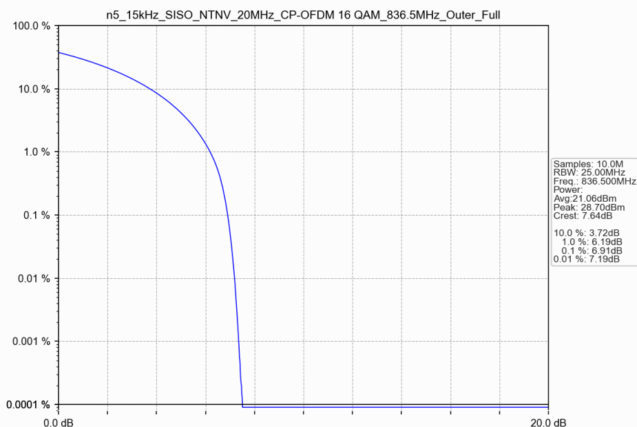
n5_15kHz_SISO_NTNV_20MHz_CP-OFDM 16 QAM_836.5MHz_Outer_Full
