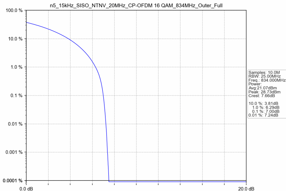
n5_15kHz_SISO_NTNV_20MHz_CP-OFDM 16 QAM_834MHz_Outer_Full
