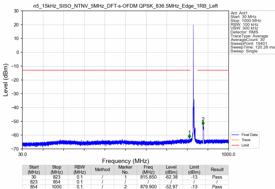
n5_15kHz_SISO_NTNV_5MHz_DFT-s-OFDM QPSK_836.5MHz_Edge_1RB_Left
