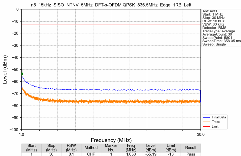
n5_15kHz_SISO_NTNV_5MHz_DFT-s-OFDM QPSK_836.5MHz_Edge_1RB_Left
