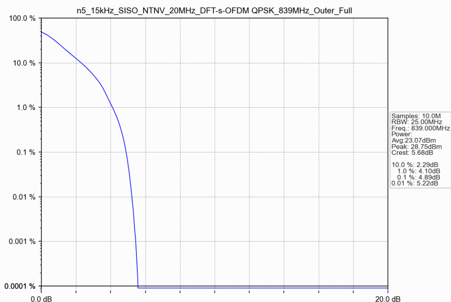
n5_15kHz_SISO_NTNV_20MHz_DFT-s-OFDM QPSK_839MHz_Outer_Full
