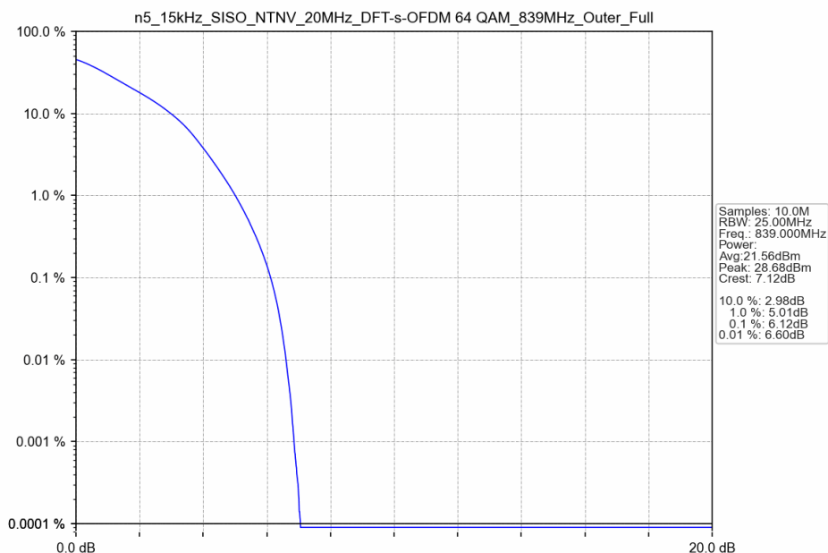
n5_15kHz_SISO_NTNV_20MHz_DFT-s-OFDM 64 QAM_839MHz_Outer_Full
