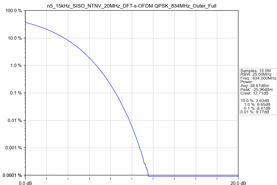
n5_15kHz_SISO_NTNV_20MHz_DFT-s-OFDM QPSK_834MHz_Outer_Full
