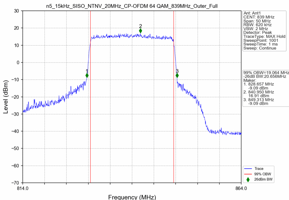
n5_15kHz_SISO_NTNV_20MHz_CP-OFDM 64 QAM_839MHz_Outer_Full
