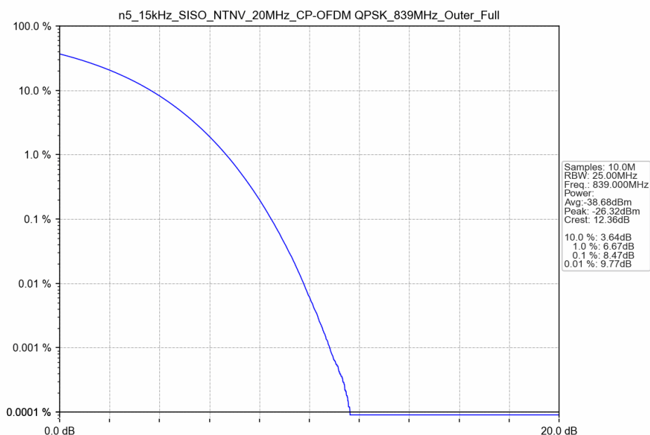
n5_15kHz_SISO_NTNV_20MHz_CP-OFDM QPSK_839MHz_Outer_Full
